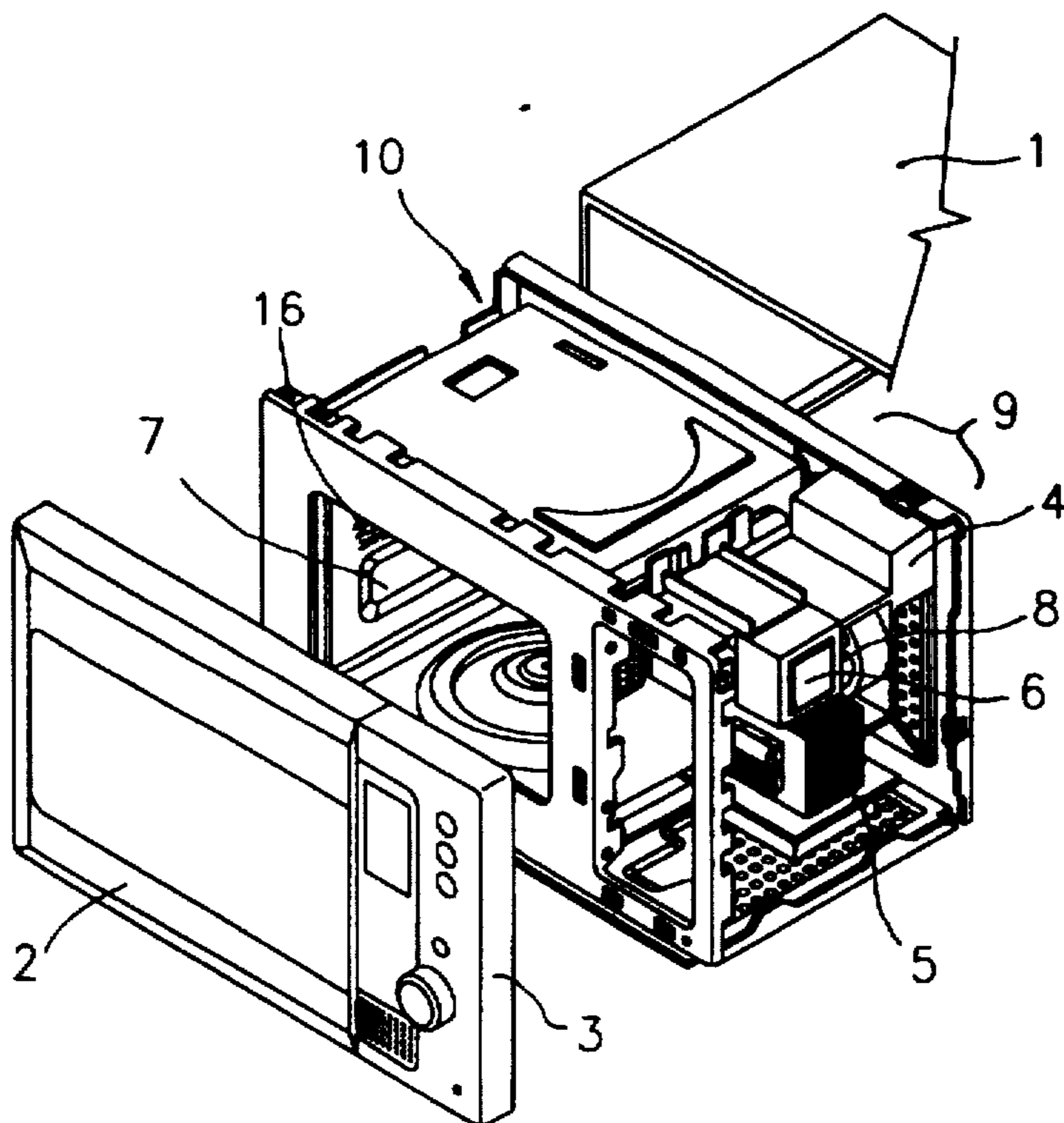
FIG. 1 CONVENTIONAL ART
