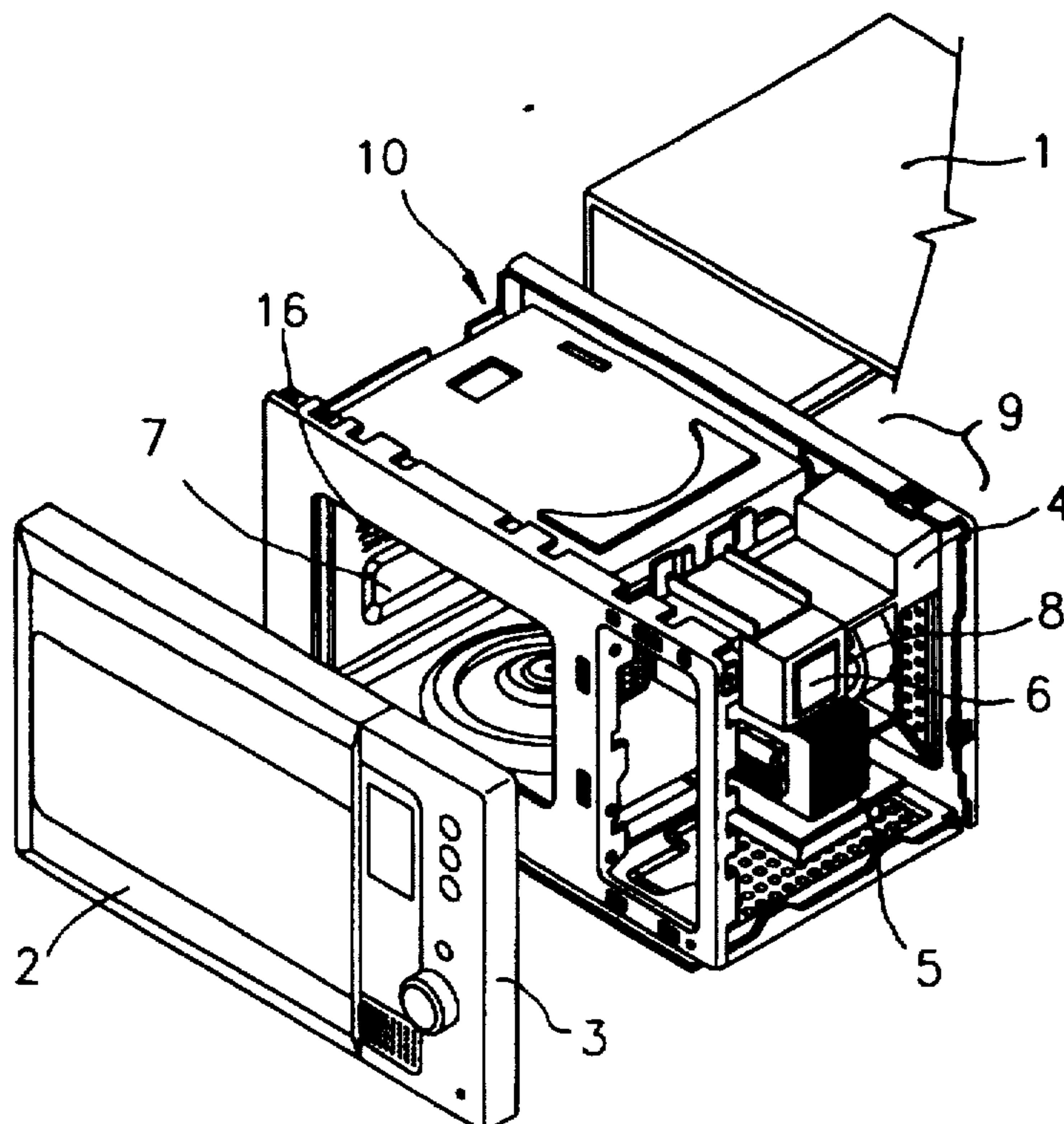
FIG. 1 CONVENTIONAL ART
