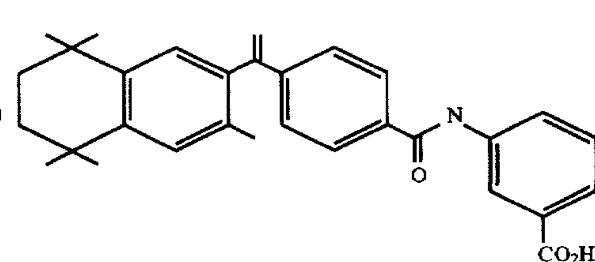
4-[1-(3,5,5,8,8-pentamethyl-5,6,7,8-tetrahydro-
