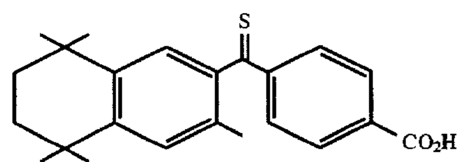
thioketone
