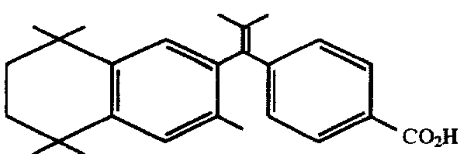
4-[1-(3,5,5,8,8-pentamethyl-5,6,7,8-tetrahydro-
