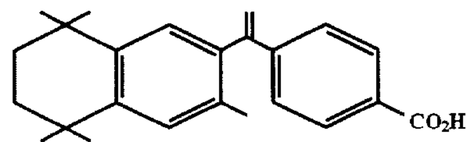
3-methyl-TTNEB
