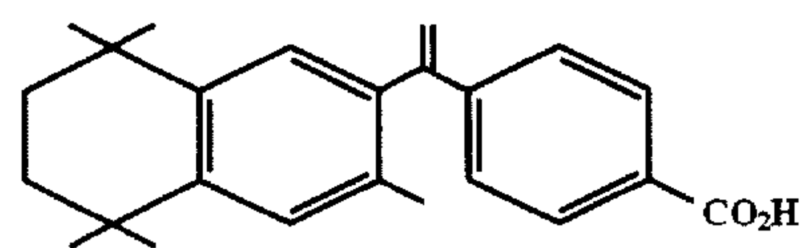
3-methyl-TTNEB
