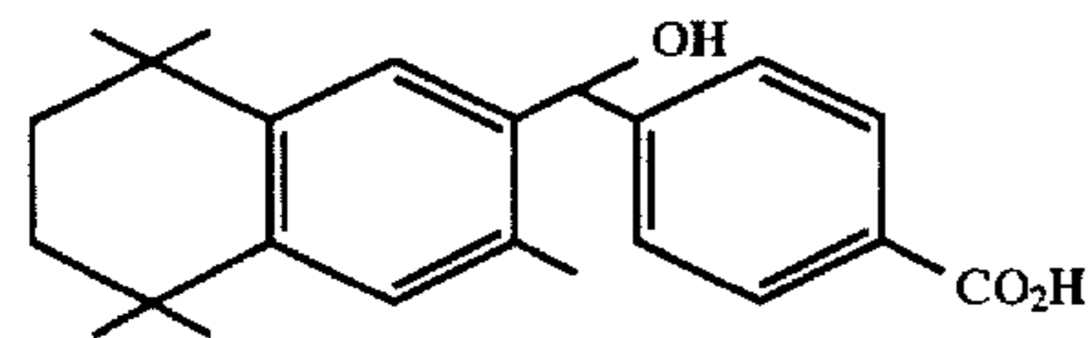
3-methyl-TTNHMB
