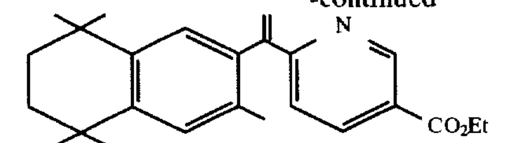
Ethyl-2-[1-(3,5,5,8,8-pentamethyl-5,6,7,8-tetrahydro-2-naphthyl)ethenyl]pyridine-5-carboxylate
