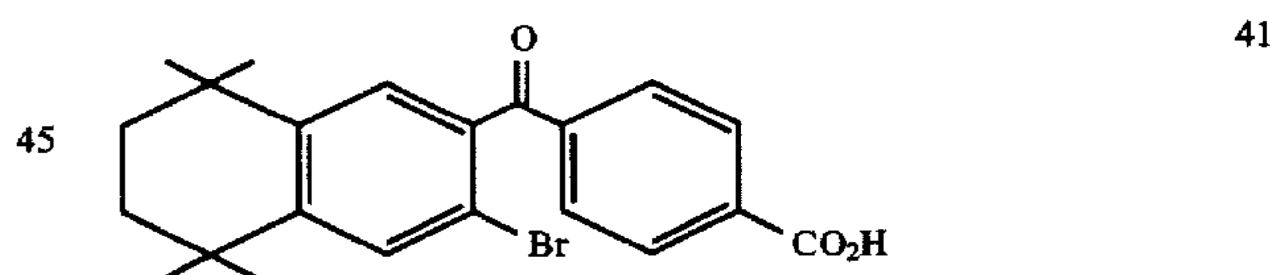
4-[1-(3-bromo-5,5,8,8-tetramethyl-5,6,7,8-tetrahydro-2-naphthyl)carbonyl]benzoic acid(3-bromo-TTNCB)
