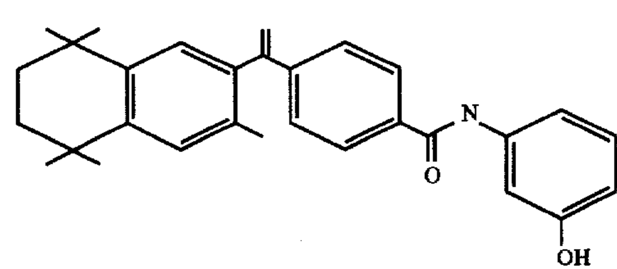
4-[1-(3,5,5,8,8-pentamethyl-5,6,7,8-tetrahydro-2-naphthyl)ethenyl]-N-(2-hydroxyphenyl)benzamide (3-Me-o-TTNEHBP)
