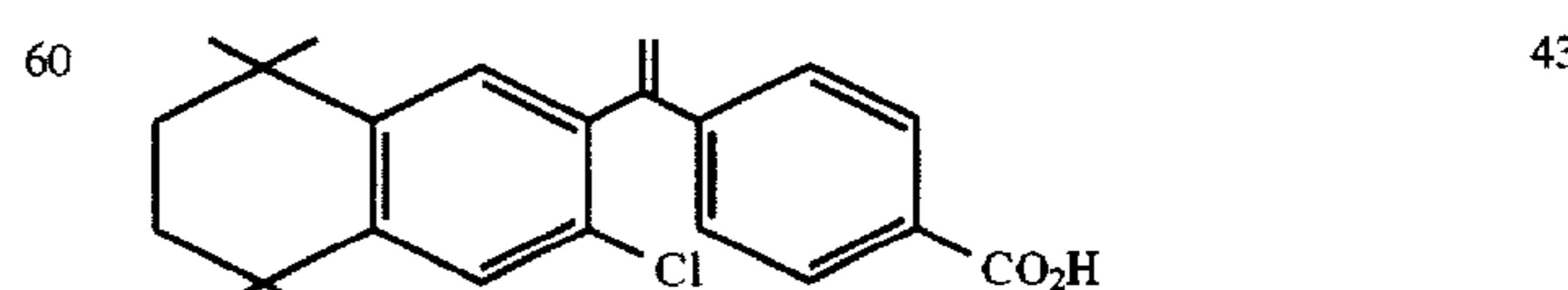
4-[1-(3-chloro-5,5,8,8-tetramethyl-5,6,7,8-tetrahydro-2-naphthyl)ethenyl]benzoic acid(3-chloro-TTNEB)
