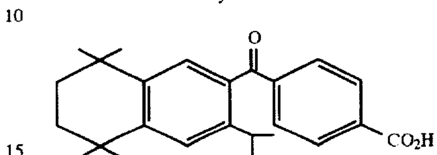
4-[(3-isopropyl-5,5,8,8-tetramethyl-5,6,7,8-tetrahydro-2-naphthyl)carbonyl]benzoic acid(3-IPr-TTNCB)
