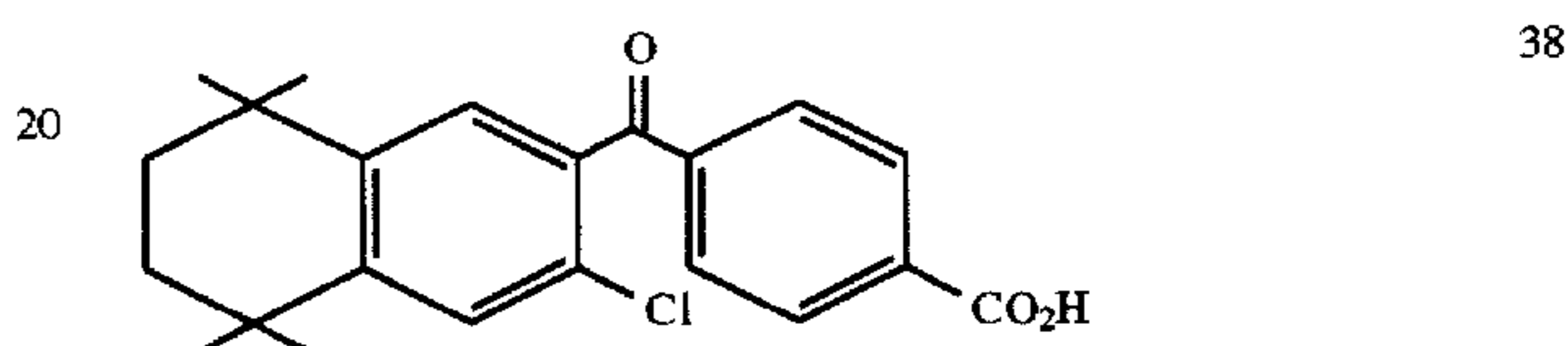
4-[1-(3-chloro-5,5,8,8-tetramethyl-5,6,7,8-tetrahydro-2-naphthyl)carbonyl]benzoic acid(3-chloro-TTNCB)
