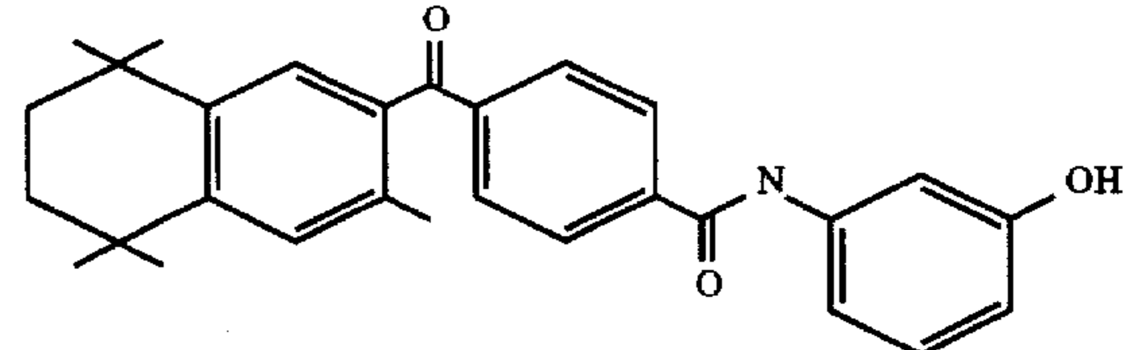
4-[1-(3,5,5,8,8-pentamethyl-5,6,7,8-tetrahydro-2-naphthyl)ethenyl]-N-(3-hydroxyphenyl)benzamide (3-Me-m-TTNEHBP)
