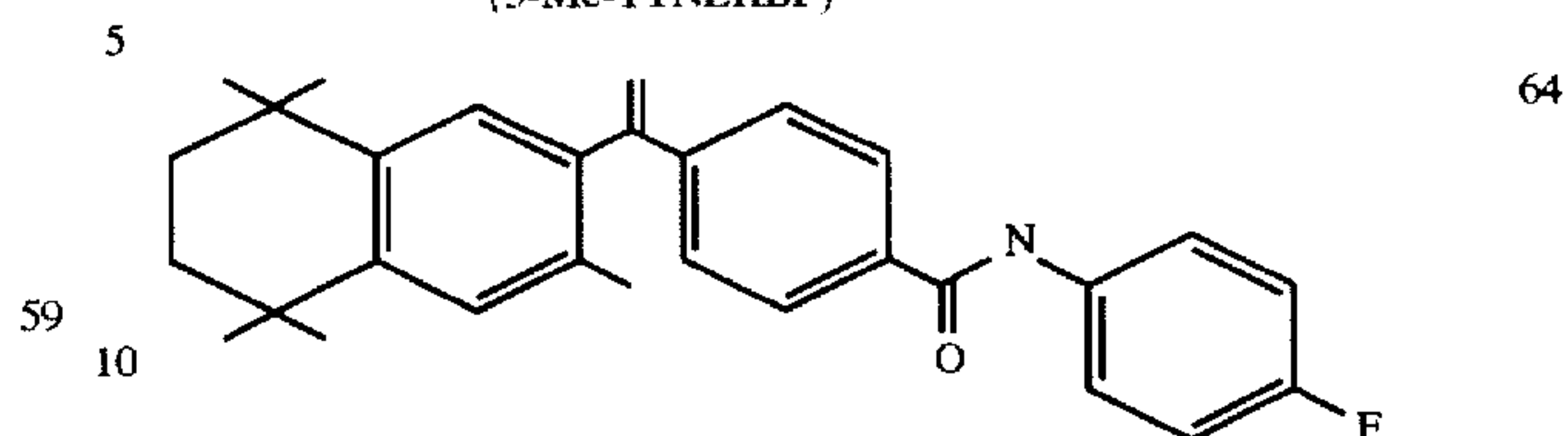
4-[1-(3,5,5,8,8-pentamethyl-5,6,7,8-tetrahydro-2-naphthyl)ethenyl]-N-(4-carboxyphenyl)benzamide (3-Me-TTNECBP)
