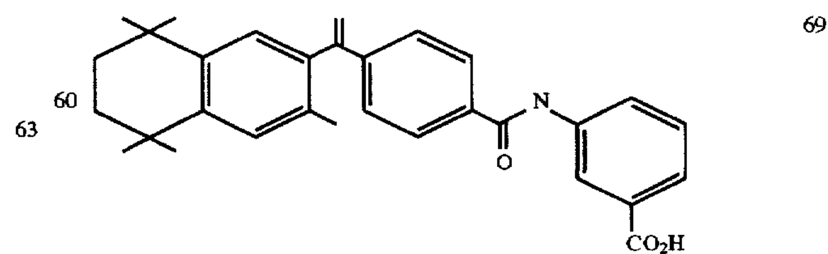
4-[1-(3,5,5,8,8-pentamethyl-5,6,7,8-tetrahydro-
