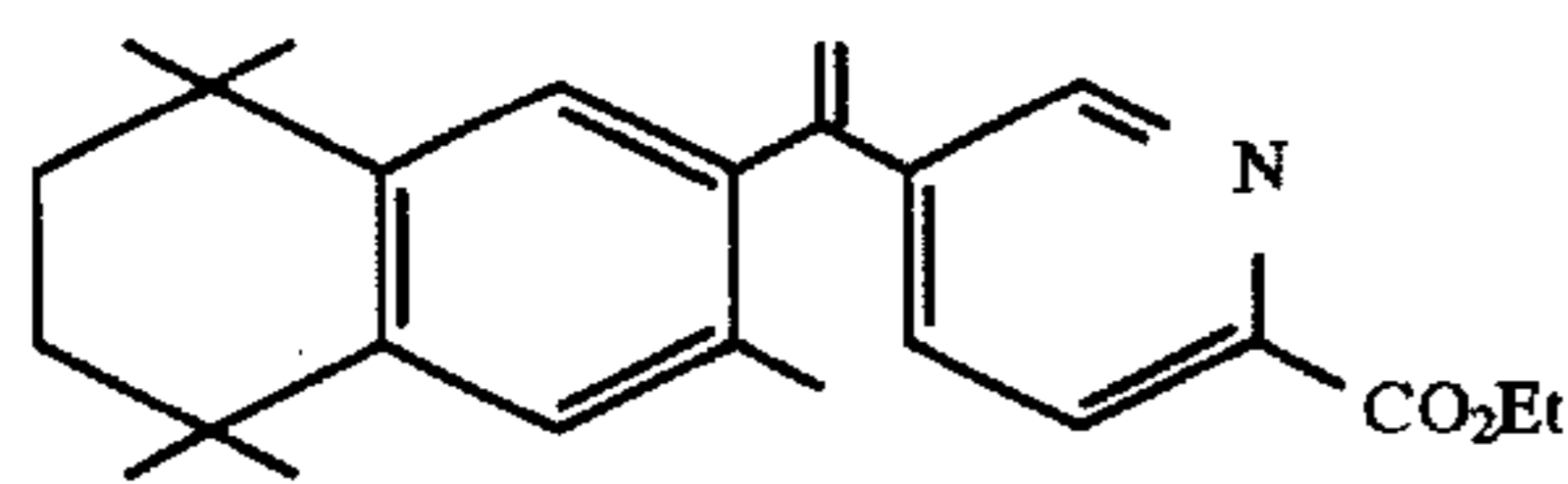
Ethyl-5-[1-(3,5,5,8,8-pentamethyl-5,6,7,8-tetrahydro-2-naphthyl)ethenyl]pyridine-2-carboxylate (3TTNEPE)
