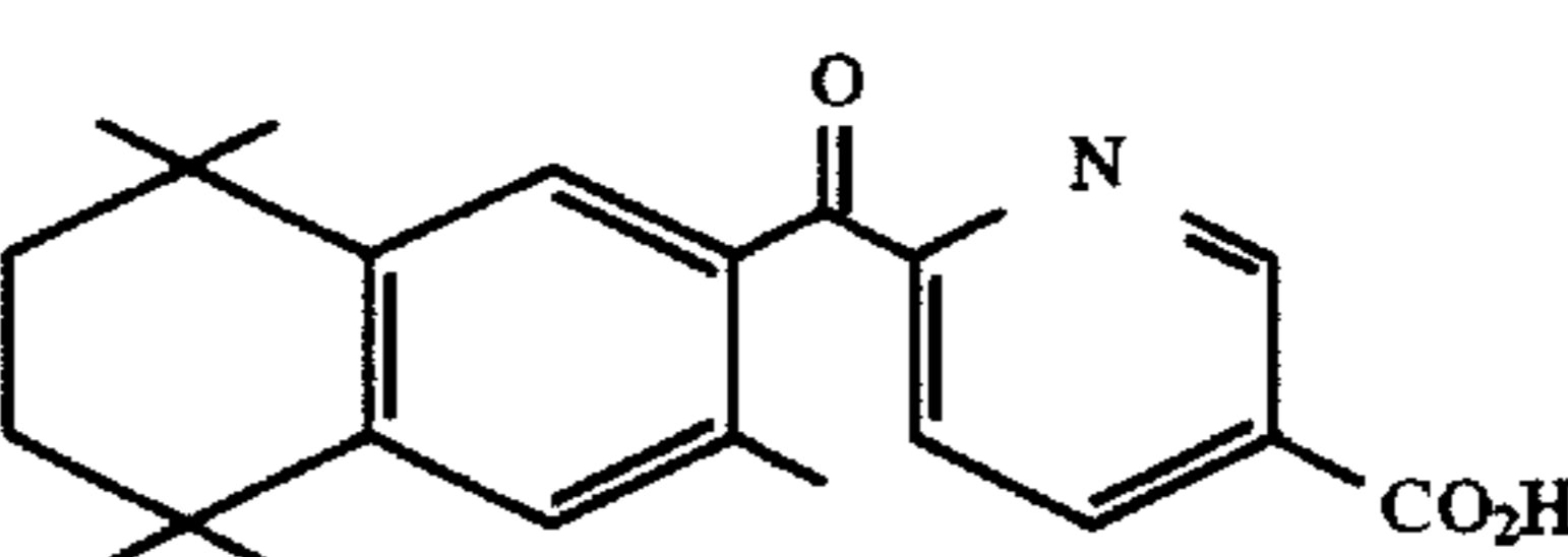
2-[1-(3,5,5,8,8-pentamethyl-5,6,7,8-tetrahydro-2-naphthyl)carbonyl]pyridine-5-carboxylic acid
