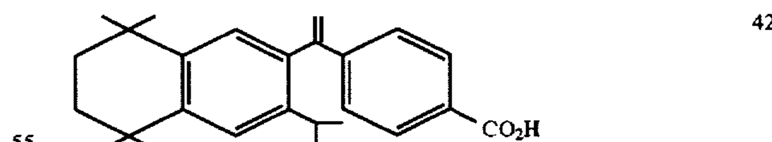
4-[1-(3-isopropyl-5,5,8,8-tetramethyl-5,6,7,8-tetrahydro-2-naphthyl)ethenyl]benzoic acid(3-IPr-TTNEB)
