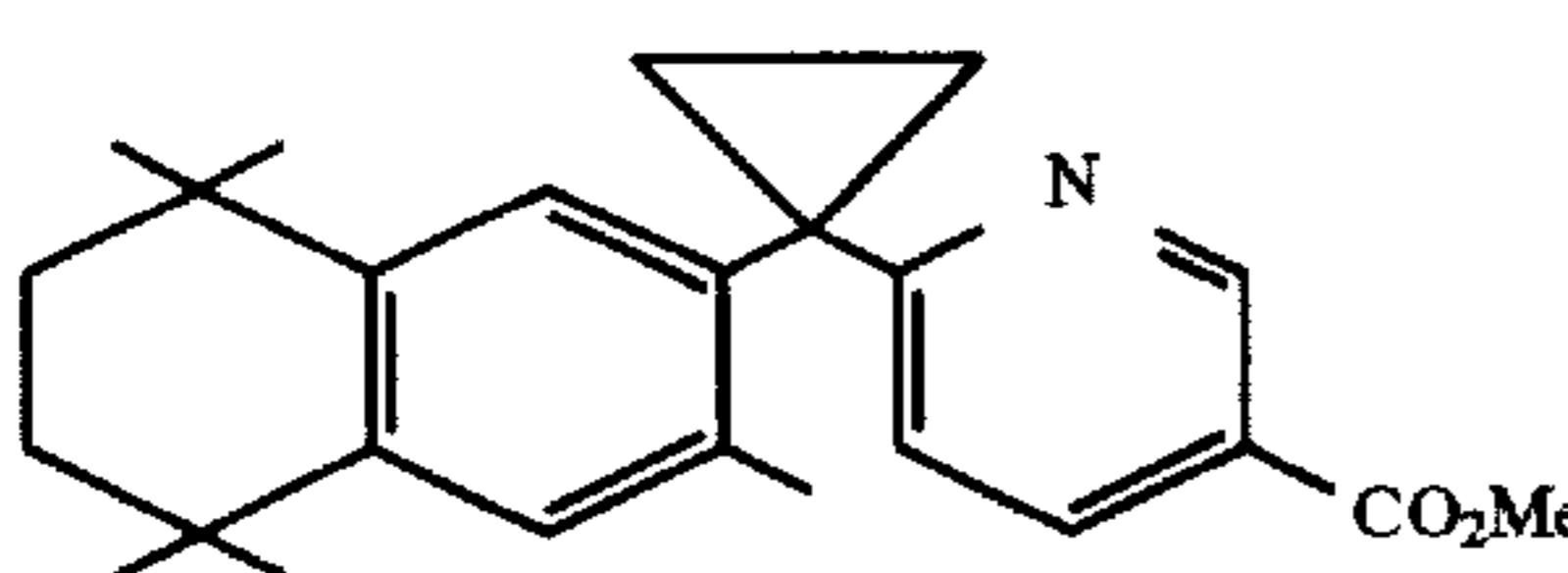
Methyl 2-[1-(3,5,5,8,8-pentamethyl-5,6,7,8-tetrahydro-2-naphthyl)cyclopropyl]pyridine-5-carboxylate
