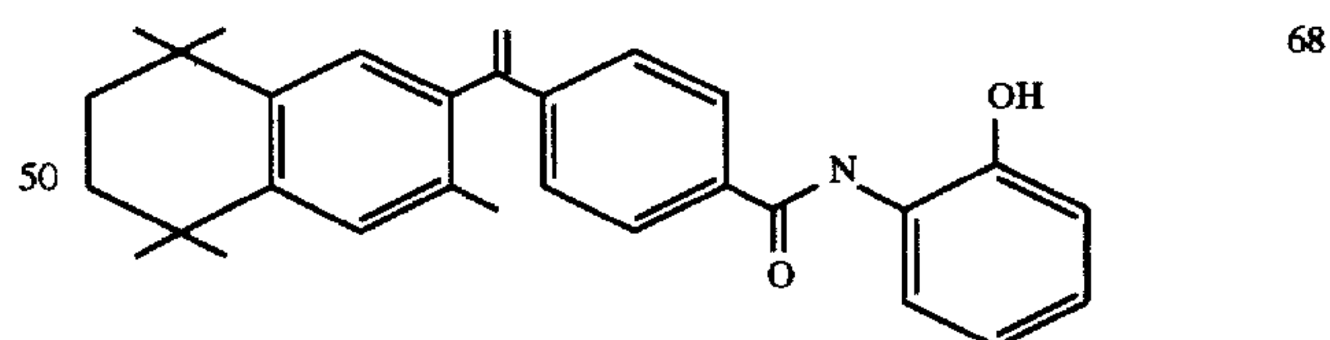
4-[1-(3,5,5,8,8-pentamethyl-5,6,7,8-tetrahydro-2-naphthyl)ethenyl]-N-(2-hydroxyphenyl)benzamide (3-Me-o-TTNEHBP)
