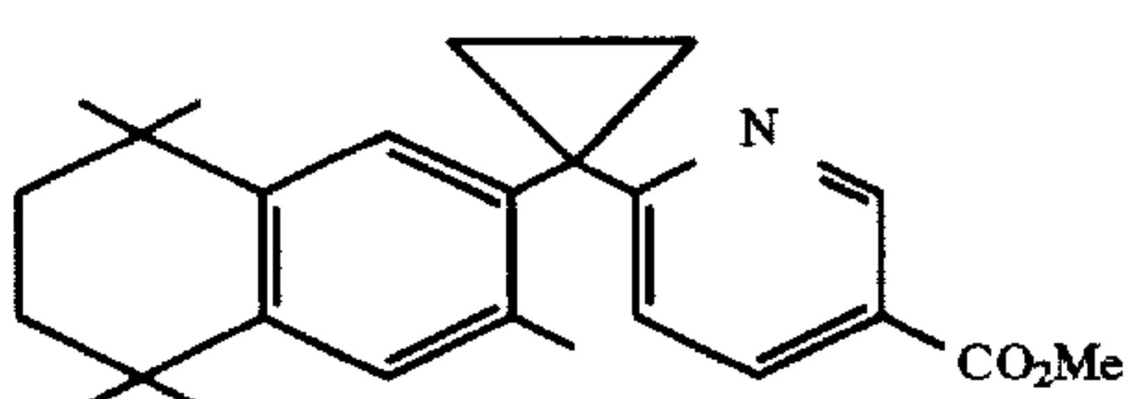
Methyl 2-[1-(3,5,5,8,8-pentamethyl-5,6,7,8-tetrahydro-2-naphthyl)cyclopropyl]pyridine-5-carboxylate
