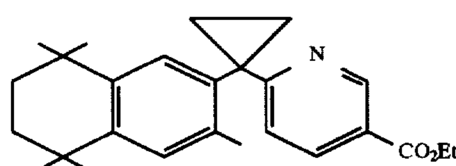
Ethyl-2-[1-(3,5,5,8,8-pentamethyl-5,6,7,8-tetrahydro-2-naphthyl)cyclopropyl]pyridine-5-carboxylate
