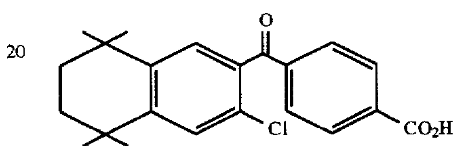
4-[(3-chloro-5,5,8,8-tetramethyl-5,6,7,8-tetrahydro-2-naphthyl)carbonyl]benzoic acid(3-chloro-TTNCB)
