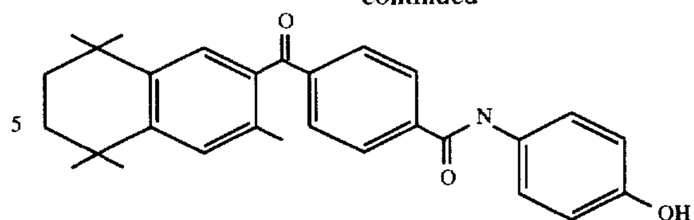
3-methyl-TTNCHBP
