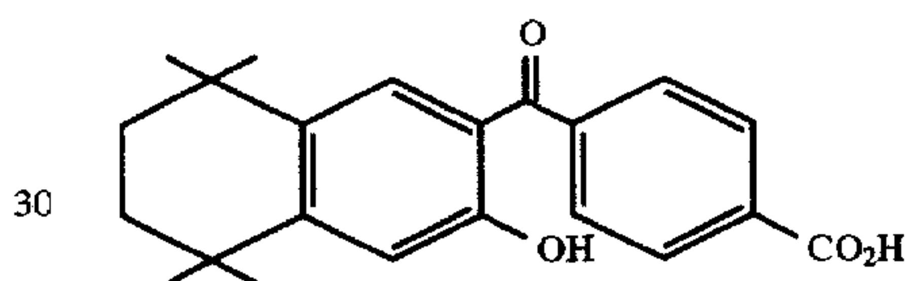
4-[(3-hydroxy-5,5,8,8-tetramethyl-5,6,7,8-tetrahydro-2-naphthyl)carbonyl]benzoic acid(3-hydroxy-TTNCB)
