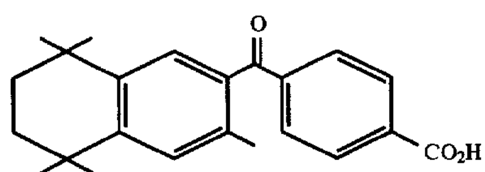
3-methyl-TTNCB
