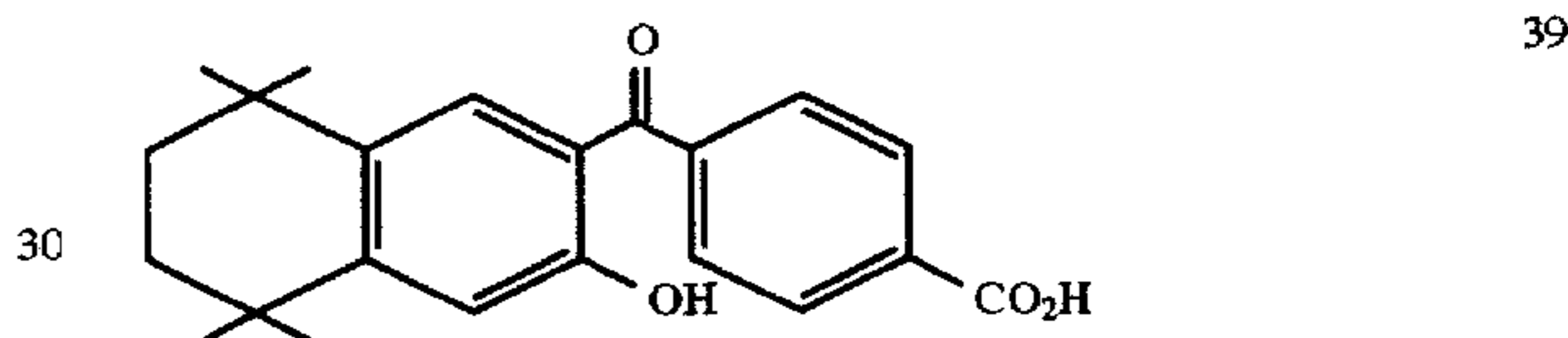
4-[1-(3-hydroxy-5,5,8,8-tetramethyl-5,6,7,8-tetrahydro-2-naphthyl)carbonyl]benzoic acid(3-hydroxy-TTNCB)
