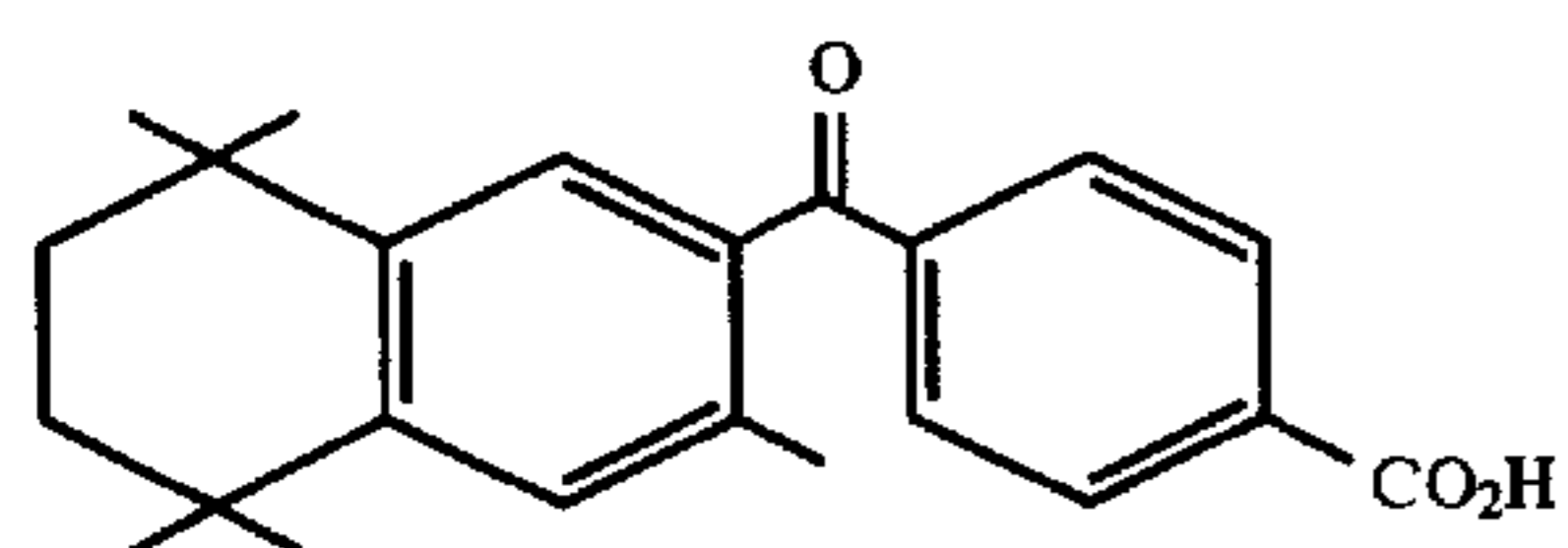
3-methyl-TTNCB
