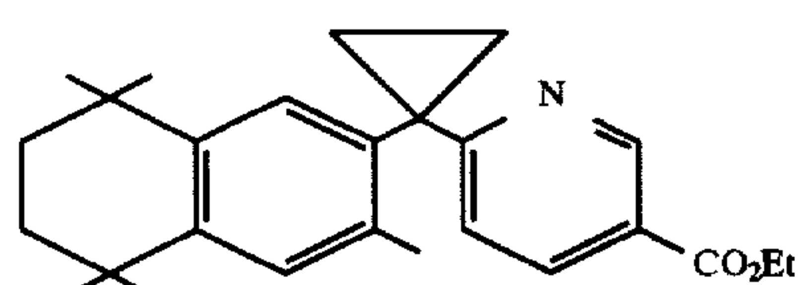
Ethyl-2-[1-(3,5,5,8,8-pentamethyl-5,6,7,8-tetrahydro-2-naphthyl)cyclopropyl]pyridine-5-carboxylate
