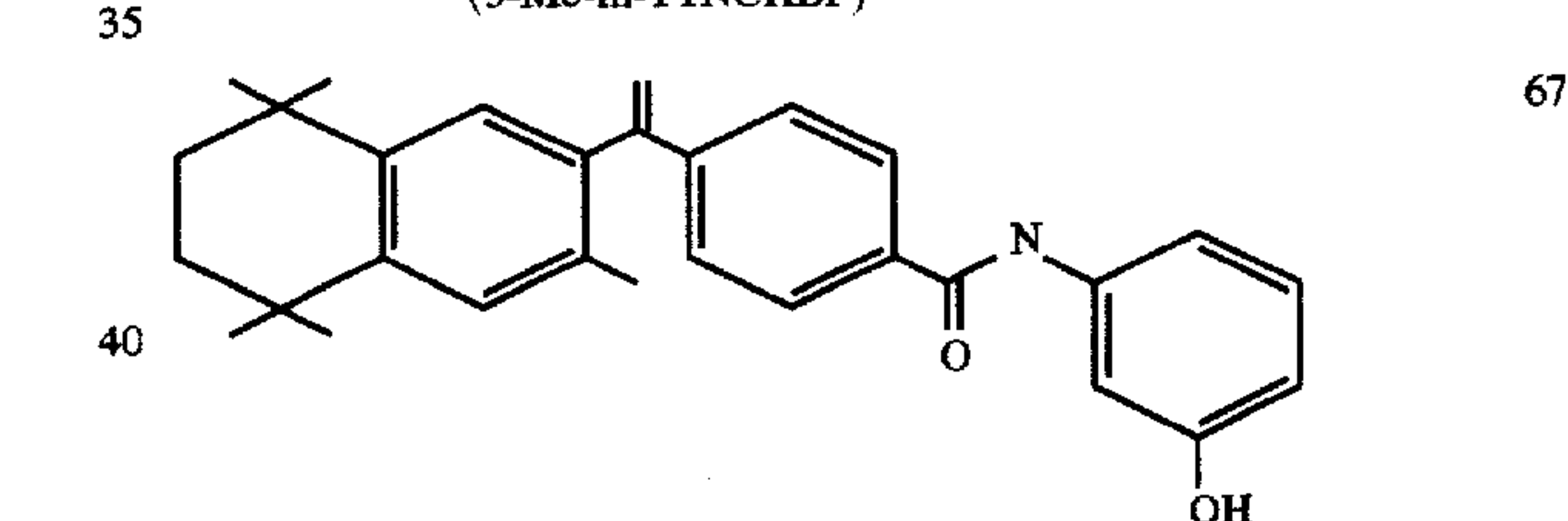
4-[1-(3,5,5,8,8-pentamethyl-5,6,7,8-tetrahydro-2-naphthyl)ethenyl]-N-(3-hydroxyphenyl)benzamide (3-Me-m-TTNEHBP)
