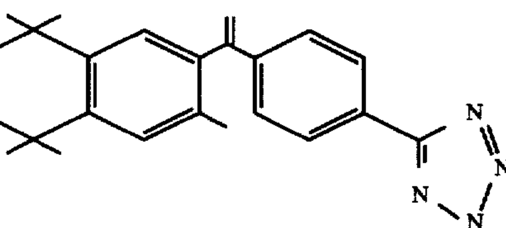
4-[1-(3,5,5,8,8-pentamethyl-5,6,7,8-tetrahydro-2-naphthyl)ethenyl]benzenetetrazole (3-methyl-TTNEBT)
