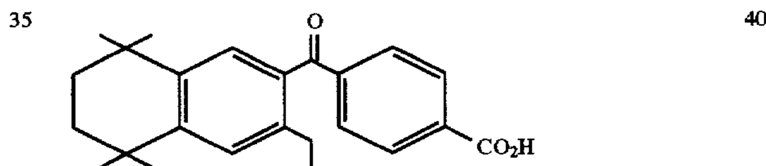
4-[1-(3-ethyl-5,5,8,8-tetramethyl-5,6,7,8-tetrahydro-2-naphthyl)carbonyl]benzoic acid(3-Et-TTNCB)
