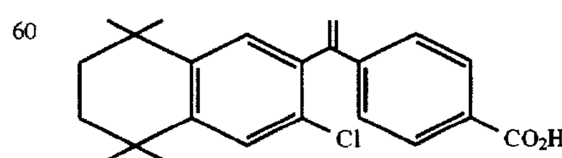
4-[1-(3-chloro-5,5,8,8-tetramethyl-5,6,7,8-tetrahydro-2-naphthyl)ethenyl]benzoic acid(3-chloro-TTNEB)
