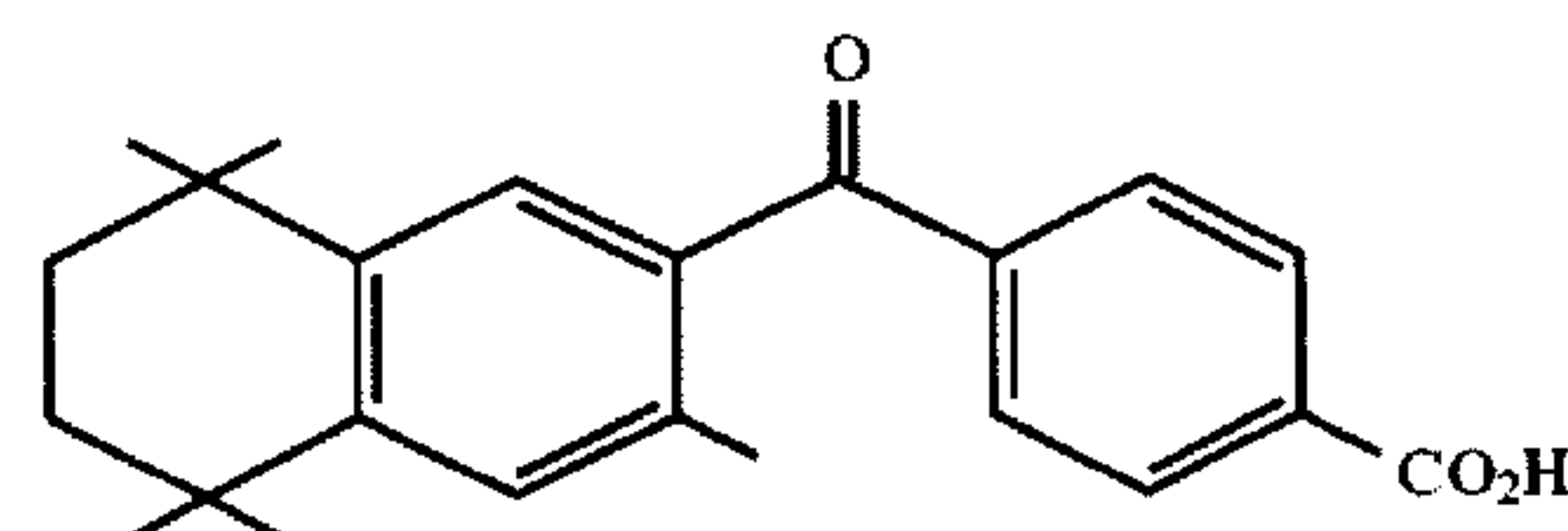
3-methyl-TTNCB
