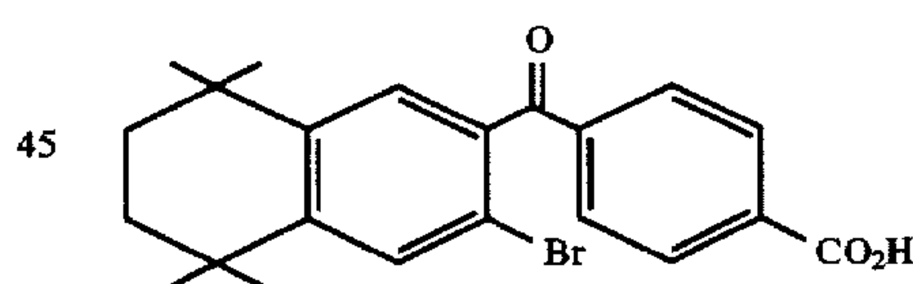
4-[(3-bromo-5,5,8,8-tetramethyl-5,6,7,8-tetrahydro-2-naphthyl)carbonyl]benzoic acid(3-bromo-TTNCB)
