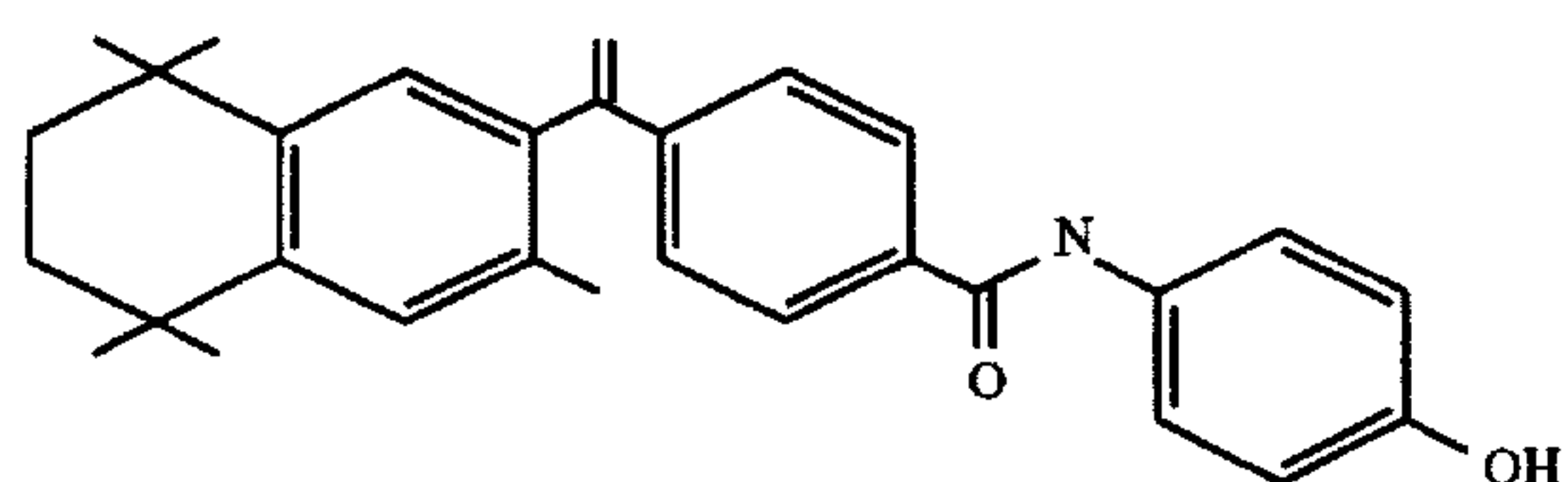
Ethyl-2-[1-(3,5,5,8,8-pentamethyl-5,6,7,8-tetrahydro-2-naphthyl)cyclopropyl]pyridine-5-carboxylate
