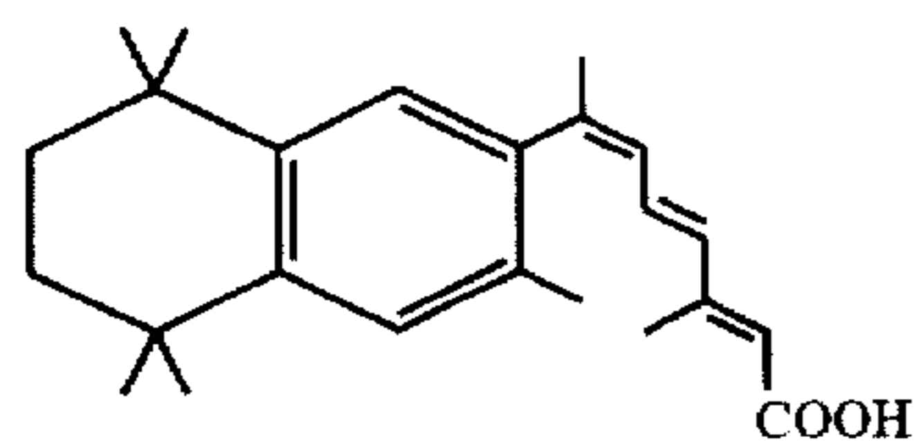
(2E,4E,6Z)-7-(3,5,5,8,8-pentamethyl-5,6,7,8-tetrahydro-2-naphthyl)-3-methyl-octa-2,4,6-trienoic acid
