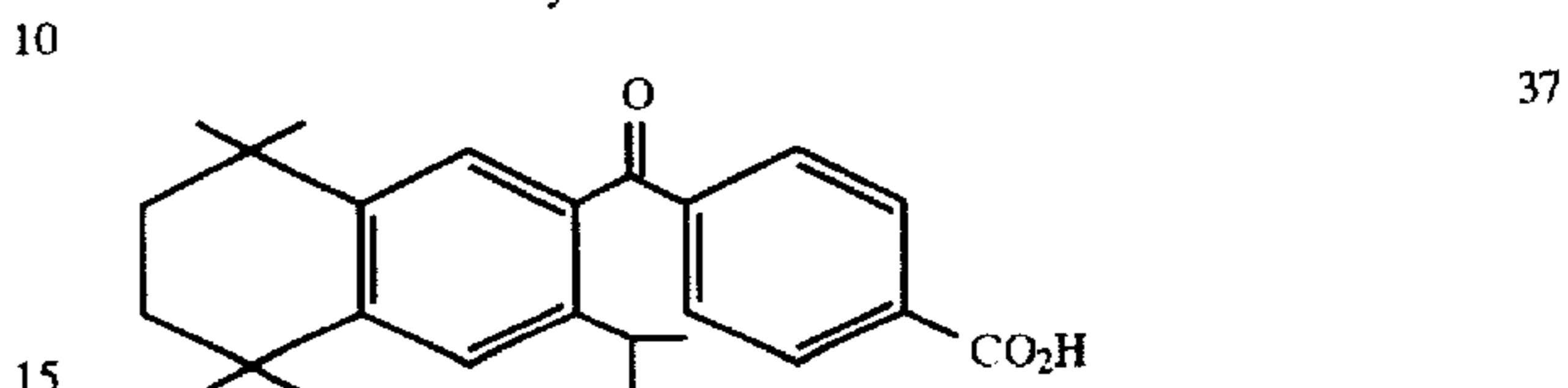
4-[1-(3-isopropyl-5,5,8,8-tetramethyl-5,6,7,8-tetrahydro-2-naphthyl)carbonyl]benzoic acid(3-IPr-TTNCB)
