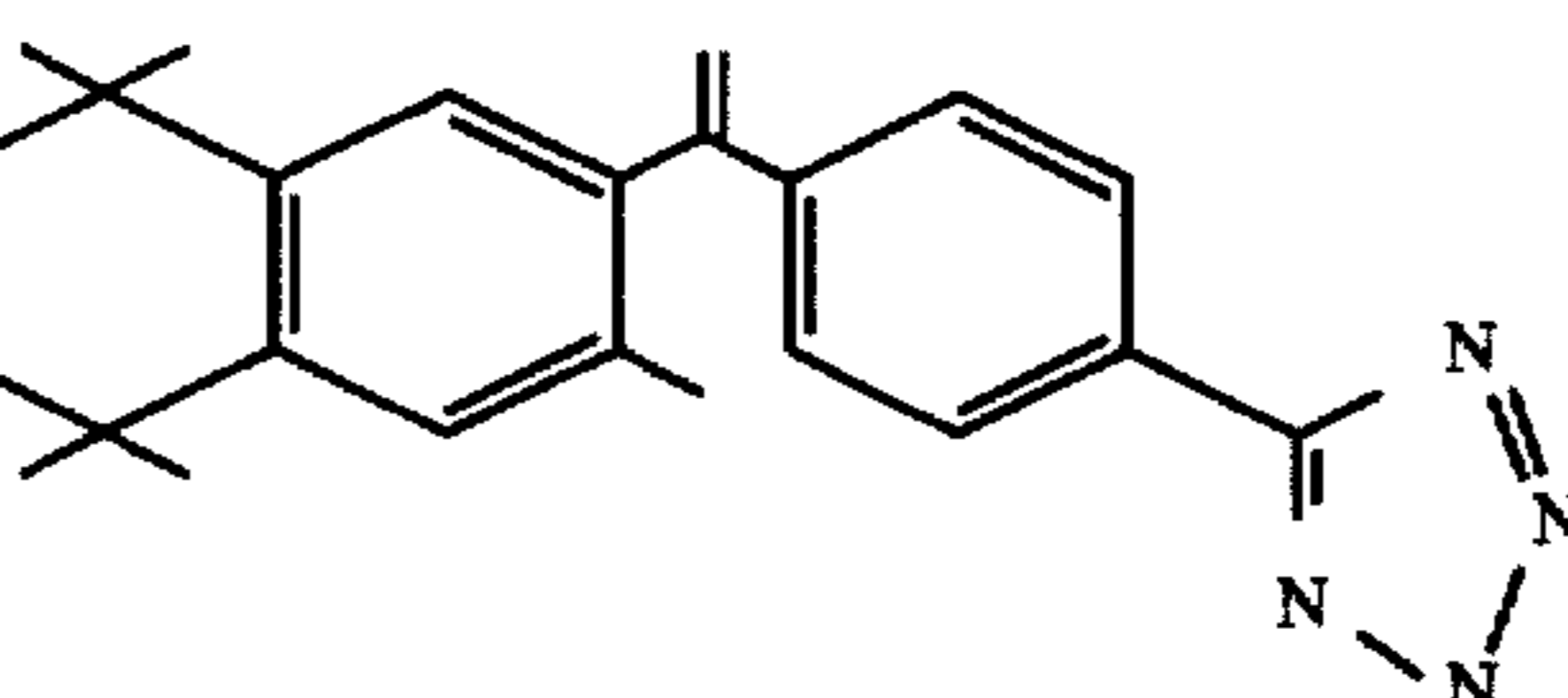
4-[1-(3,5,5,8,8-pentamethyl-5,6,7,8-tetrahydro-2-naphthyl)ethenyl]benzenetetrazole (3-methyl-TTNEBT)
