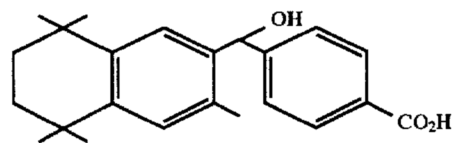
3-methyl-TTNHMB
