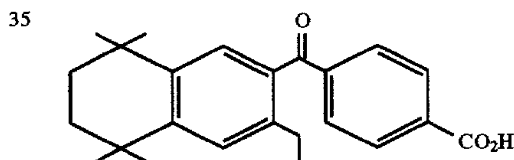
4-[(3-ethyl-5,5,8,8-tetramethyl-5,6,7,8-tetrahydro-2-naphthyl)carbonyl]benzoic acid(3-Et-TTNCB)
