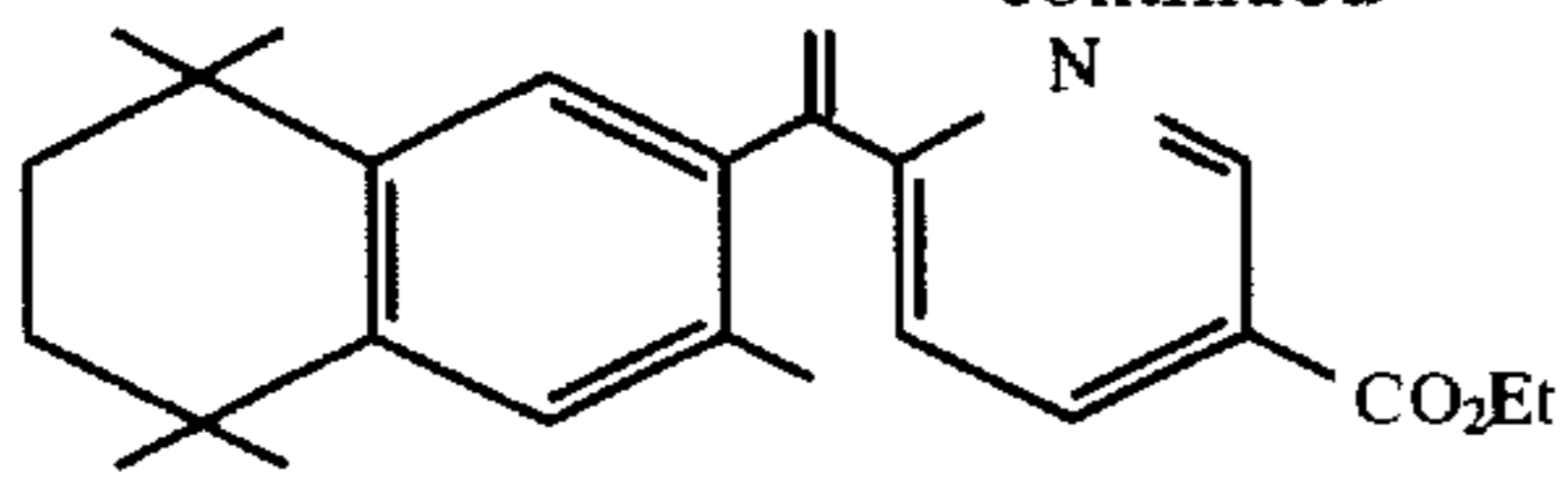
Ethyl-2-[1-(3,5,5,8,8-pentamethyl-5,6,7,8-tetrahydro-2-naphthyl)ethenyl]pyridine-5-carboxylate
