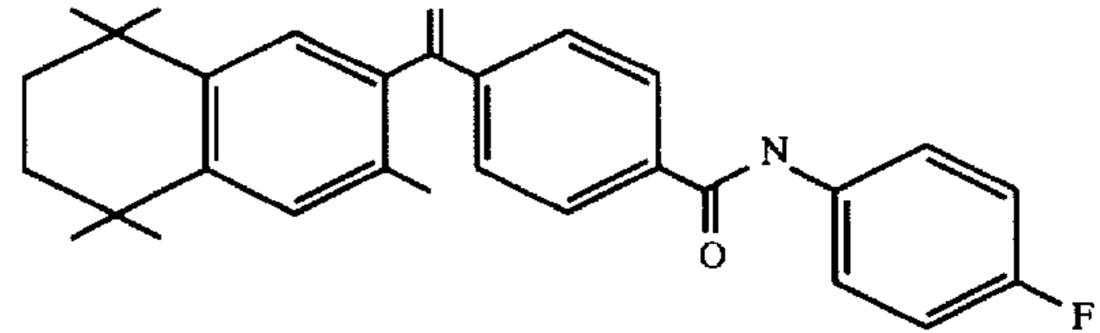
4-[1-(3,5,5,8,8-pentamethyl-5,6,7,8-tetrahydro-2-naphthyl)ethenyl]-N-(4-carboxyphenyl)benzamide (3-Me-TTNECBP)
