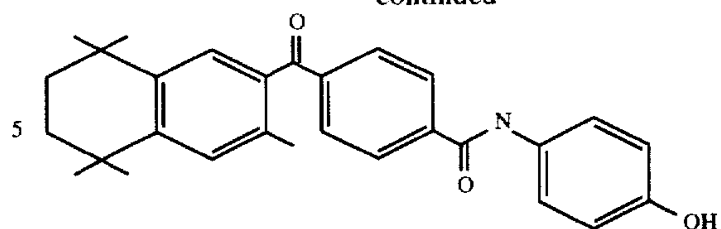
3-methyl-TTNCHBP
