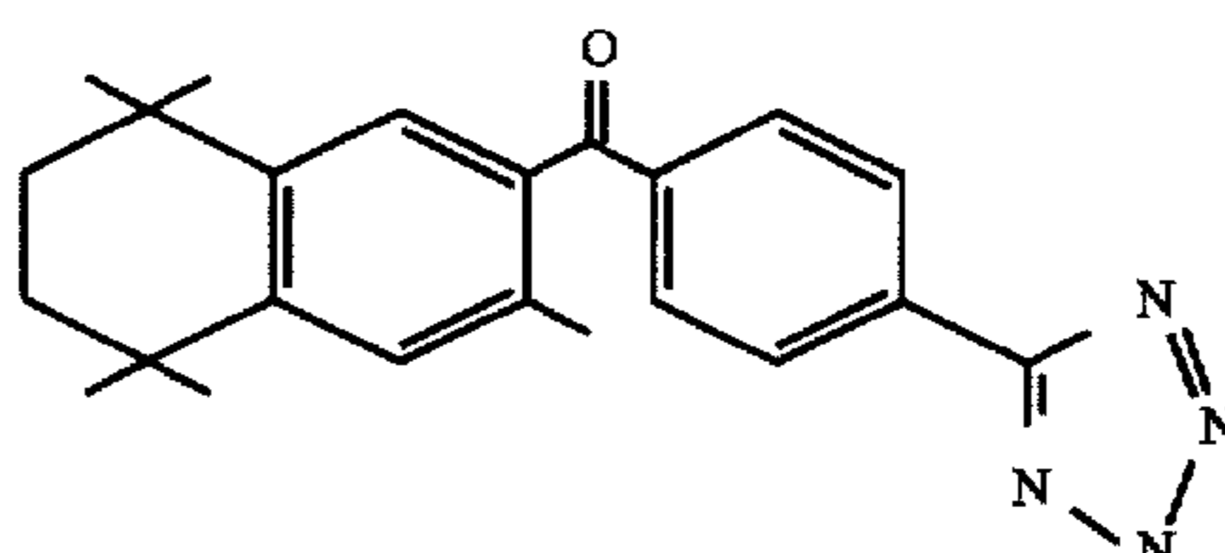
4-[1-(3,5,5,8,8-pentamethyl-5,6,7,8-tetrahydro-2-naphthyl)carbonyl]benzenetetrazole (3-methyl-TTNCBT)
