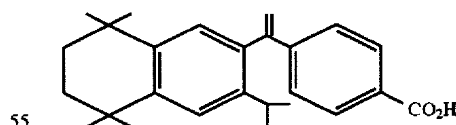
4-[1-(3-isopropyl-5,5,8,8-tetramethyl-5,6,7,8-tetrahydro-2-naphthyl)ethenyl]benzoic acid(3-IPr-TTNEB)
