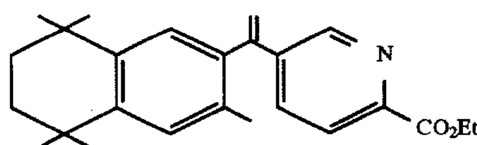
Ethyl-5-[1-(3,5,5,8,8-pentamethyl-5,6,7,8-tetrahydro-2-naphthyl)ethenyl]pyridine-2-carboxylate (3TTNEPE)
