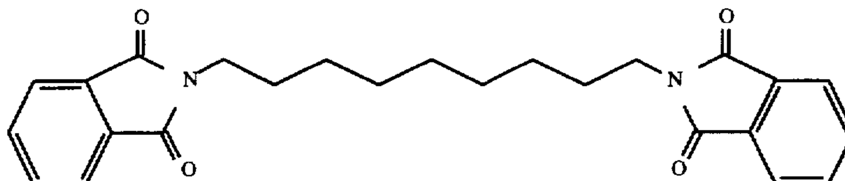
1118 (N-(9-Phthalimidononyl)-phthalimide
