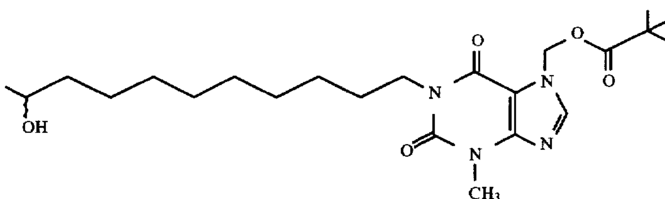
1444 1-(10-Hydroxyundecyl)-3-methyl-7-methylpivaloyloxanthine
