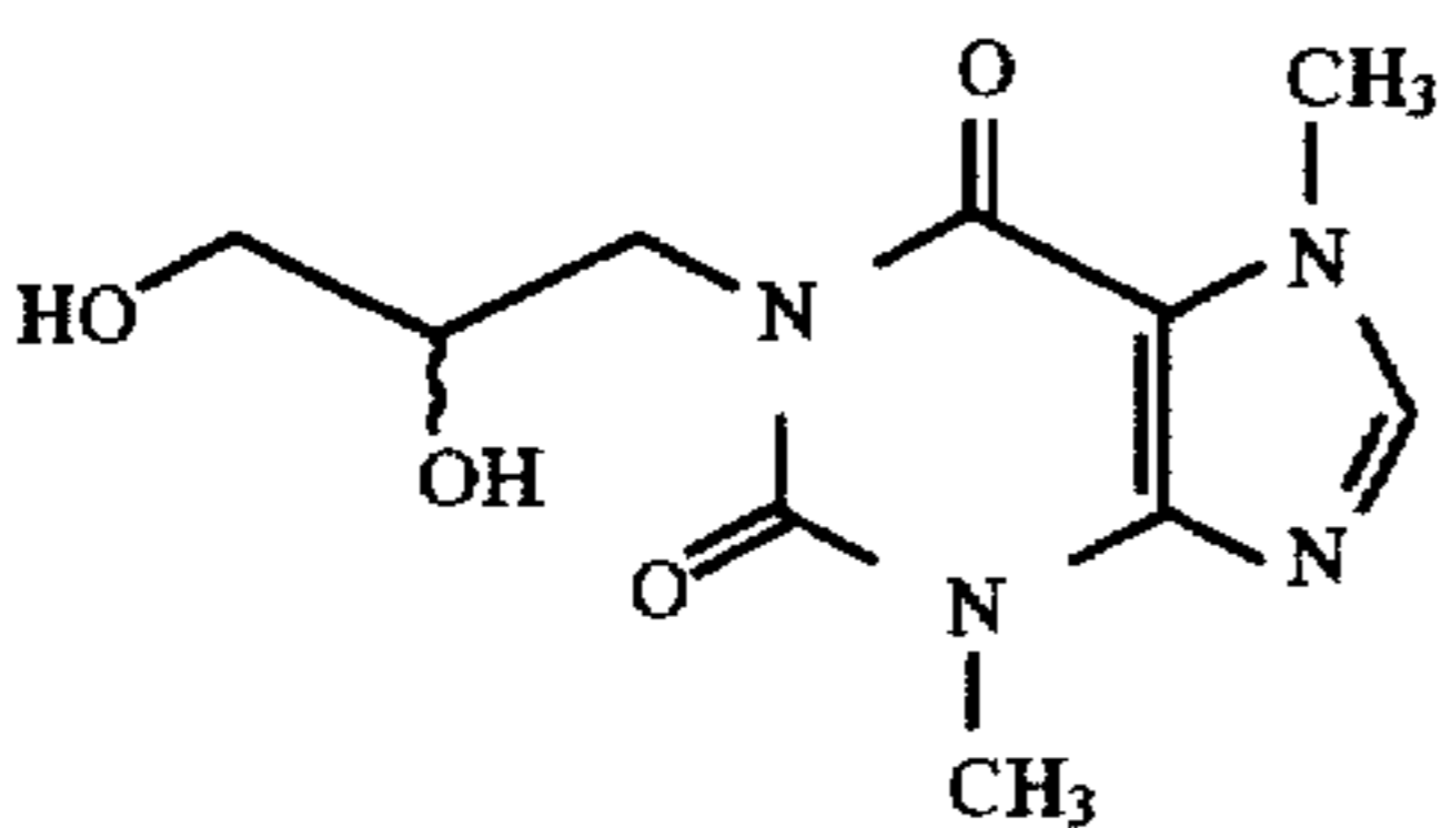
1540 1-(2,3-Dihydroxypropyl)-3,7-dimethylxanthine
