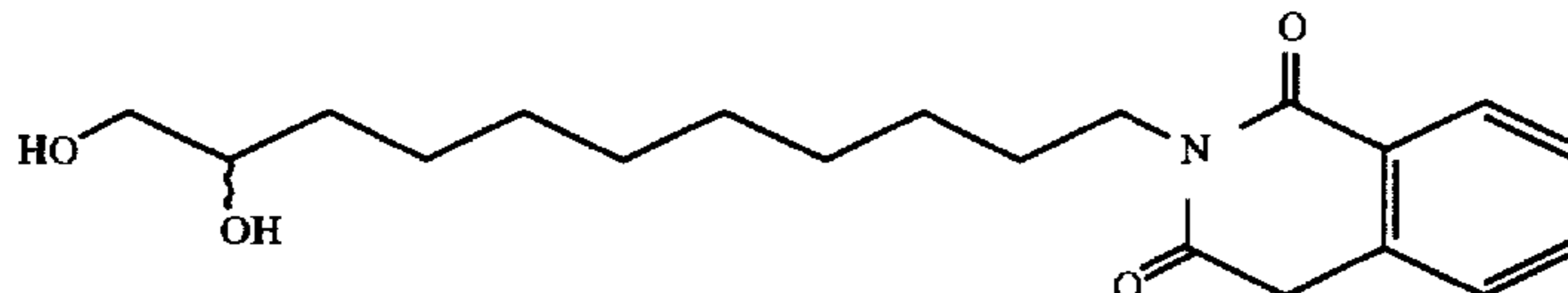
1113 N-(10,11-Dihydroxyundecyl)-homophthalimide
