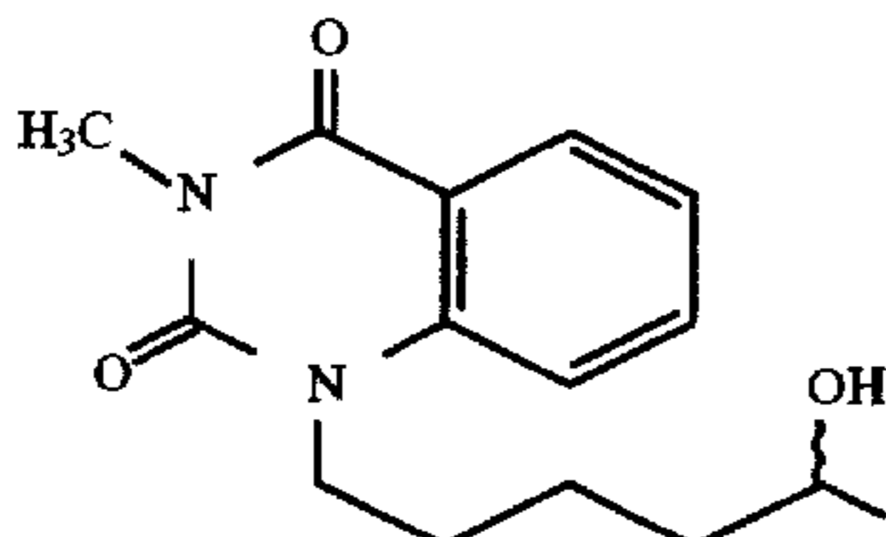
1207 1-(5-Hydroxyhexyl)-3-methylbenzoyl-eneurea
