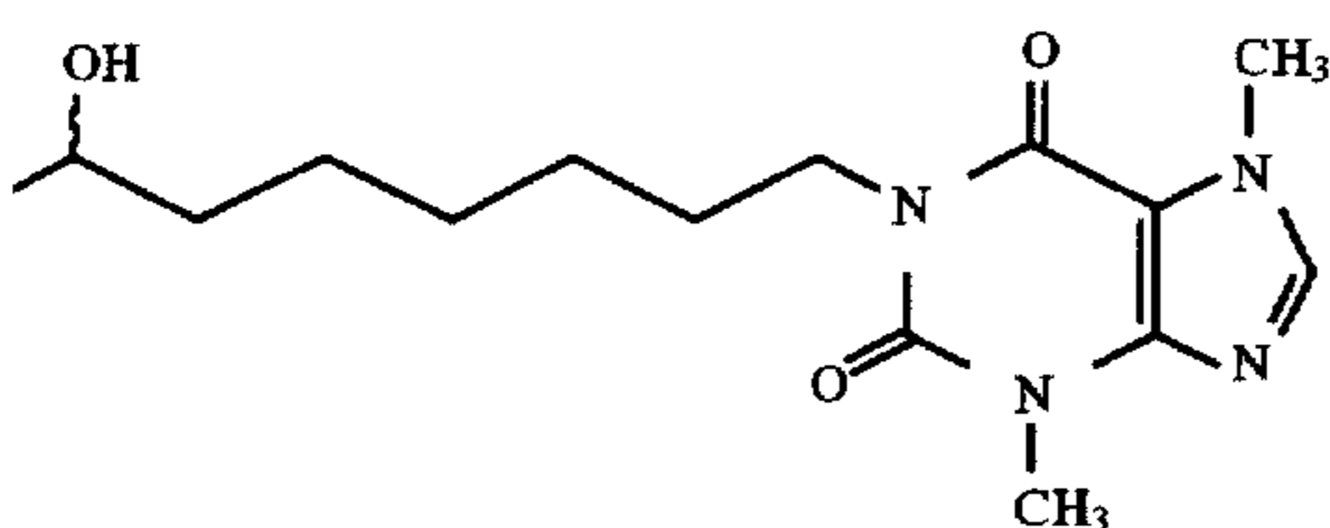
1536 1-(7-Hydroxyoctyl)-3,7-dimethylxanthine
