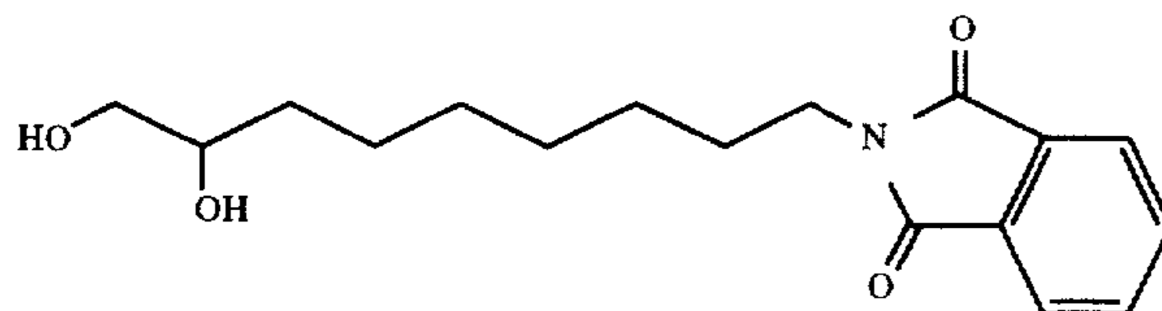
1106 N-(8,9-Dihydroxynonyl)-phthalimide
