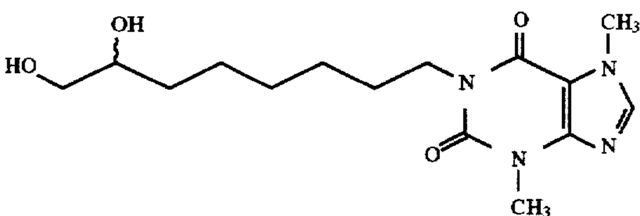
1538 1-(7,8-Dihydroxyoctyl)-3,7-dimethylxanthine
