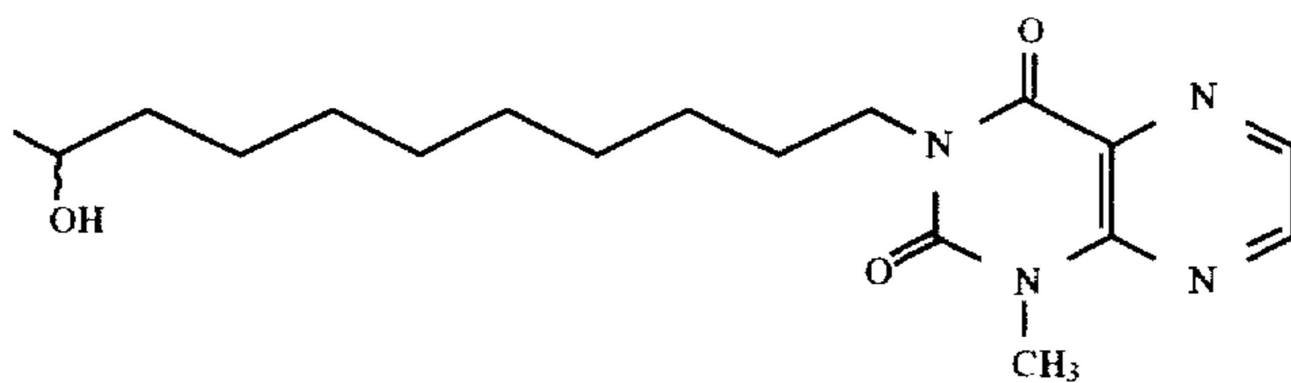
1429 3-(10-Hydroxyundecyl)-1-methyl-2,4-dioxotetrahydropteridine
