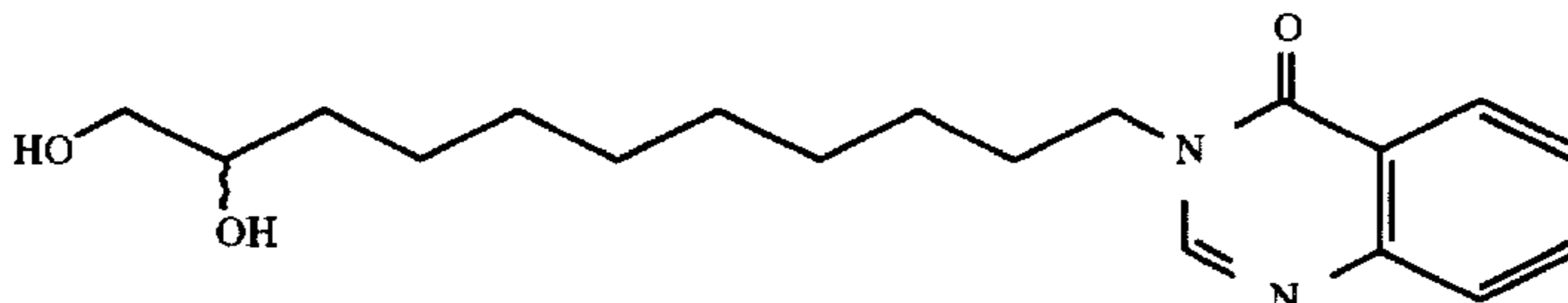
1215 3-(11,10-Dihydroxyundecyl)-quinazoline-4-(3H)-one
