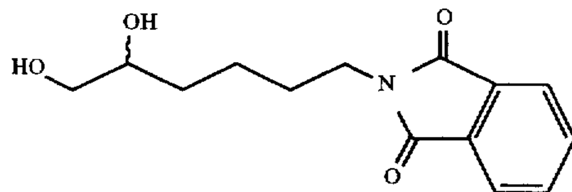
1104 N-(5,6-Dihydroxyhexyl)-phthalimide
