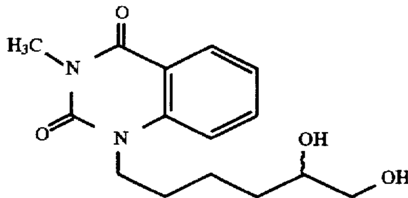
1204 1-(5,6-Dihydroxyhexyl)-3-methylbenzoyl-eneurea
