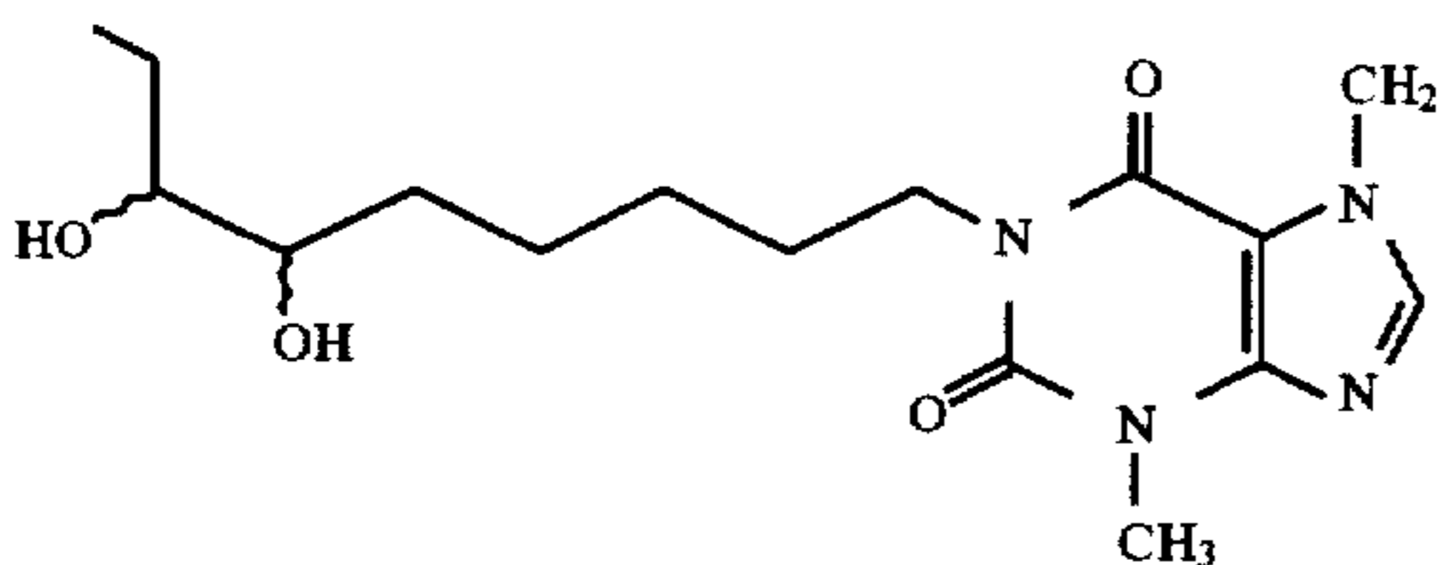
1528 1-(6,7-Dihydroxynonyl)-3,7-dimethylxanthine
