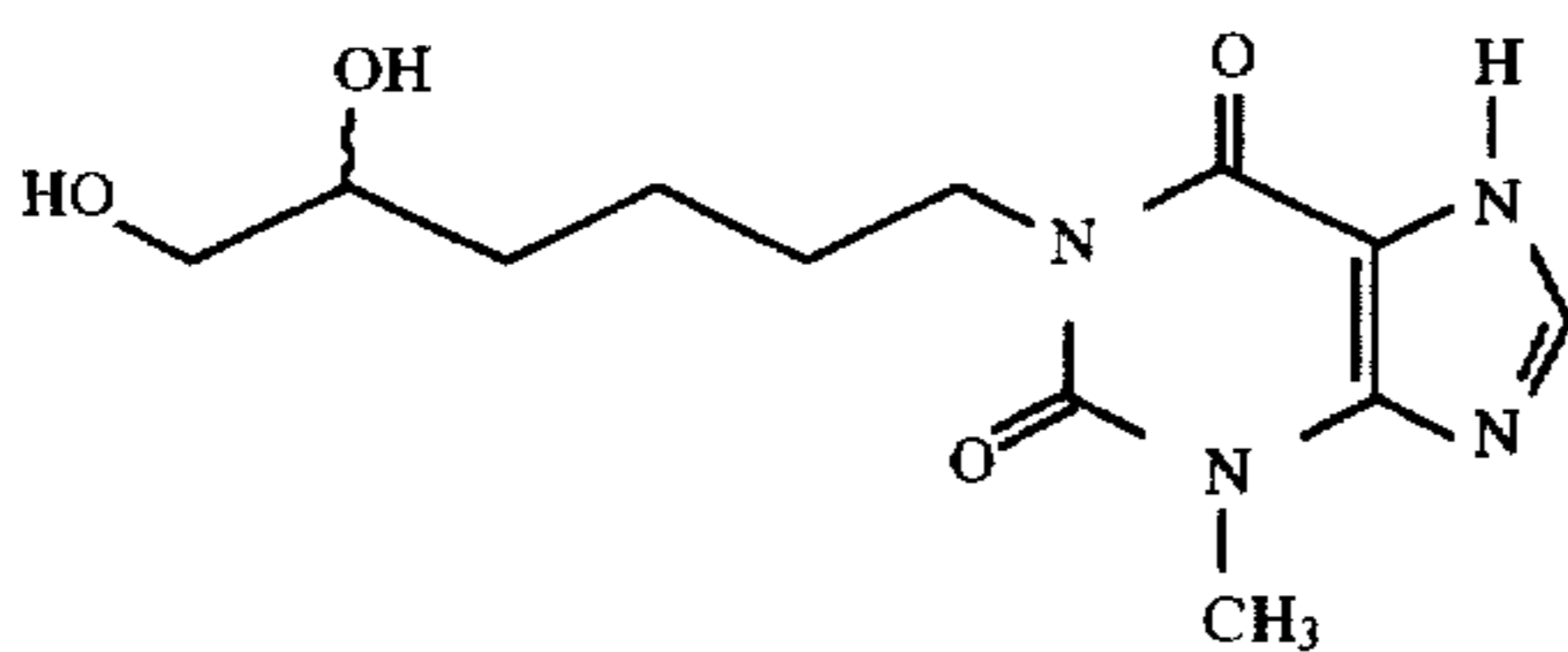
1440 1-(5,6-Dihydroxyhexyl)-3-methylxanthine
