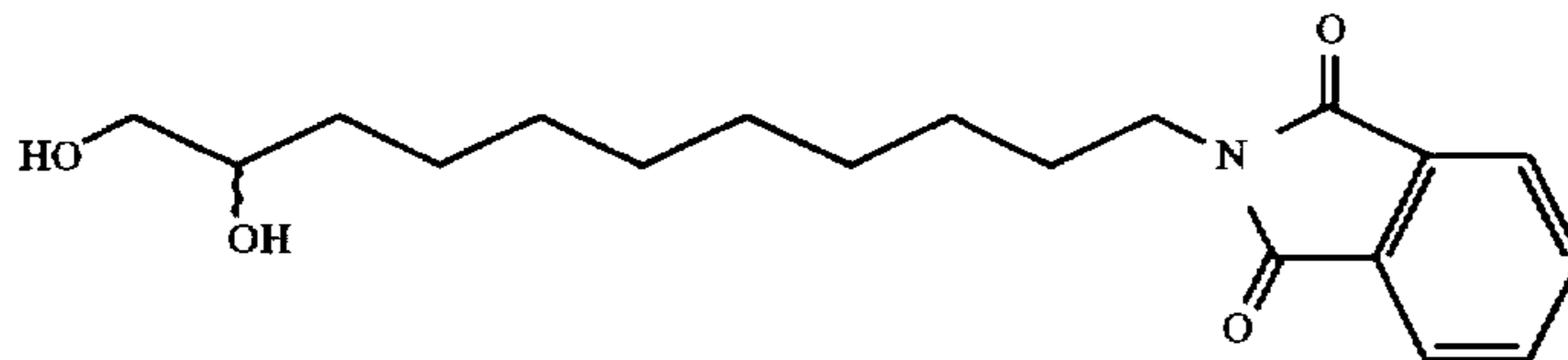
1108 N-(10,11-Dihydroxyundecyl)-phthalimide
