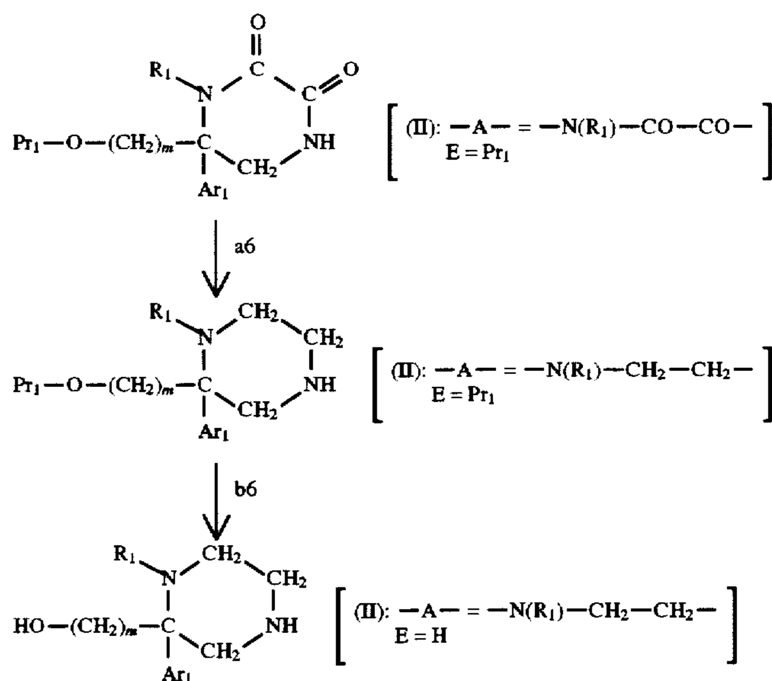
SCHEME 6
