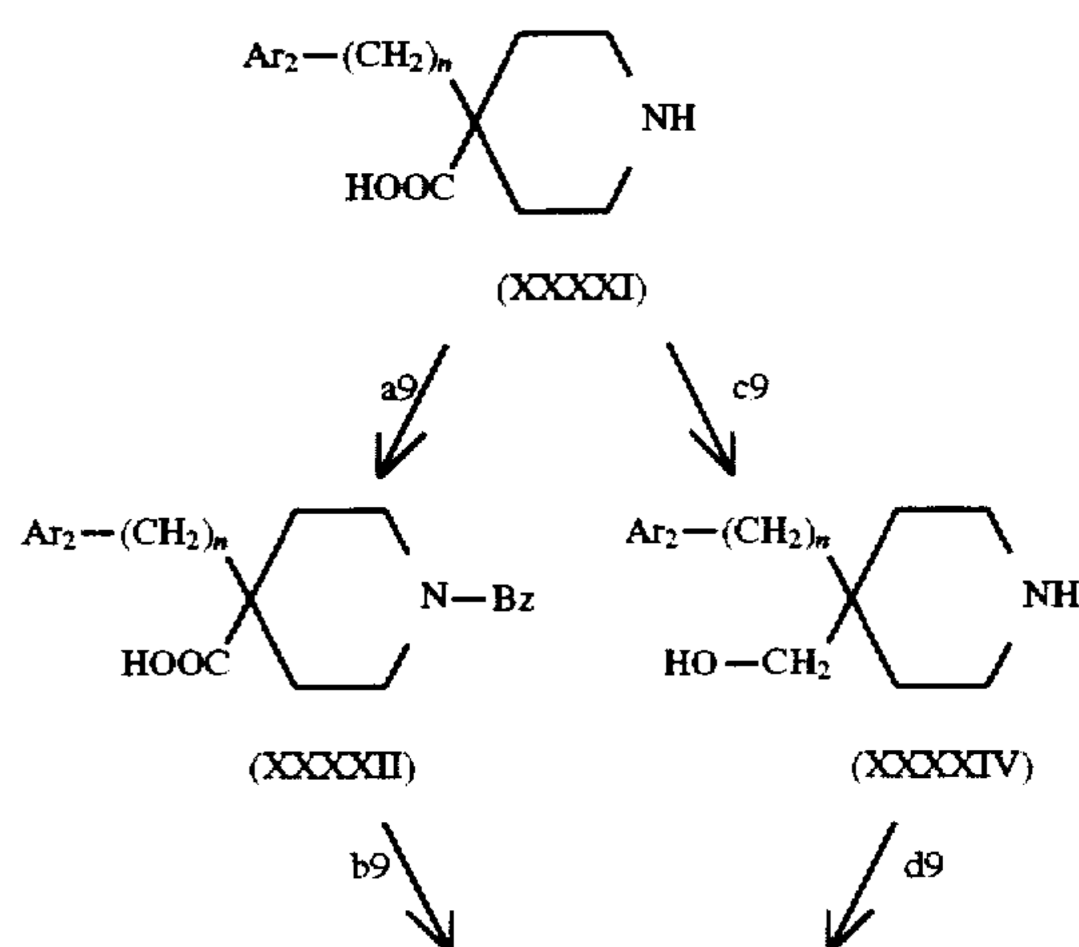
SCHEME 9
