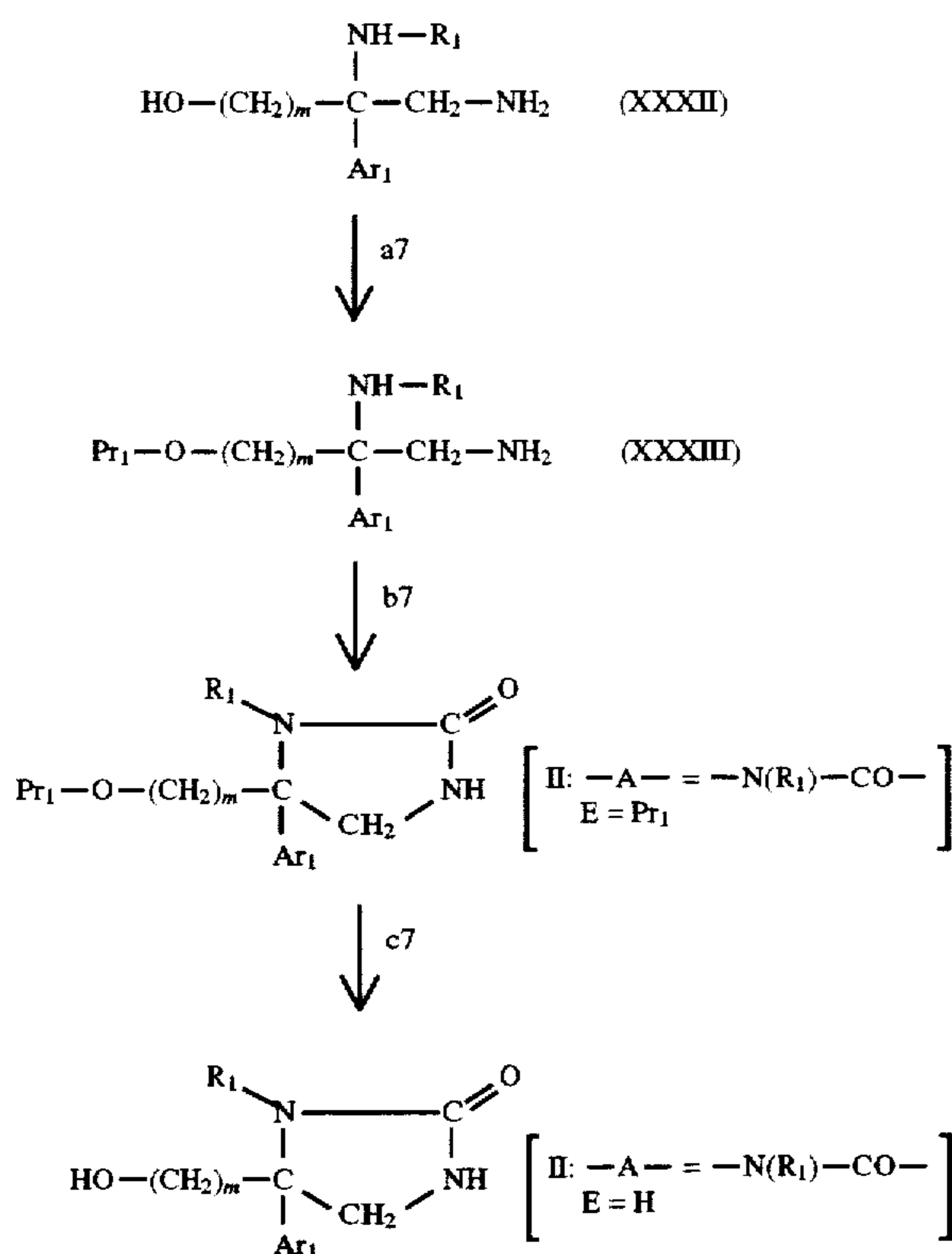
SCHEME 7
