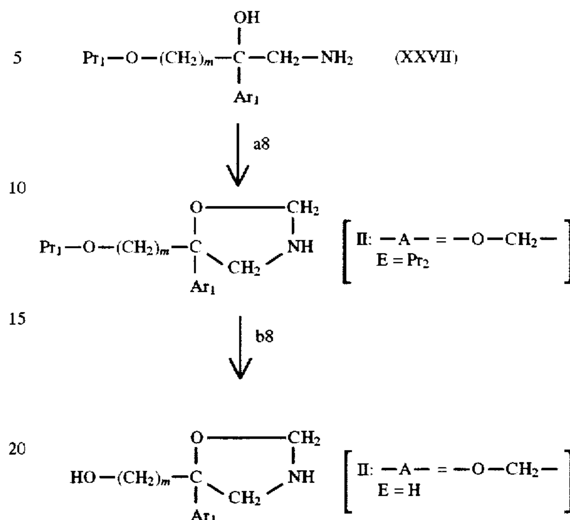
SCHEME 8
