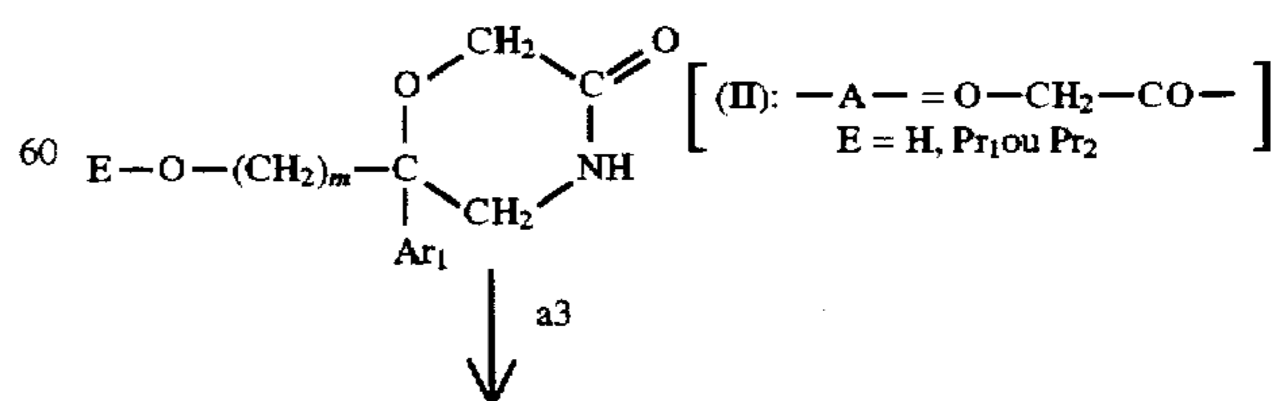
SCHEME 3
