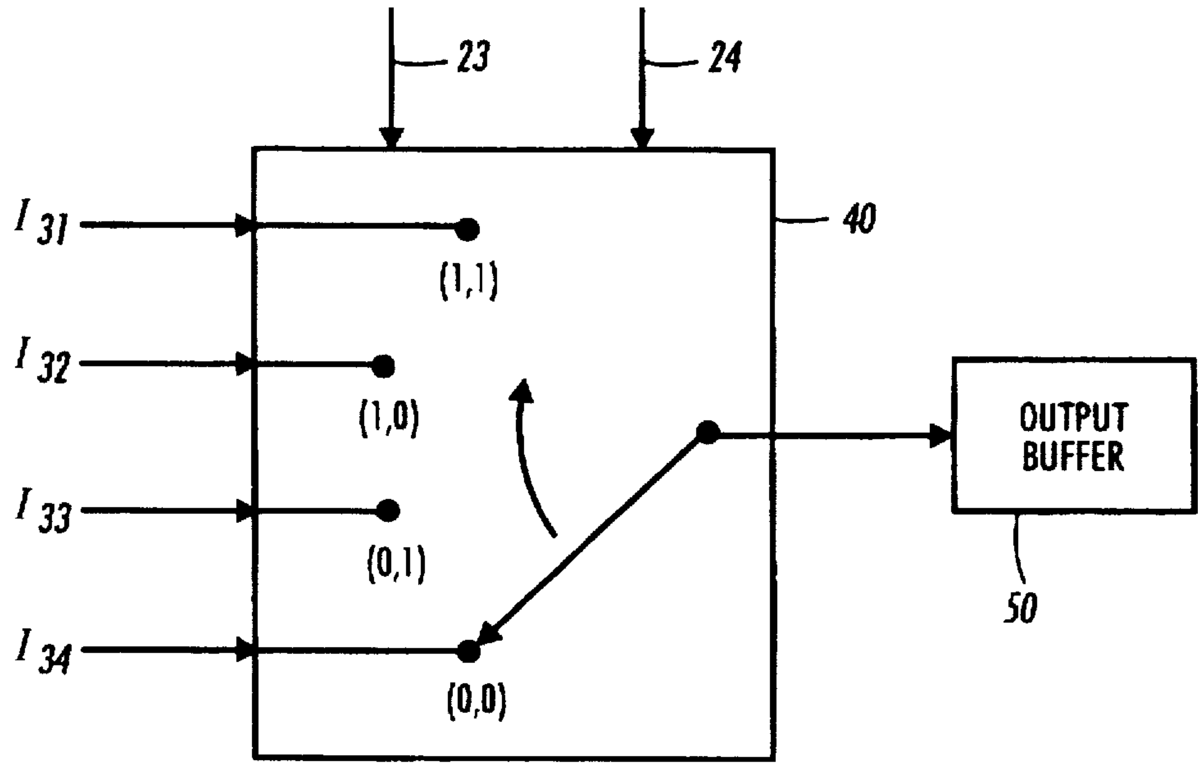
FIG. 17 (Prior Art)
