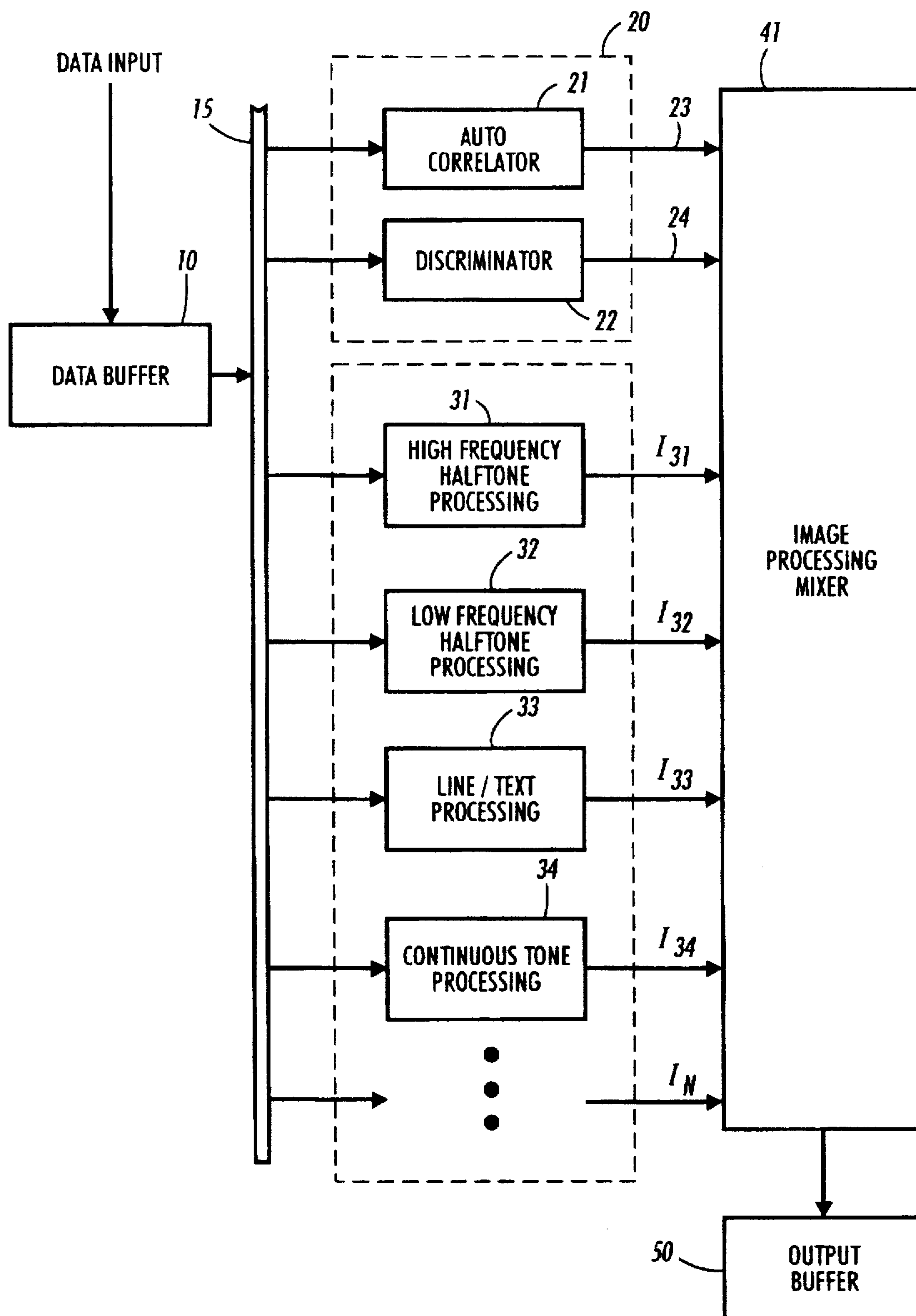
FIG. 15 (Prior Art)
