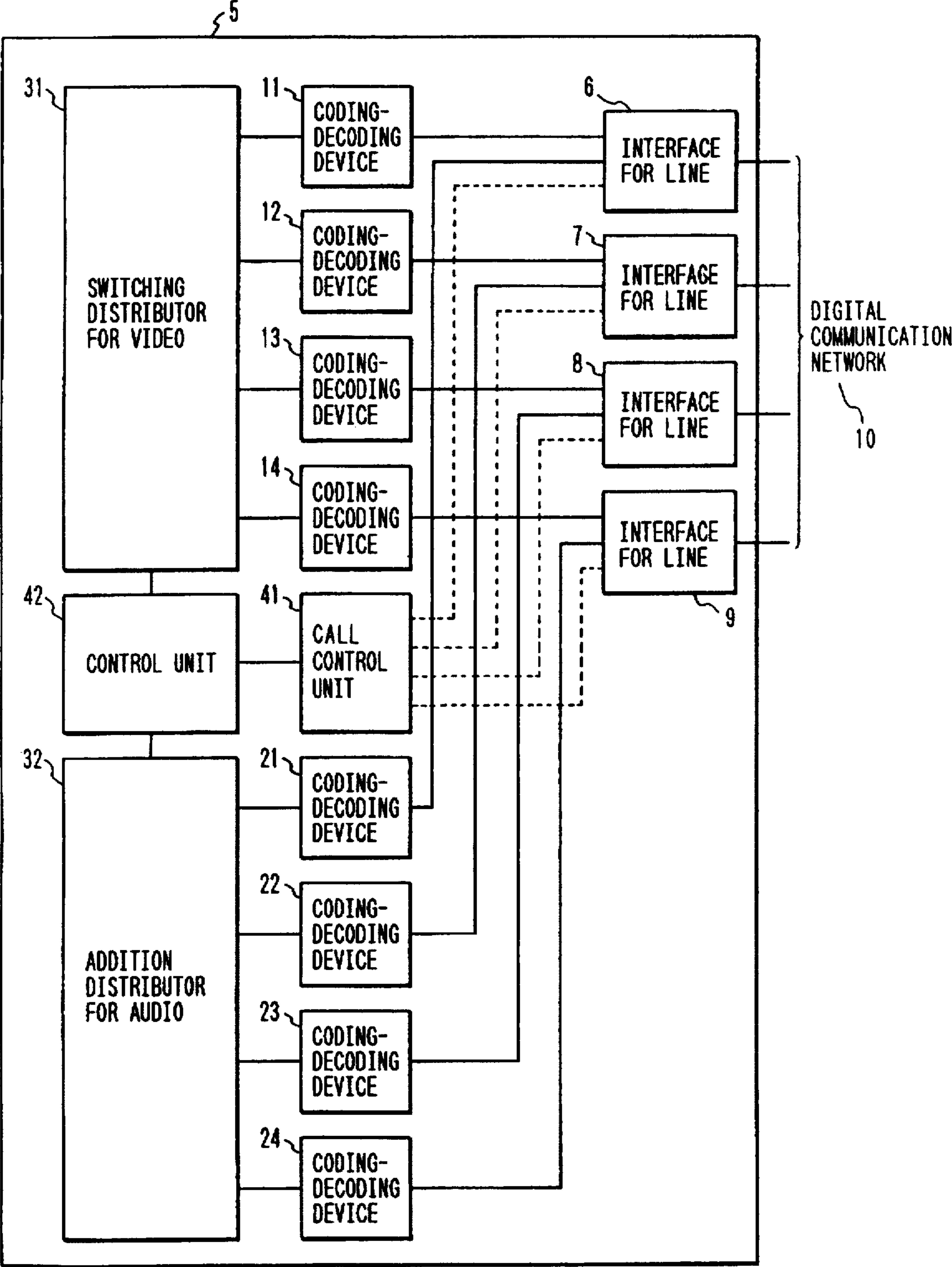
FIG. 2 PRIOR ART
