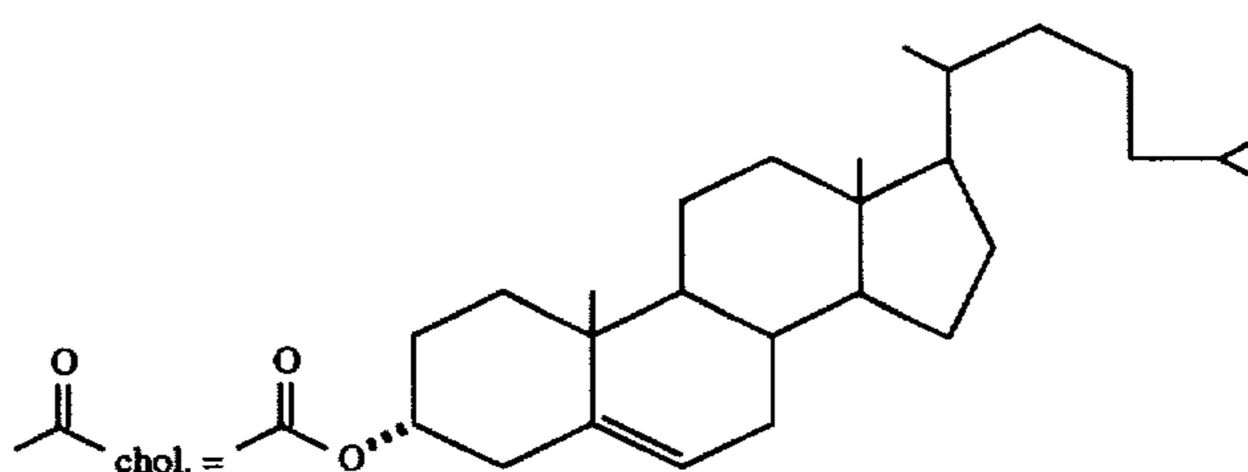
SCHEME 2
