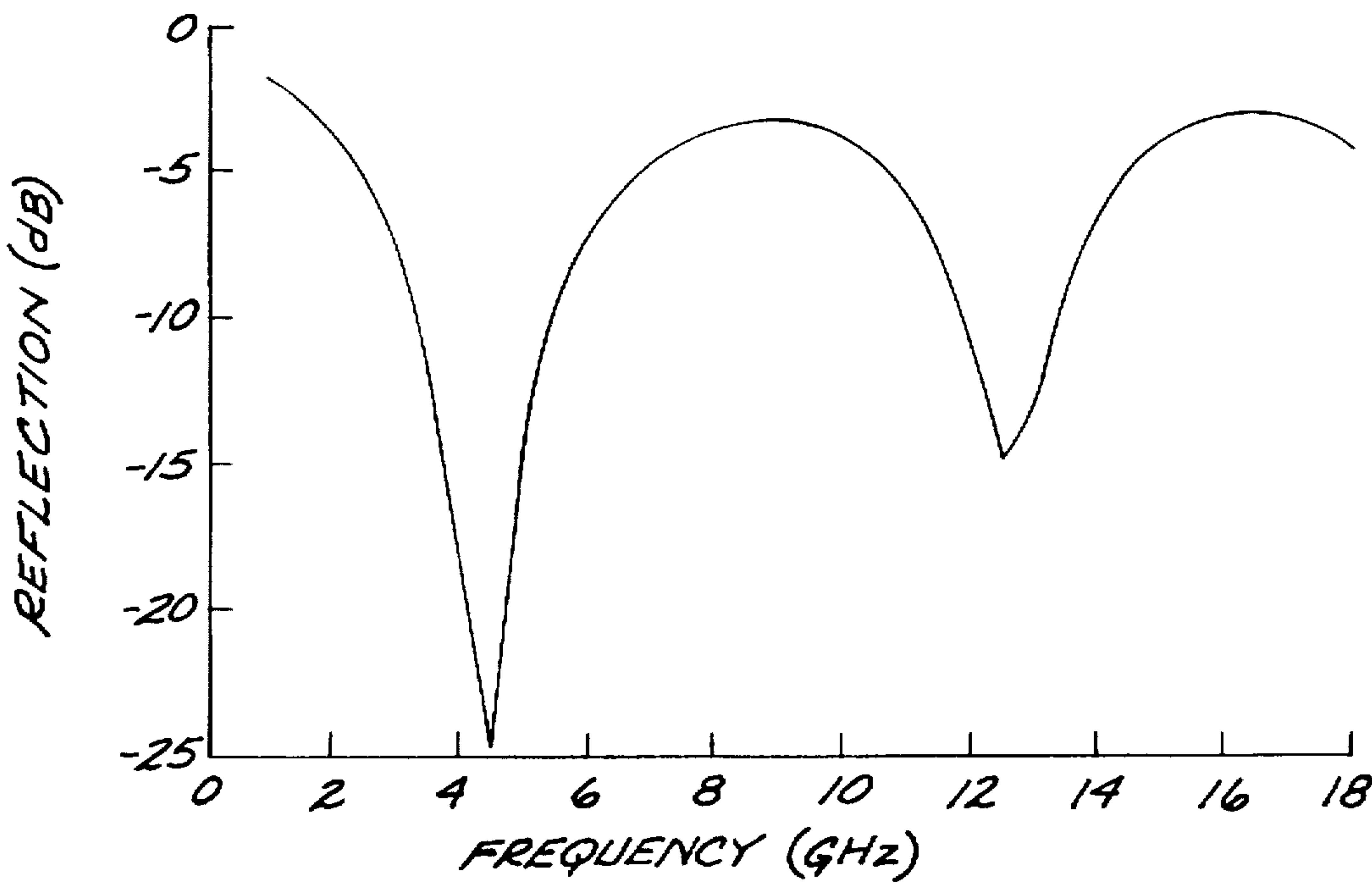
FIG. 17 BK7/BK7 WINDOW
