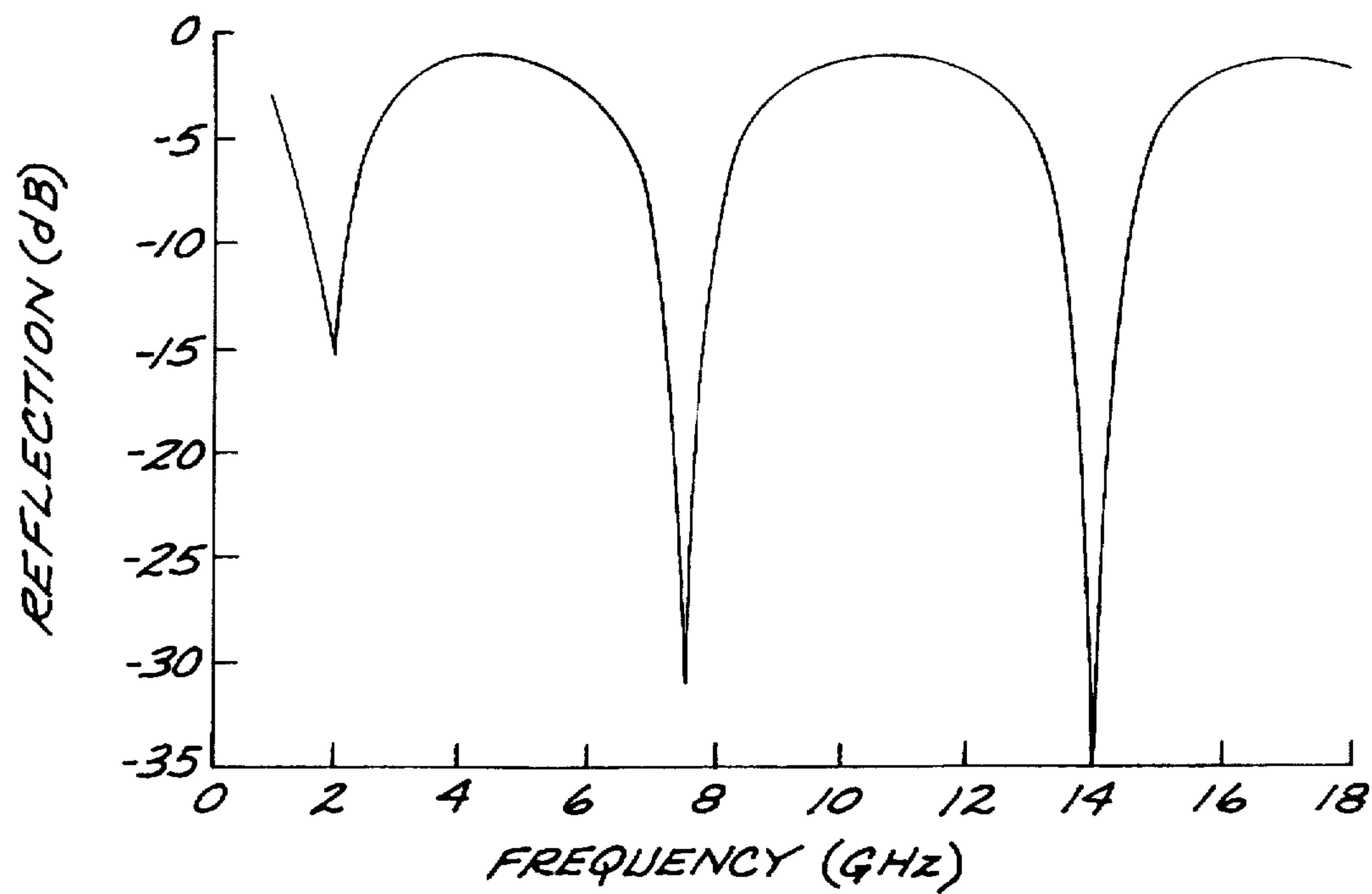
FIG. 16 SAPPHIRE-SILICON AIR SPACED WINDOW
