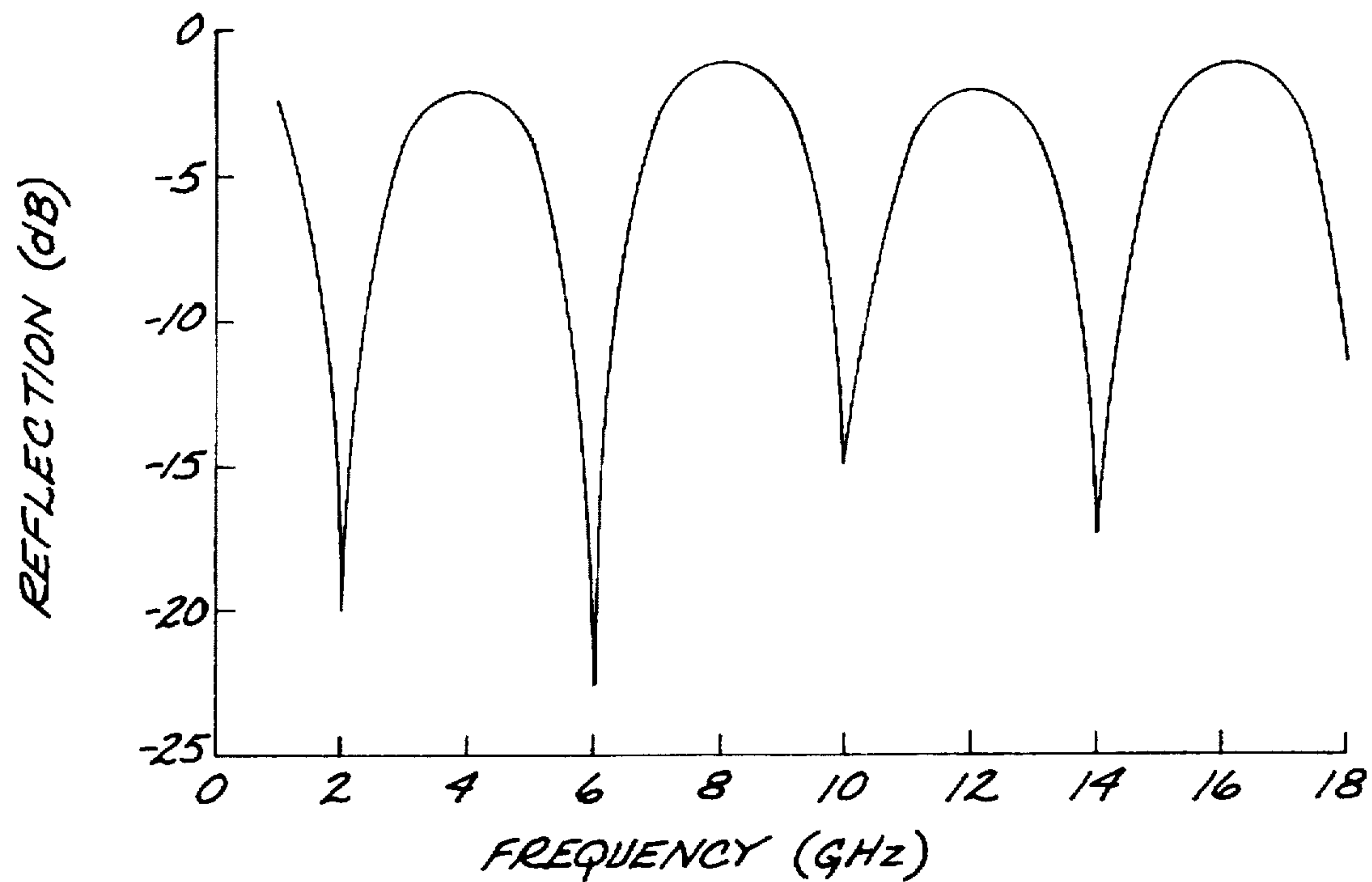
FIG. 12 ZnSe/ZnSe WINDOW
