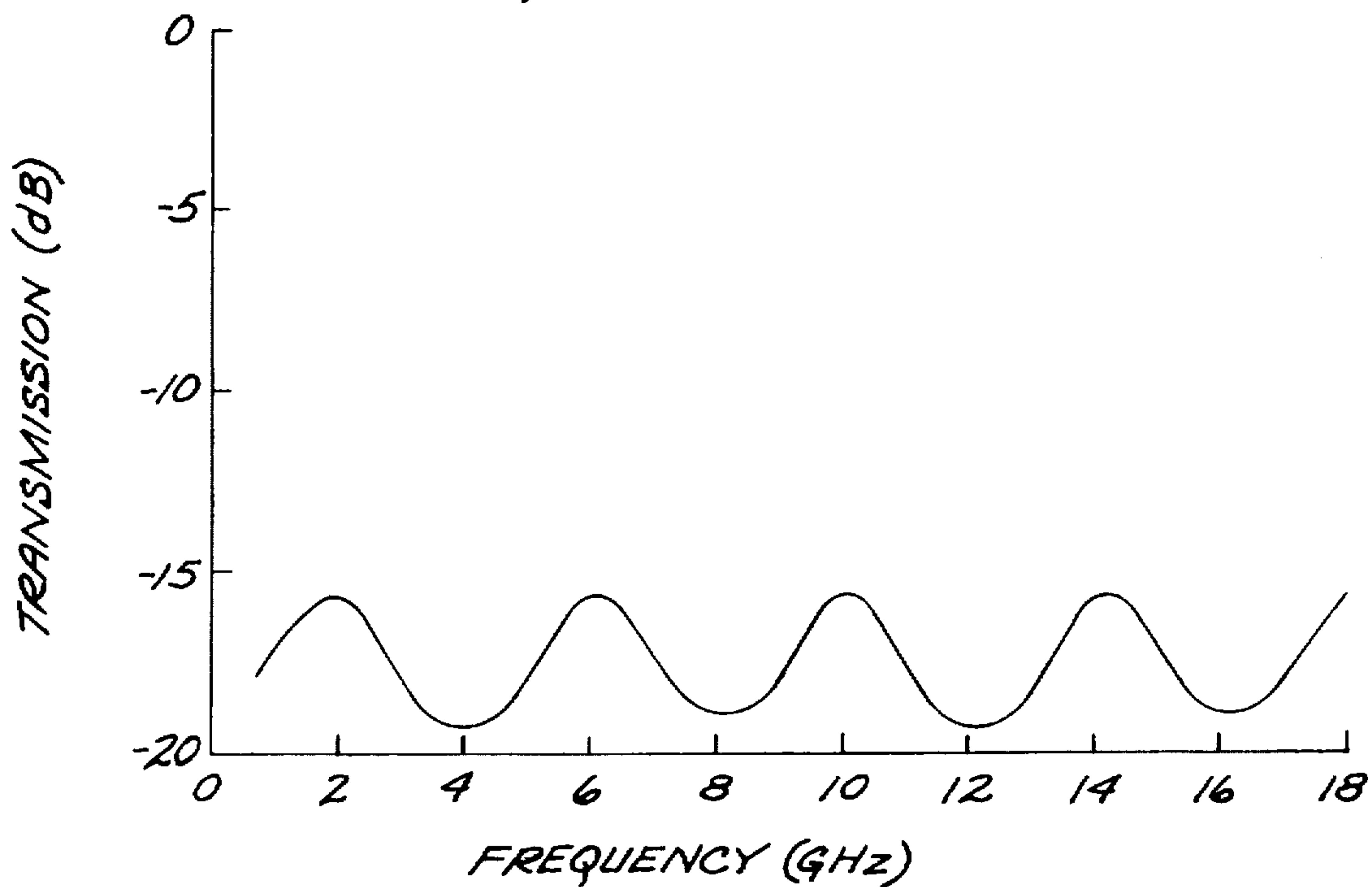
FIG. 13 ZnSe/ZnSe WINDOW
