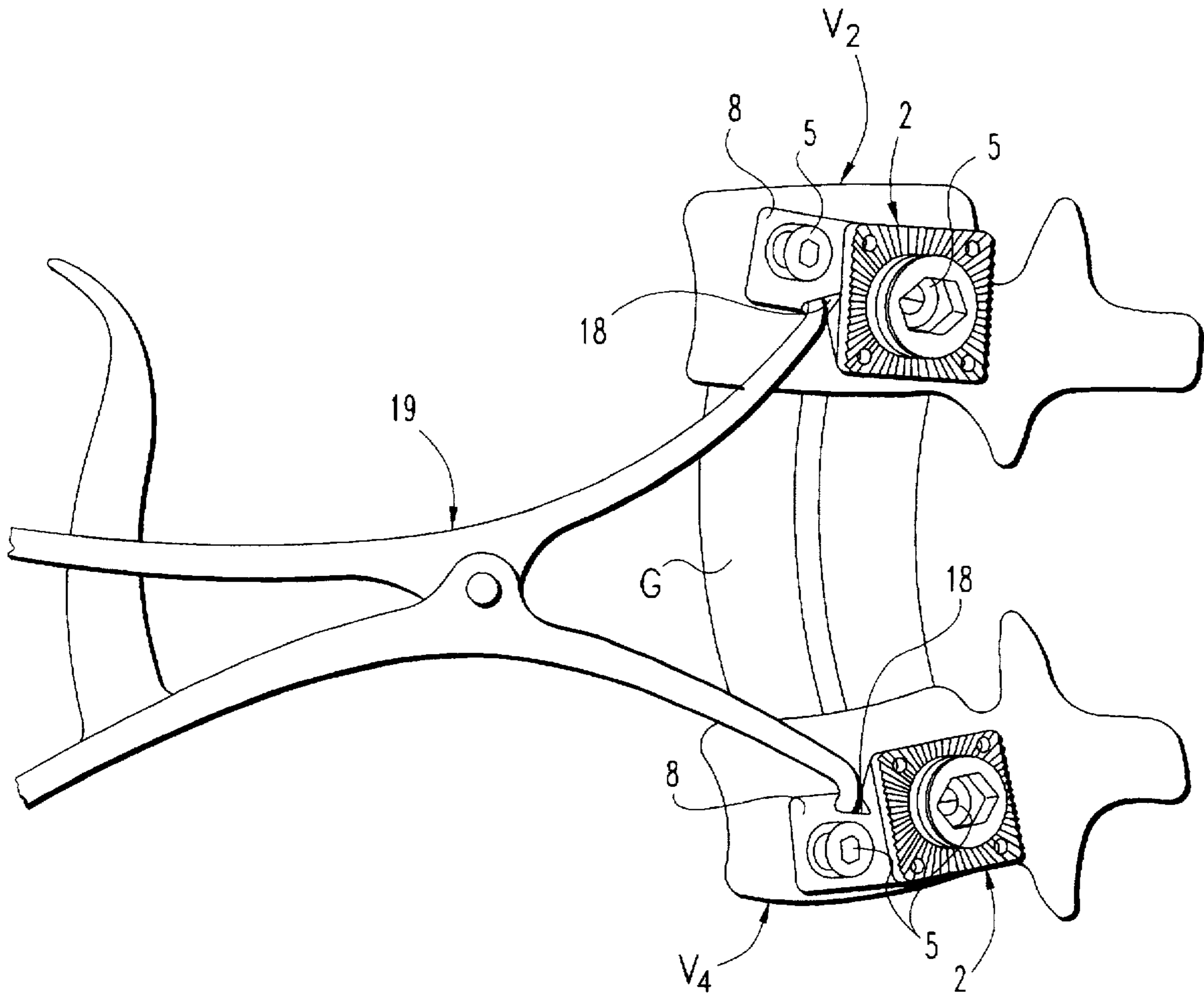
Fig. 2 (PRIOR ART)
