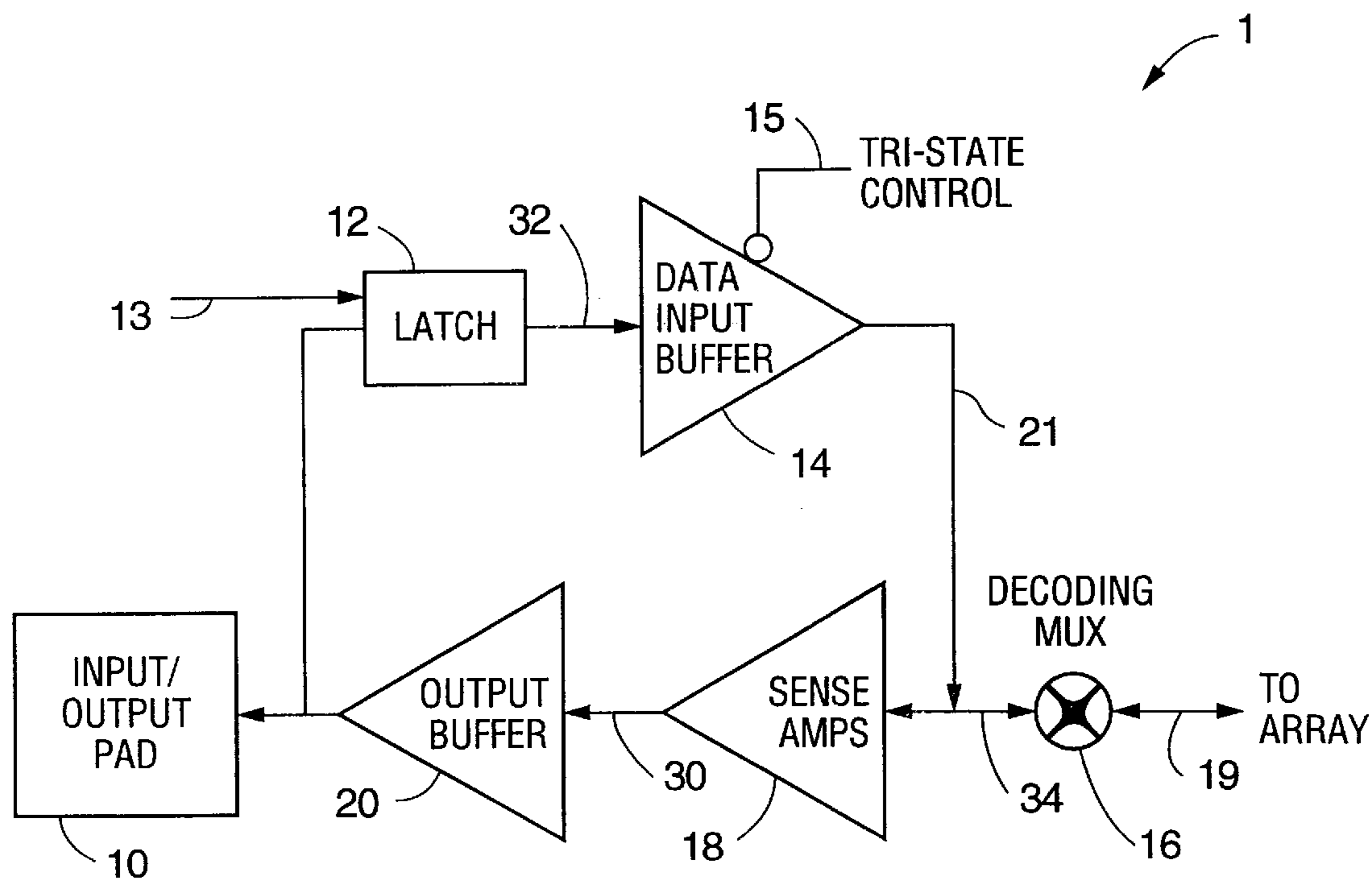
FIG. 1 (PRIOR ART)
