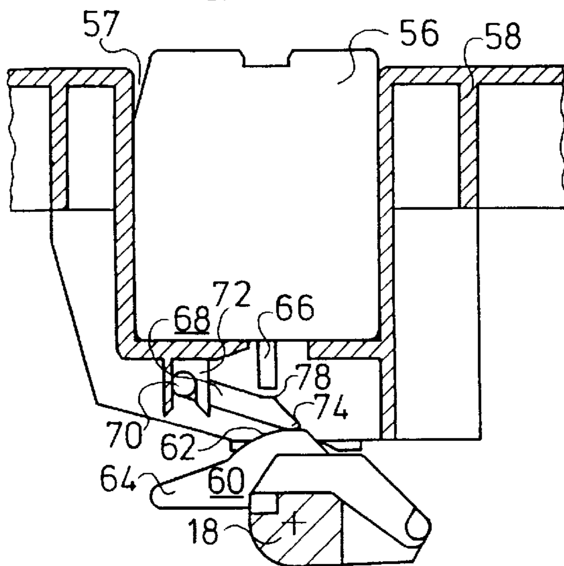
Fig.4 ENGAGED
