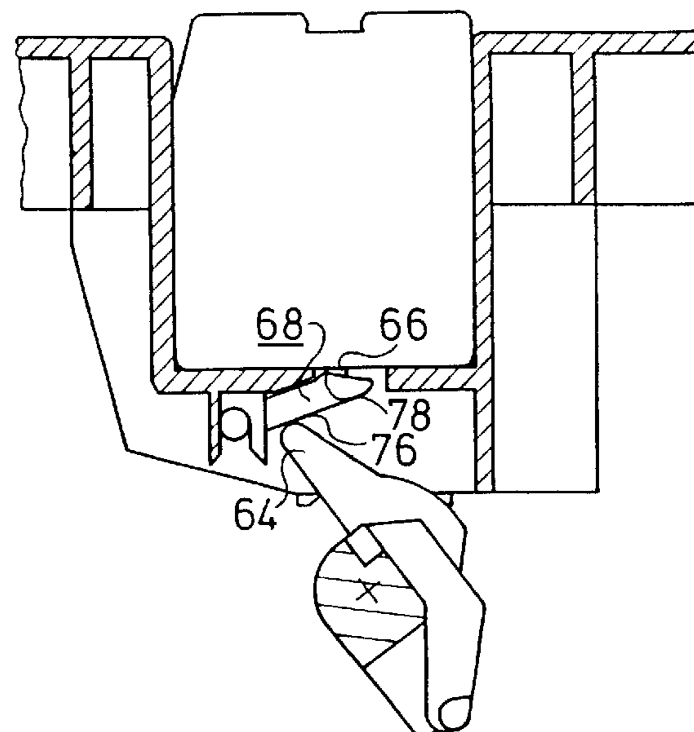
Fig.5 TRIPPED
