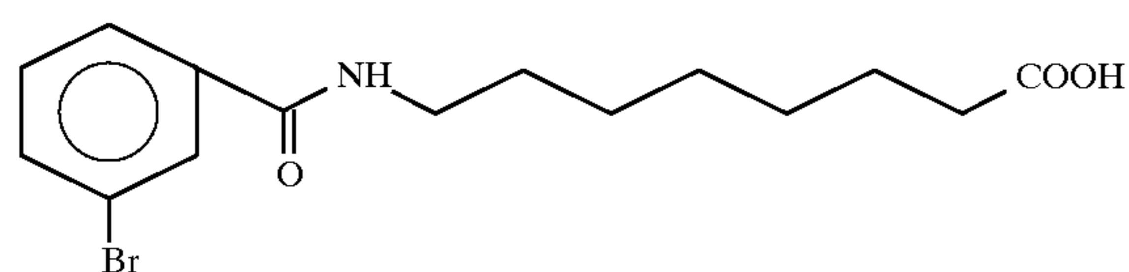
8-[N-(3-bromobenzoyl)]aminocaprylic acid
