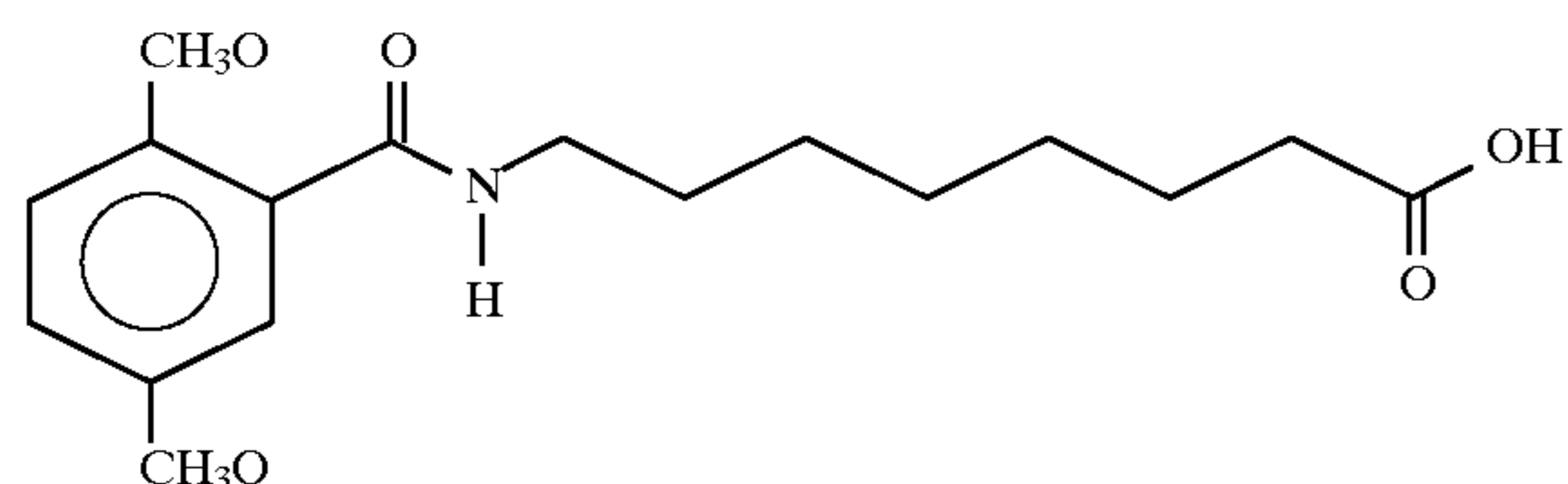
8-(N-(2,5-Dimethoxybenzoyl))aminocaprylic acid
