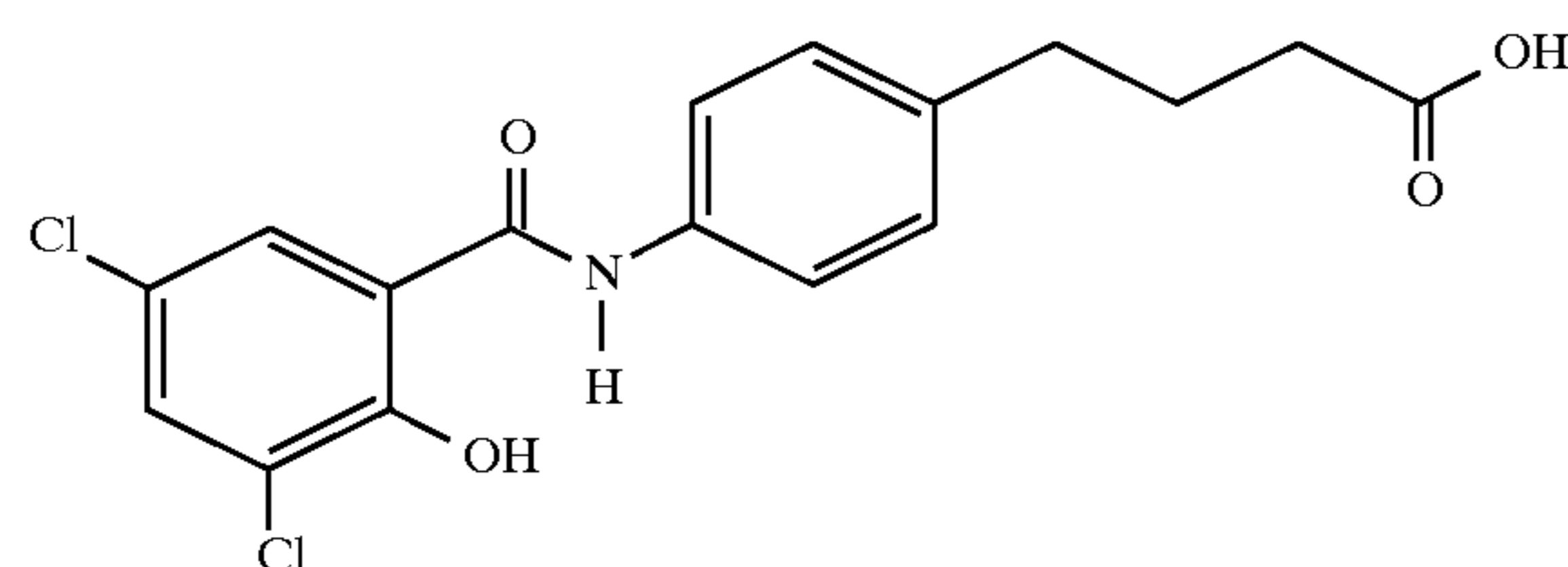
N-[3,5-dichloro-2-hydroxybenzoyl-4(4aminophenyl)]butyric acid
