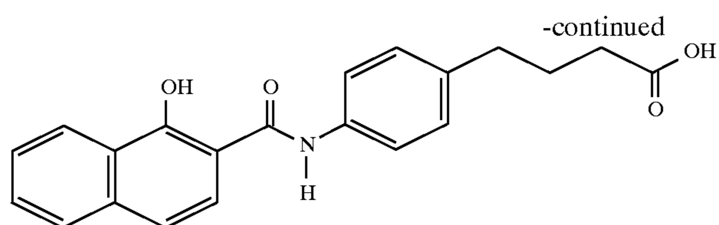
4-[4-[N-(1-hydroxy-2-naphthoyl)aminophenyl]]butyric acid
