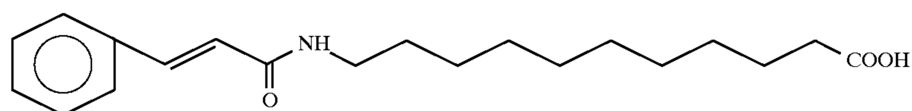
11-cinnamoylamoniundecanoic acid
