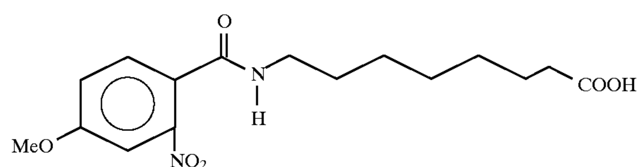
8-N-(4-methoxy-3-nitrobenzoyl)aminocaprylic acid
