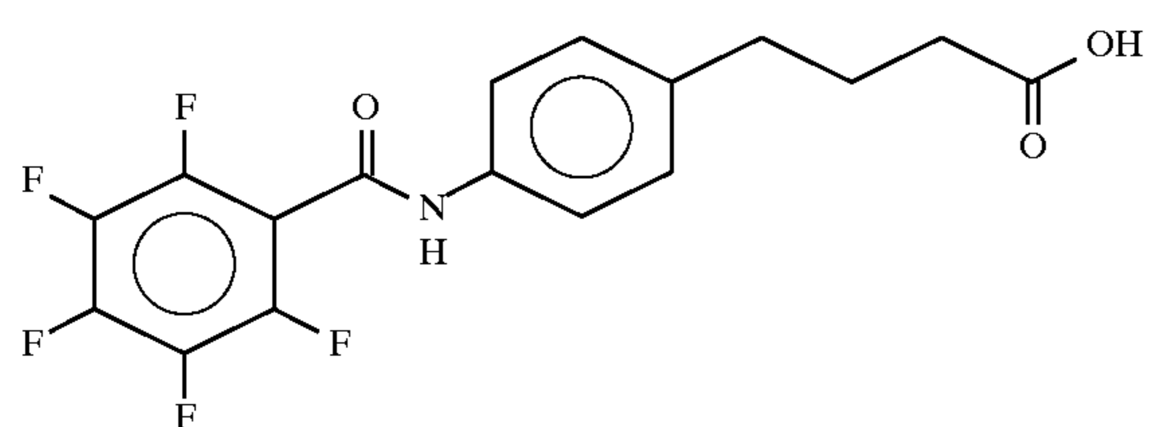
4-(4-(pentafluorobenzoyl)aminophenyl)butyric acid
