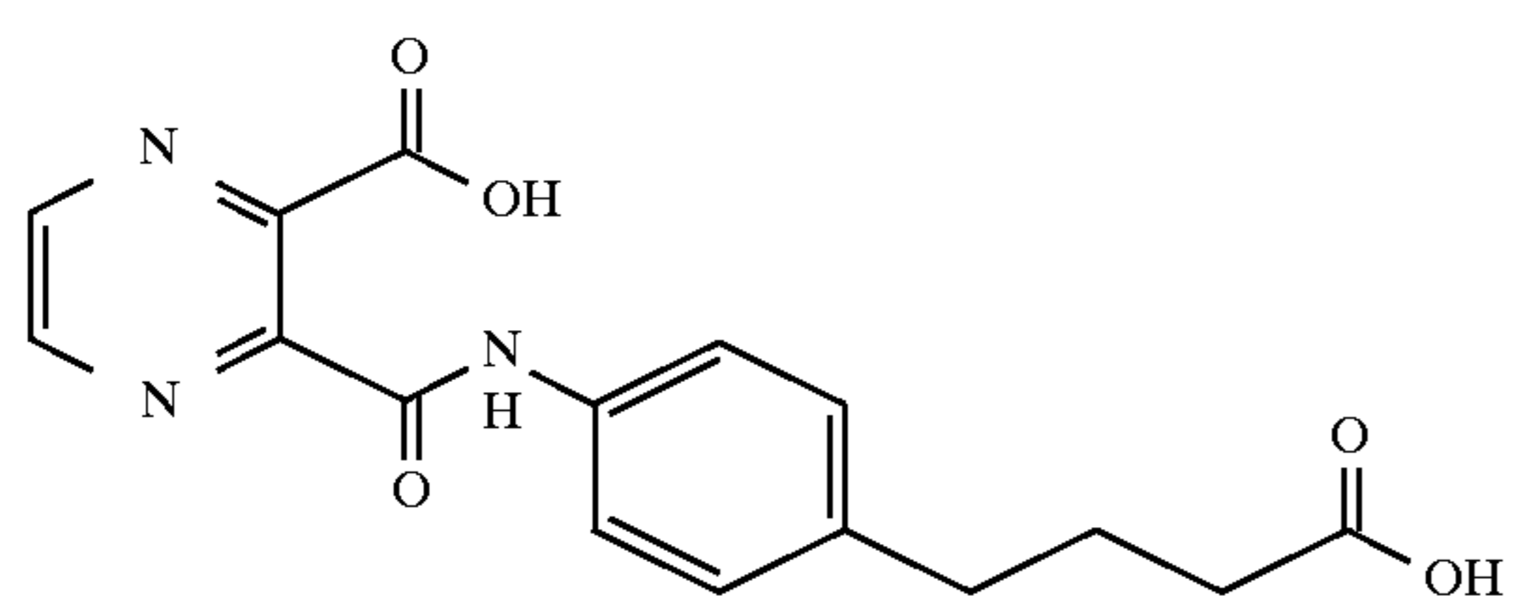
4-(4-(2-(3-carboxyl)pyrazinecarbonyl)aminophenyl)butyric acid
