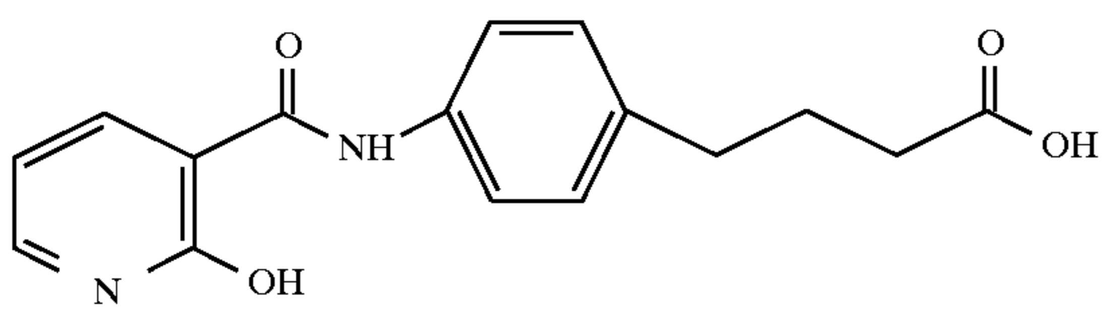
4-(4-(2-hydroxynicotinoyl)aminophenyl)butyric acid
