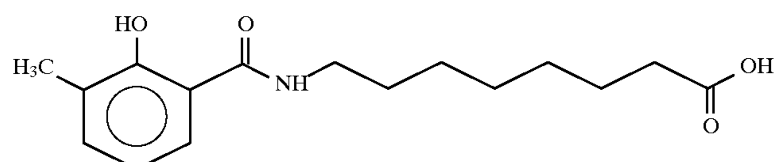
8-(N-3-methylsalicyloyl)aminocaprylic acid
