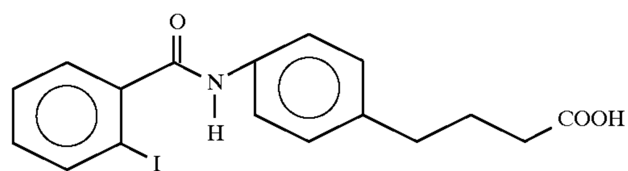
4-{4-[N-(2-iodobenzoyl)aminophenyl]}butyric acid
