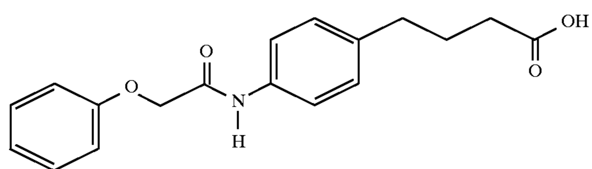
4-(4-(phenoxyacetyl)aminophenyl)butyric acid
