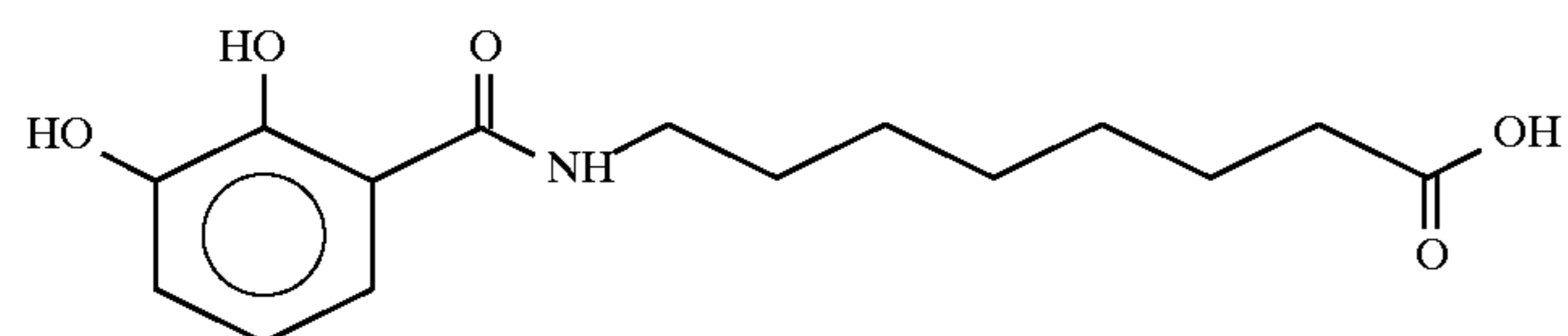
8-(N-2,3-Dihydroxybenzoyl)aminocaprylic acid
