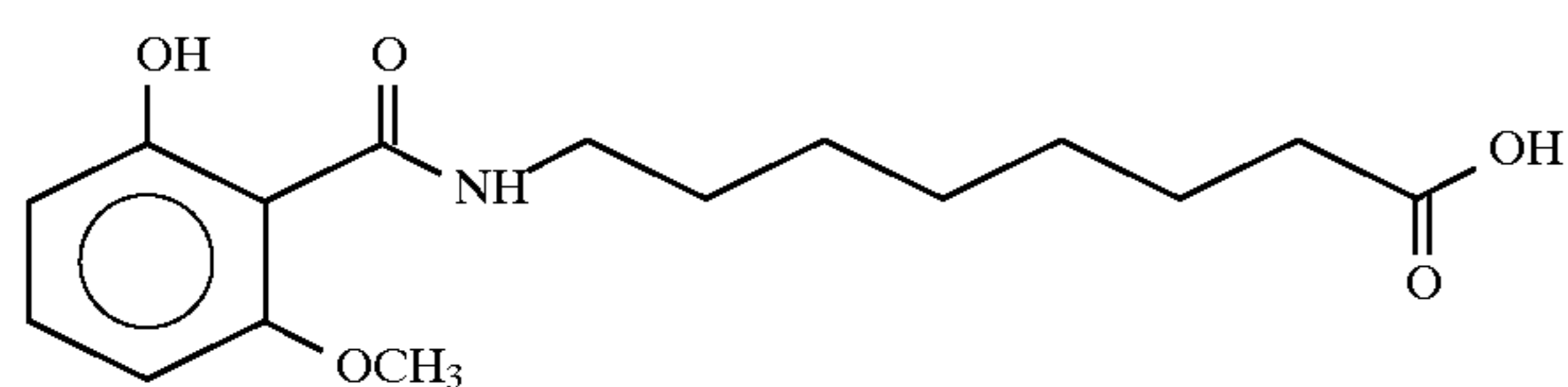
8-(N-2-Hydroxy-6-methoxybenzoyl)aminocaprylic acid
