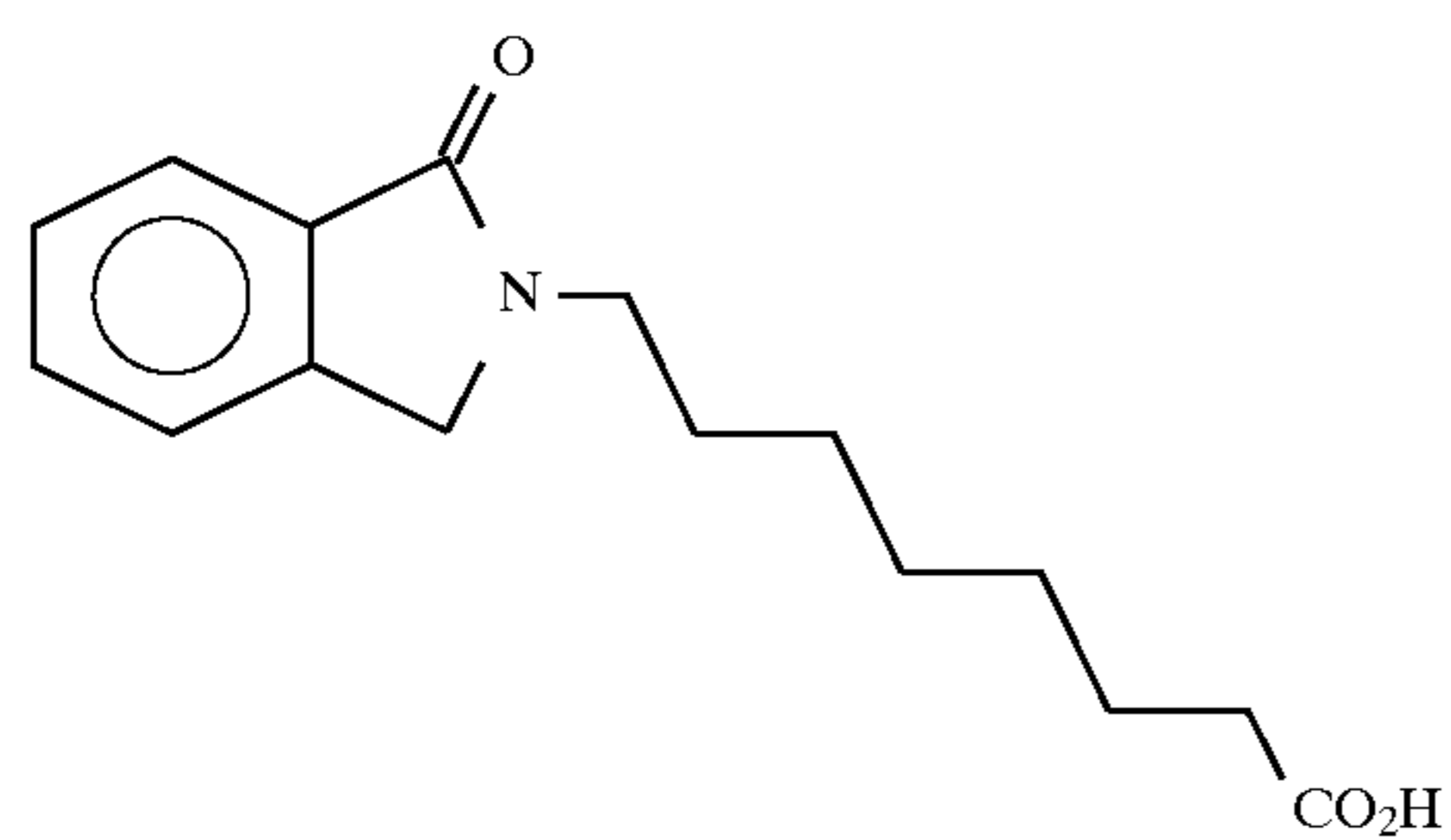
8-(2-(1,2-dihydroisindole-1-one))octanoic acid
