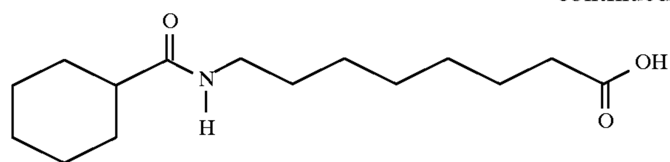
8-N-cyclohexanoylaminovaleric acid
