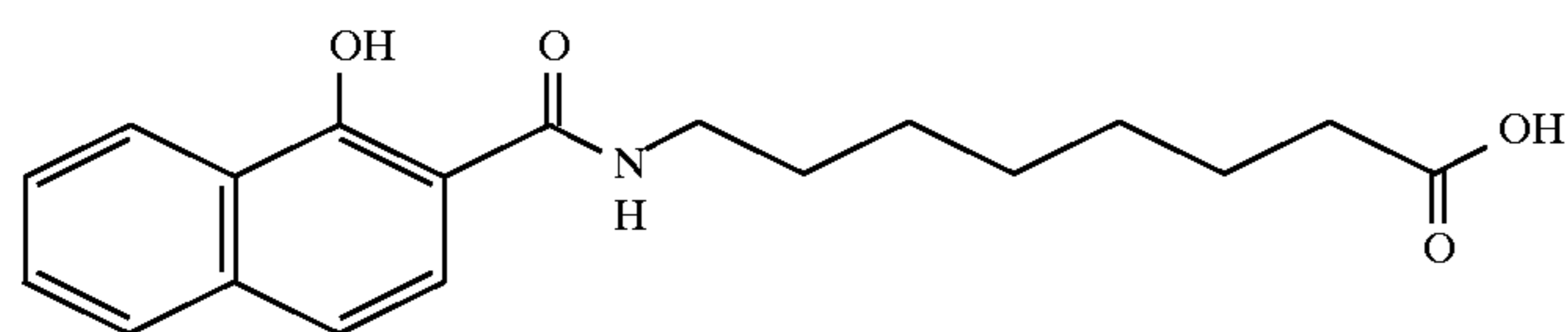
8-(N-(1-hydroxy-2-naphthoyl)aminocaprylic acid
