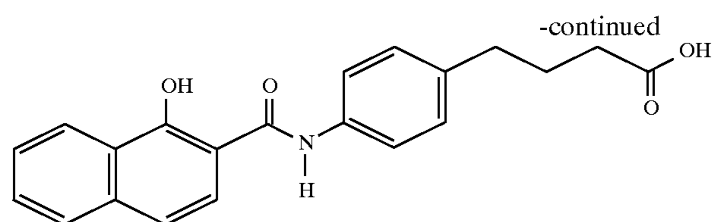
4-[4-[N-(1-hydroxy-2-naphthoyl)aminophenyl]]butyric acid
