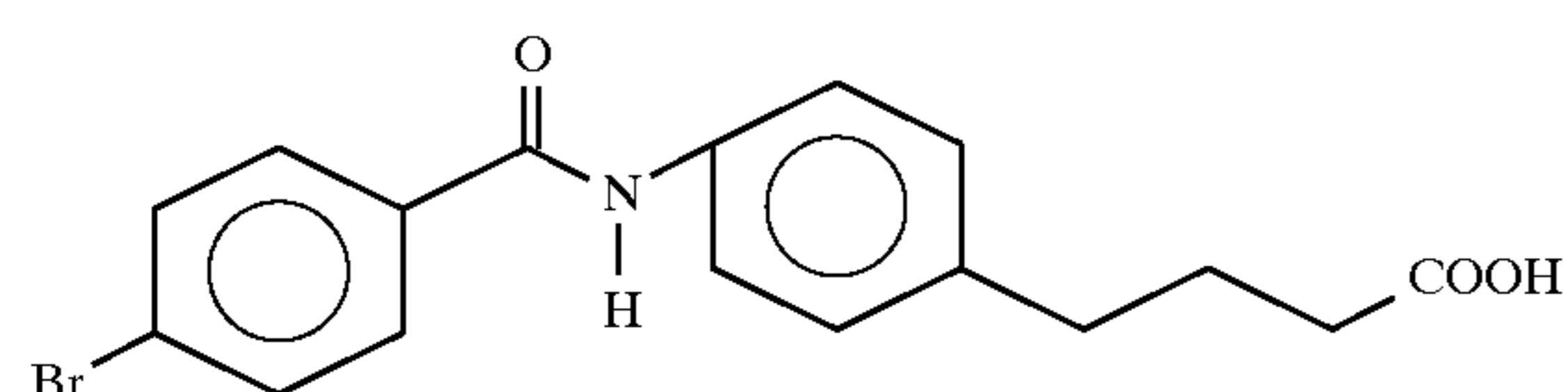
4-{4-[N-(4-bromobenzoyl)aminophenyl]}butyric acid
