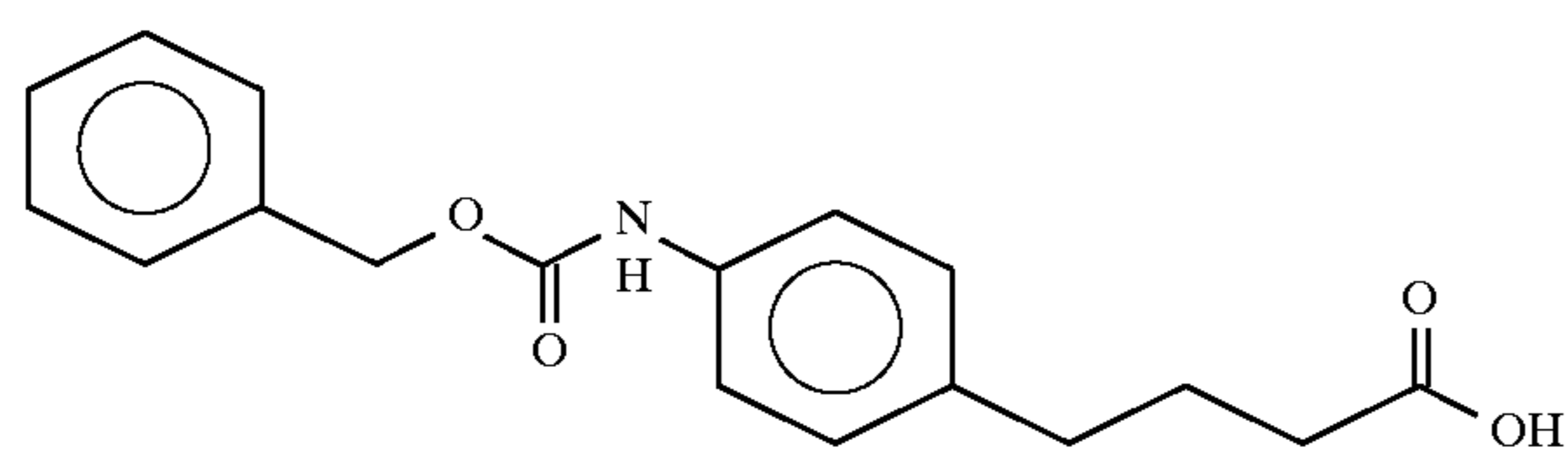
4-(4-benzyloxycarbonylamino)phenyl)butyric acid
