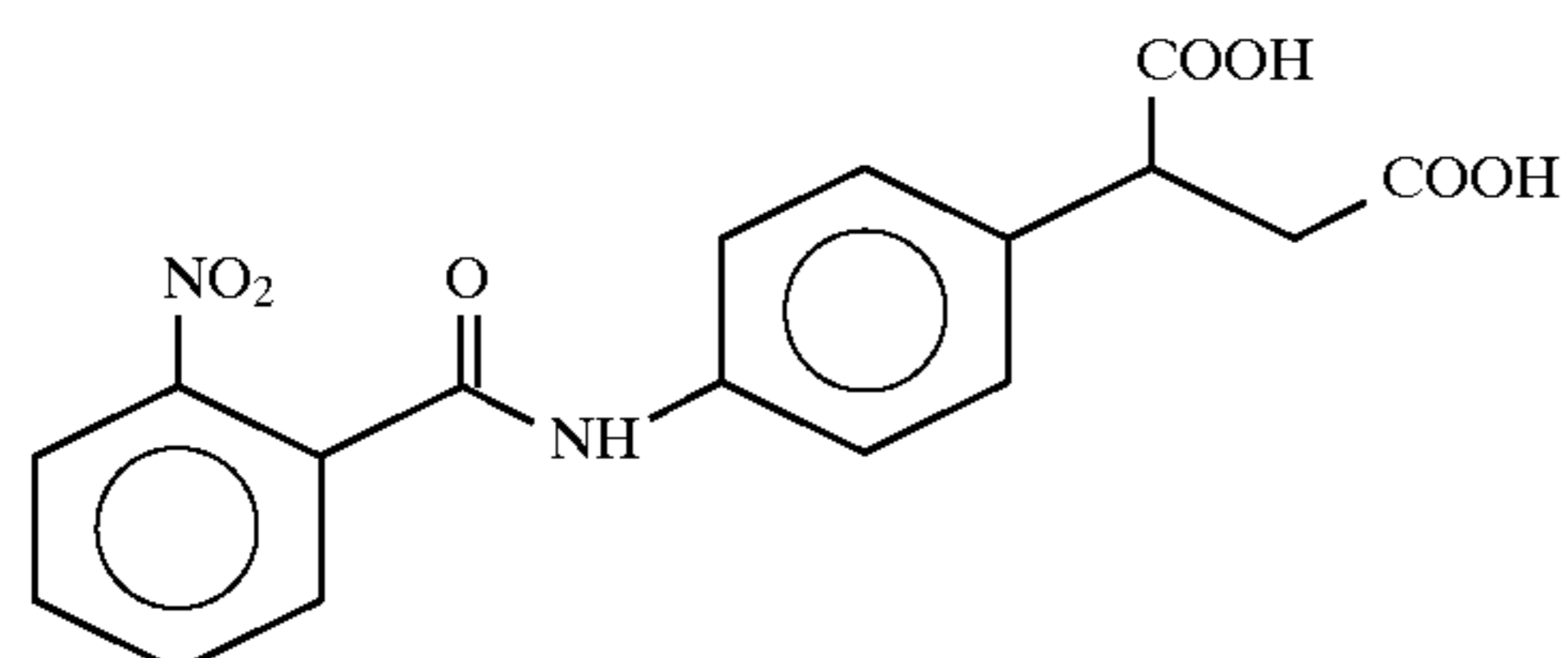
4-(2-Nitrobenzoyl)aminophenylsuccinic acid
