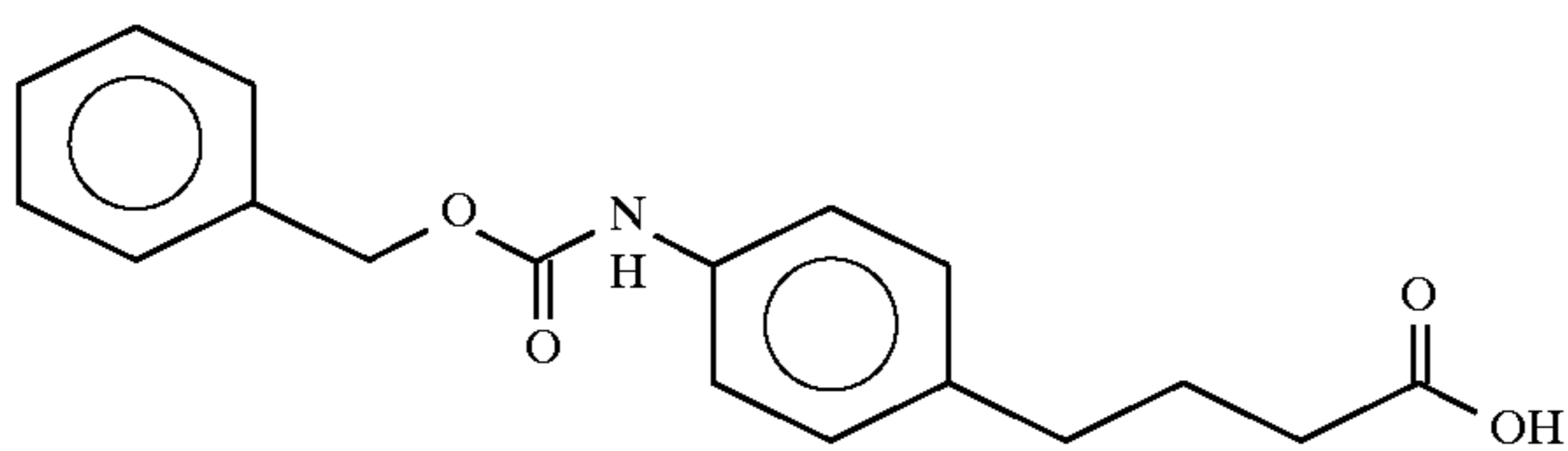
4-(4-benzyloxycarbonylamino)phenyl)butyric acid
