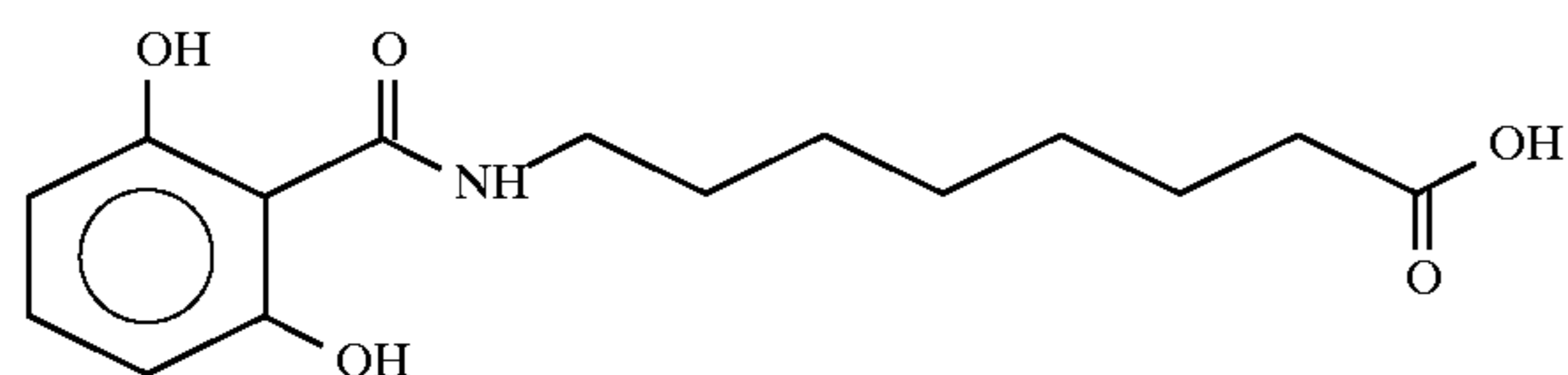
8-(N-2,6-Dihydroxybenzoyl)aminocaprylic acid
