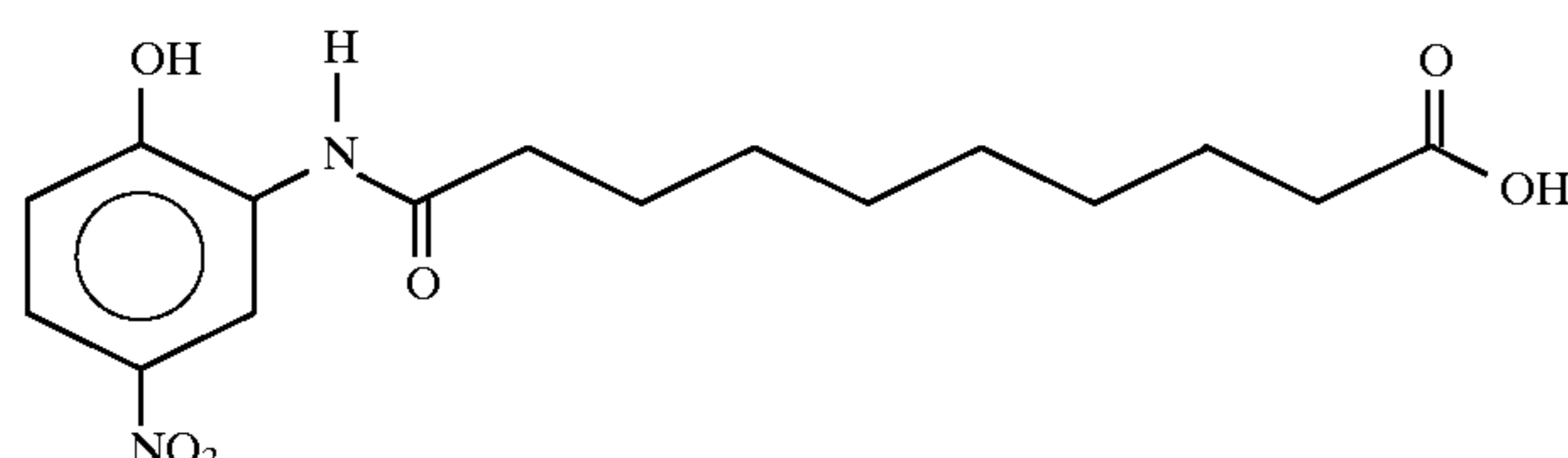
N-10-(2-hydroxy-5-nitroanilino)decanoic acid
