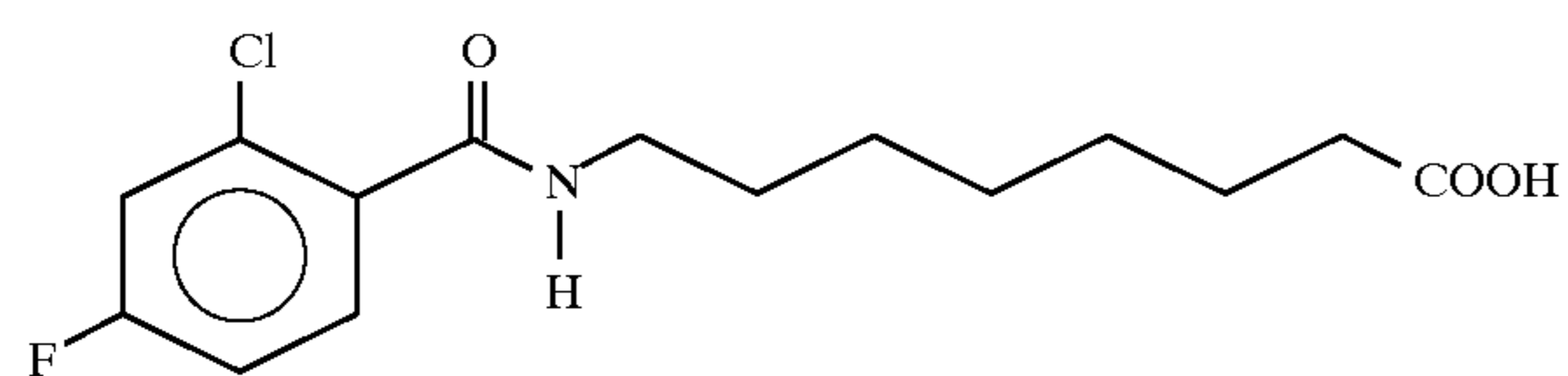
8-(N-(2-chloro-4-fluorobenzoyl)aminocaprylic acid
