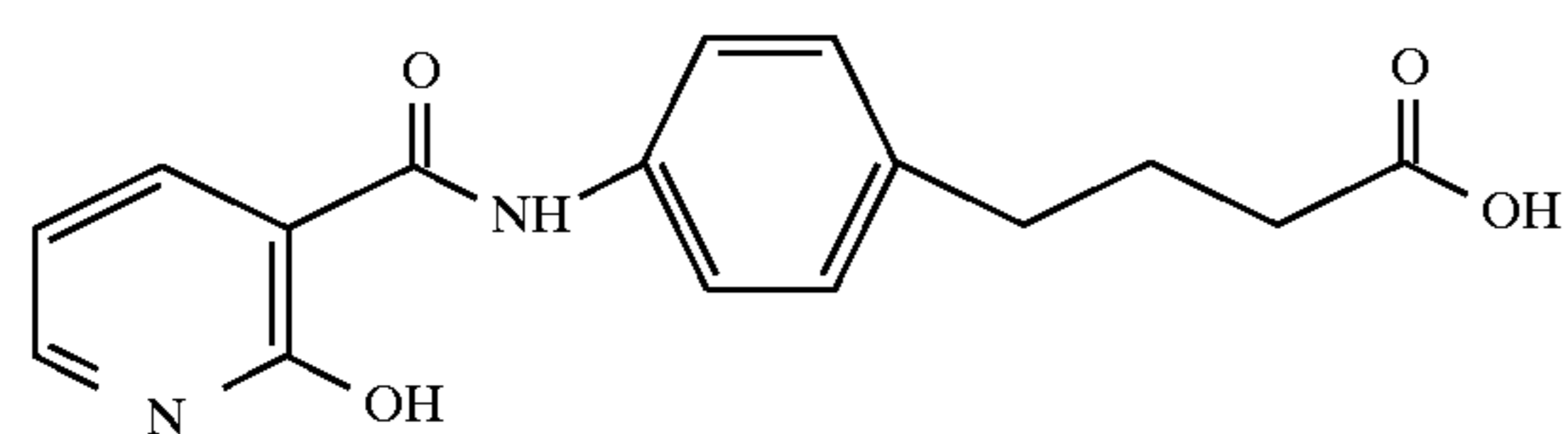
4-(4-(2-hydroxynicotinoyl)aminophenyl)butyric acid
