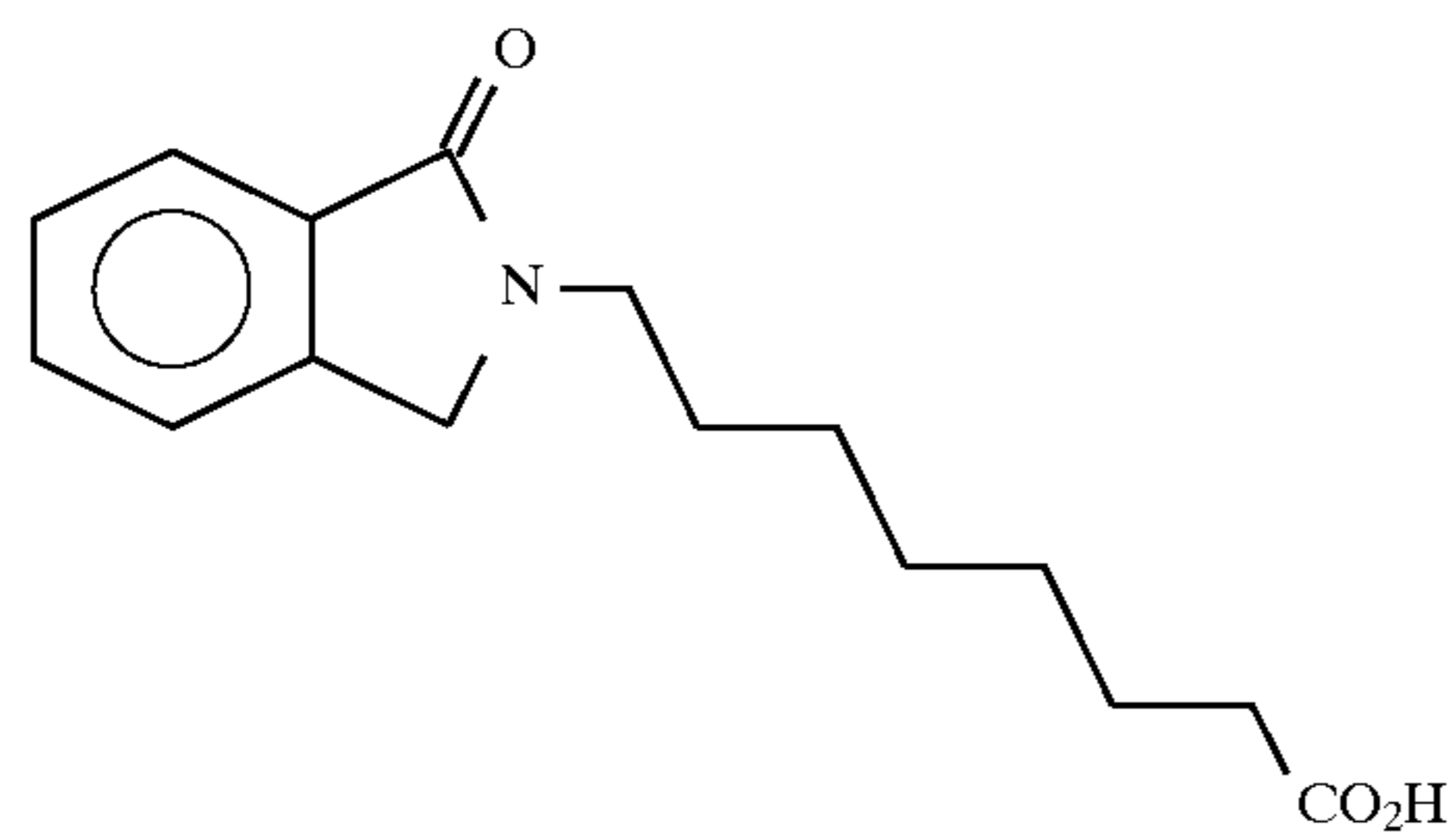
8-(2-(1,2-dihydroisindole-1-one))octanoic acid
