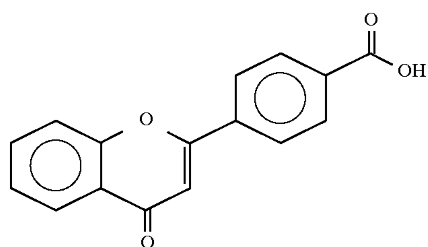
4'-flavonic acid
