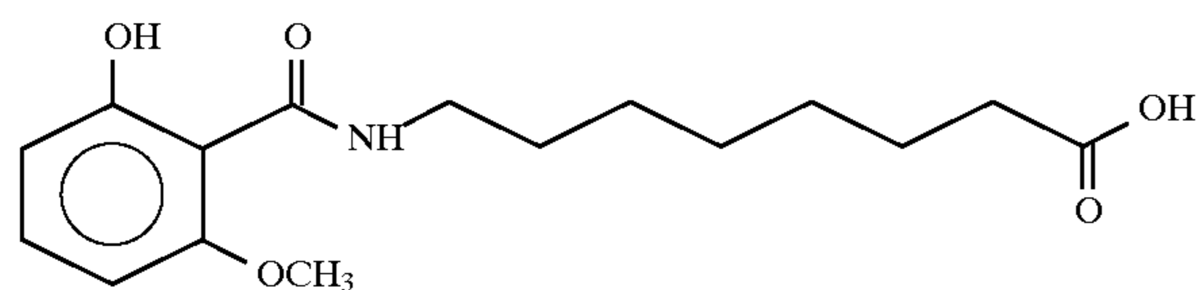
8-(N-2-Hydroxy-6-methoxybenzoyl)aminocaprylic acid
