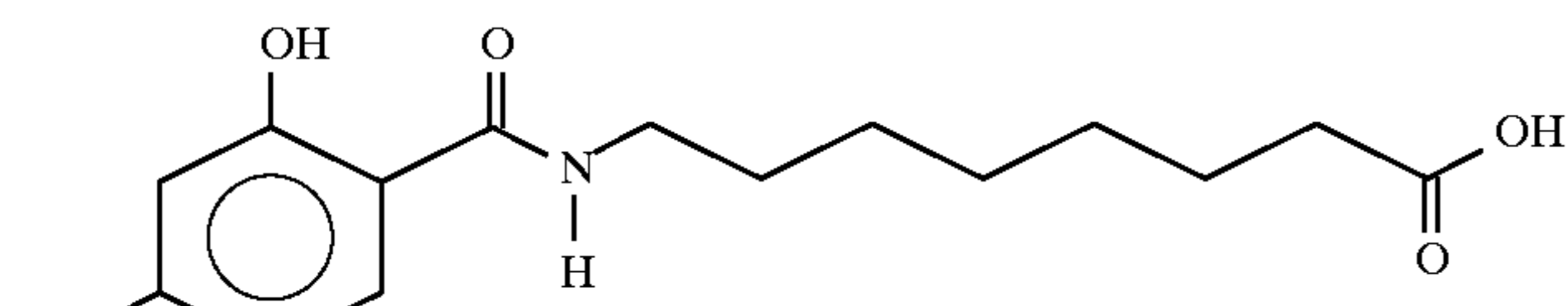
8-(N-(2,4-Dihydroxybenzoyl))aminocaproic acid
