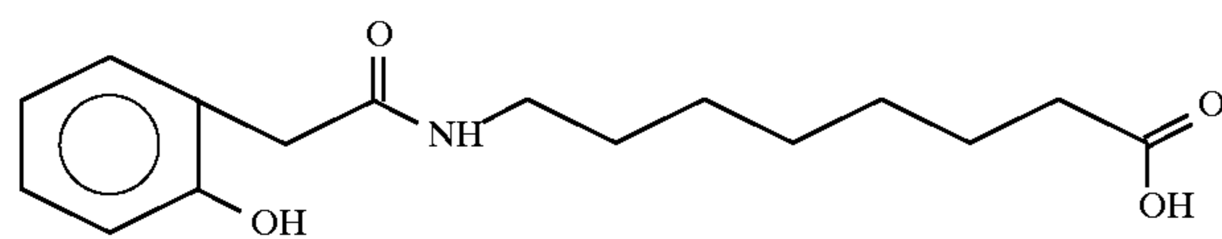
8-(2-hydroxyphenoxy)aminocaproic acid
