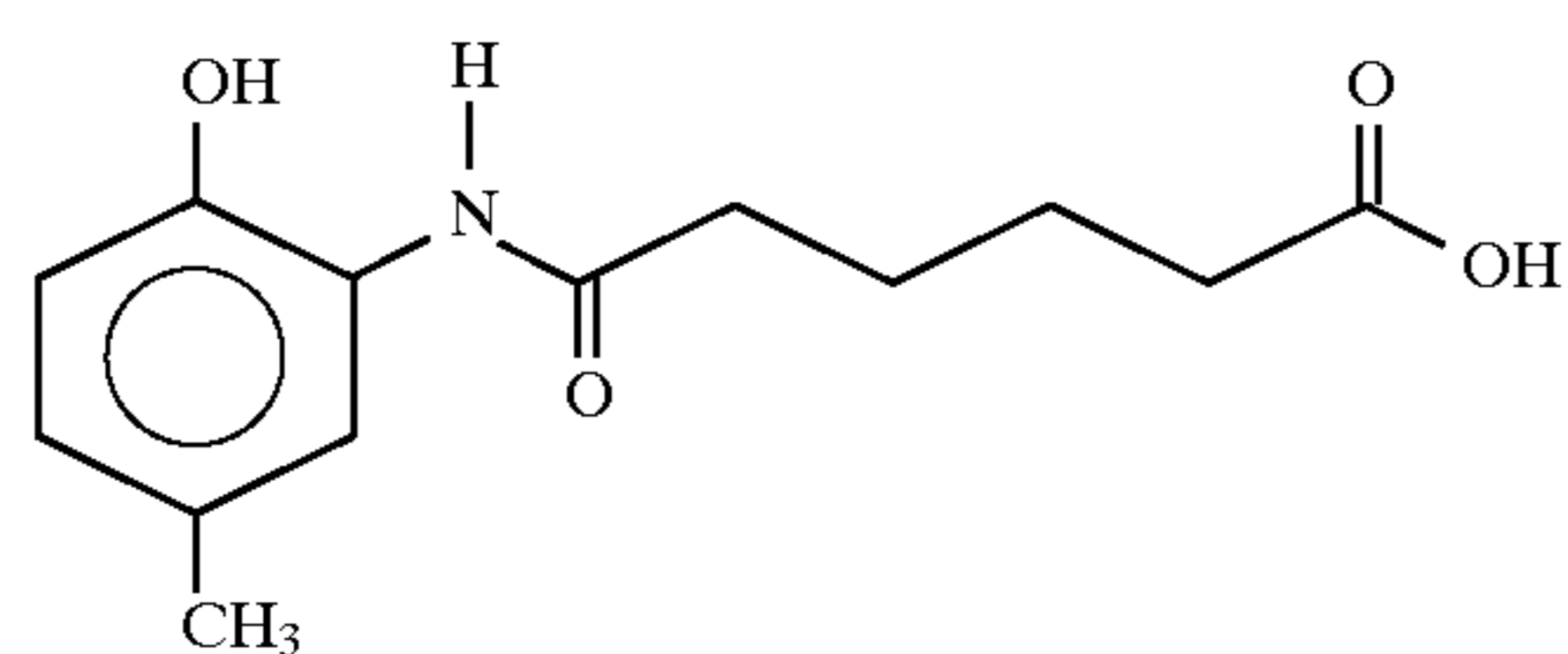
5-(2-hydroxy-5-methylanilino)valeric acid
