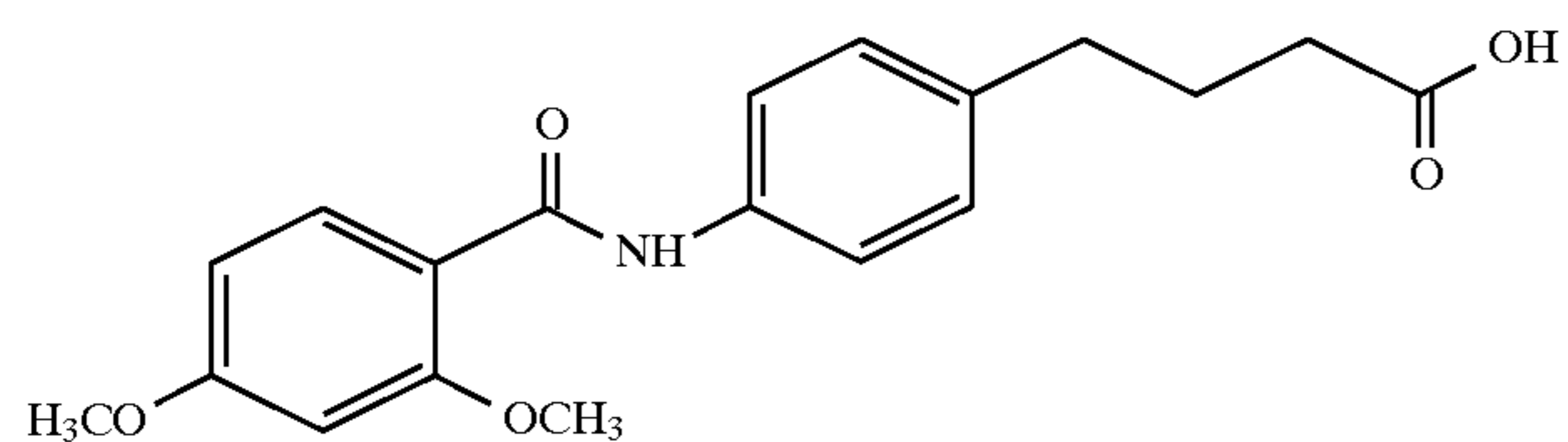
4-(4-(2,4-dimethoxybenzoyl)aminophenyl)butyric acid
