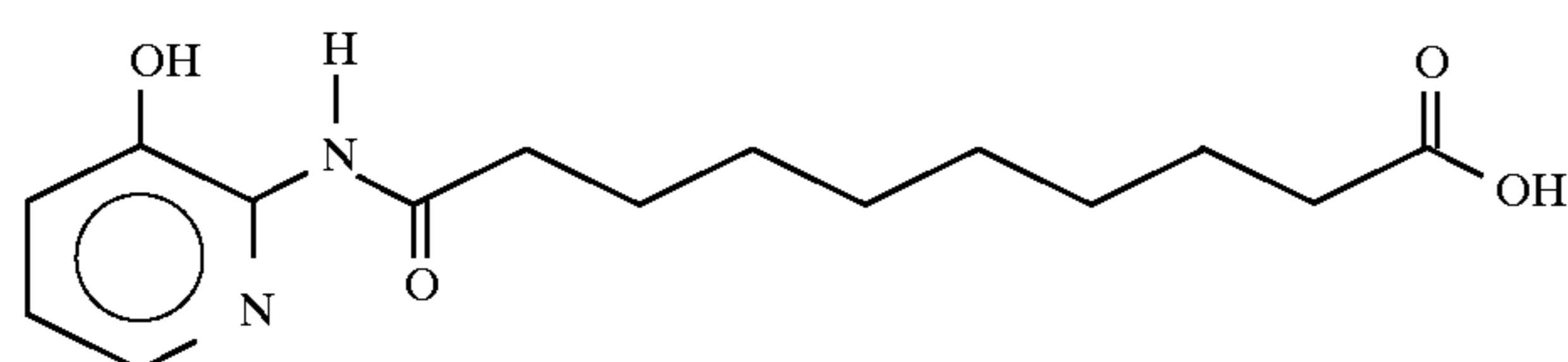
9-[2-(3-hydroxy)pyridylaminocarbonyl]nonanoic acid
