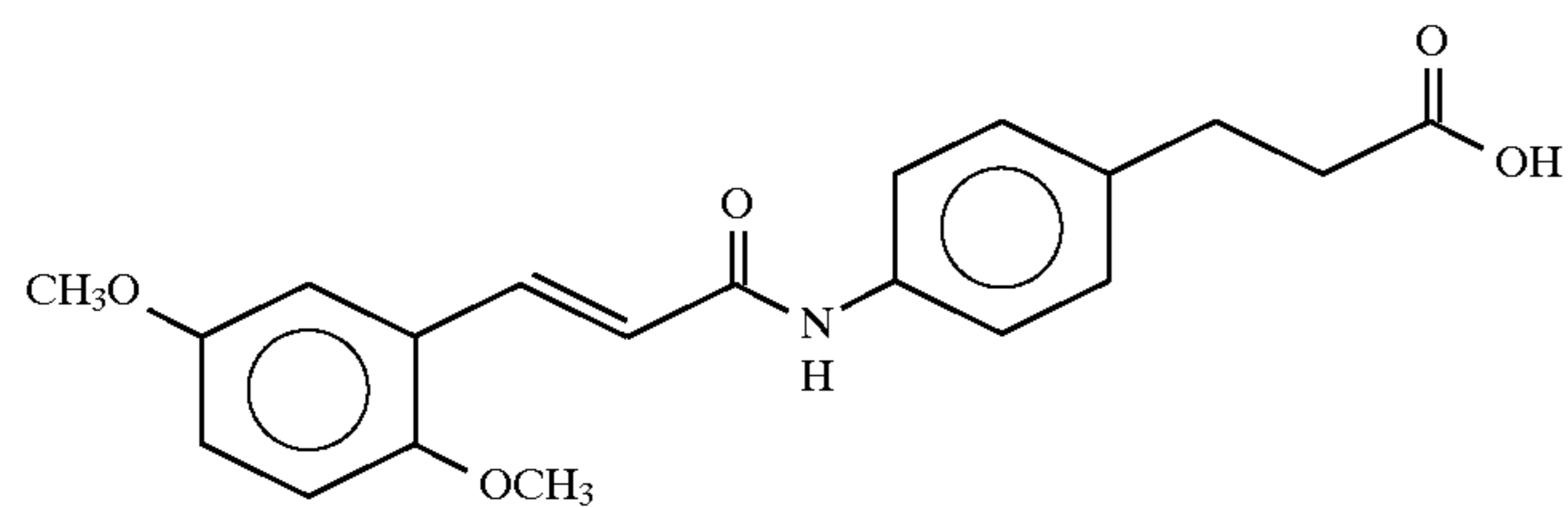
3-(4-(2,5-dimethoxycinnamoyl)aminophenyl)propionic acid
