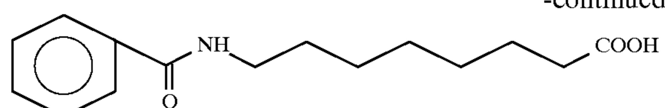
8-[N-(3-fluorobenzoyl)]aminocaprylic acid
