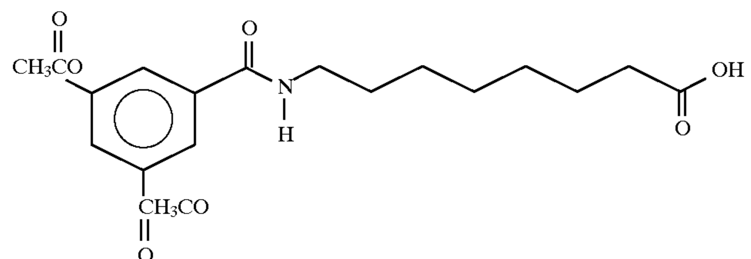
8-(N-(3,5-Diacetyloxybenzoyl)]aminocaproic acid
