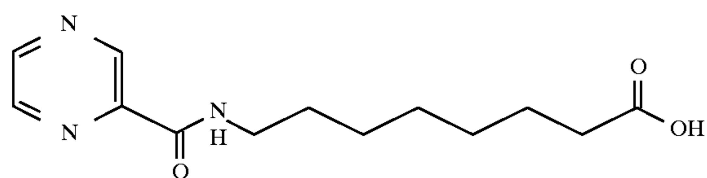
8-(2-pyrazinecarbonyl)aminocaproic acid
