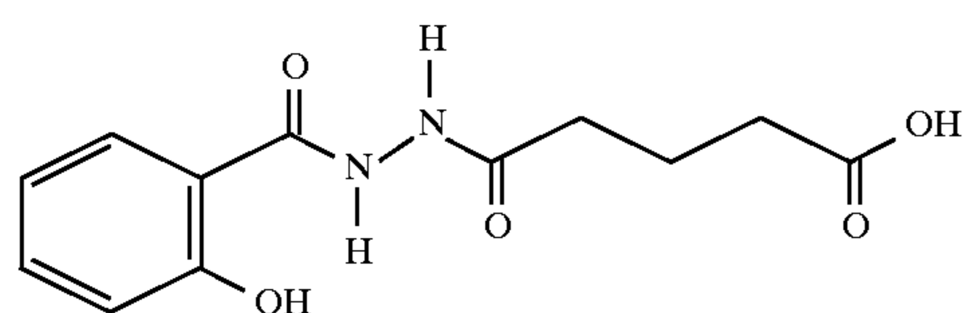
1-salicyloyl-2-glutaryl hydrazide
