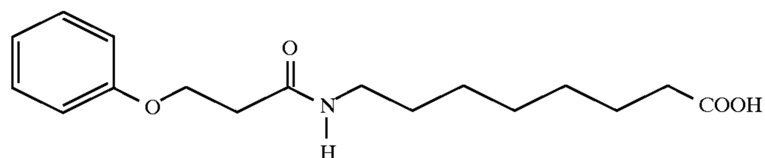
8-(3-Phenoxypropionylamino)caprylic acid
