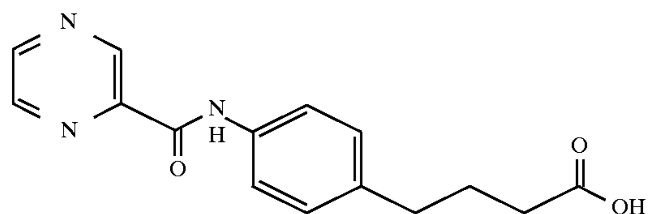
4-(4-(2-pyrazinecarbonyl)aminophenyl)butyric acid
