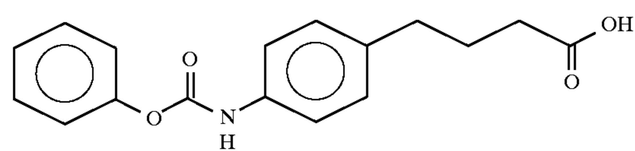
4-(4-phanyloxycarbonylamino)phenyl)butyric acid
