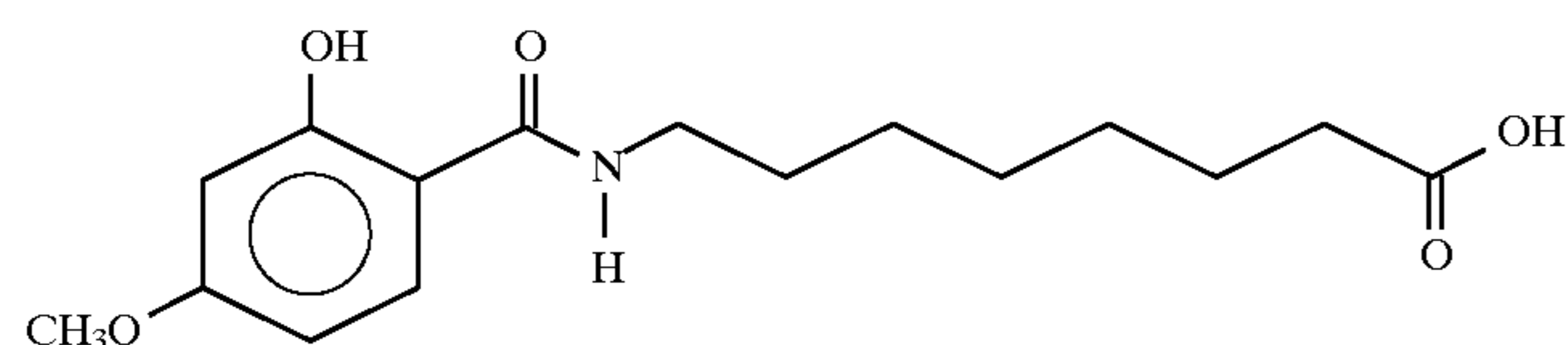
8-(N-2-Hydroxy-4-methoxybenzoyl)aminocaprylic acid
