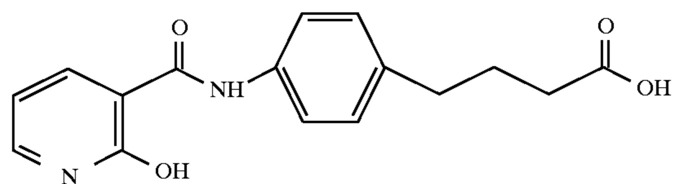
4-(4-(2-hydroxynicotinoyl)aminophenyl)butyric acid
