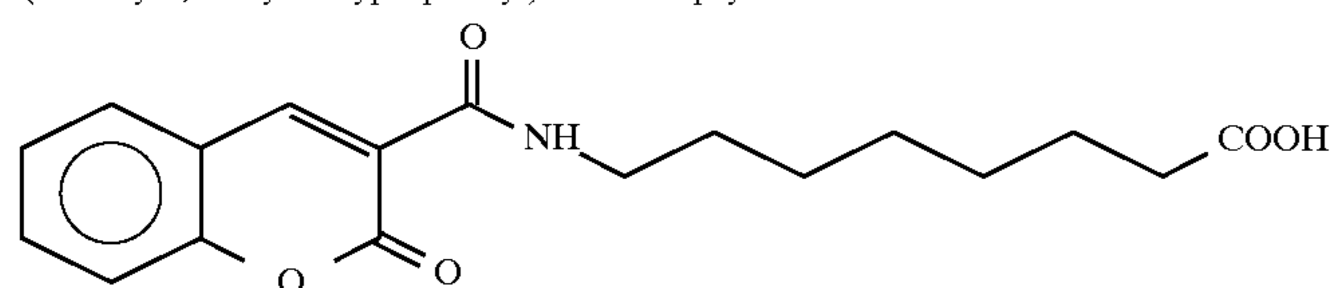
8-[N-(3-coumarincarbonyl)]aminocaprylic acid
