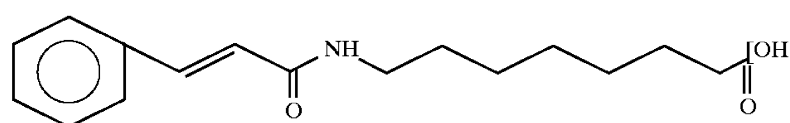
7-cinnamoylaminoheptanoic acid
