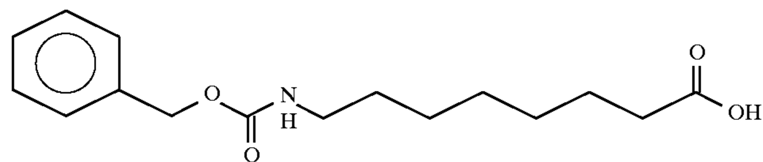
8-Benzylcarbonylamino)caprylic acid
