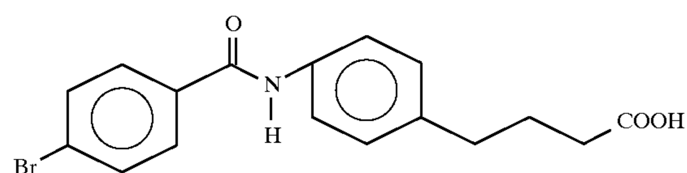
4-{4-[N-(4-bromobenzoyl)aminophenyl]}butyric acid
