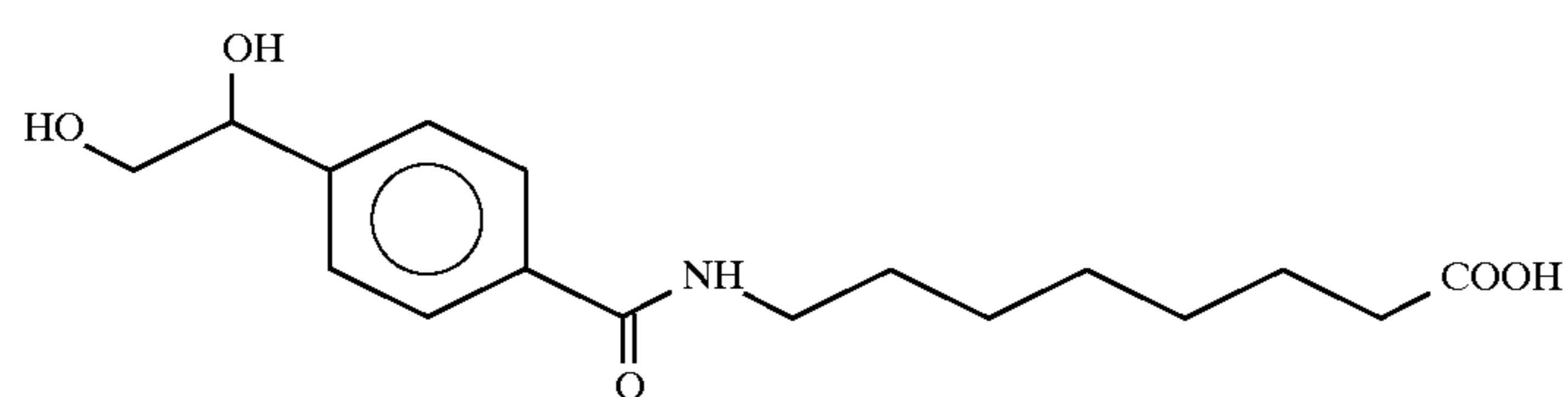
8-(4-(1,2-dihydroxyethyl)benzoyl)aminocaprylic acid
