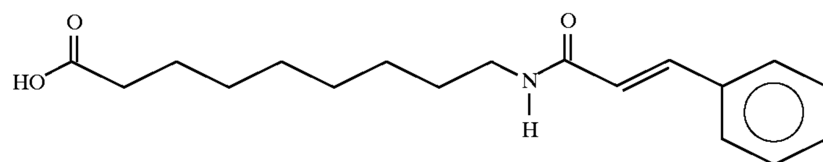
9-(cinnamoylamino)nonanoic acid
