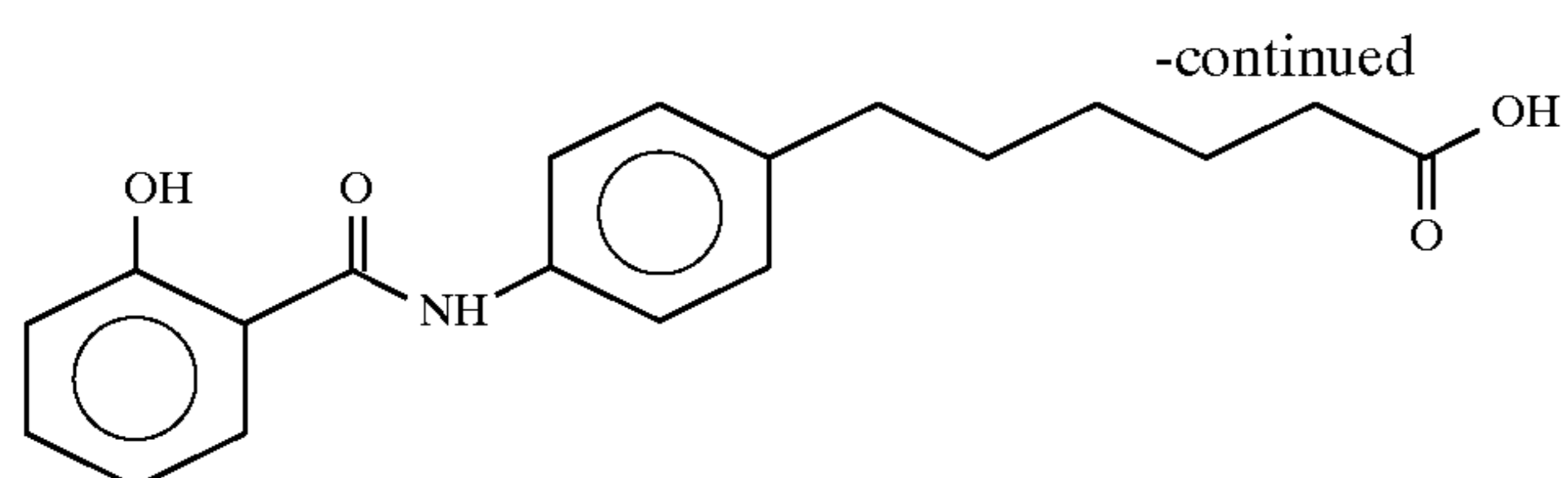
6-(4-salicyloyl)aminophenyl)hexanoic acid
