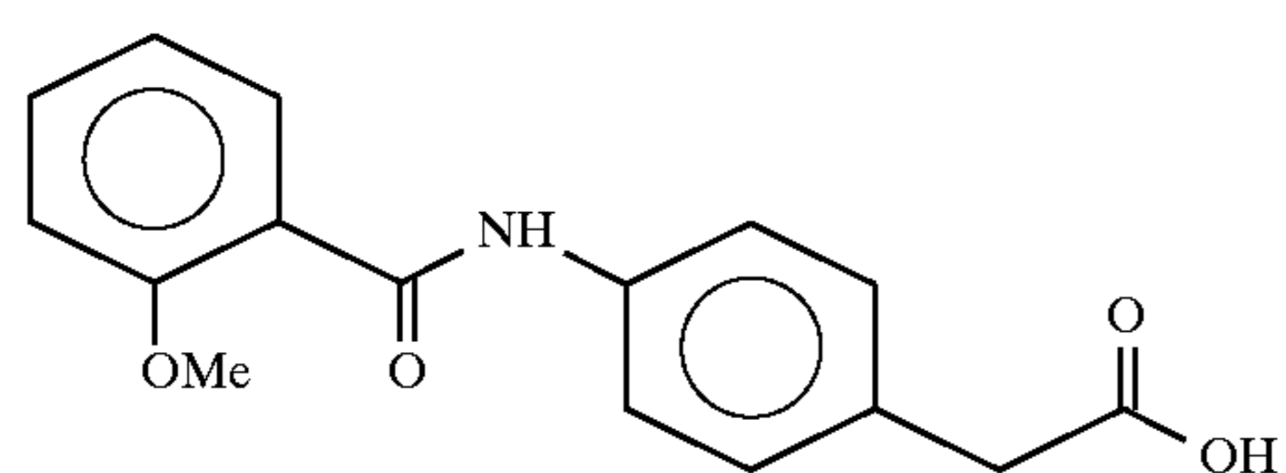
4-(o-anisoyl)aminophenylacetic acid
