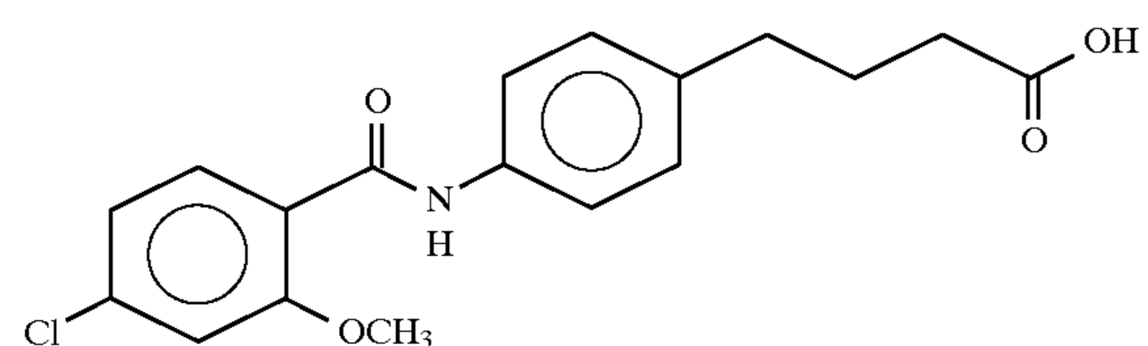
4-(4-(4-chloro-o-anisoyl)aminophenyl)butyric acid
