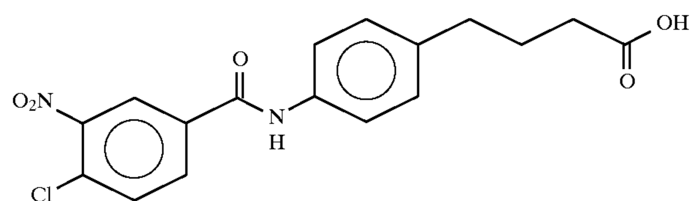
4-(4-(4-chloro-3-nitrobenzoyl)aminophenyl)butyric acid
