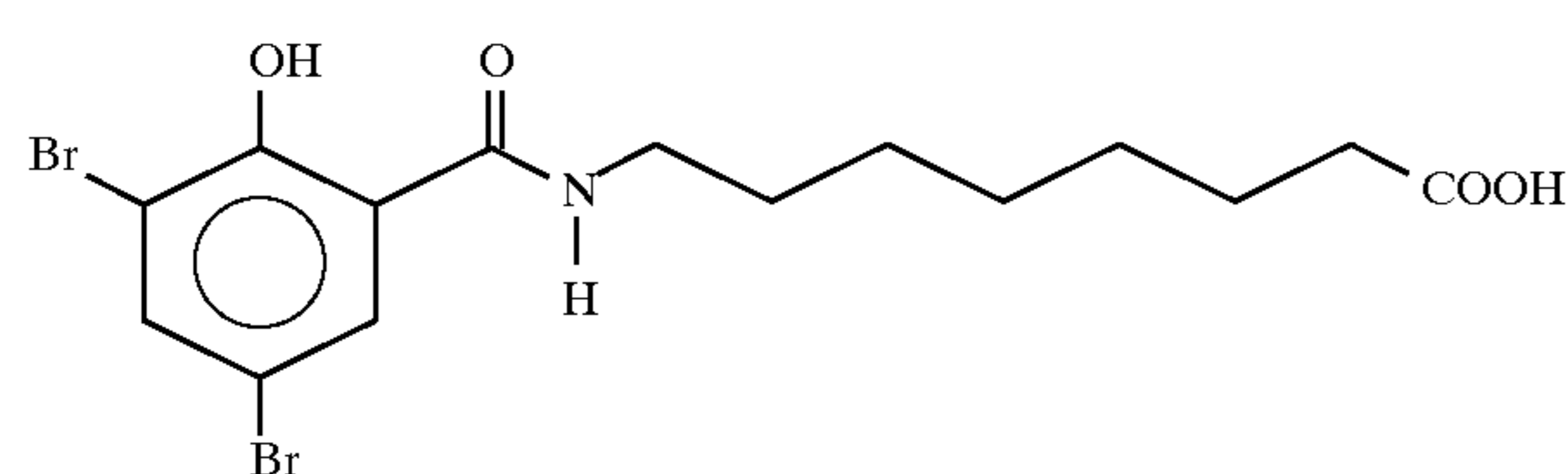
8-[N-(2-acetoxy-3,5-dibromobenzoyl)]aminocaprylic acid
