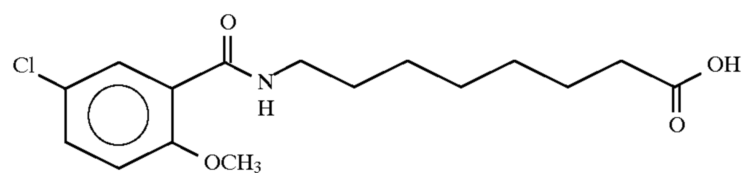
8-(5-chloro-o-anisoyl)aminocaprylic acid
