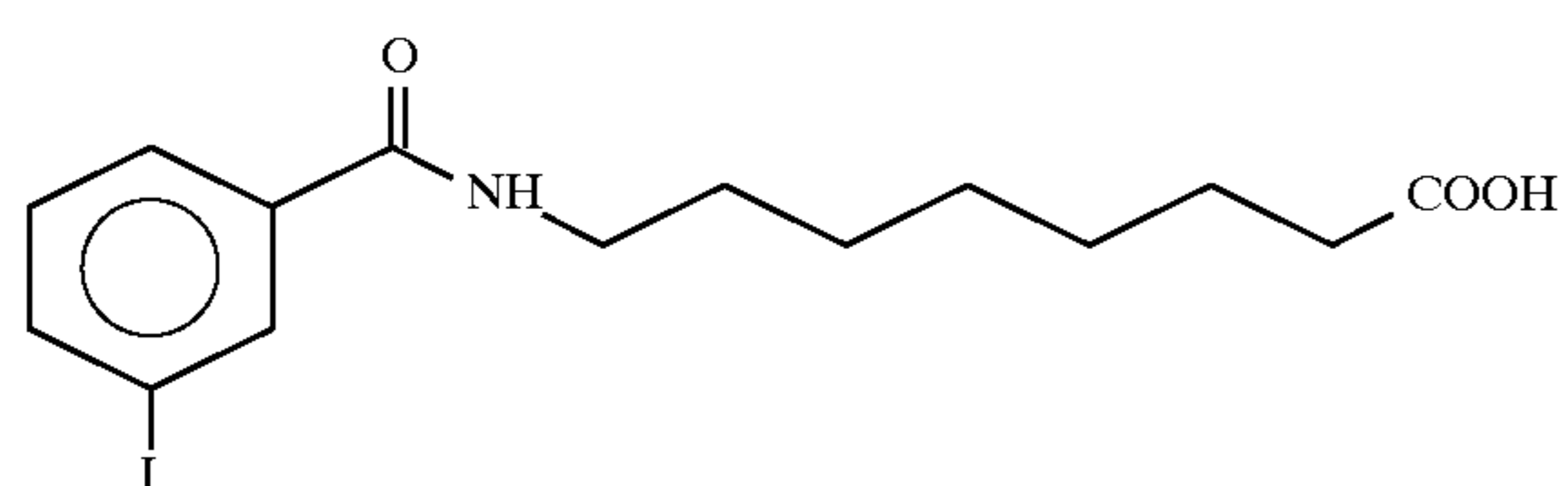
8-N-(3-iodobenzoyl)aminocaprylic acid
