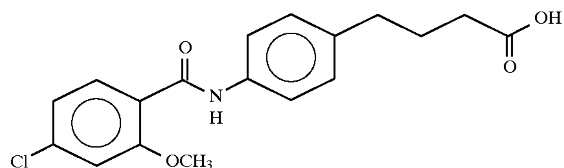
4-(4-(4-chloro-o-anisoyl)aminophenyl)butyric acid
