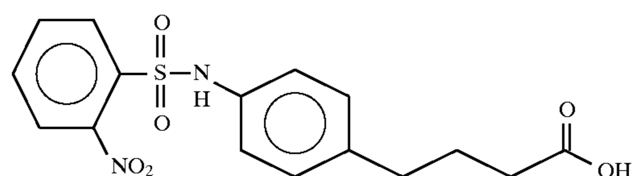
4-(4-(2-nitrobenzenesulfonyl)aminophenyl)butyric acid
