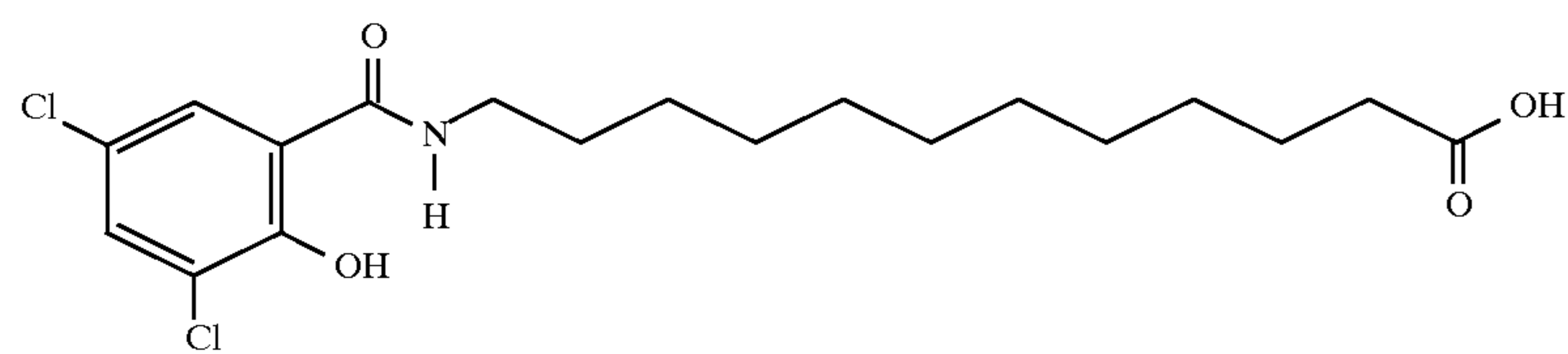
12-N0(3,5-dichloro-2-hydroxybenzoyl)aminododecanoic acid
