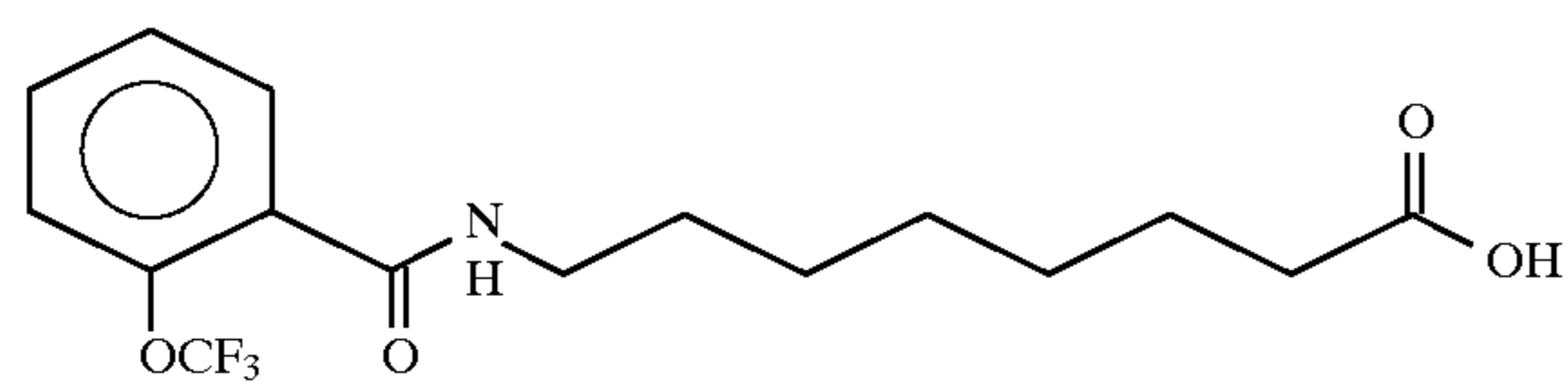
8-(2-(trifluoromethoxy)benzoyl)aminocaprylic acid
