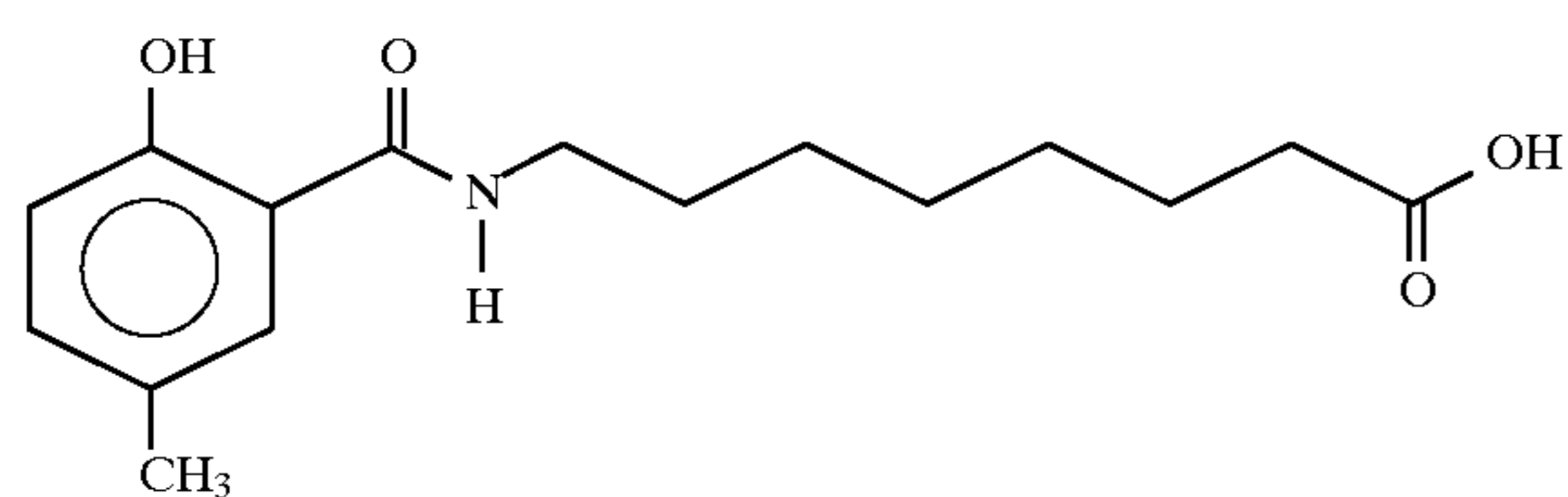
8-(N-5-methylsalicyloyl)aminocaprylic acid
