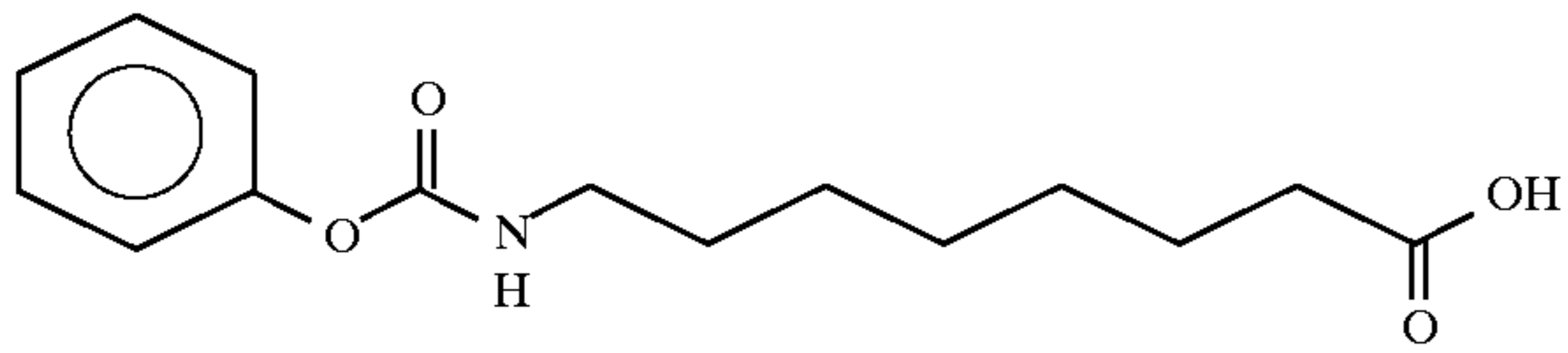
8-(phenylcarbonylamino)caprylic acid
