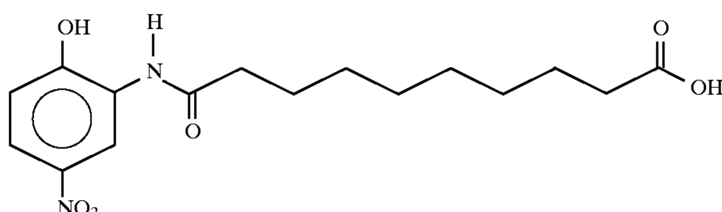
N-10-(2-hydroxy-5-nitroanilino)decanoic acid
