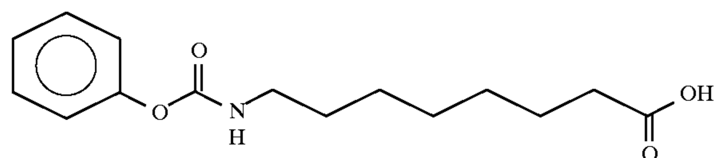
8-(phenylcarbonylamino)caprylic acid
