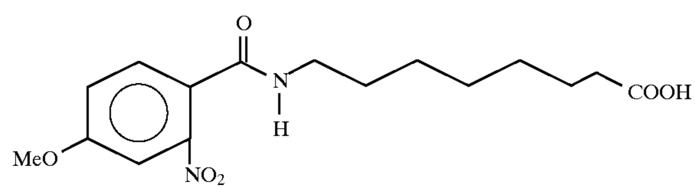
8-N-(4-methoxy-3-nitrobenzoyl)aminocaprylic acid
