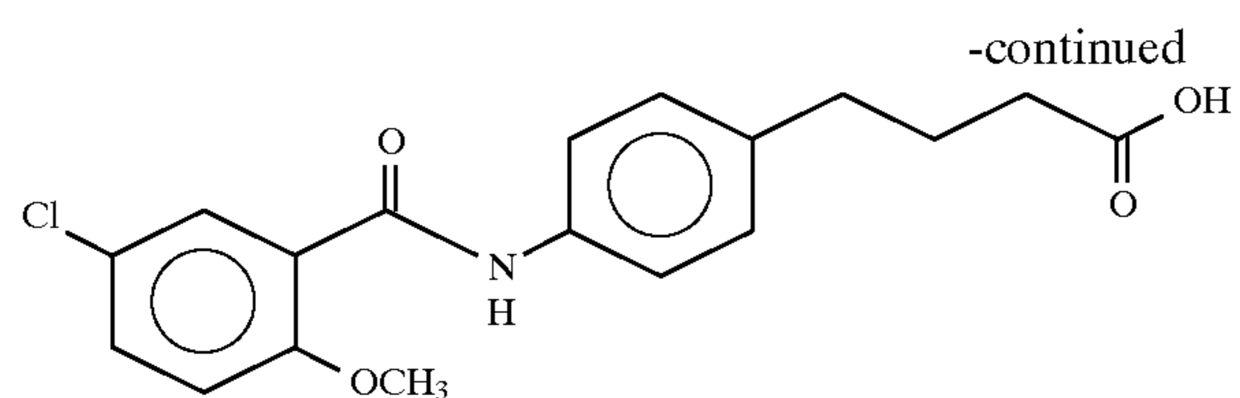
4-(4-(5-chloro-o-anisoyl)aminophenyl)butyric acid
