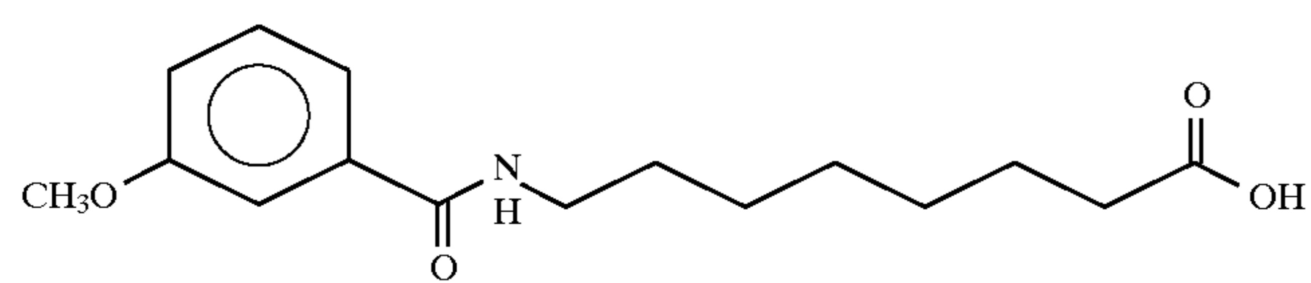
8-(3-anisoyl)aminocaprylic acid
