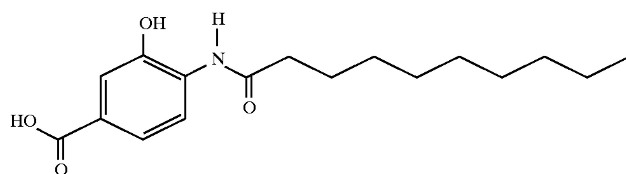
4-octanoylamino-3-hydroxybenzoic acid
