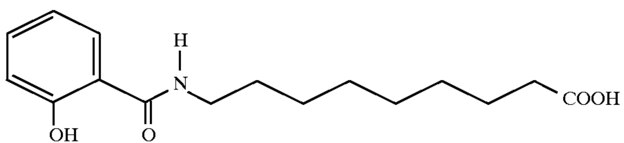
9-Salicyloylaminononanoic acid
