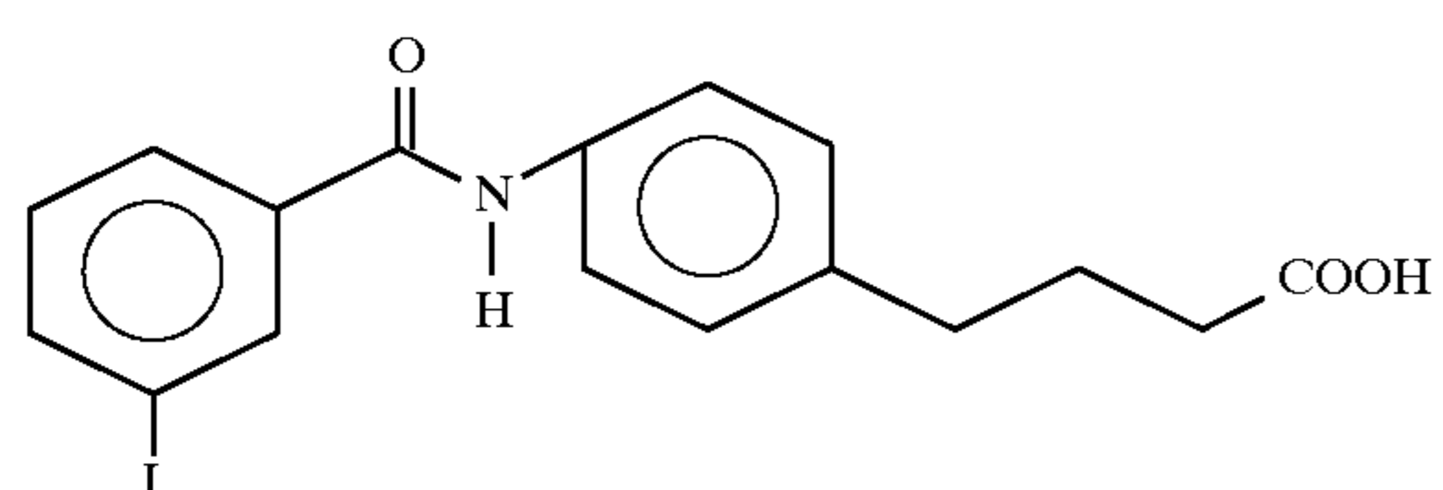
4-[N-[4-(3-iodobenzoyl)aminophenyl]]butyric acid
