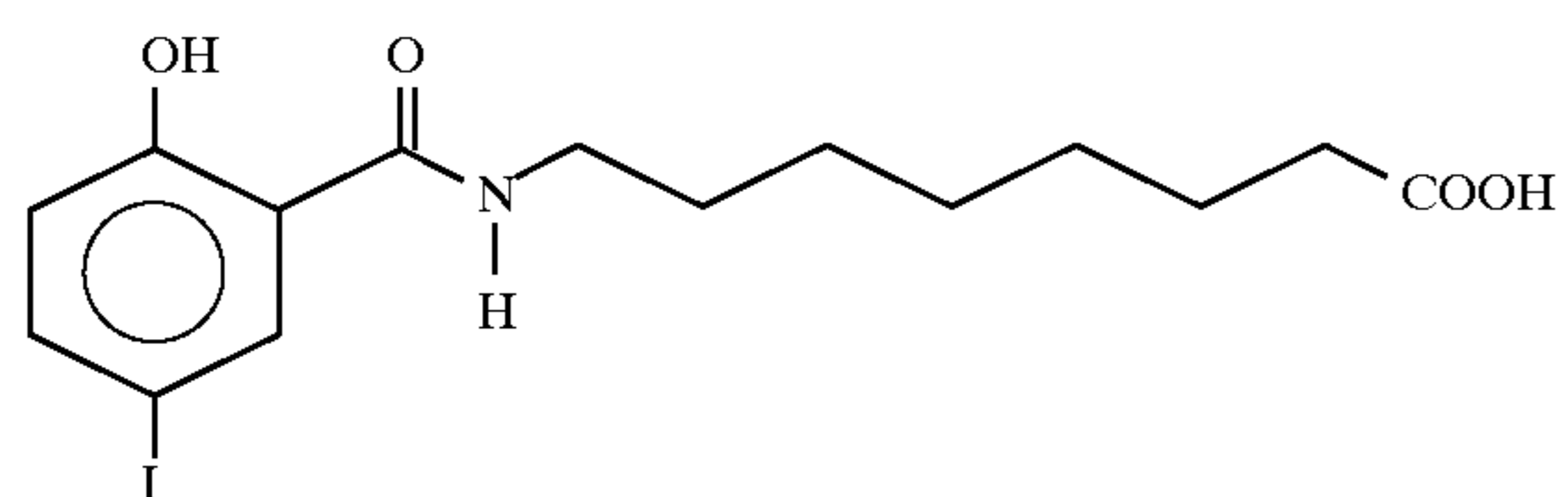
8-(N-2-hydroxy-5-iodobenzoyl)aminocaprylic acid
