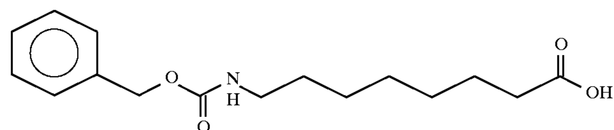
8-Benzylcarbonylamino)caprylic acid
