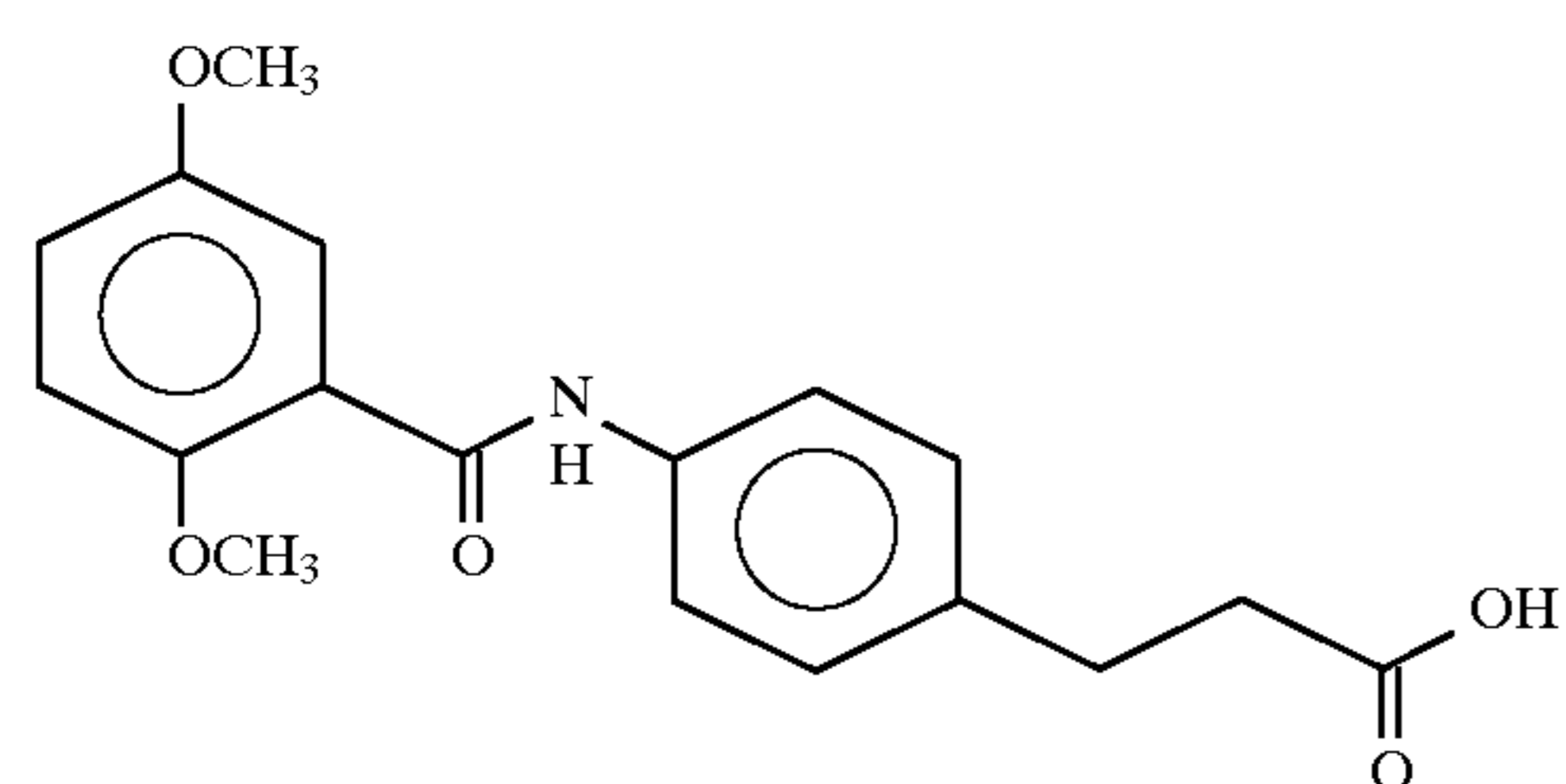
3-(4-(2,5-dimethoxybenzoyl)aminophenyl)propionic acid
