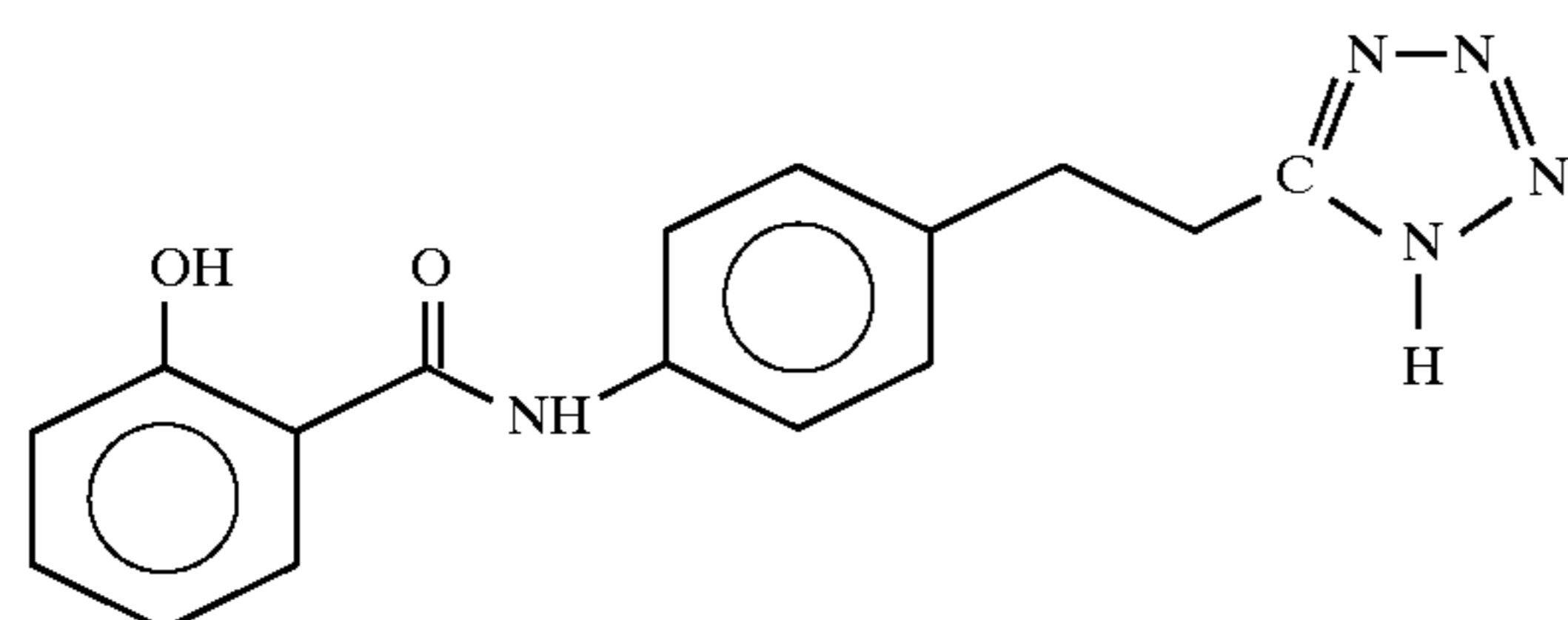
4-(Salicyloyl)aminophenylethyltetrazole
