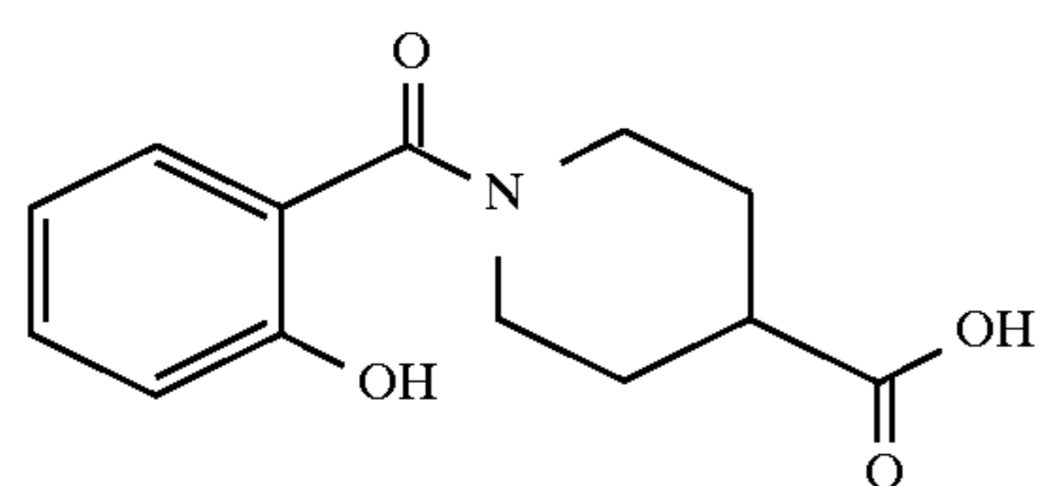
N-(2-hydroxybenzoyl)isonipecotic acid
