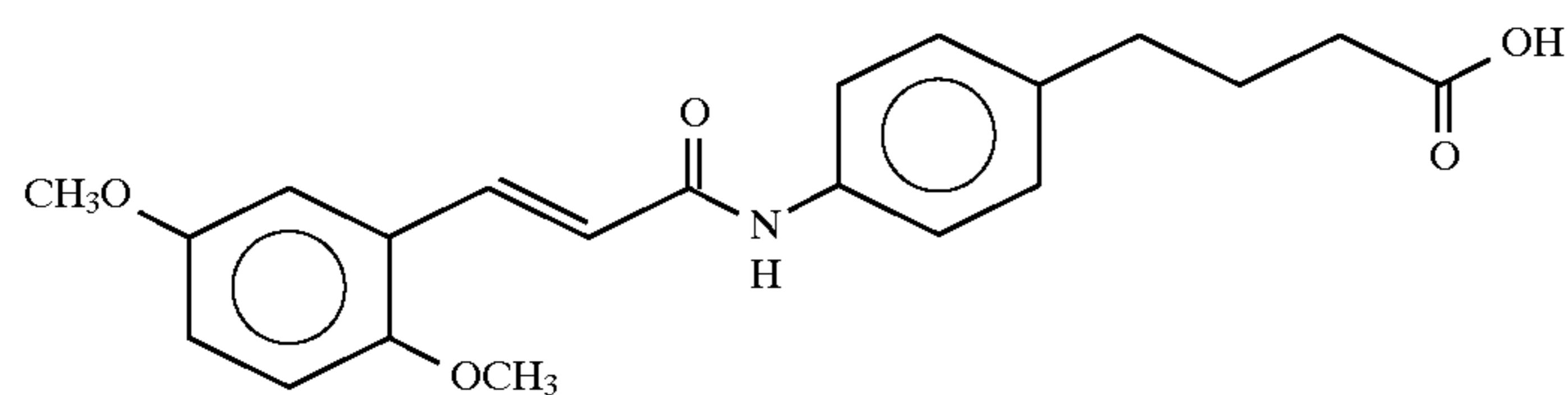
4-(4-(2,5-dimethoxycinnamoyl)aminophenyl)butyric acid
