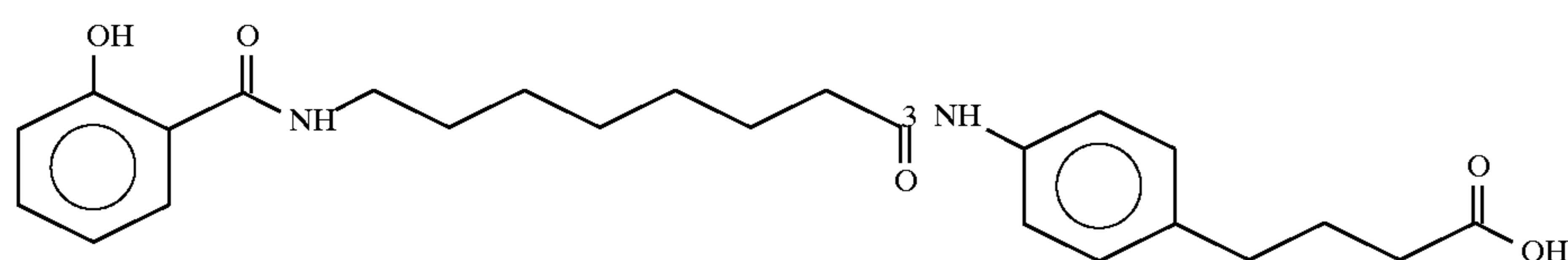
4-(4-(N-8(N-Salicyloyl)aminocaprylic)aminophenyl)butyric acid
