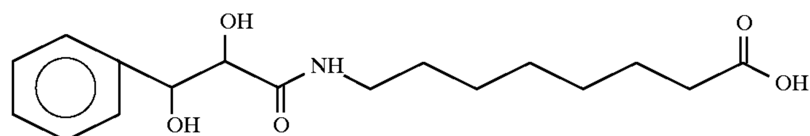
(3-phenyl-2,3-dihydroxypropanoyl)8aminocaprylic acid
