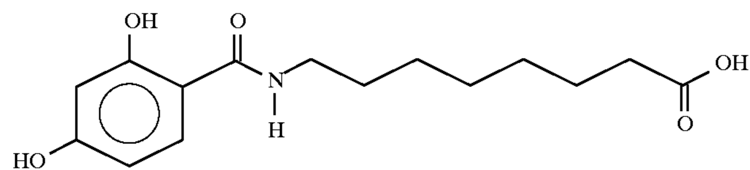
8-(N-(2,4-Dihydroxybenzoyl)]aminocaproic acid
