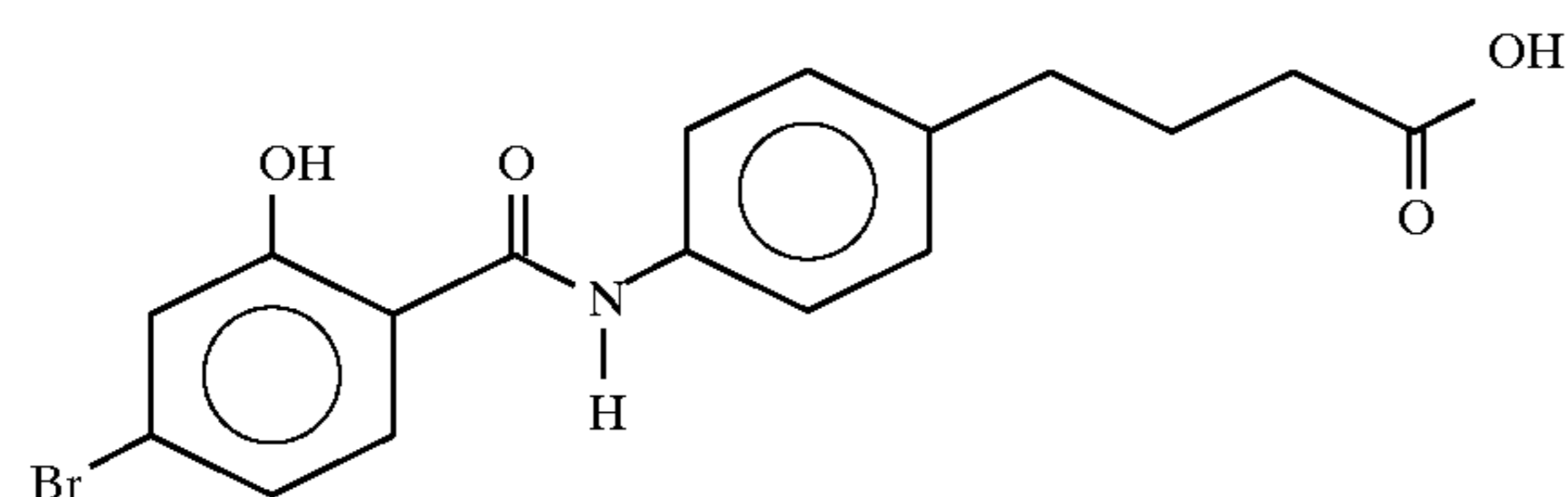
4-[N-(2-hydroxy-4-bromobenzoyl)aminophenyl]butyric acid
