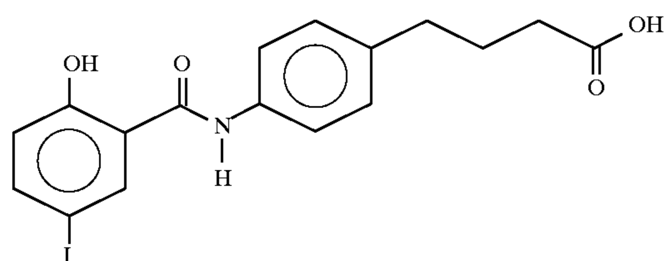
4-{[N-(2-hydroxy-5-iodobenzoyl)]aminophenyl}butyric acid
