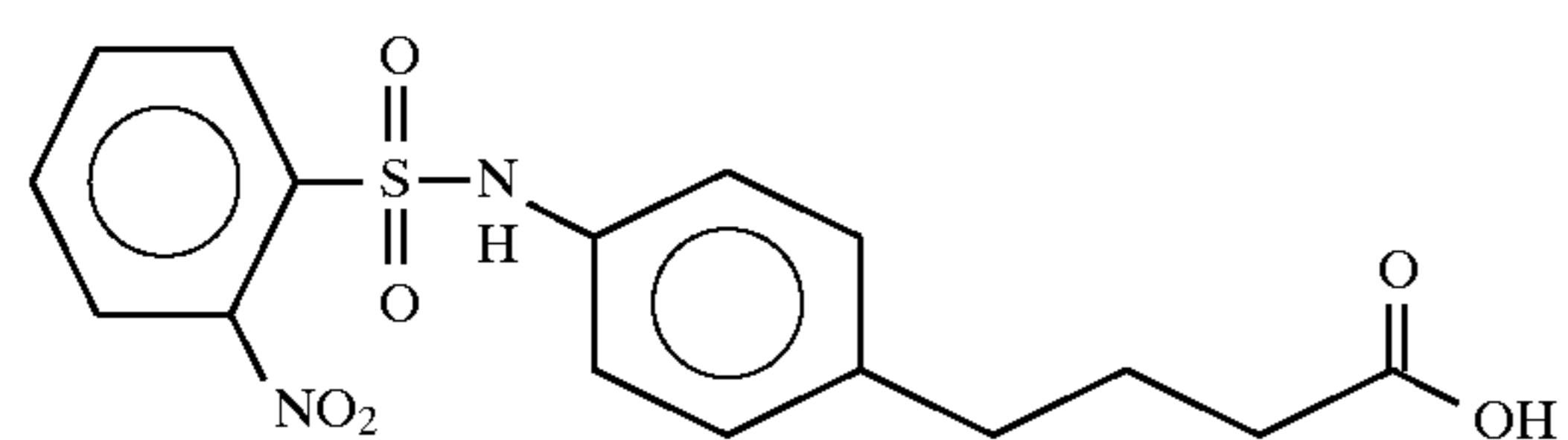
4-(4-(2-nitrobenzenesulfonyl)aminophenyl)butyric acid
