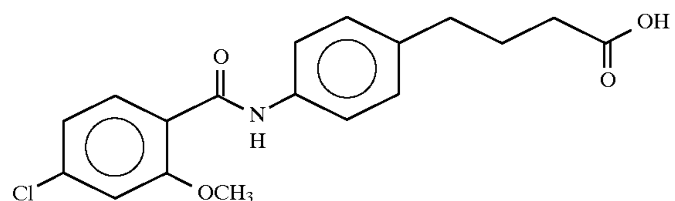
4-(4-(4-chloro-o-anisoyl)aminophenyl)butyric acid
