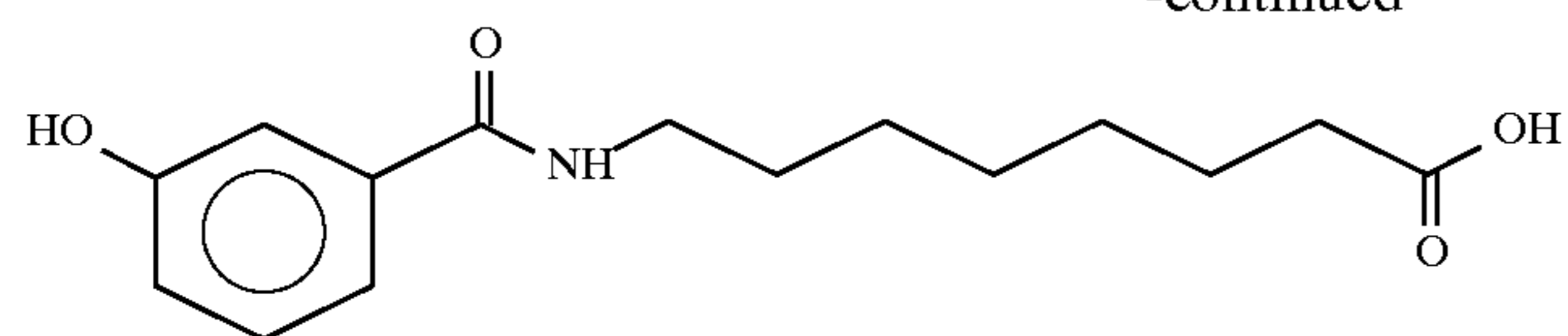
8-(2-Hydroxybenzoyl)aminocaprylic acid
