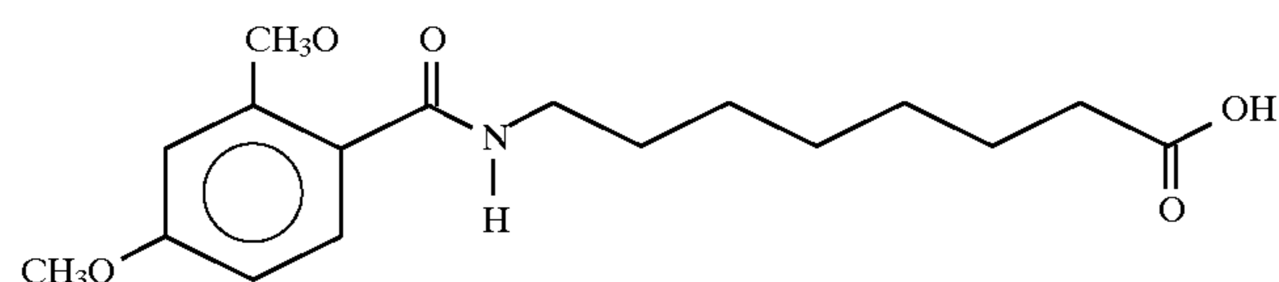
8-(N-(2,4-Dihydroxybenzoyl)]aminocaproic acid
