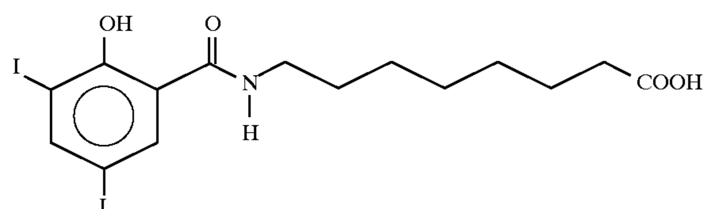
8-(N-(2-hydroxy-3,5-diiodobenzoyl)aminocaprylic acid
