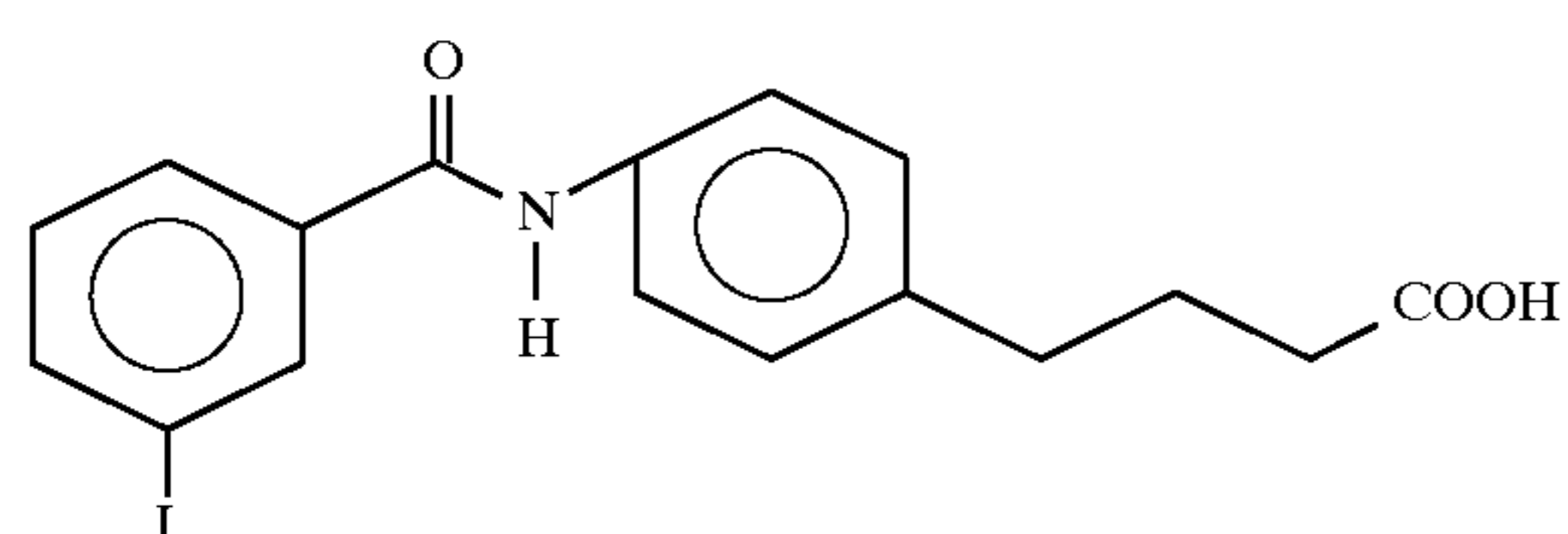
4-[N-[4-(3-iodobenzoyl)aminophenyl]]butyric acid
