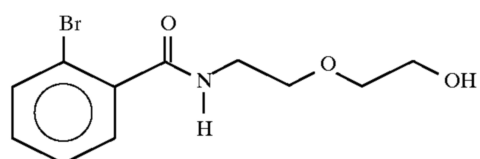
2-[N-(2-bromobenzoyl)aminoethoxy]ethanol
