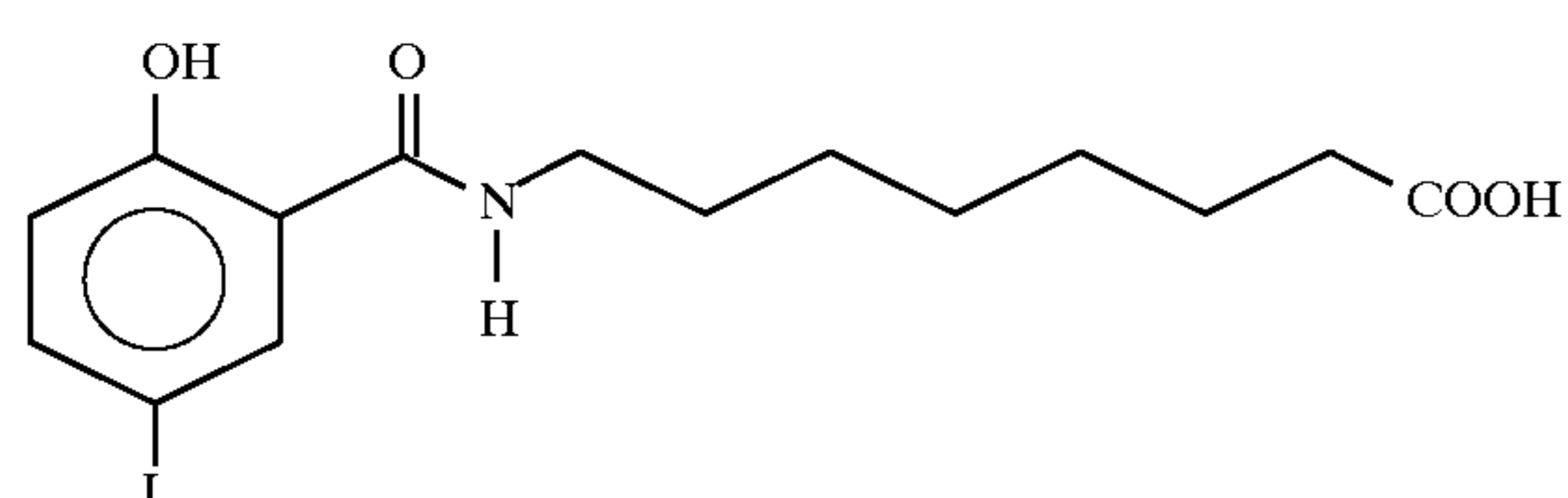
8-(N-2-hydroxy-5-iodobenzoyl)aminocaprylic acid
