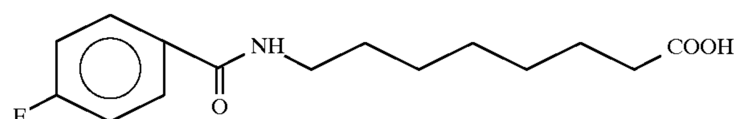
8-[N-(4-fluorobenzoyl)]aminocaprylic acid
