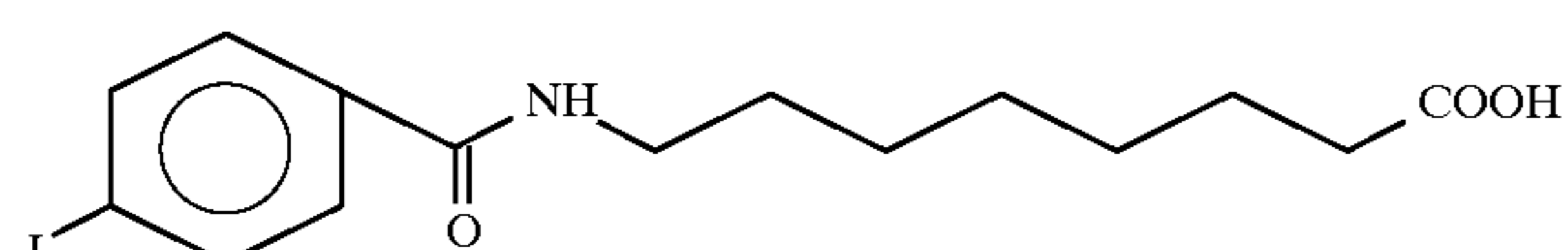
8-[N-(4-iodobenzoyl)]aminocaprylic acid
