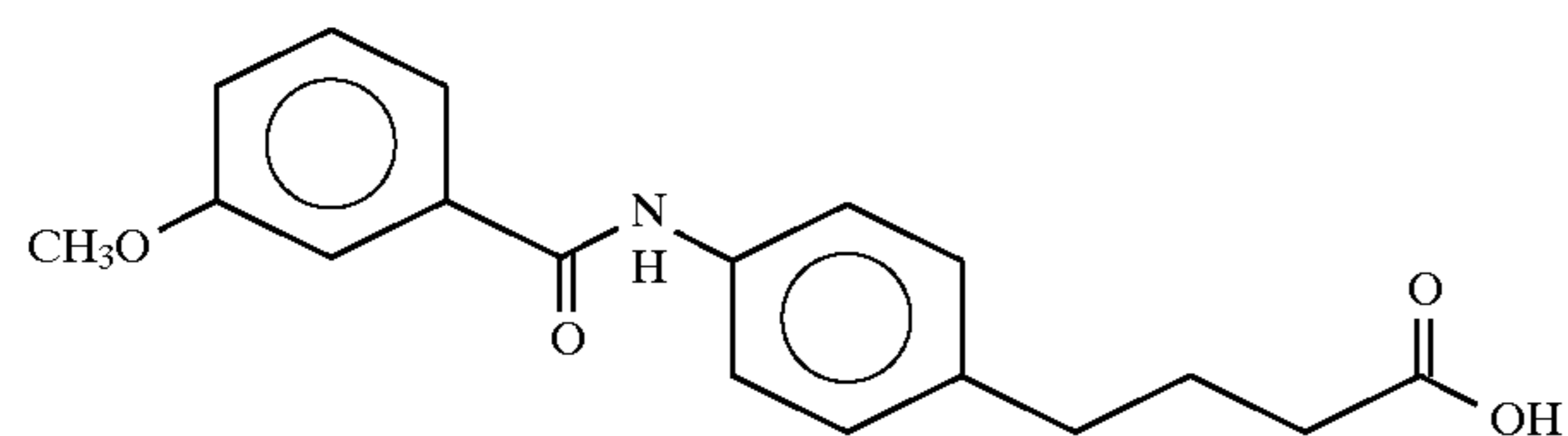
4-(4-(3-anisoyl)aminophenyl)butyric acid
