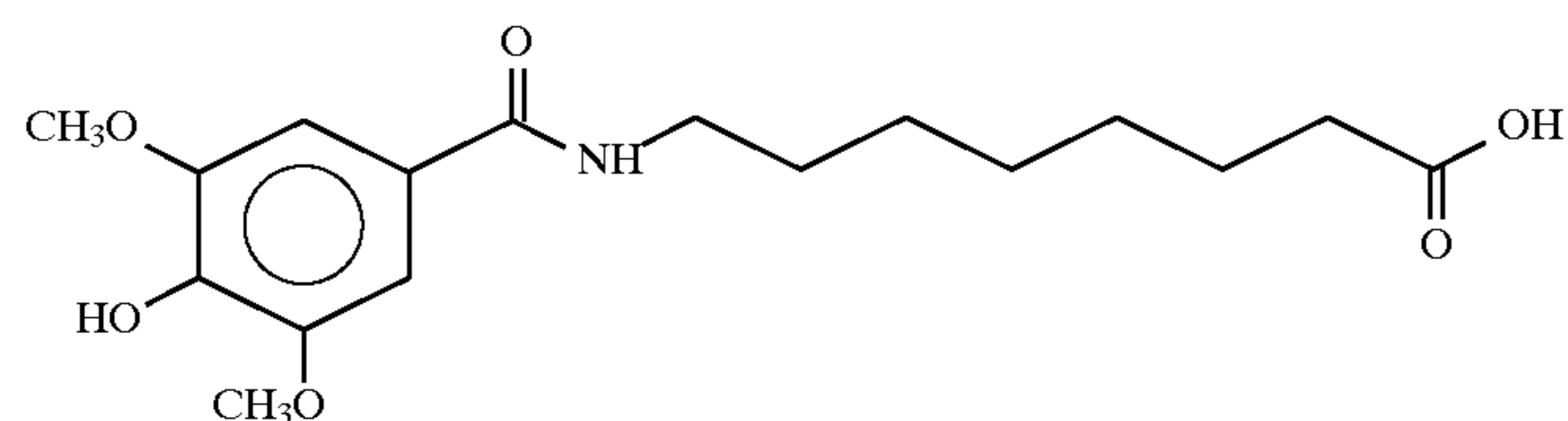
8-(N-3,5-Dimethoxy-4-hydroxybenzoyl)aminocaprylic acid
