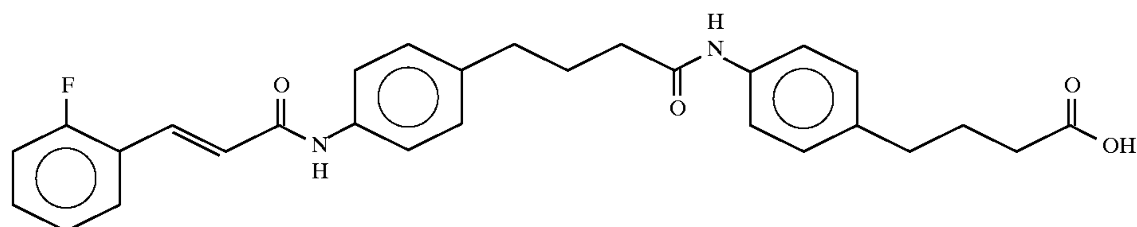
4-(4-(N-(2-Fluorocinnamoyl)aminophenyl) butyric
