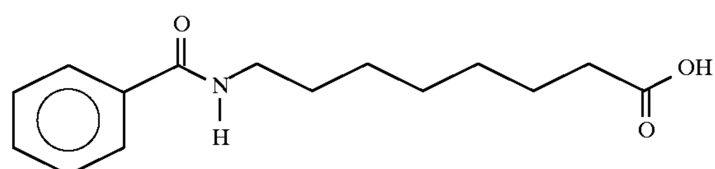
8-(N-benzoyl)aminocaprylic acid
