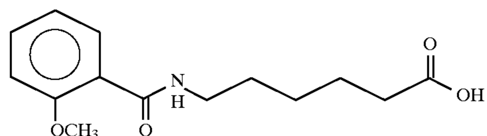
6-(anisoyl)aminocaproic acid
