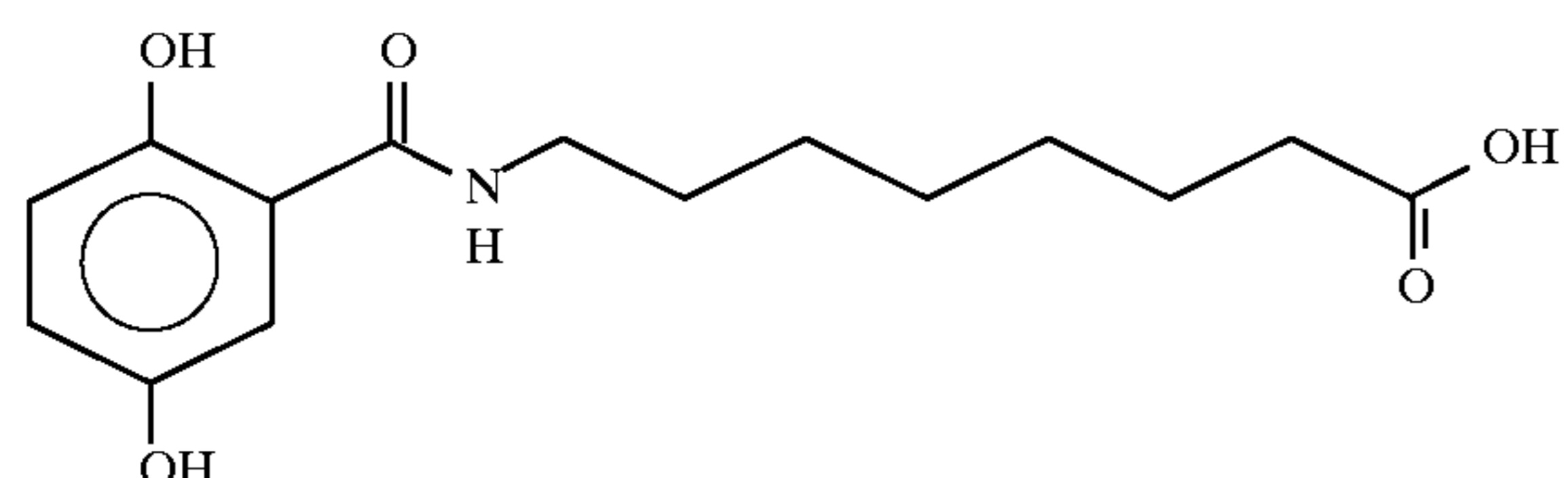
8-(N-(2,5-Dihydroxybenzoyl)]aminocaproic acid
