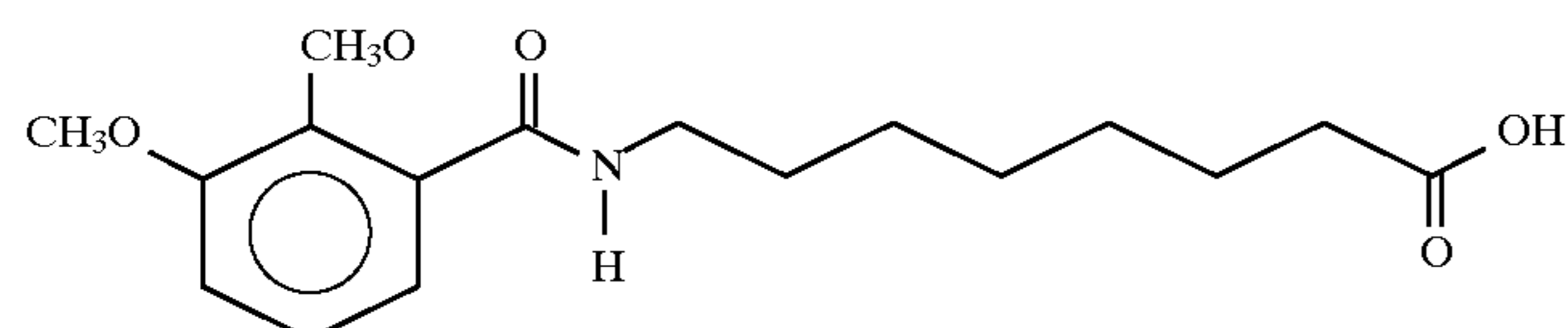
8-(N-(2,3-Dimethoxybenzoyl)]aminocaproic acid
