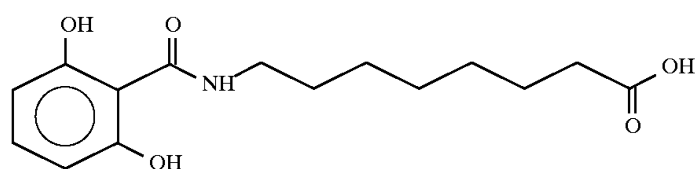
8-(N-2,6-Dihydroxybenzoyl)aminocaprylic acid
