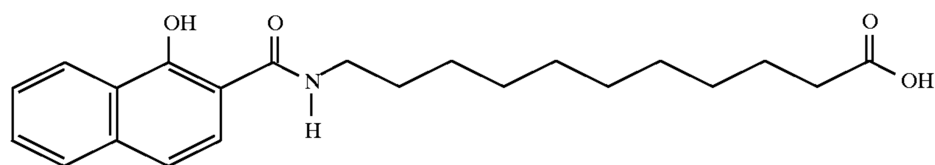
11-N-(1-hydroxy-2-naphthoyl)aminoundecanoic acid
