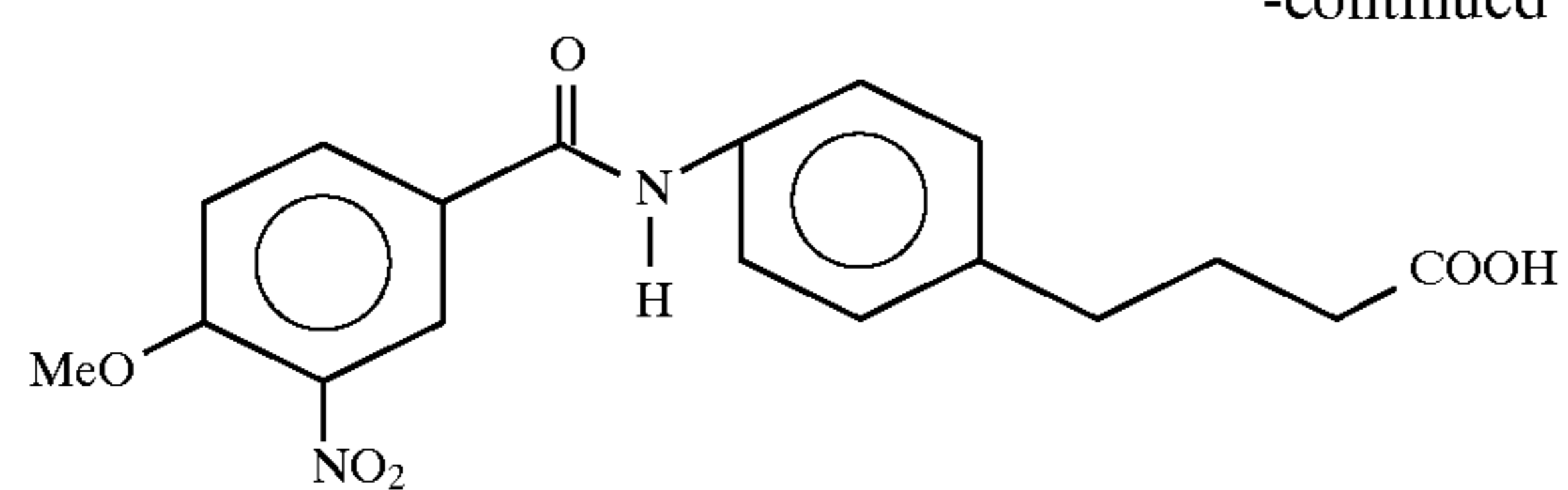
4-[4-N-(4-methoxy-3-nitrobenzoyl)aminophenyl]butyric acid
