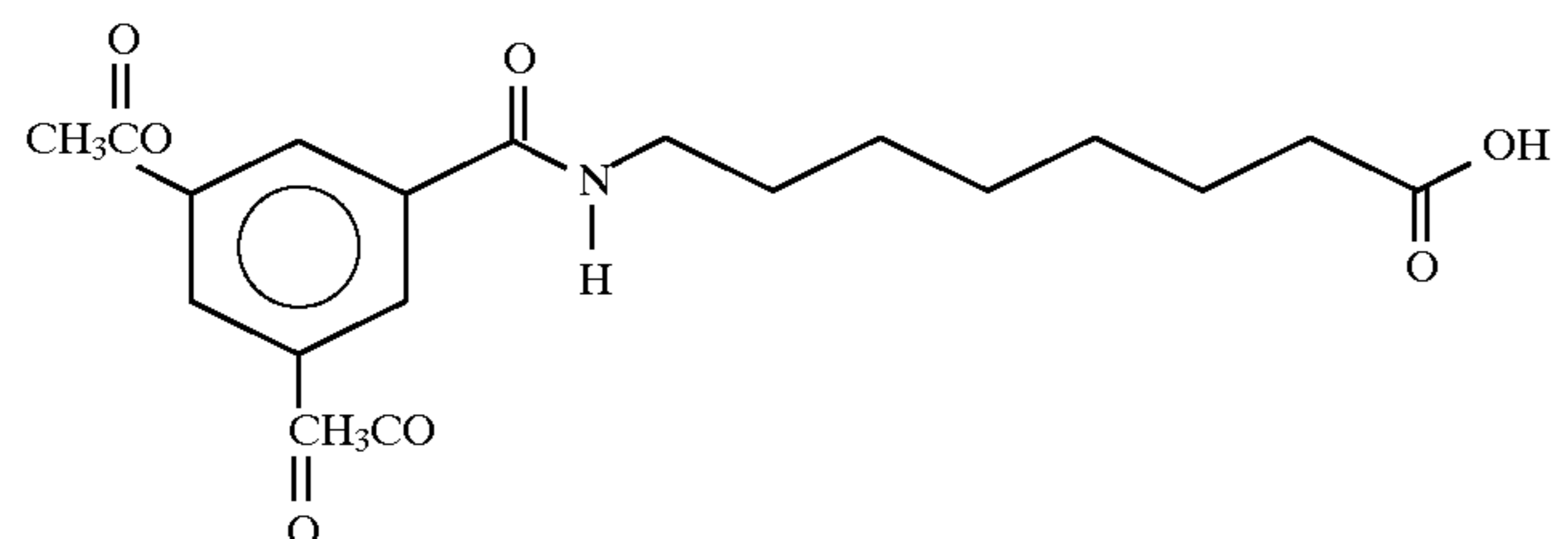
8-(N-(3,5-Diacetyloxybenzoyl))aminocaprylic acid
