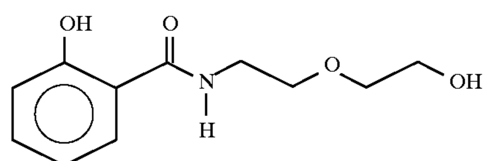
2-[N-(2-hydroxybenzoylamino)ethoxy]ethanol
