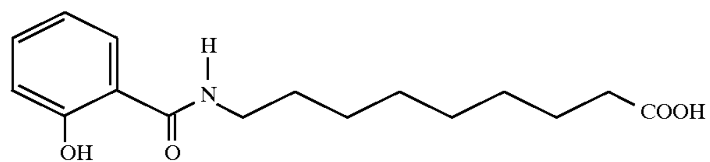
9-Salicyloylaminononanic acid
