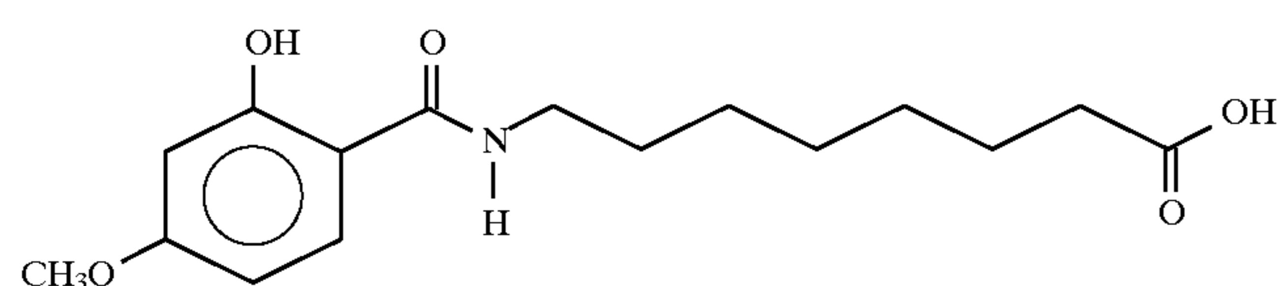
8-(N-2-Hydroxy-4-methoxybenzoyl)aminocaprylic acid
