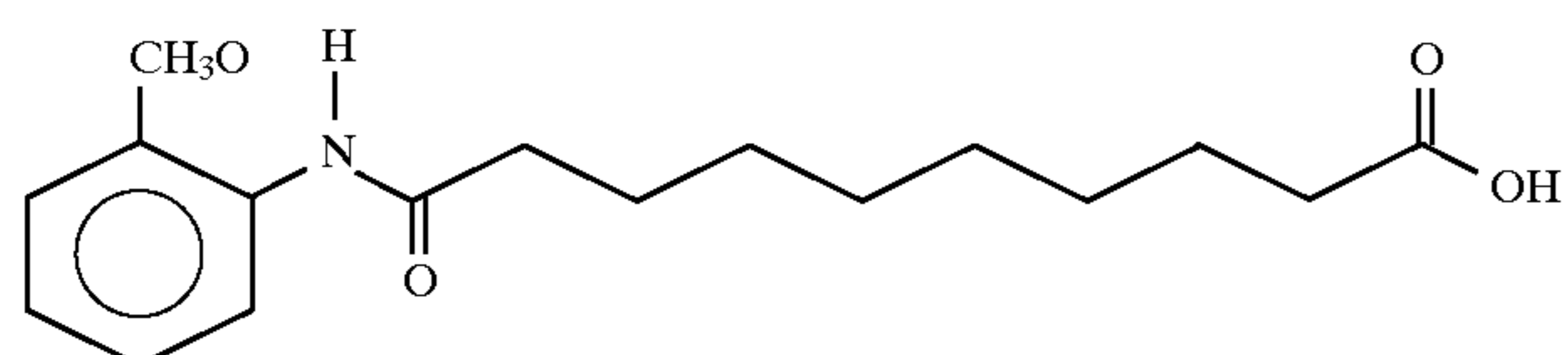
10-(N-(2-Methoxyanilino))sebacic acid
