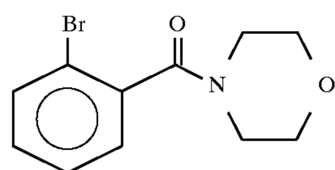
N-(2-bromobenzoyl)morpholine
