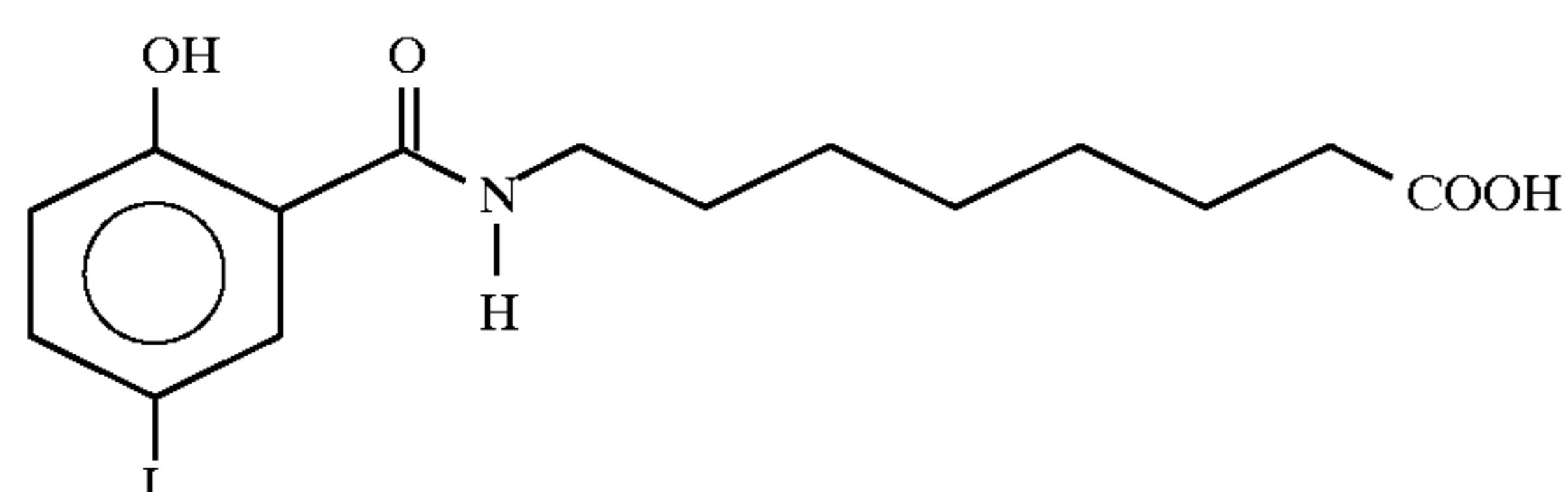
8-(N-2-hydroxy-5-iodobenzoyl)aminocaprylic acid
