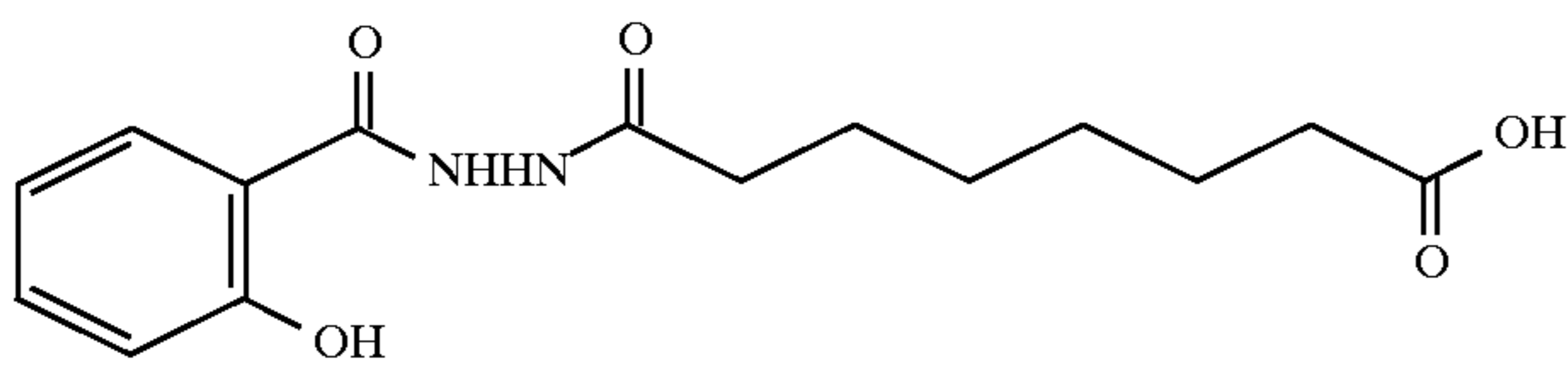
1-salicyloyl-2-suberyl hydrazide
