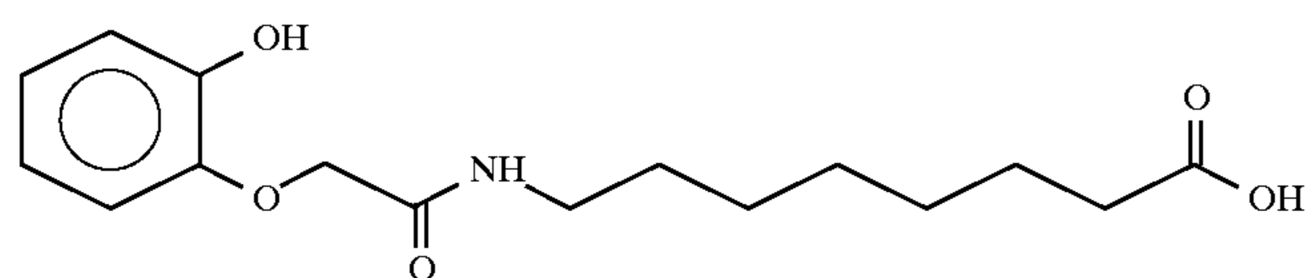
7-(2-hydroxyphenoxyacetyl)aminocaproic acid
