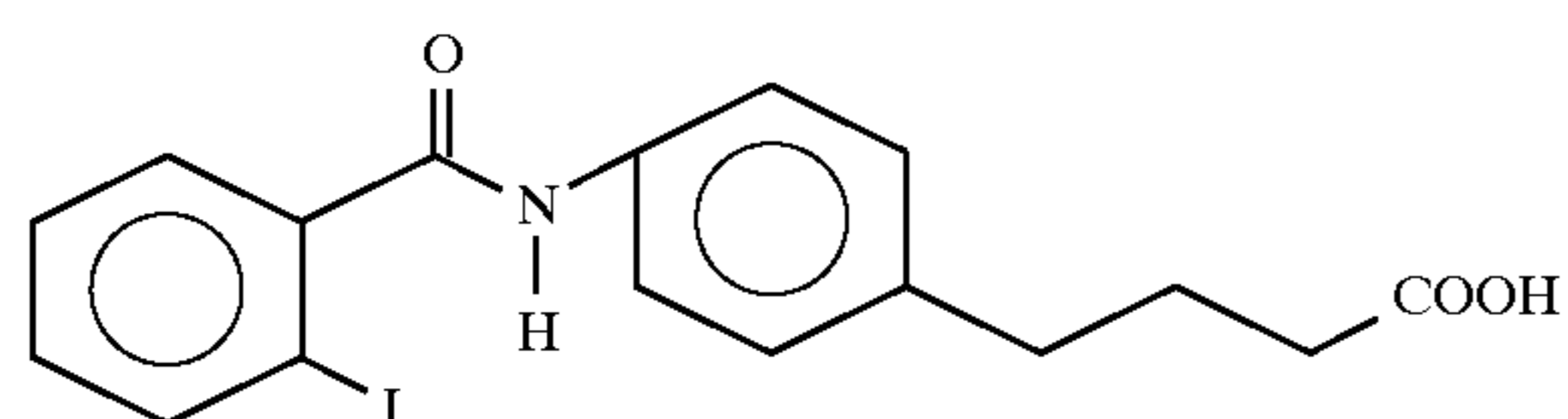
4-{4-[N-(2-iodobenzoyl)aminophenyl]}butyric acid
