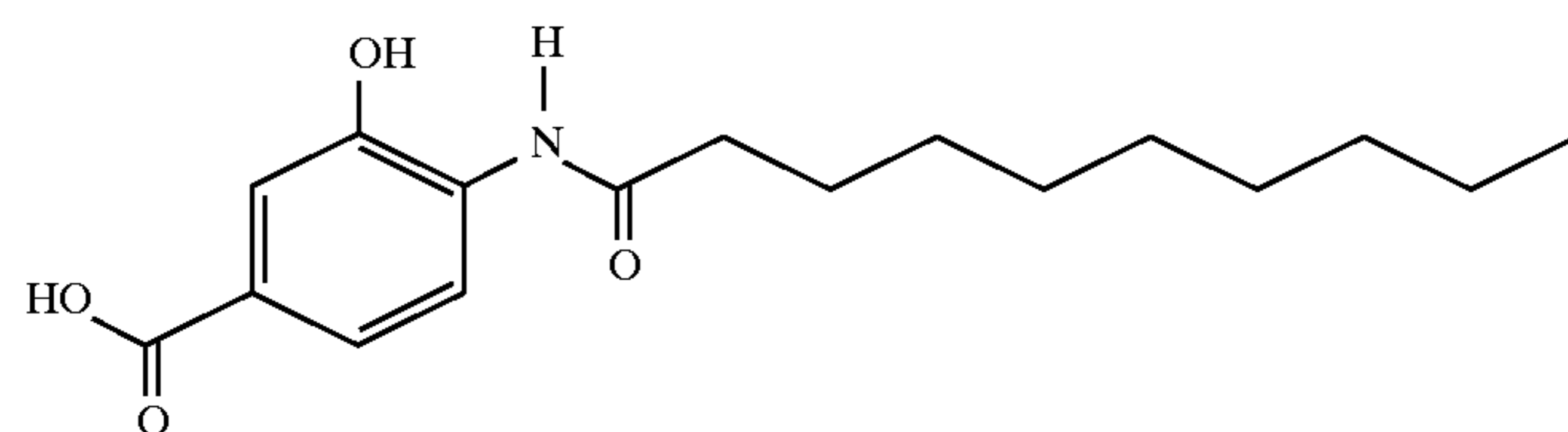
4-octanoylamino-3-hydroxybenzoic acid
