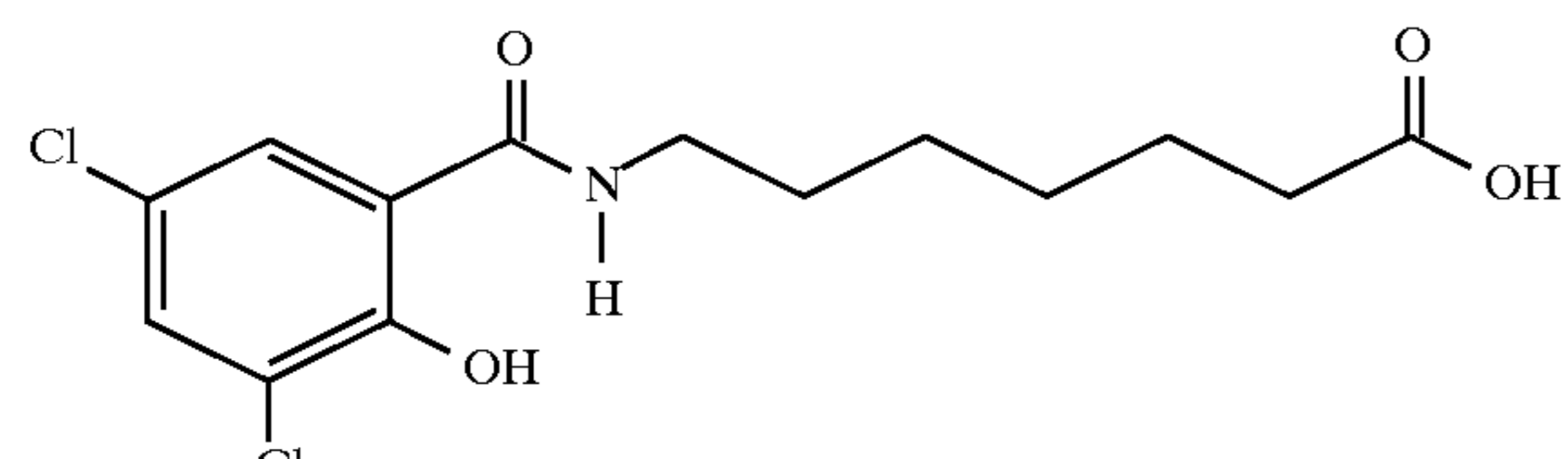
7-N-(3,5-dichloro-2-hydroxybenzoyl)aminoheptanoic acid
