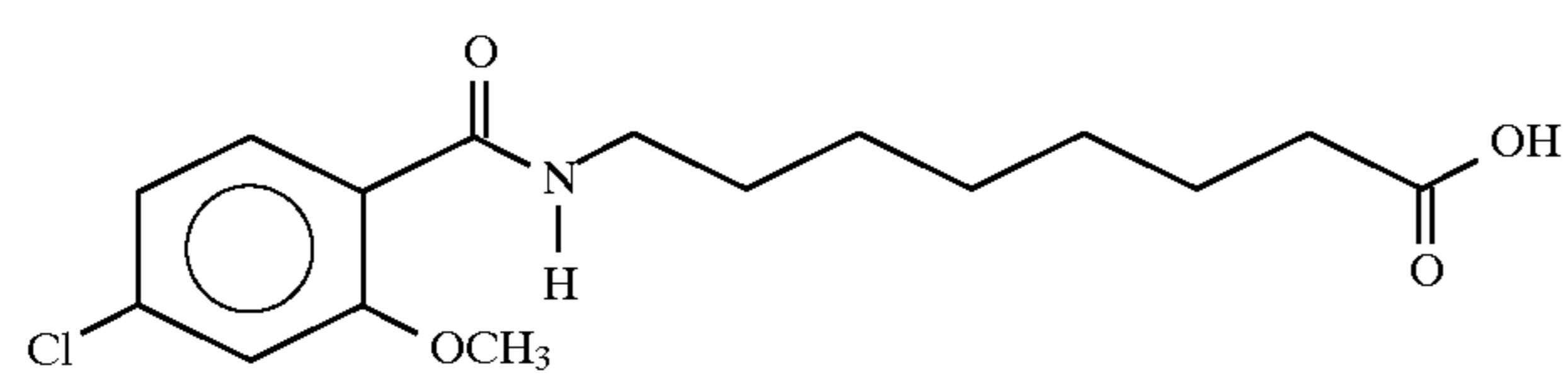
8-(4-chloro-o-anisoyl)aminocaprylic acid
