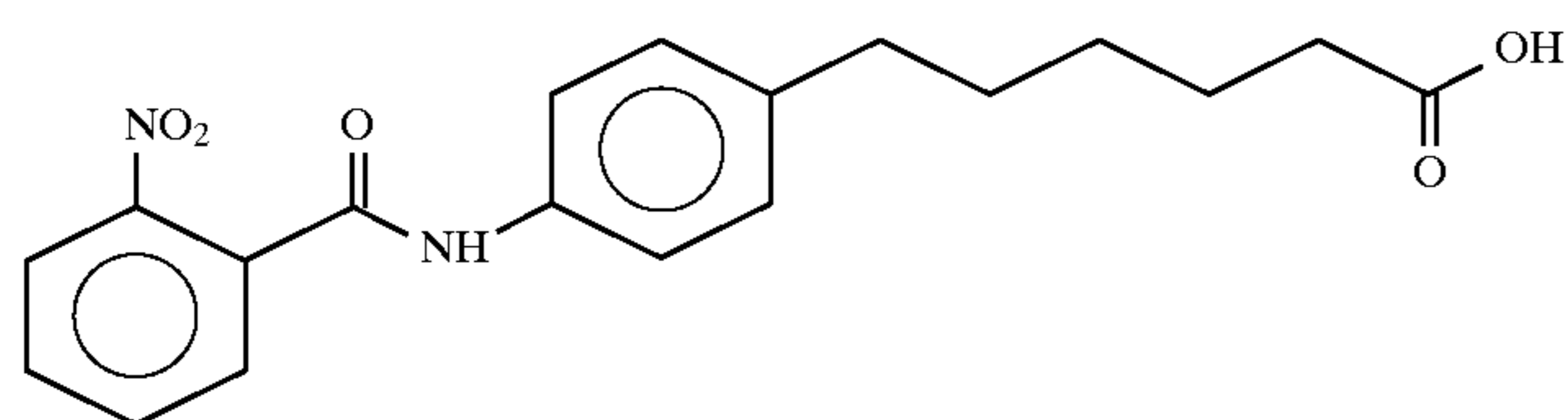
6-(4-(N-(2-Nitrobenzoyl)aminophenyl)hexanoic acid
