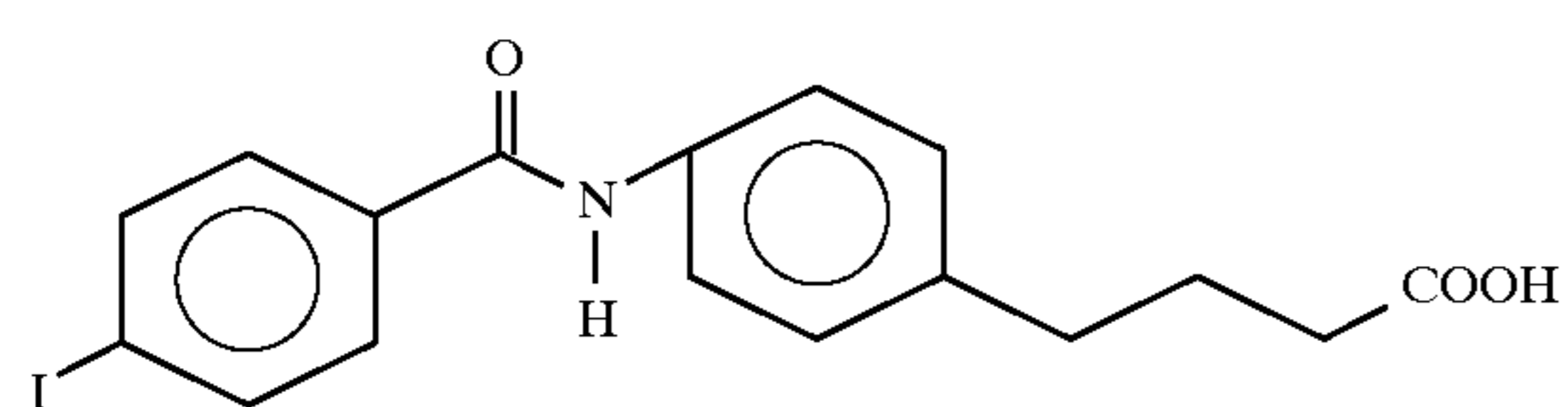
4-[4-[N-(4-iodobenzoyl)aminophenyl]butyric acid
