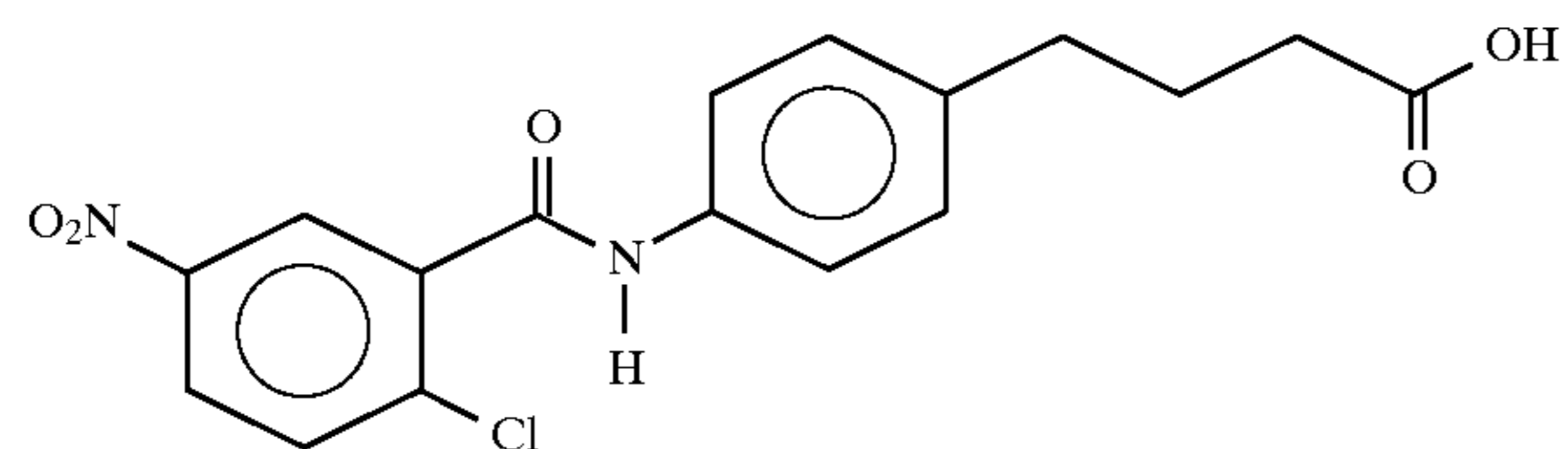
4-(4-(2-chloro-5-nitrobenzoyl)aminophenyl)butyric acid
