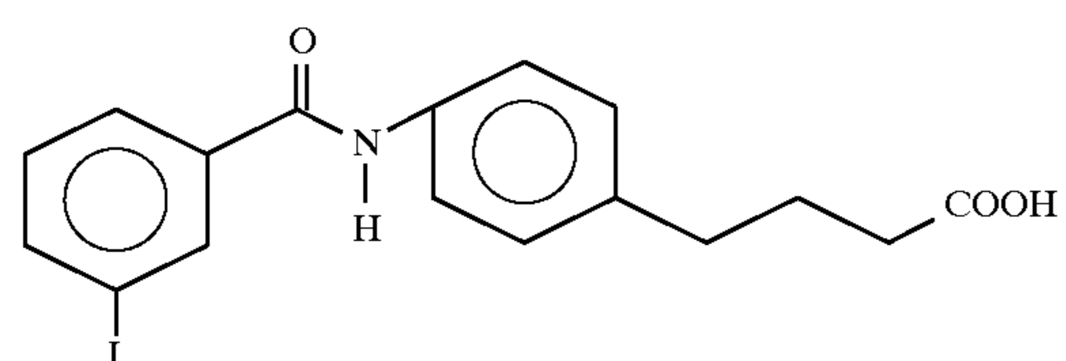
4-[N-[4-(3-iodobenzoyl)aminophenyl]]butyric acid
