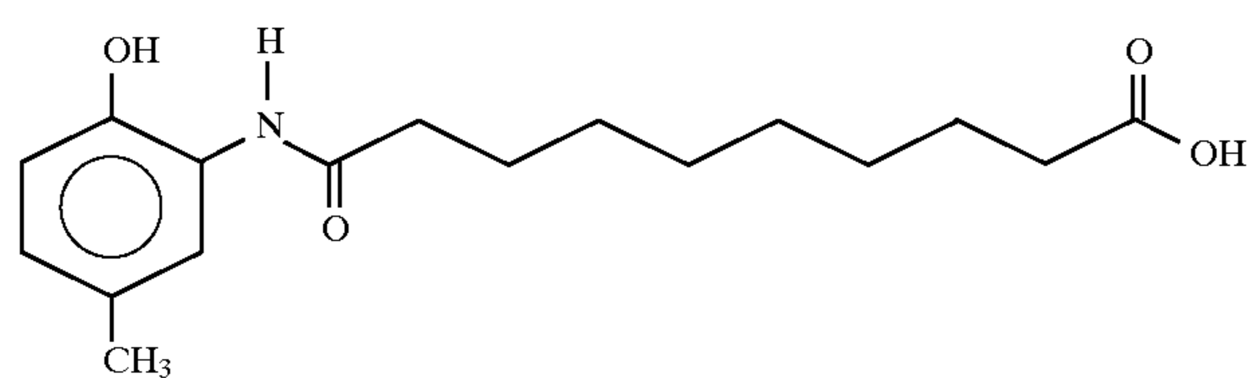
9-(2-hydroxy-5-methylanilino)nonanoic acid
