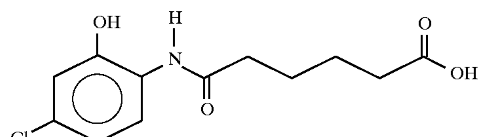
5-(4-chloro-2-hydroxyanilino)valeric acid
