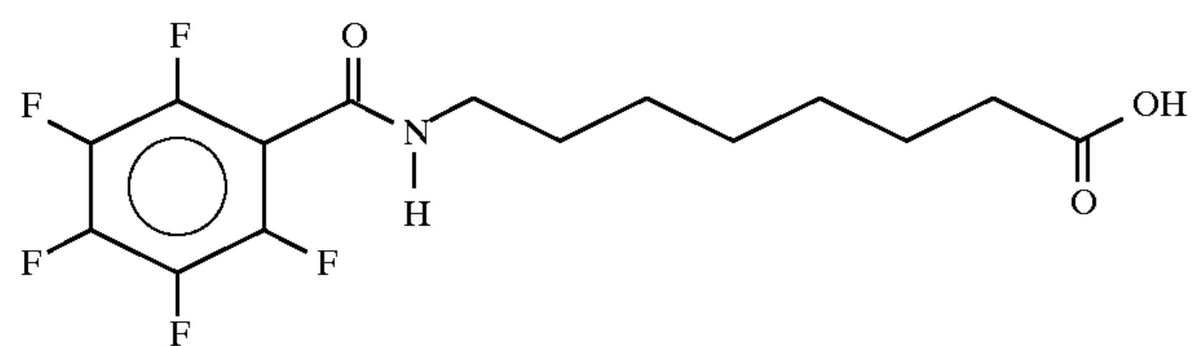
8-(pentafluorobenzoyl)aminocaproic acid
