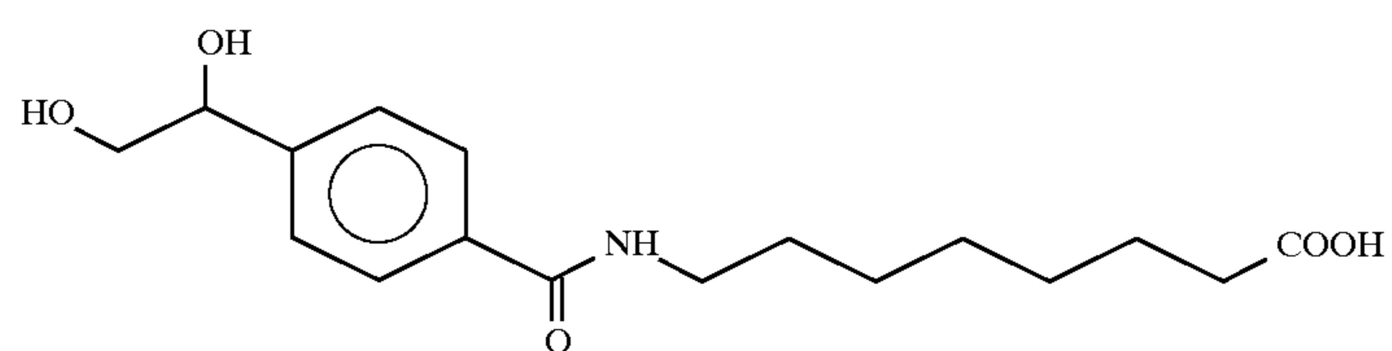
8(4-(1,2-dihydroxyethyl)benzoyl)aminocaprylic acid
