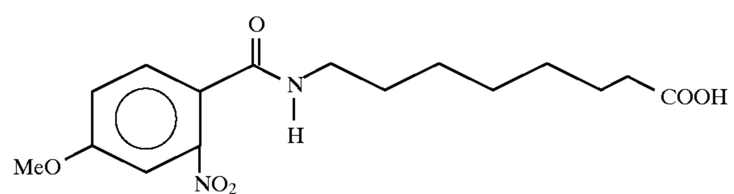
8-N-(4-methoxy-3-nitrobenzoyl)aminocaprylic acid
