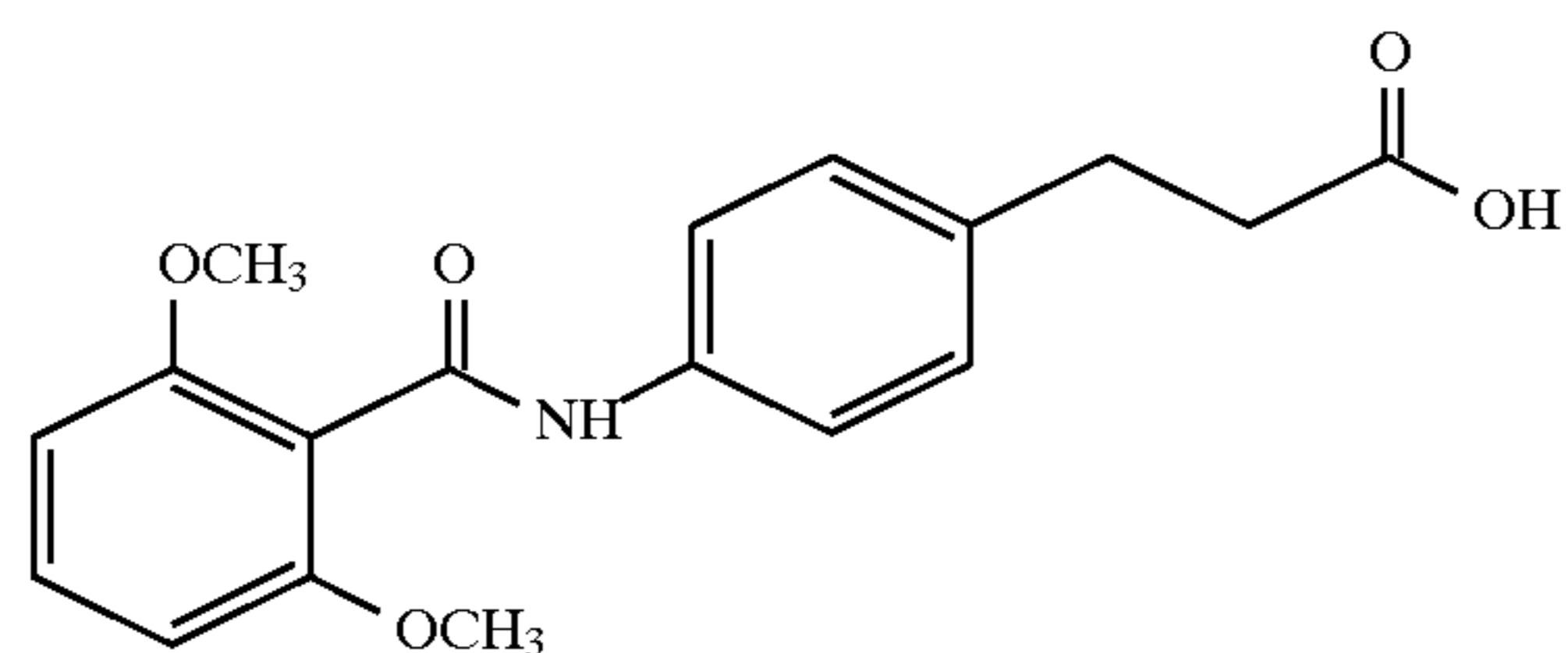
3-(4-(2,6-dimethoxybenzoyl)aminophenyl)propionic acid
