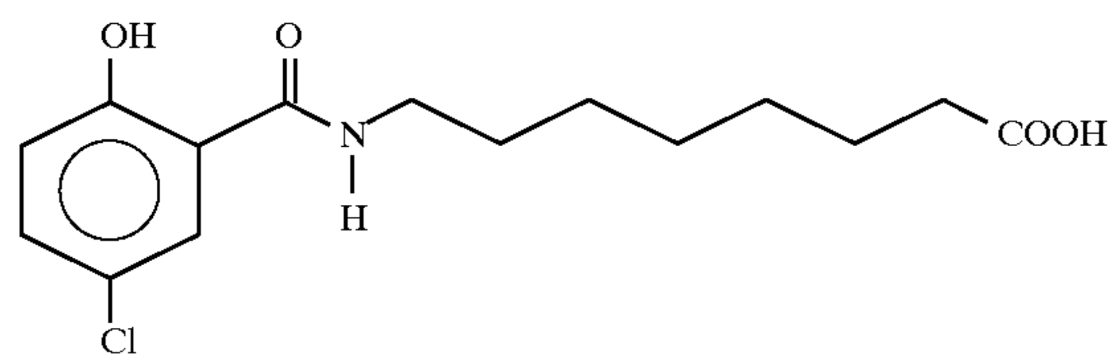
8-(N-2-hydroxy-5-chlorobenzoyl)aminocaprylic acid
