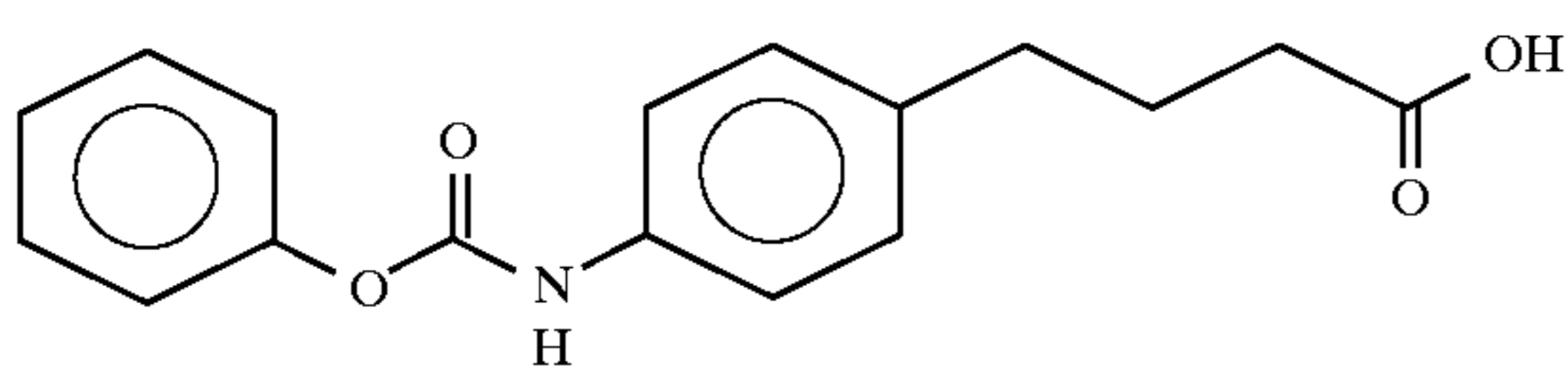
4-(4-phanyloxycarbonylamino)phenyl)butyric acid
