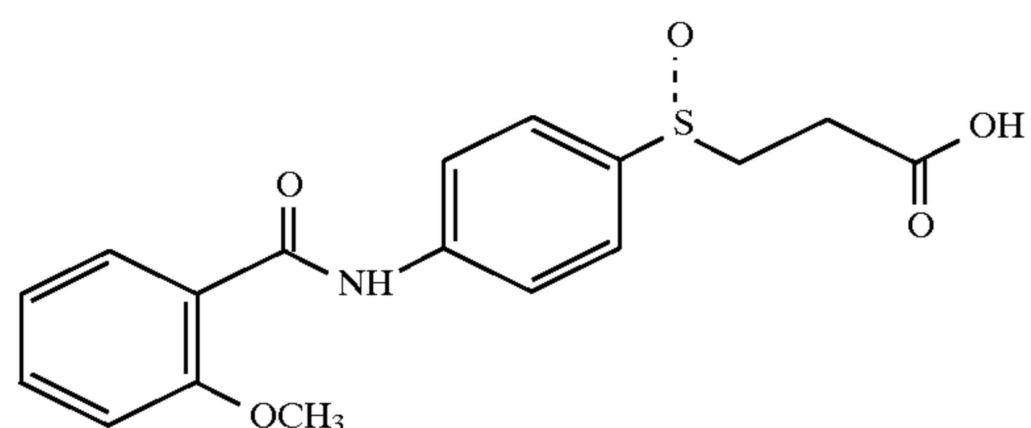
4-(2-methoxybenzoyl)amino 3-carboxylsulfoxide
