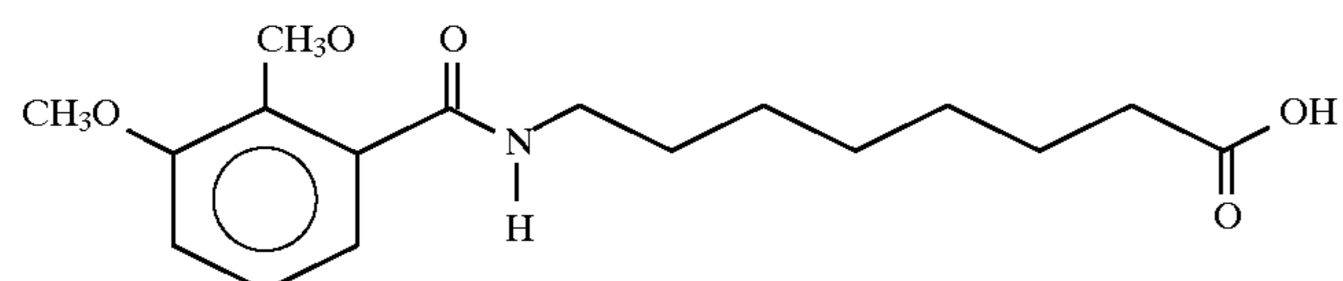
8-(N-(2,3-Dimethoxybenzoyl))aminocaprylic acid
