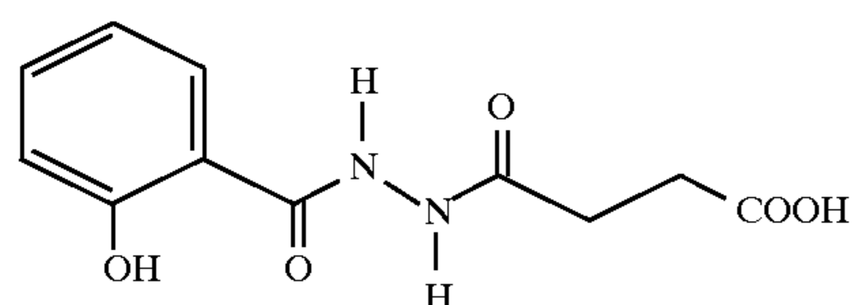
1-Salicyloyl-2-succinyl hydrazide
