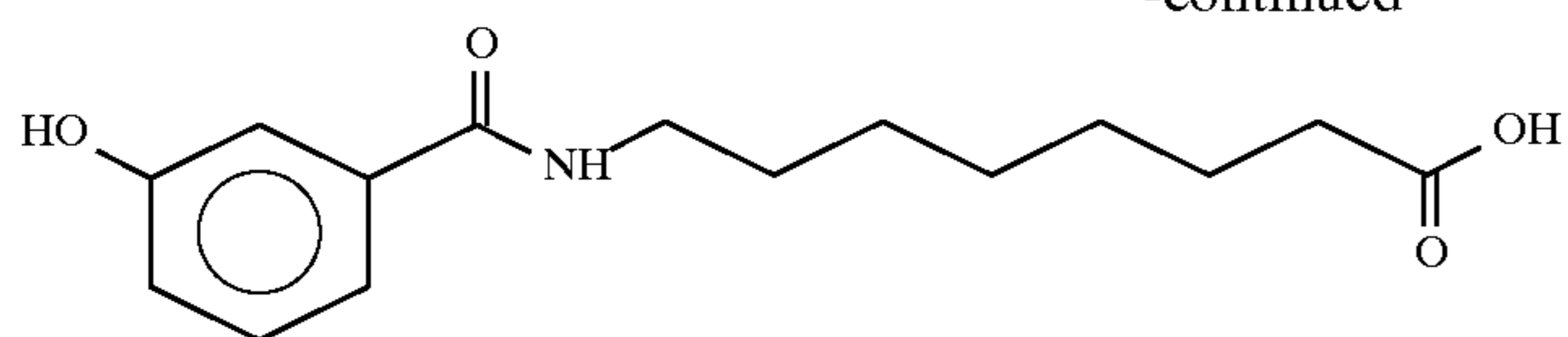
8-(2-Hydroxybenzoyl)aminocaprylic acid
