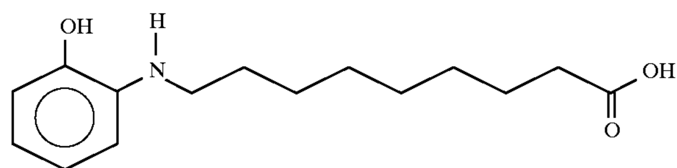
9-(2-hydroxybenzamido)nonanoic acid
