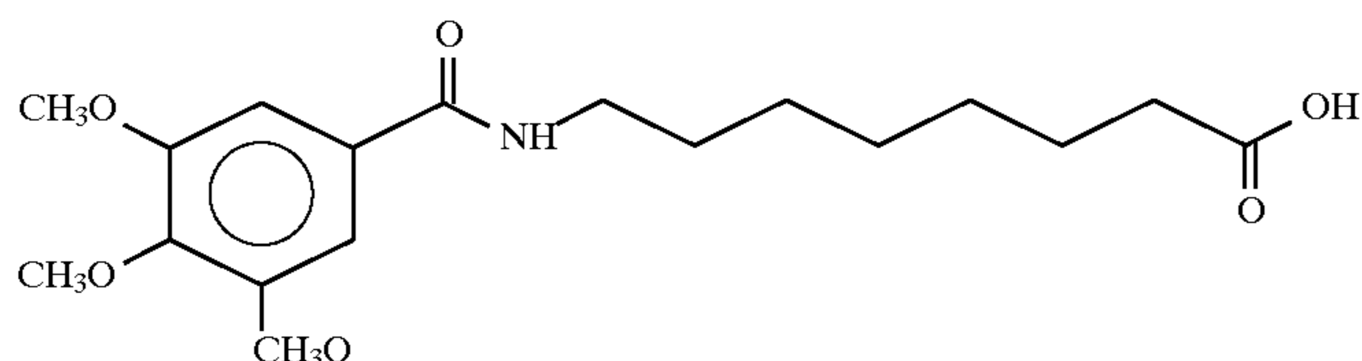
8-(3,4,5-Trimethoxybenzoyl)aminocaprylic acid
