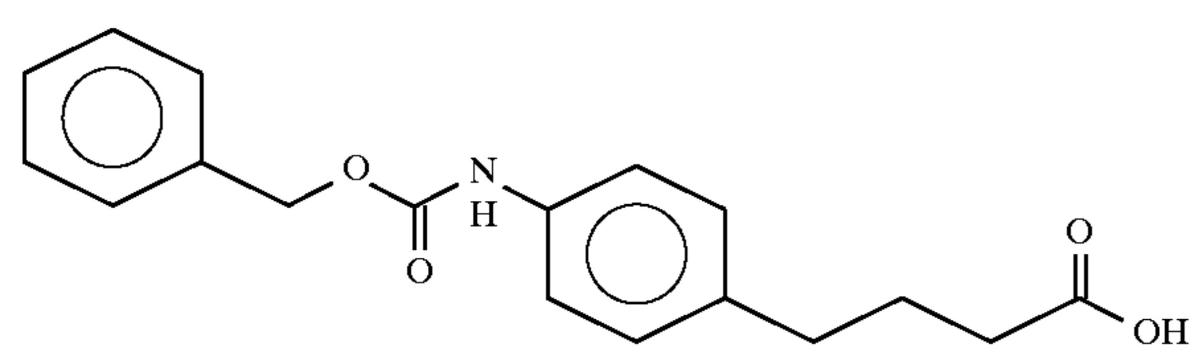
4-(4-benzoyloxycarbonylamino)phenyl)butyric acid
