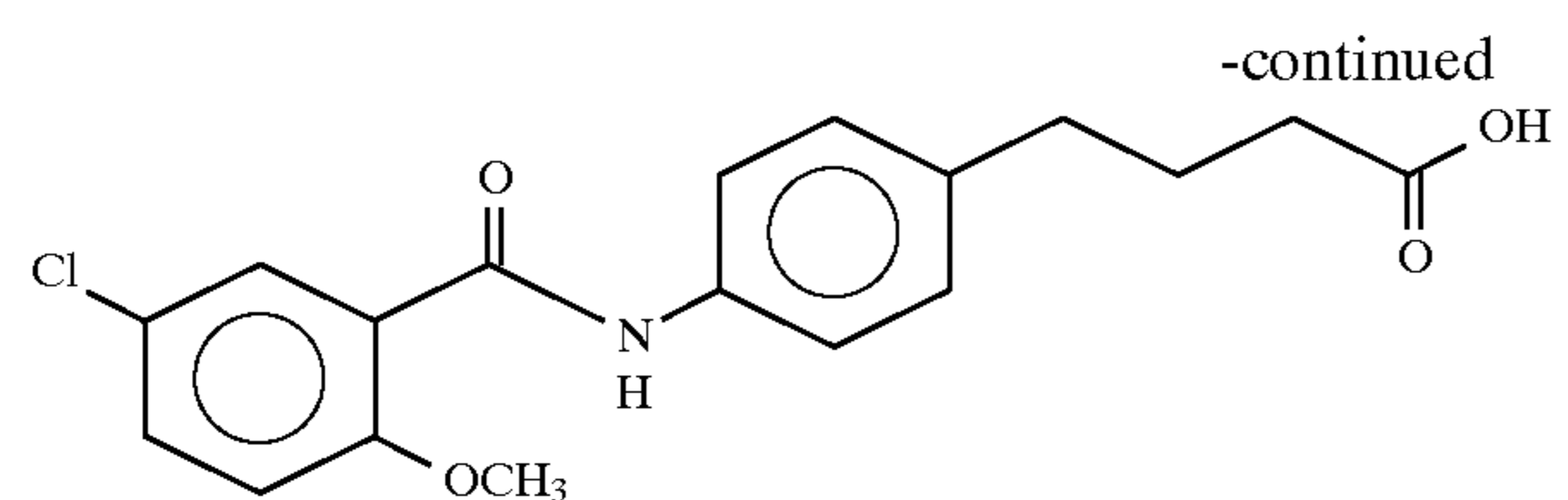
4-(4-(5-chloro-o-anisoyl)aminophenyl)butyric acid
