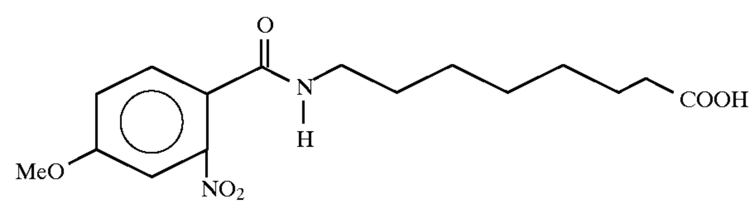
8-N-(4-methoxy-3-nitrobenzoyl)aminocaprylic acid
