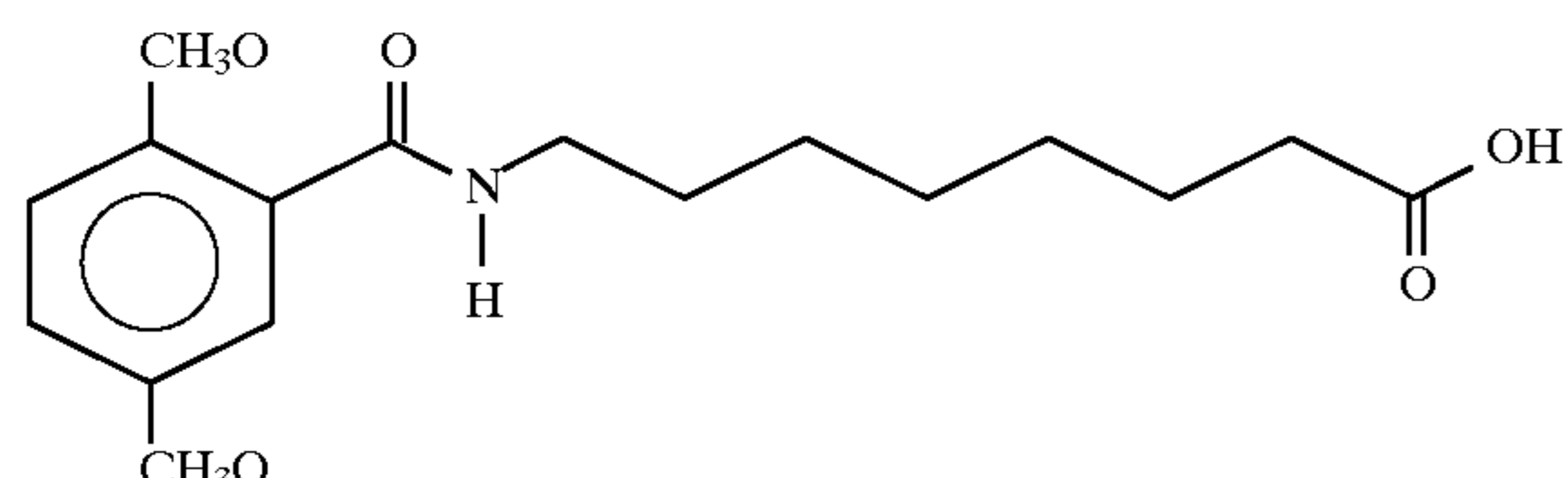
8-(N-(2,5-Dimethoxybenzoyl)]aminocaproic acid
