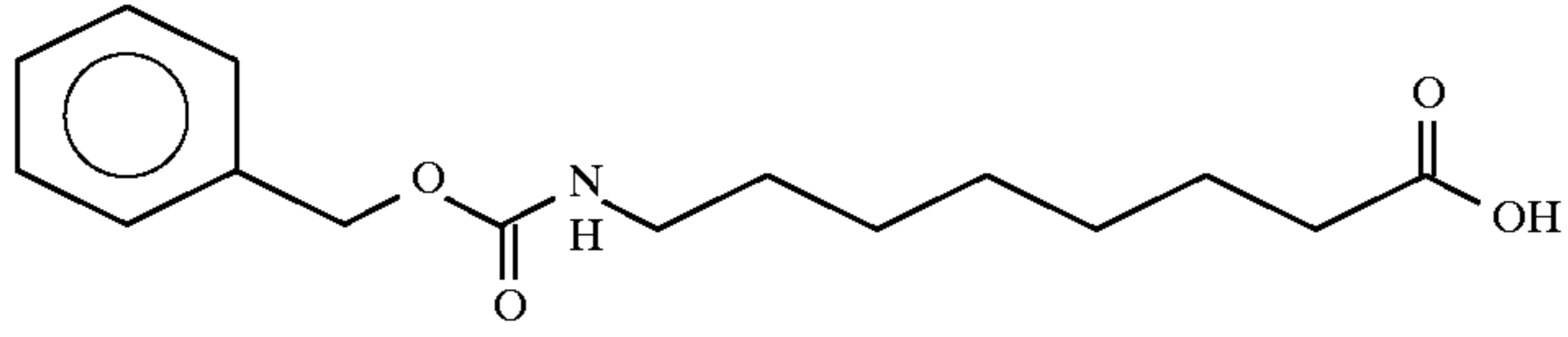
8-Benzylcarbonylamino)caprylic acid
