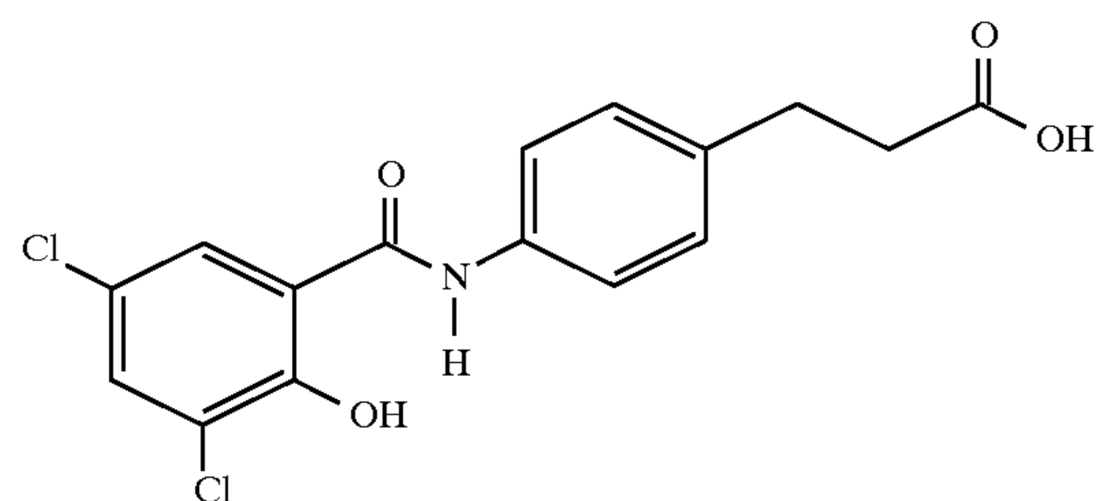
n-[3,5-dichloro-2-hydroxybenzoyl-3-(4-aminophenyl)]propionic acid
