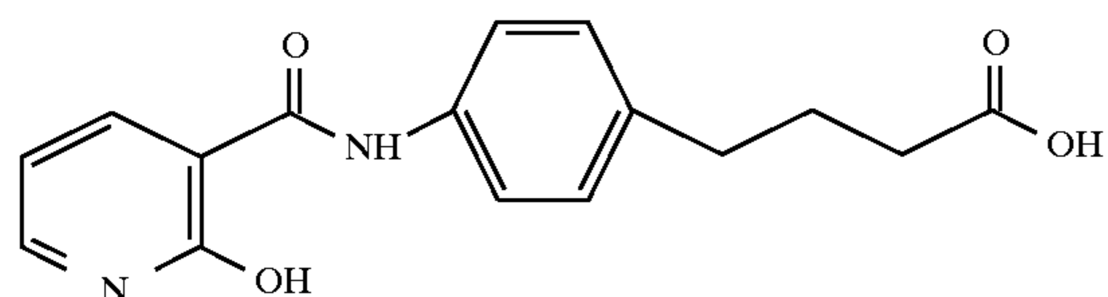
4-(4-(2-hydroxynicotinoyl)aminophenyl)butyric acid
