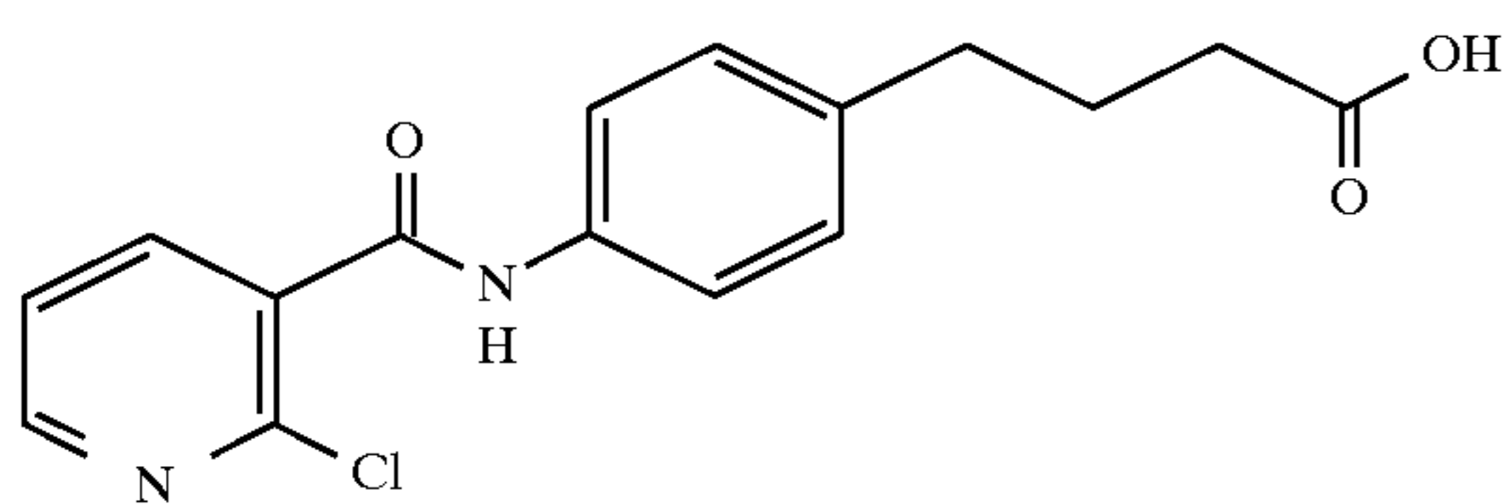
4-(4-(2-chloronicotinoyl)aminophenyl)butyric acid
