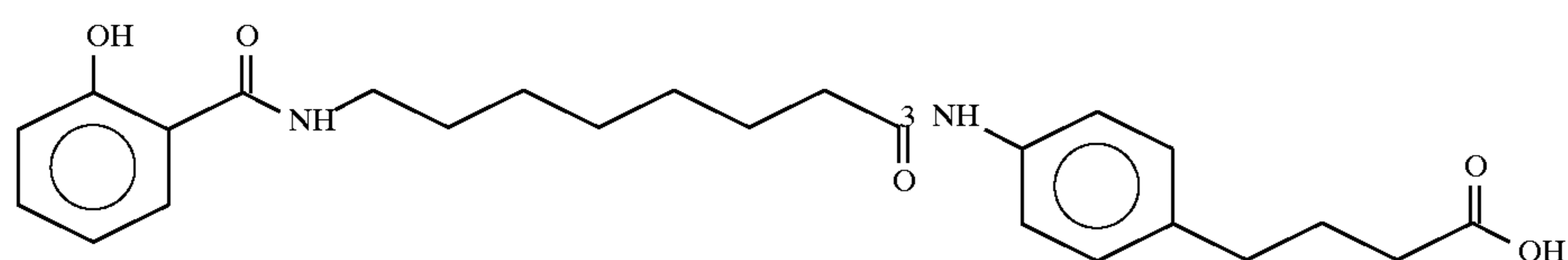
4-(4-(N-8(N-Salicyloyl)aminocaprylic)aminophenyl)butyric acid
