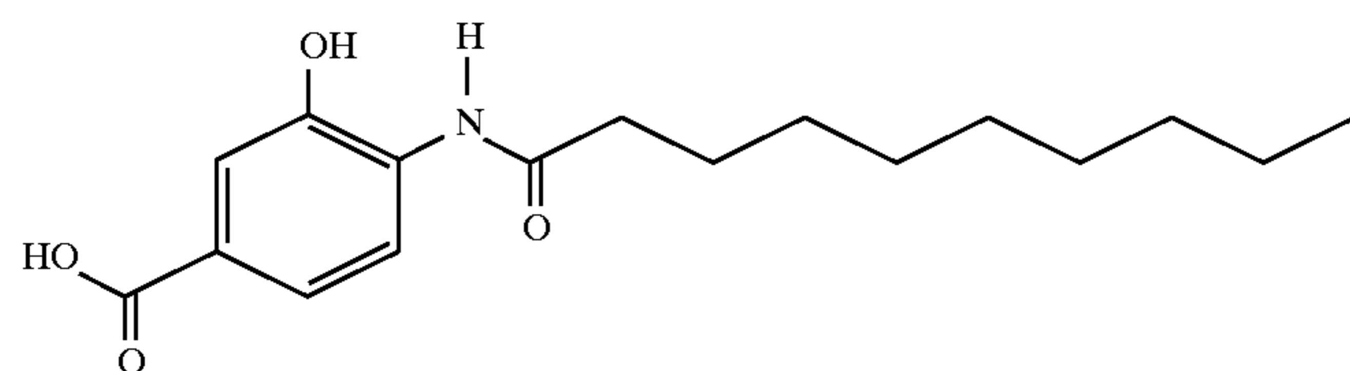
4-octanoylamino-3-hydroxybenzoic acid
