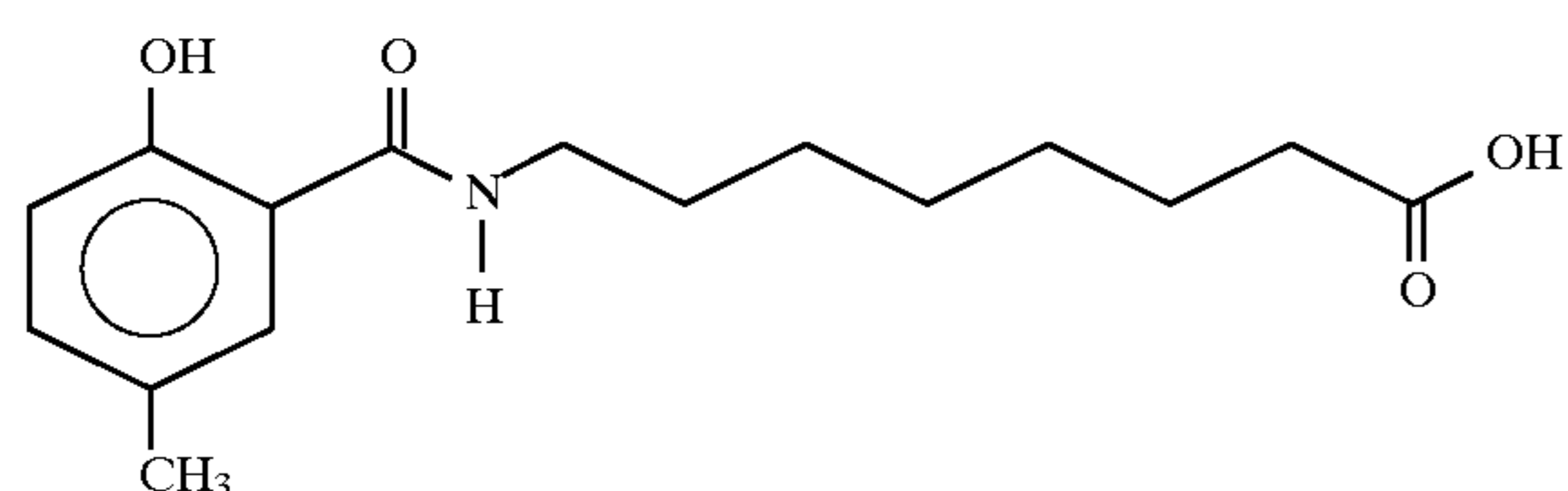
8-(N-5-methylsalicyloyl)aminocaprylic acid
