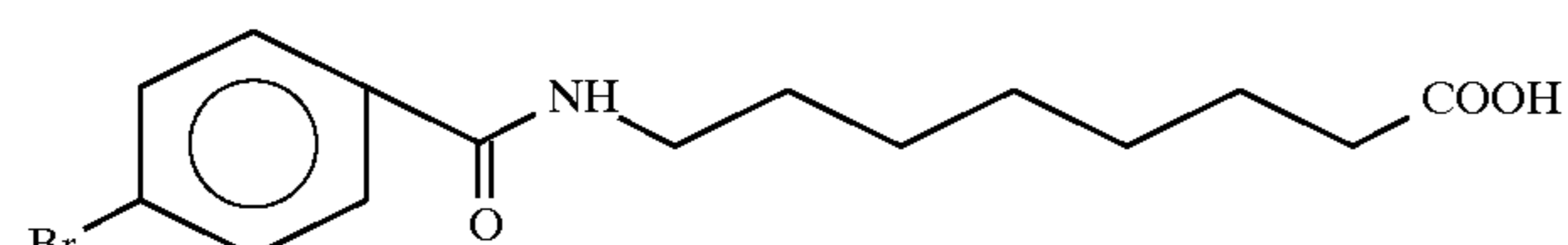
8-[N-(4-bromobenzoyl)]aminocaprylic acid
