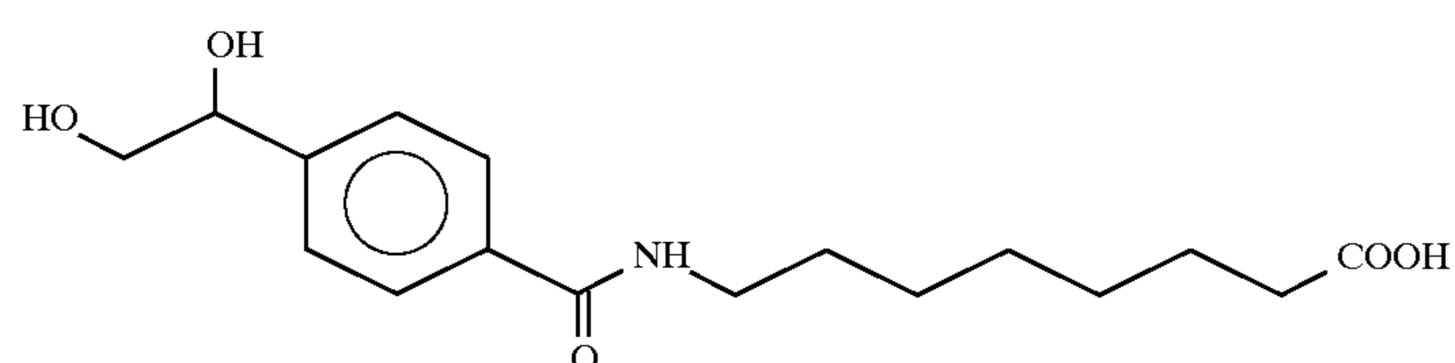
8(4-(1,2-dihydroxyethyl)benzoyl)aminocaprylic acid
