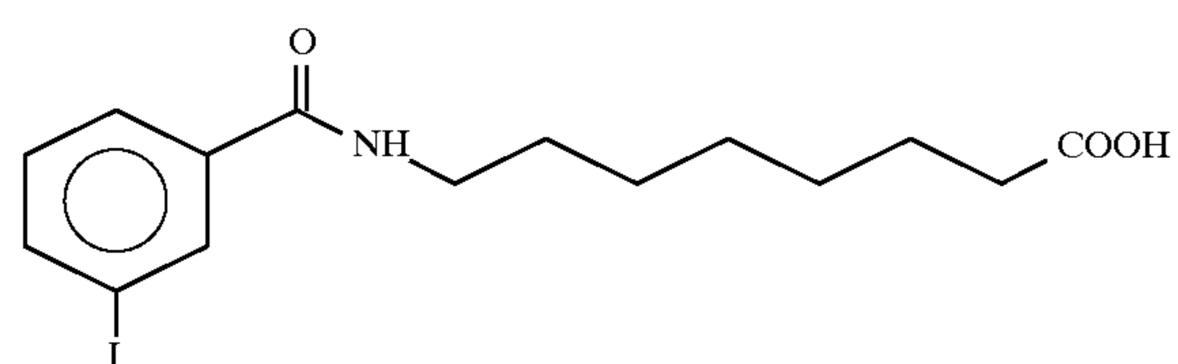
8-N-(3-iodobenzoyl)aminocaprylic acid
