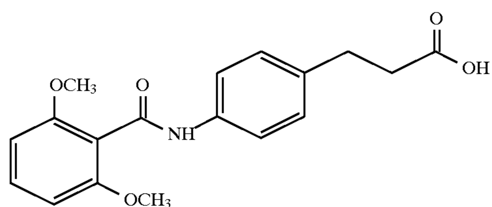
3-(4-(2,6-dimethoxybenzoyl)aminophenyl)propionic acid
