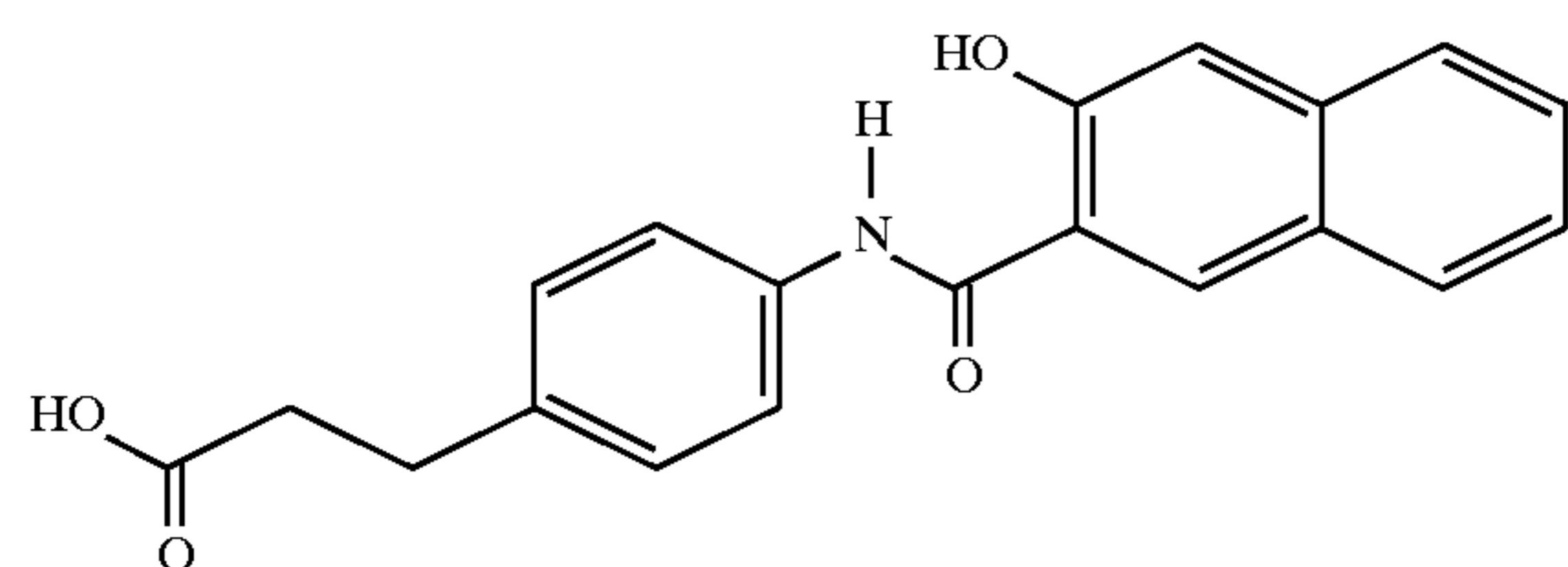
4-[4-[N-(3-hydroxy-2-naphthoyl)aminophenyl]]propanoic acid
