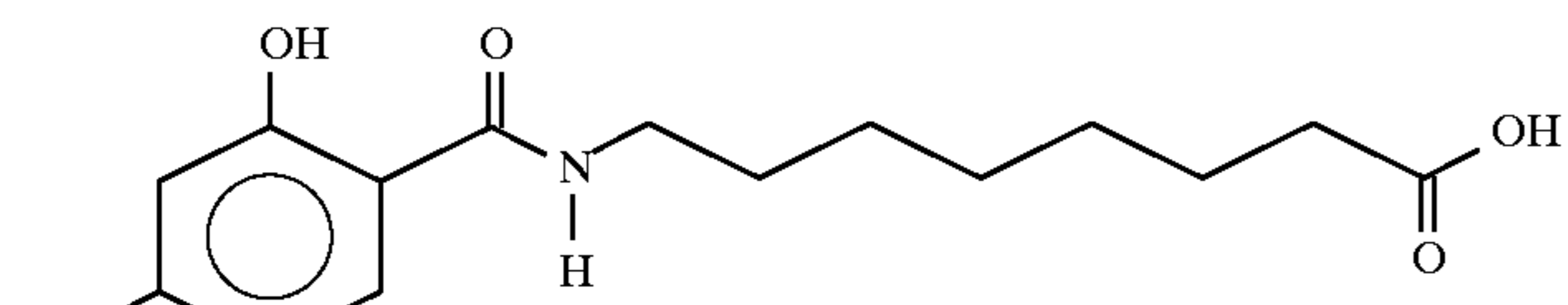
8-(N-(2,4-Dihydroxybenzoyl))aminocaprylic acid
