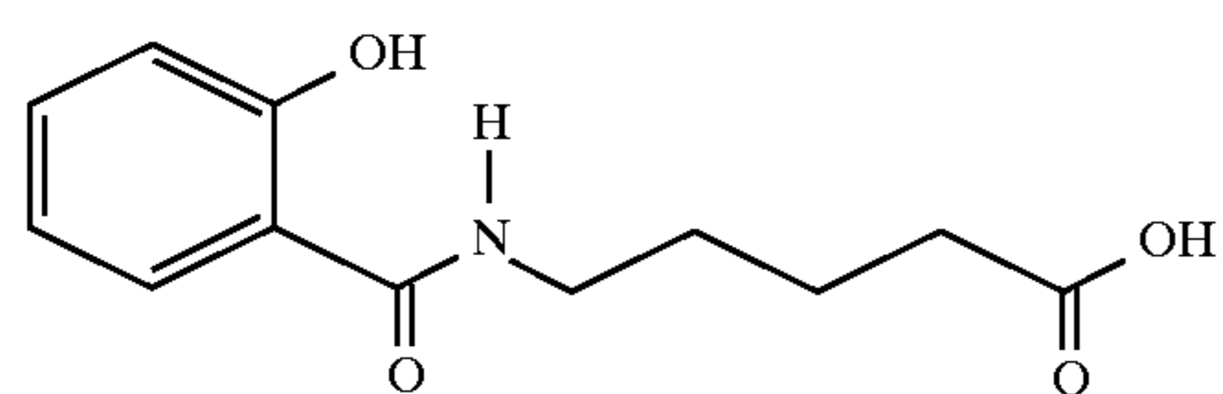
5-(N-salicyloylamino)valeric acid
