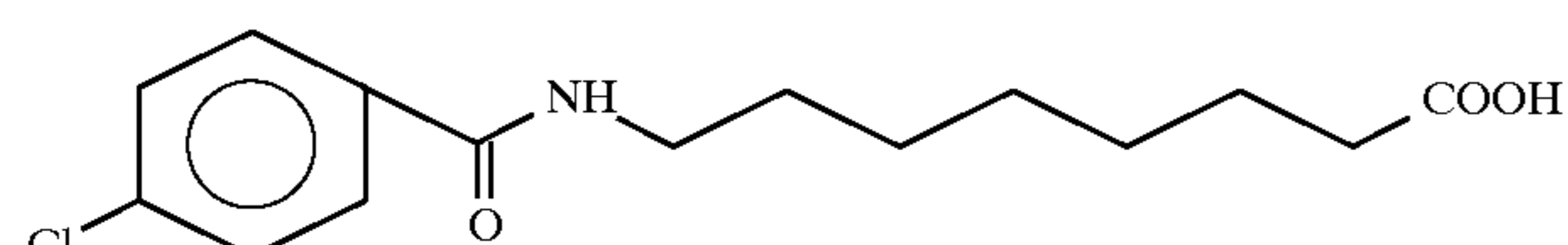
8-[N-(4-chlorobenzoyl)]aminocaprylic acid
