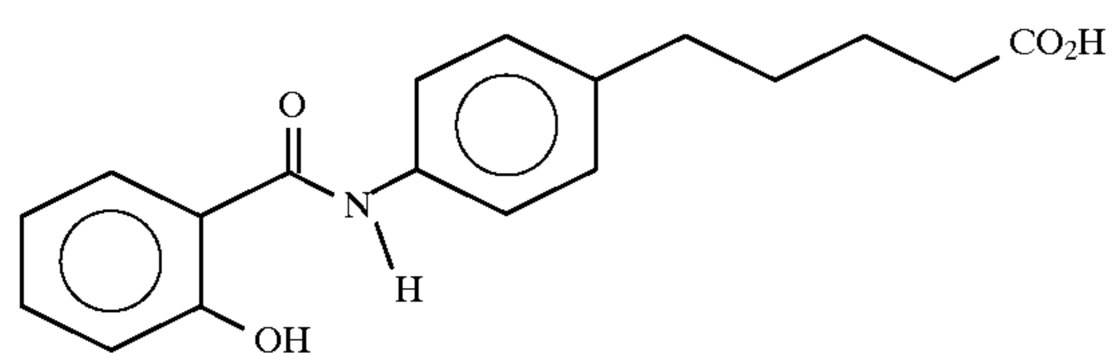
N-salicyloyl-5-(4-aminophenyl)valeric acid
