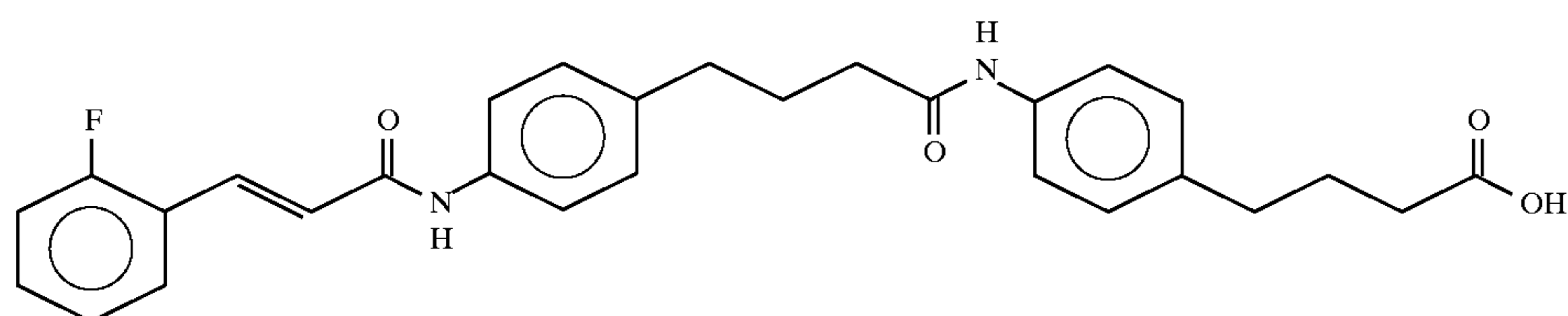
4-(4-(N-(2-Fluorocinnamoyl)aminophenyl) butyric
