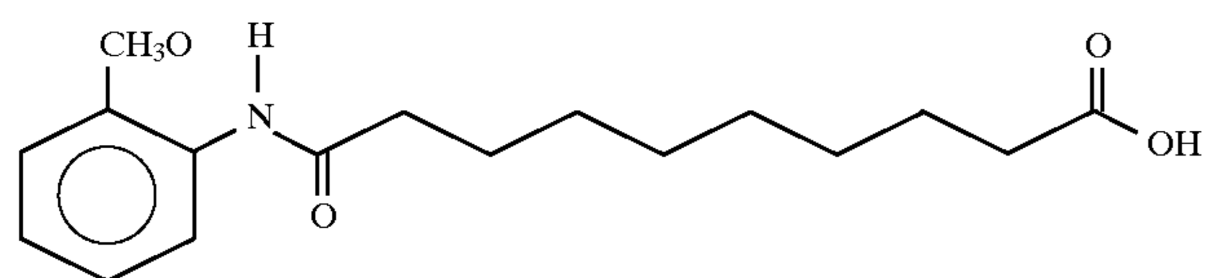
10-(N-(2-Methoxyanilino)]sebacic acid
