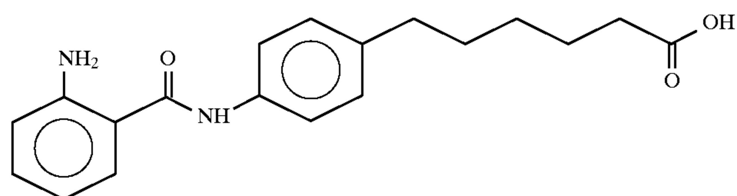
6-(4-(N-(2-aminobenzoyl)aminophenyl)hexanoic acid
