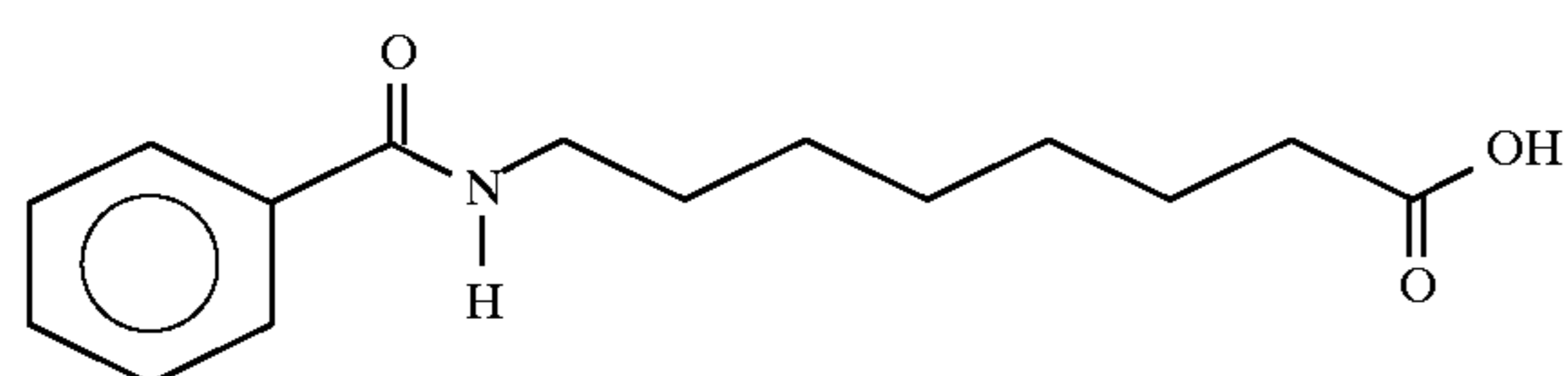
8-(N-benzoyl)aminocaprylic acid
