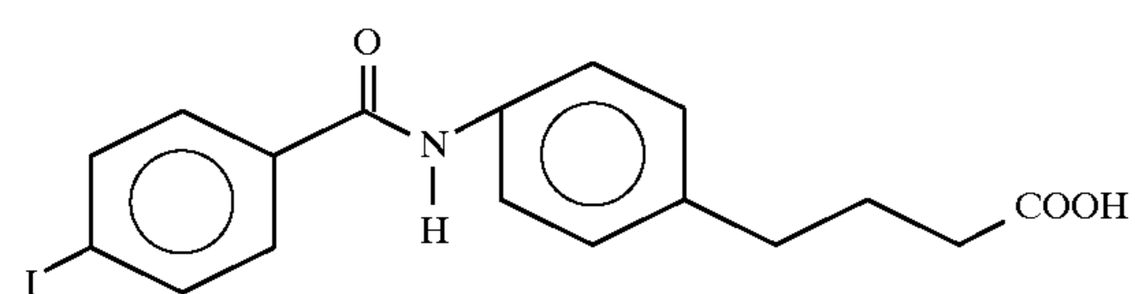
4-[4-[N-(4-iodobenzoyl)aminophenyl]butyric acid
