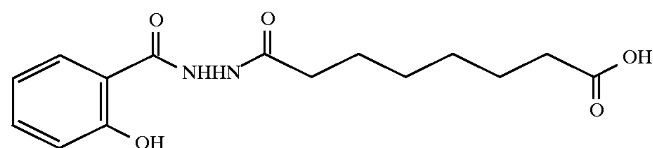
1-salicyloyl-2-suberyl hydrazide
