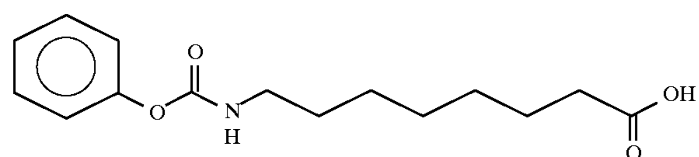
8-(phenylcarbonylamino)caprylic acid
