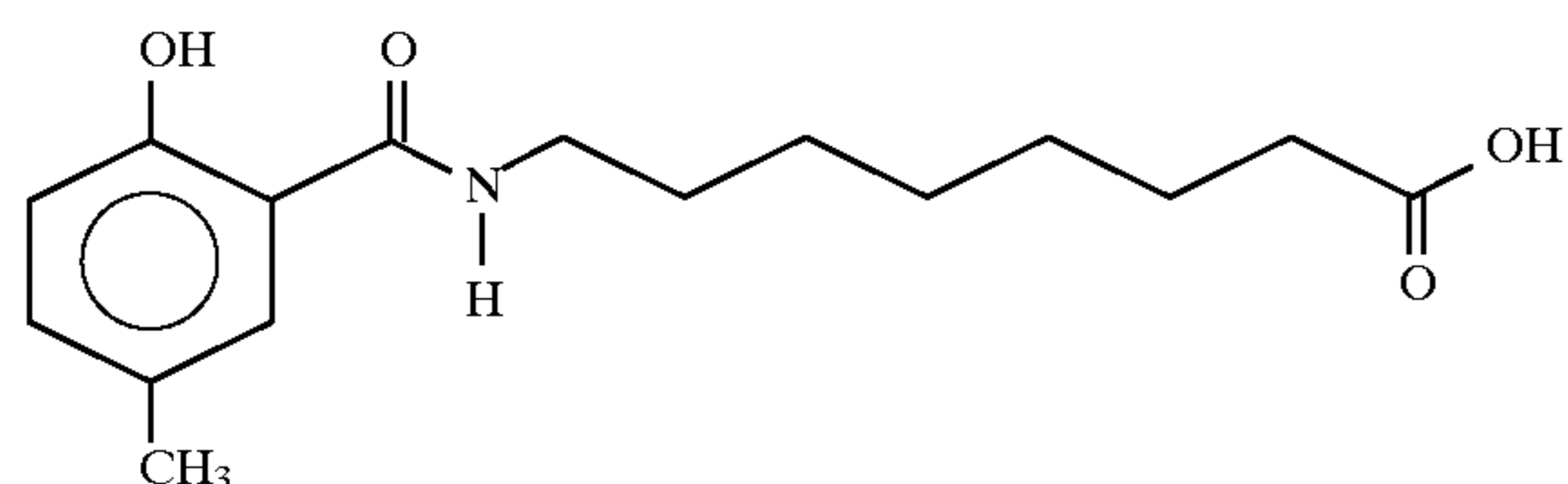
8-(N-5-methylsalicyloyl)aminocaprylic acid
