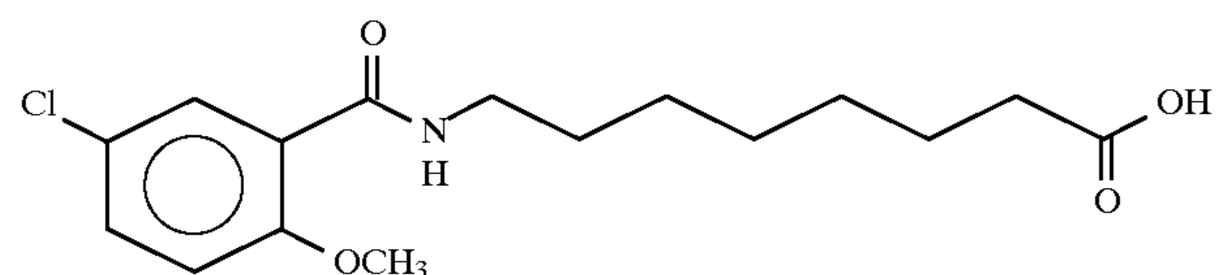
8-(5-chloro-o-anisoyl)aminocaprylic acid
