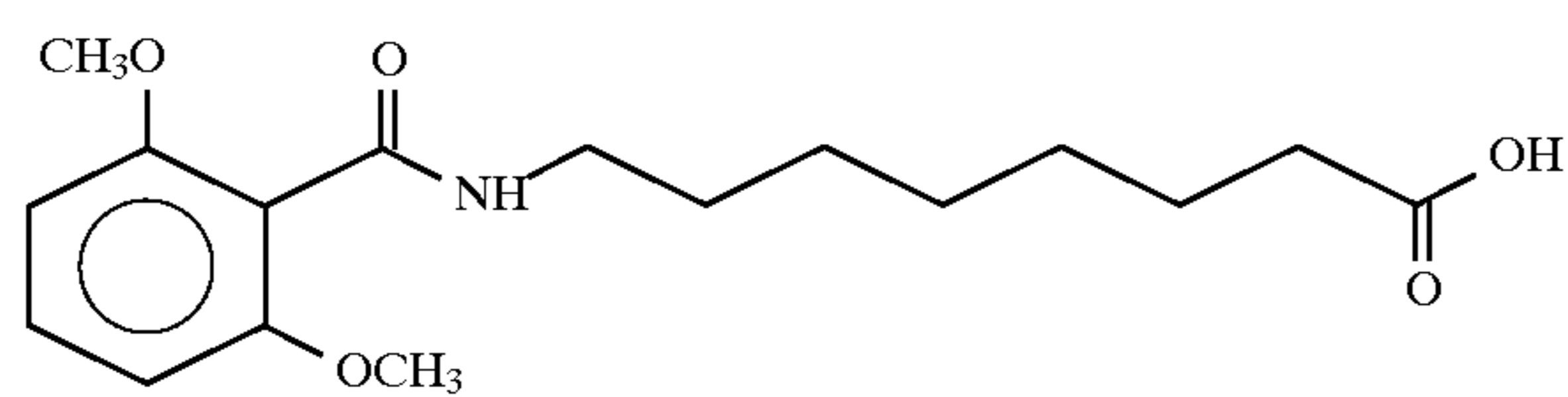
8-(N-2,6-Dimethoxybenzoyl)aminocaprylic acid
