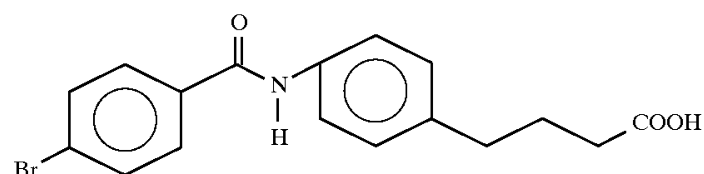
4-{4-[N-(4-bromobenzoyl)aminophenyl]}butyric acid
