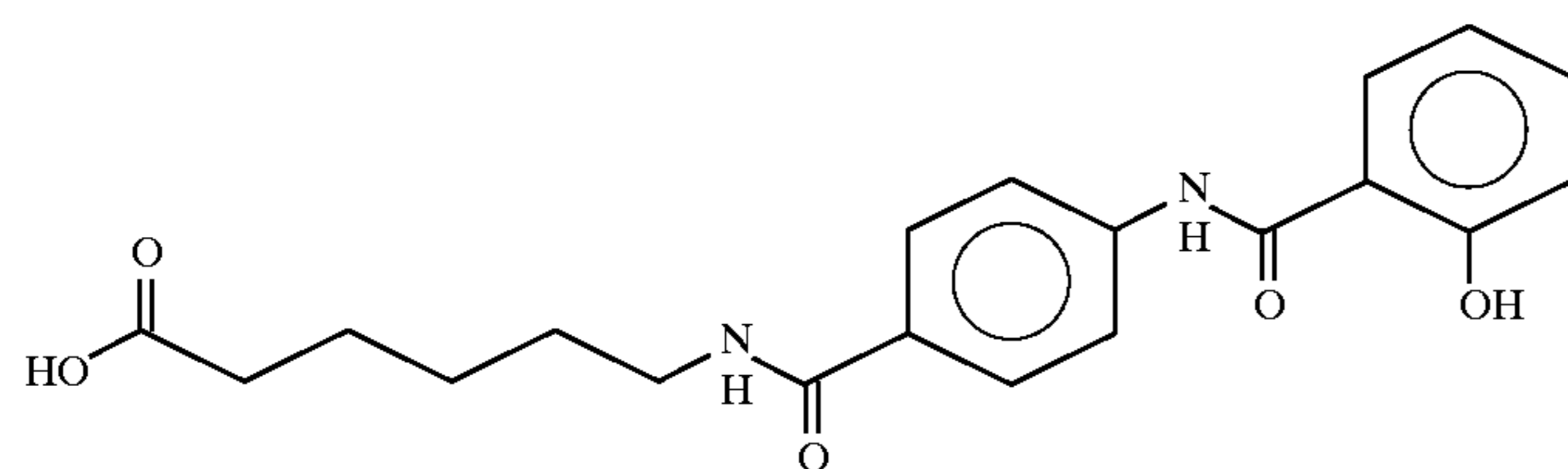
N-(4-salicyloylamino)-6-caproic acid
