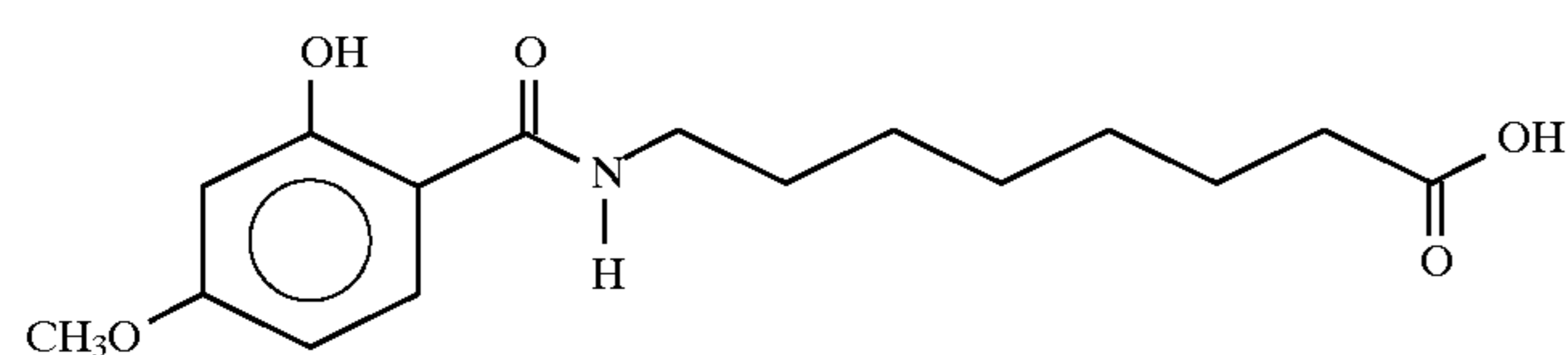
8-(N-2-Hydroxy-4-methoxybenzoyl)aminocaprylic acid
