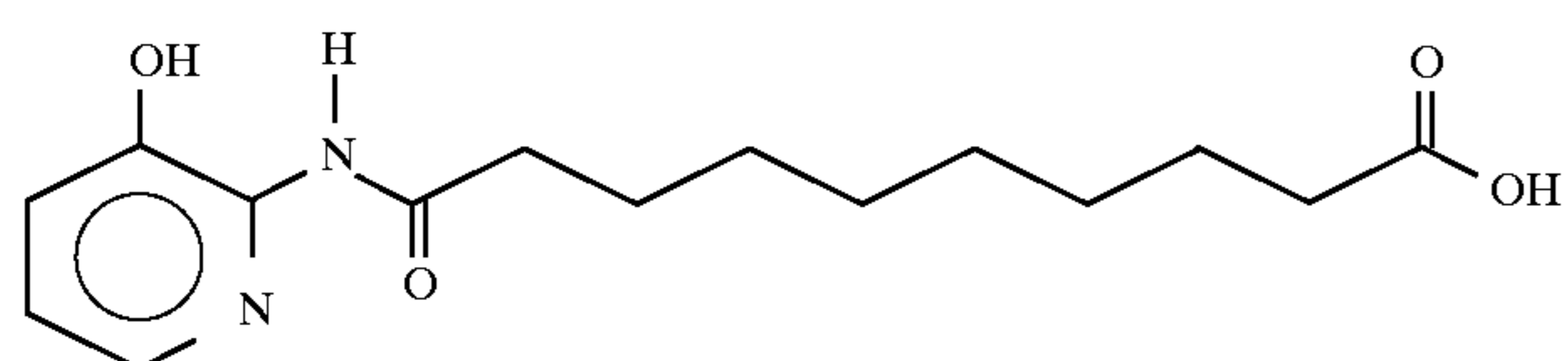
9-[2-(3-hydroxy)pyridylaminocarbonyl]nonanoic acid
