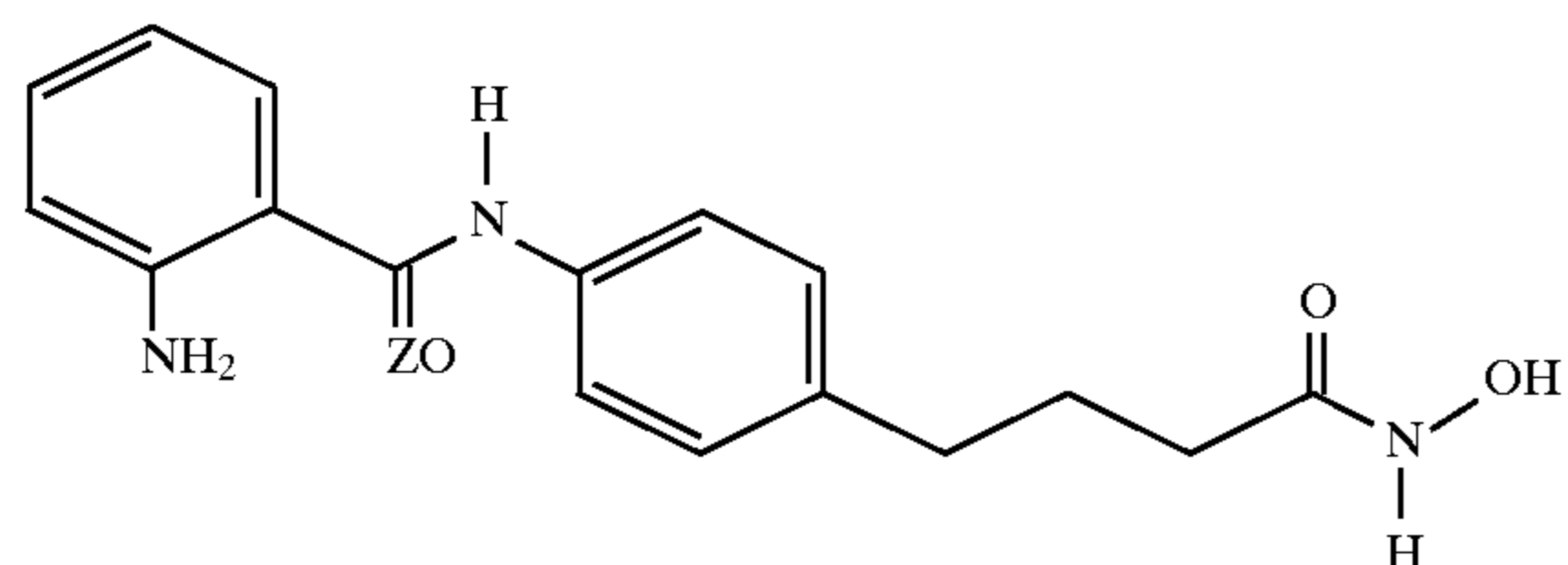
4-[4-(2-aminobenzoylamino)phenyl]butyrylhydroxamic acid
