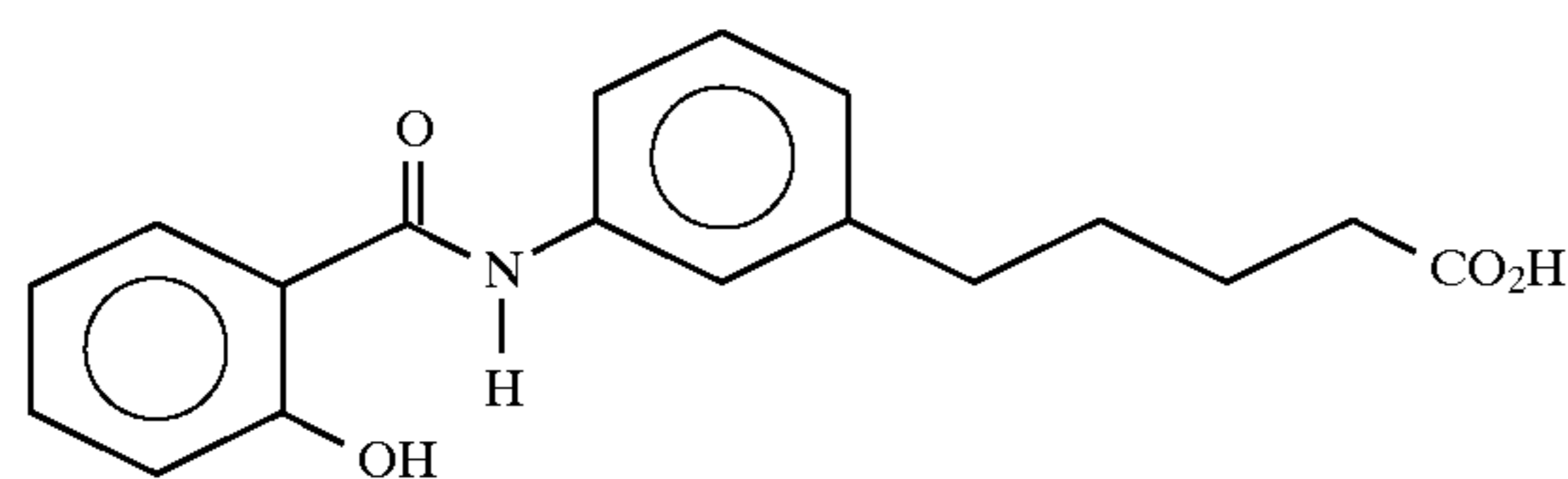
N-salicyloyl-5-(3-aminophenyl)valeric acid
