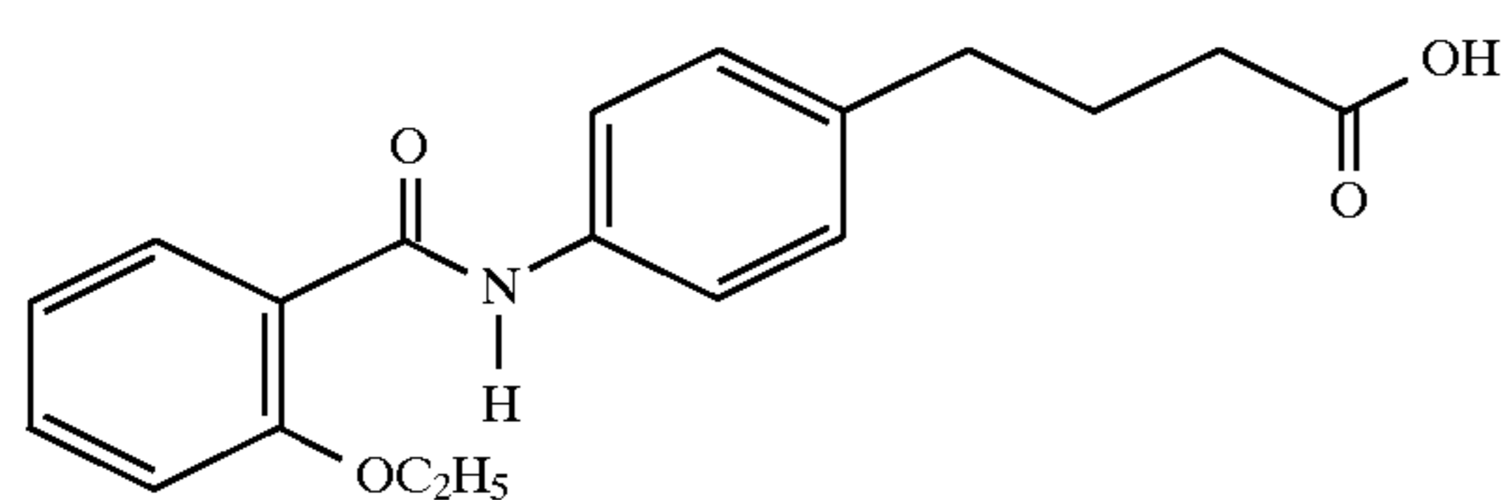
4-(4-(2-ethoxybenzoyl)aminophenyl)butyric acid
