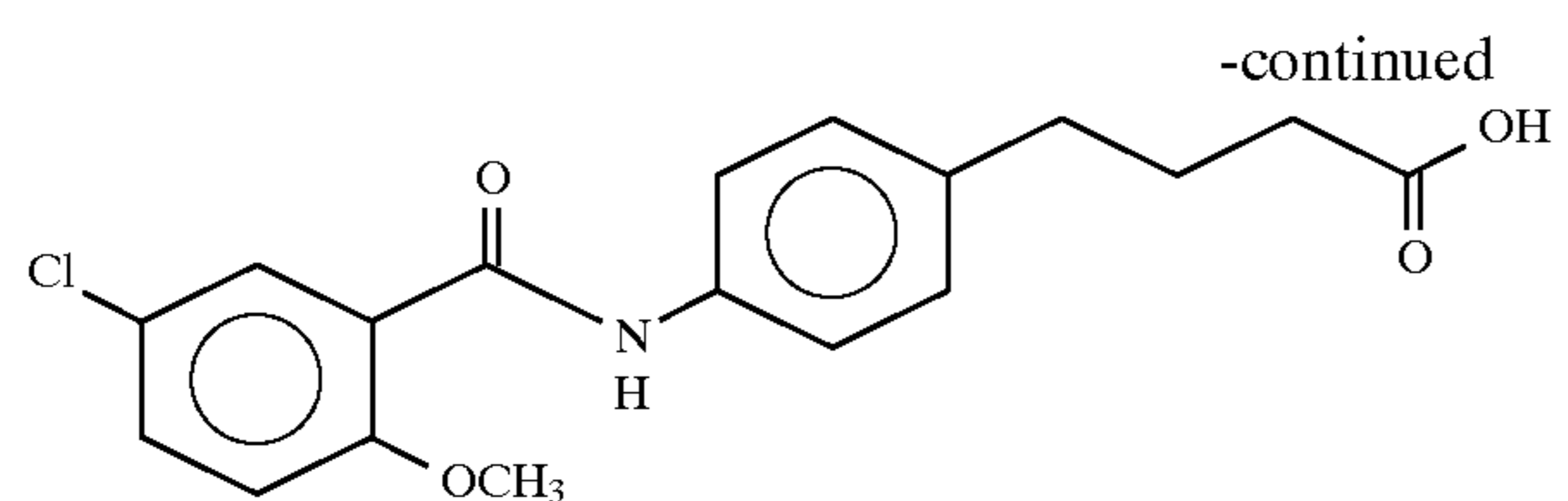
4-(4-(5-chloro-o-anisoyl)aminophenyl)butyric acid
