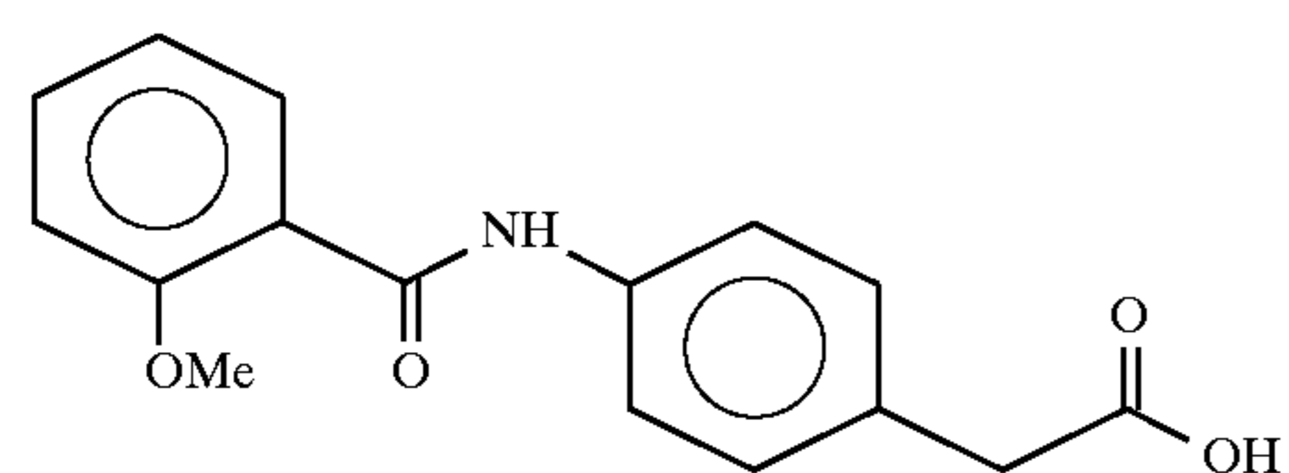
4-(o-anisoyl)aminophenylacetic acid
