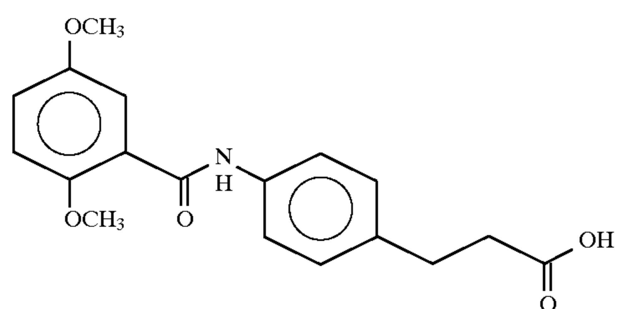
3-(4-(2,5-dimethoxybenzoyl)aminophenyl)propionic acid
