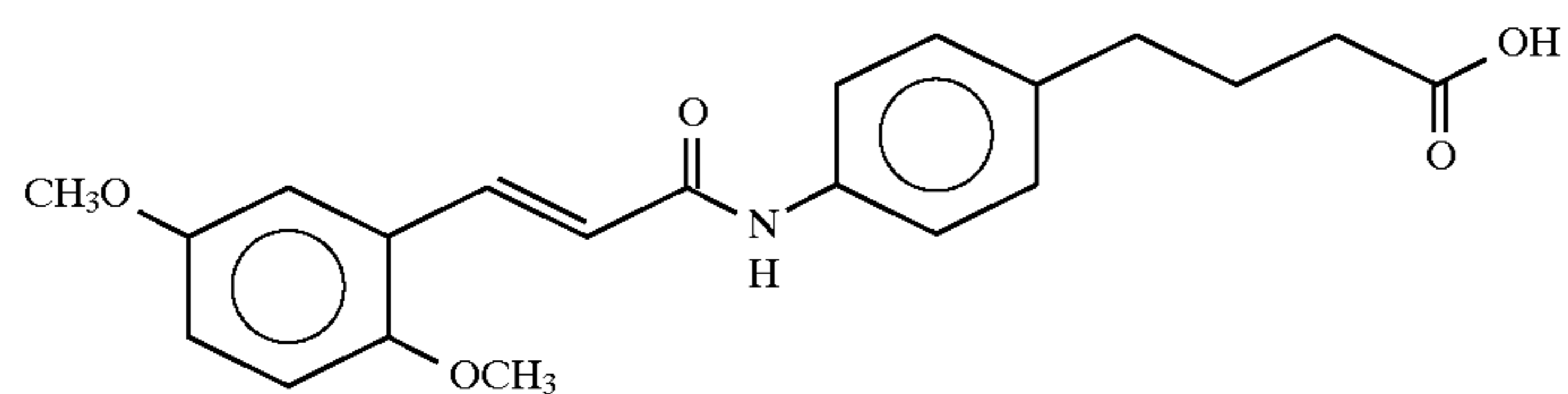
4-(4-(2,5-dimethoxycinnamoyl)aminophenyl)butyric acid
