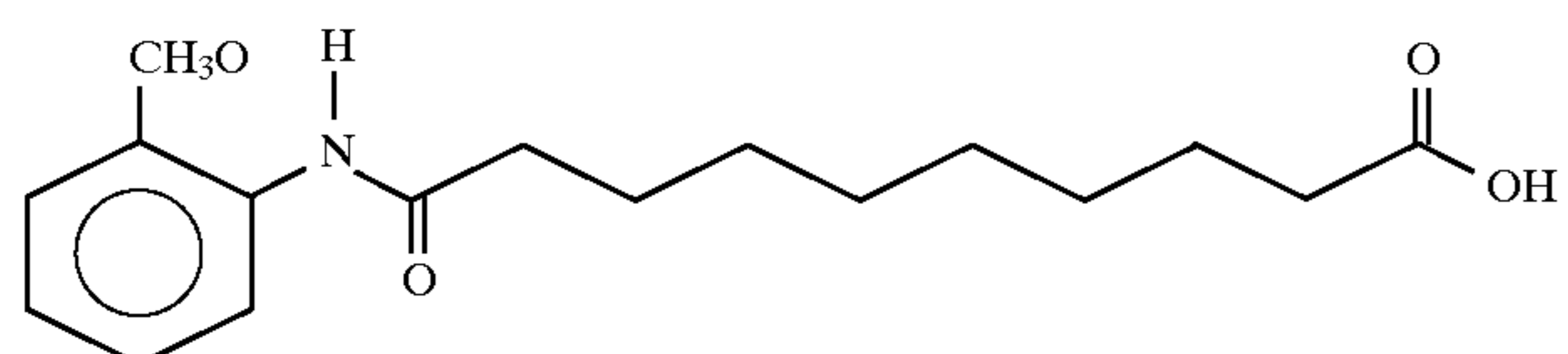
10-(N-(2-Methoxyanilino)]sebacic acid
