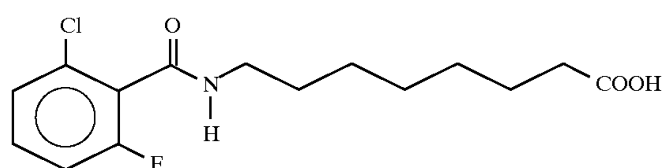
8-N-(2-chloro-6-fluorobenzoyl)aminocaprylic acid
