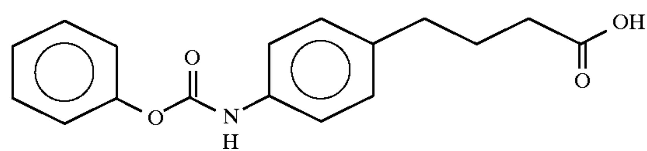
4-(4-phanyloxycarbonylamino)phenyl)butyric acid
