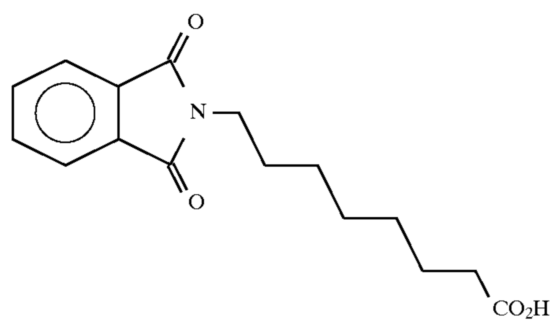
8-(phthalimido)caprylic acid
