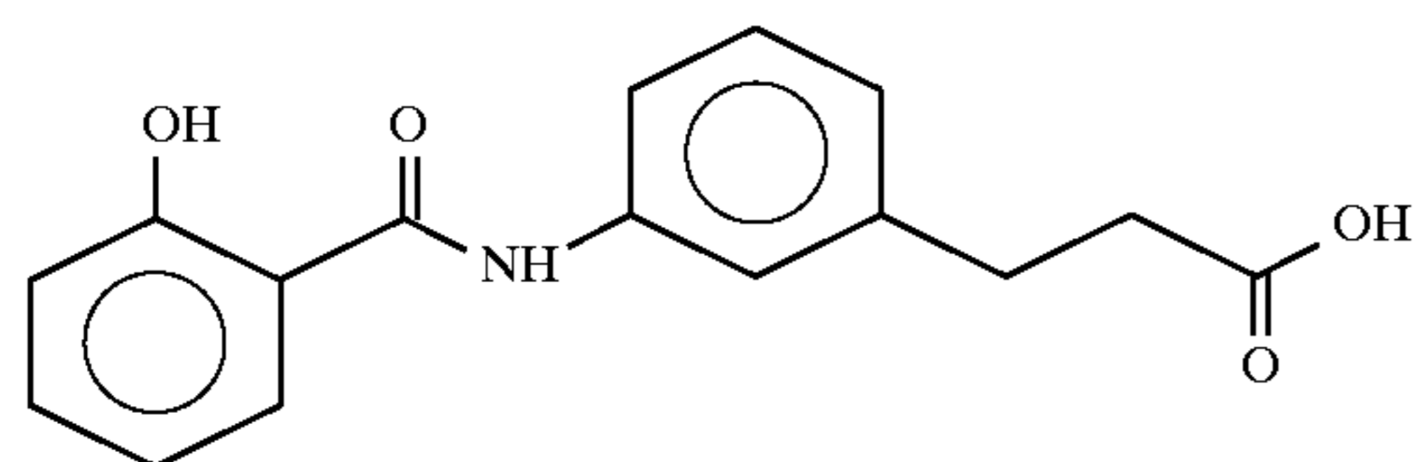
3-(3-(salicyloyl)aminophenyl)propionic acid
