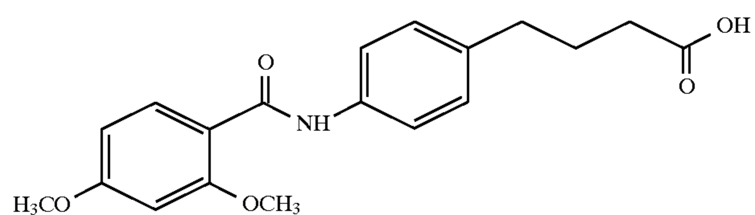
4-(4-(2,4-dimethoxybenzoyl)aminophenyl)butyric acid
