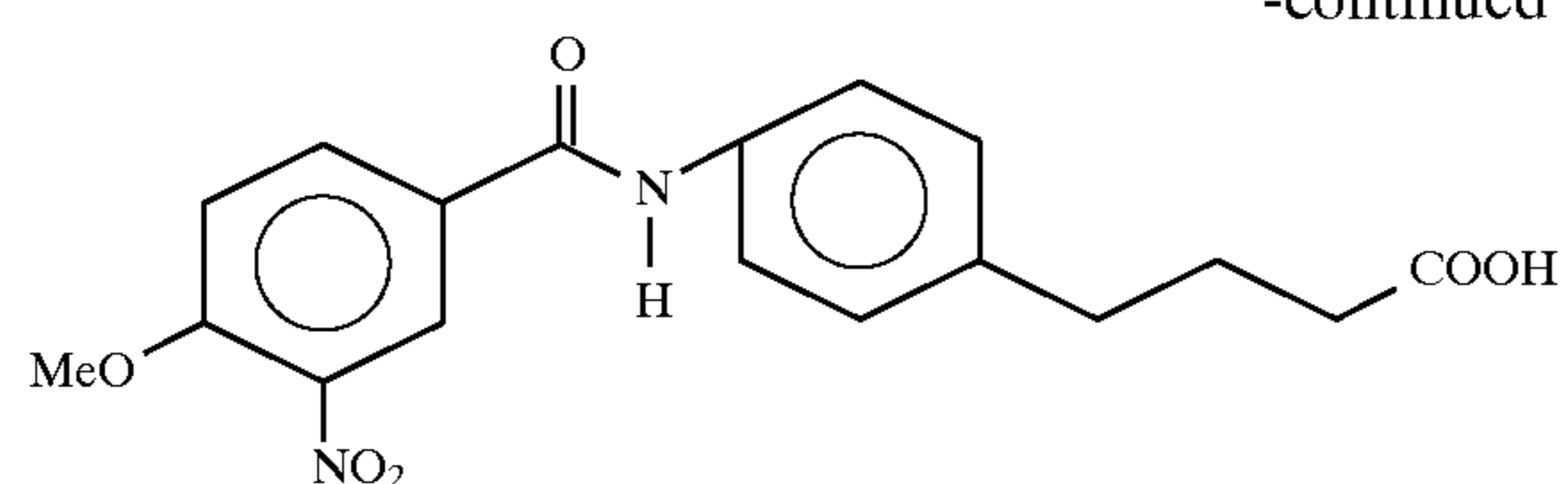
4-[4-N-(4-methoxy-3-nitrobenzoyl)aminophenyl]butyric acid
