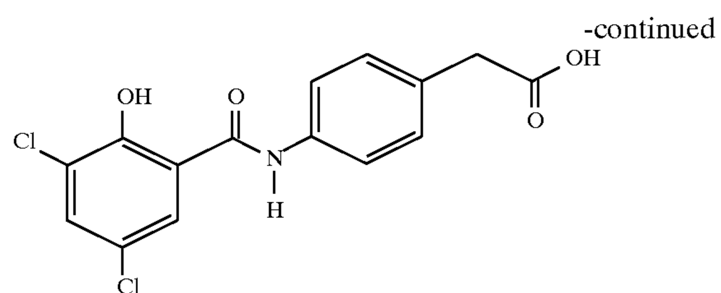
4-[N-(3,5-chloro-2-hydroxybenzoyl)]aminophenylacetic acid
