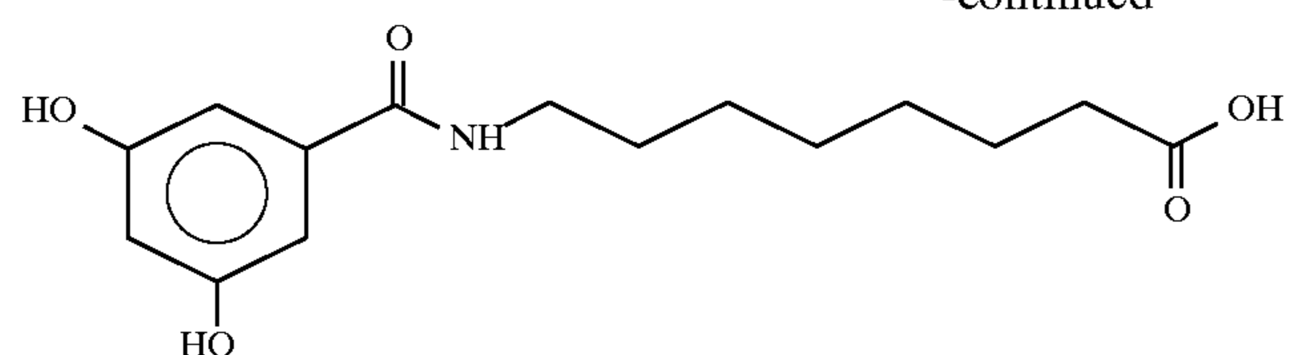
8-(N-3,5-Dihydroxybenzoyl)aminocaprylic acid
