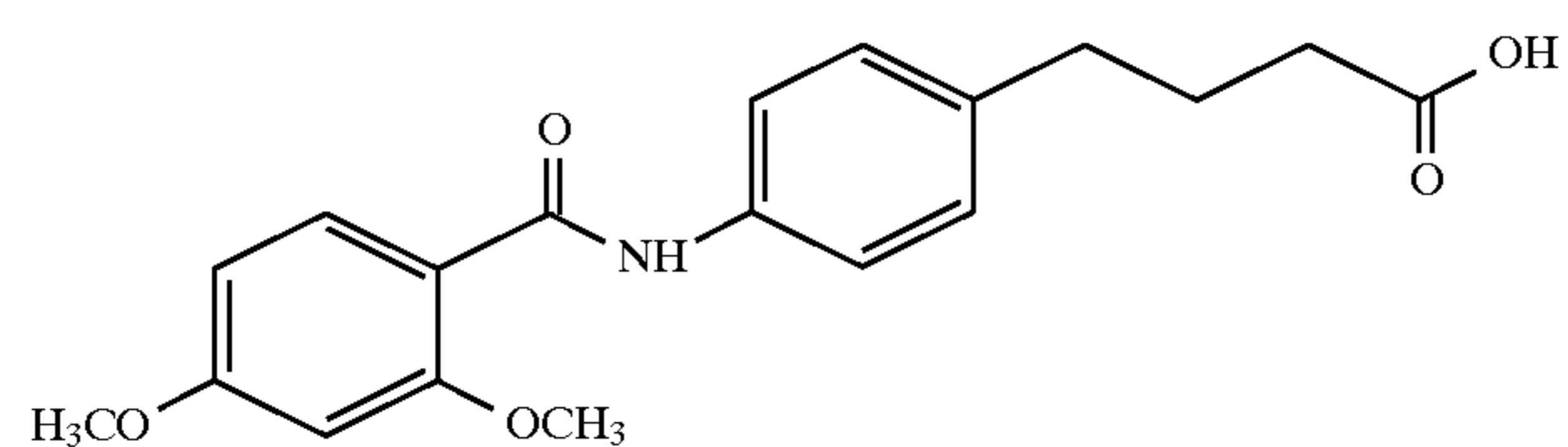
4-(4-(2,4-dimethoxybenzoyl)aminophenyl)butyric acid
