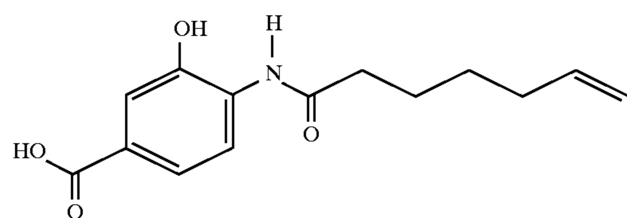
N-(2-hydroxy-4-carboxy)-6-heptenamide
