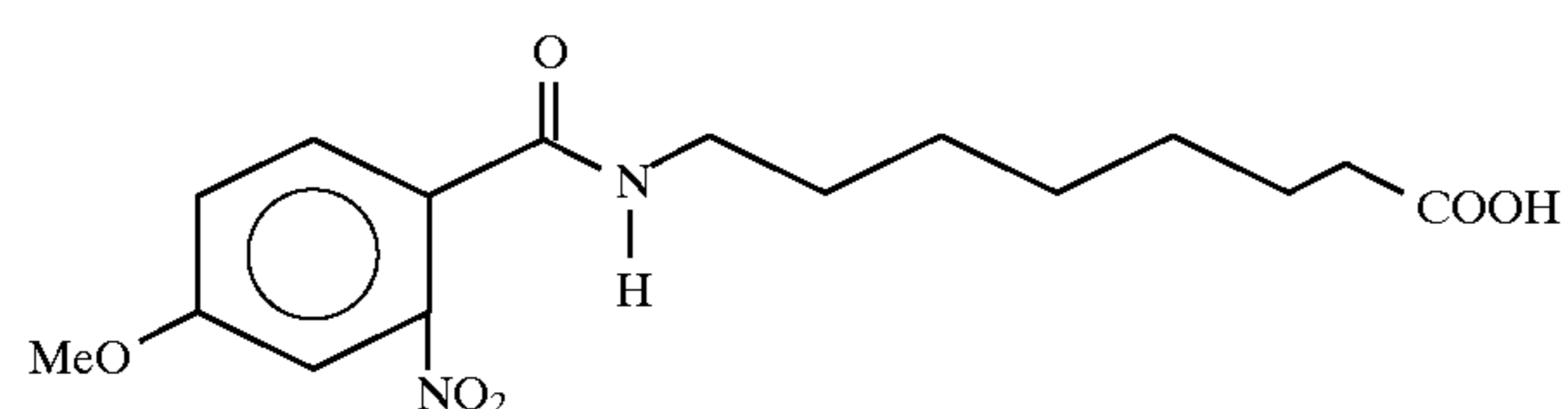
8-N-(4-methoxy-3-nitrobenzoyl)aminocaprylic acid
