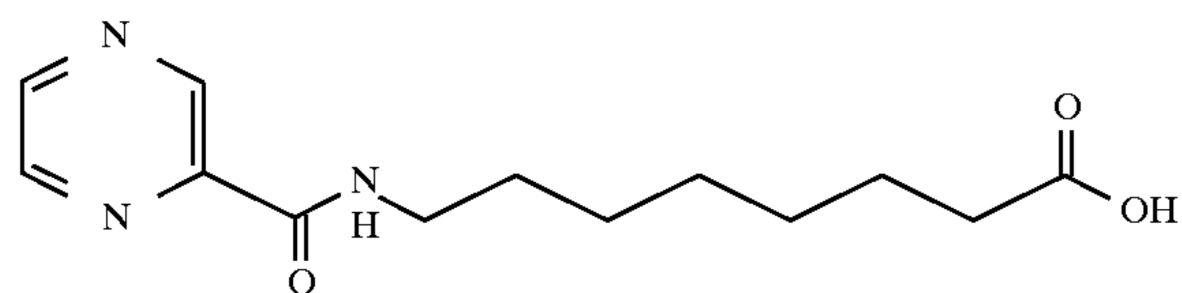
8-(2-pyrazinecarbonyl)aminocaprylic acid
