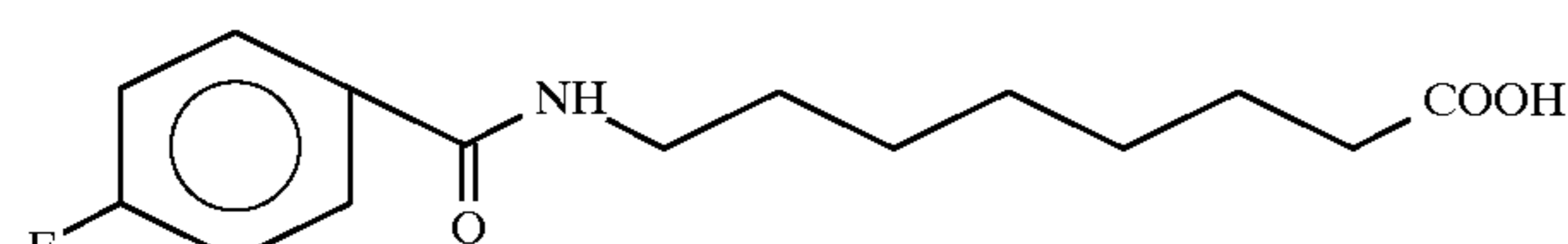
8-[N-(4-fluorobenzoyl)]aminocaprylic acid
