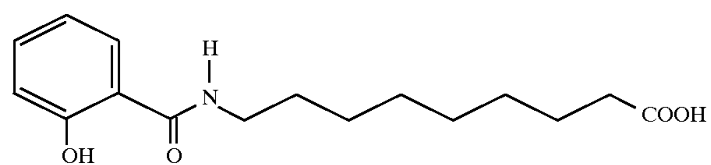
9-Salicyloylaminononanic acid
