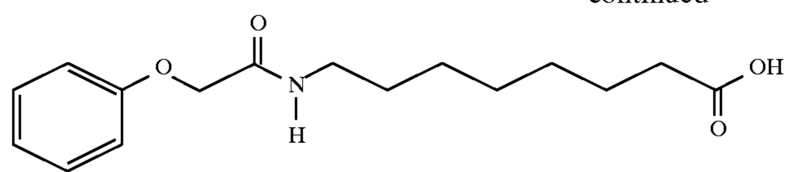
8-(Phenoxyacetyl)aminocaprylic acid
