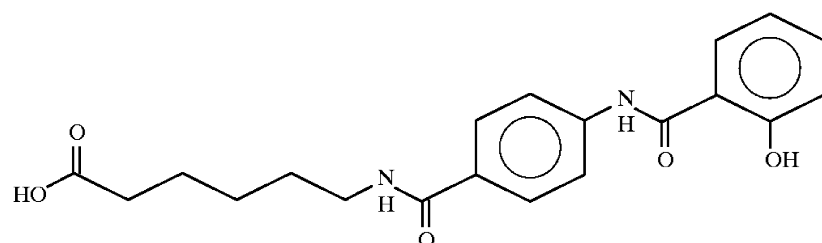
N-(4-salicyloylamino)-6-caproic acid
