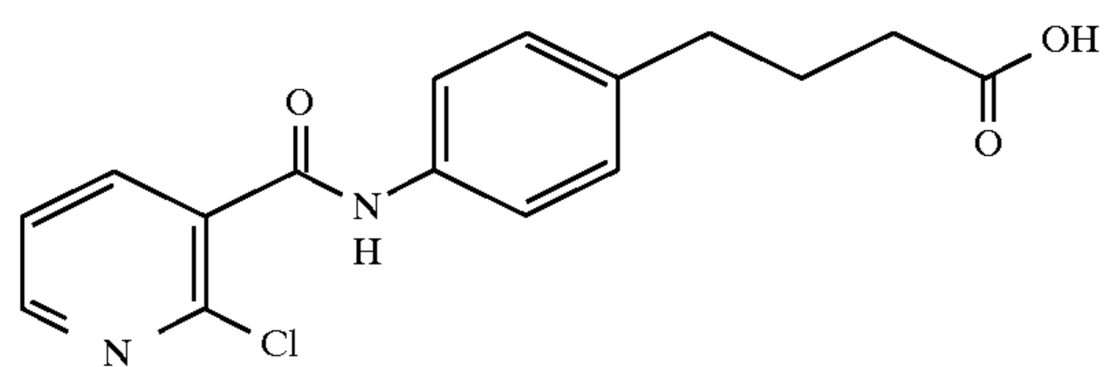
4-(4-(2-chloronicotinoyl)aminophenyl)butyric acid
