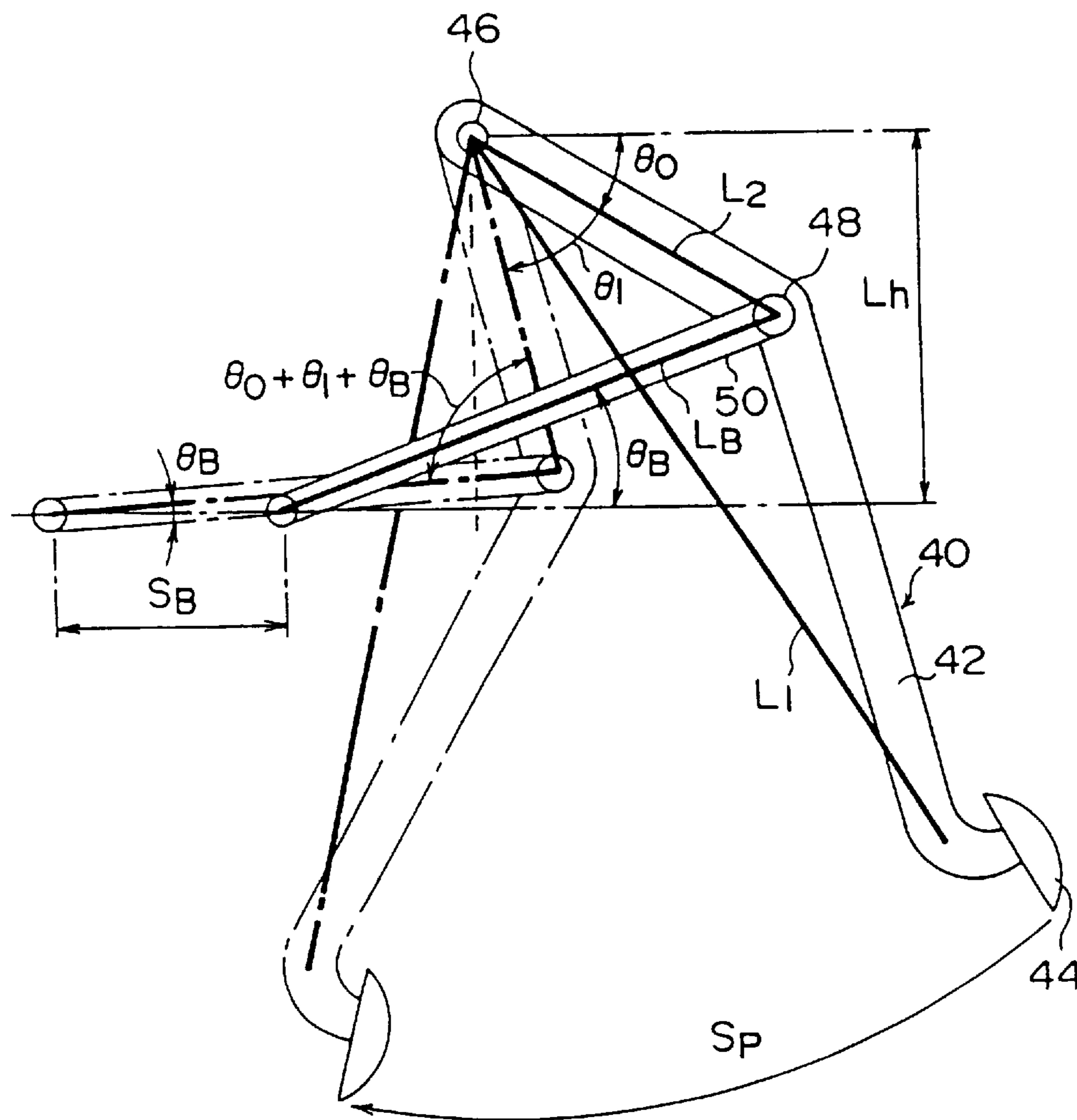
FIG. 7 PRIOR ART
