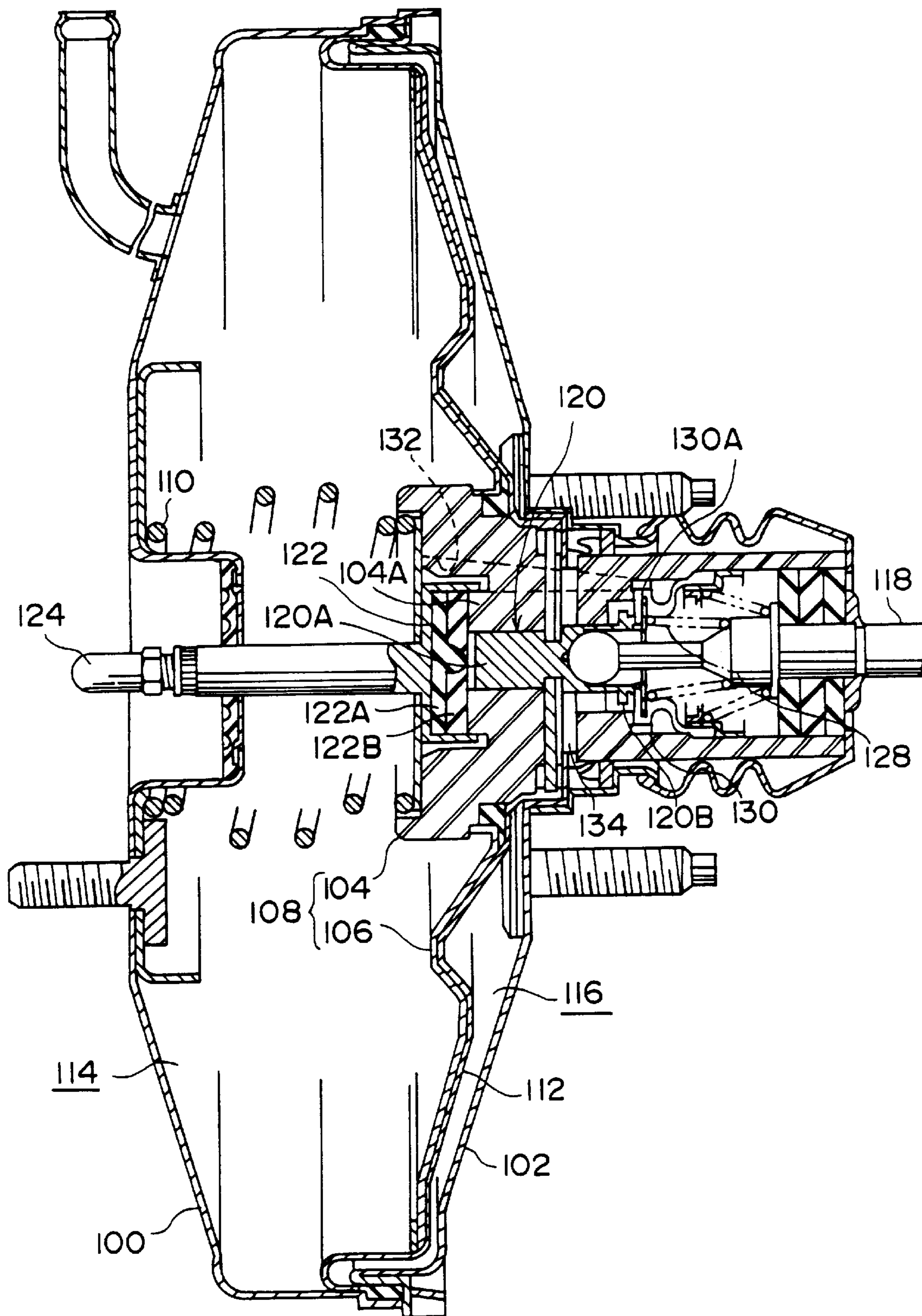
FIG. 1 PRIOR ART
