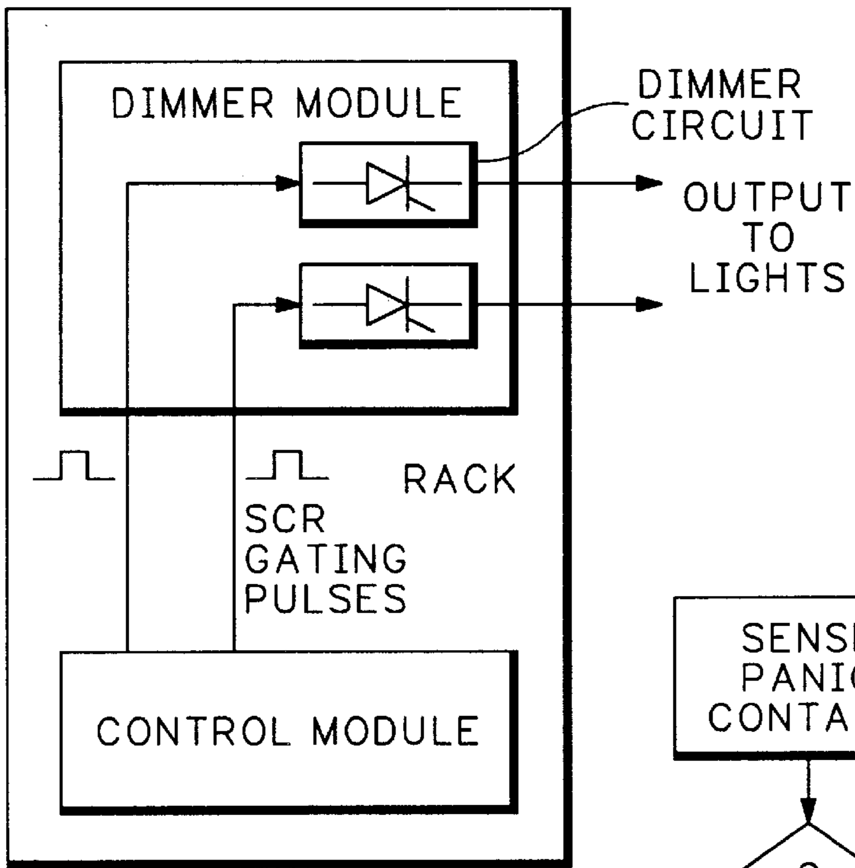
FIG.19 (PRIOR ART)
