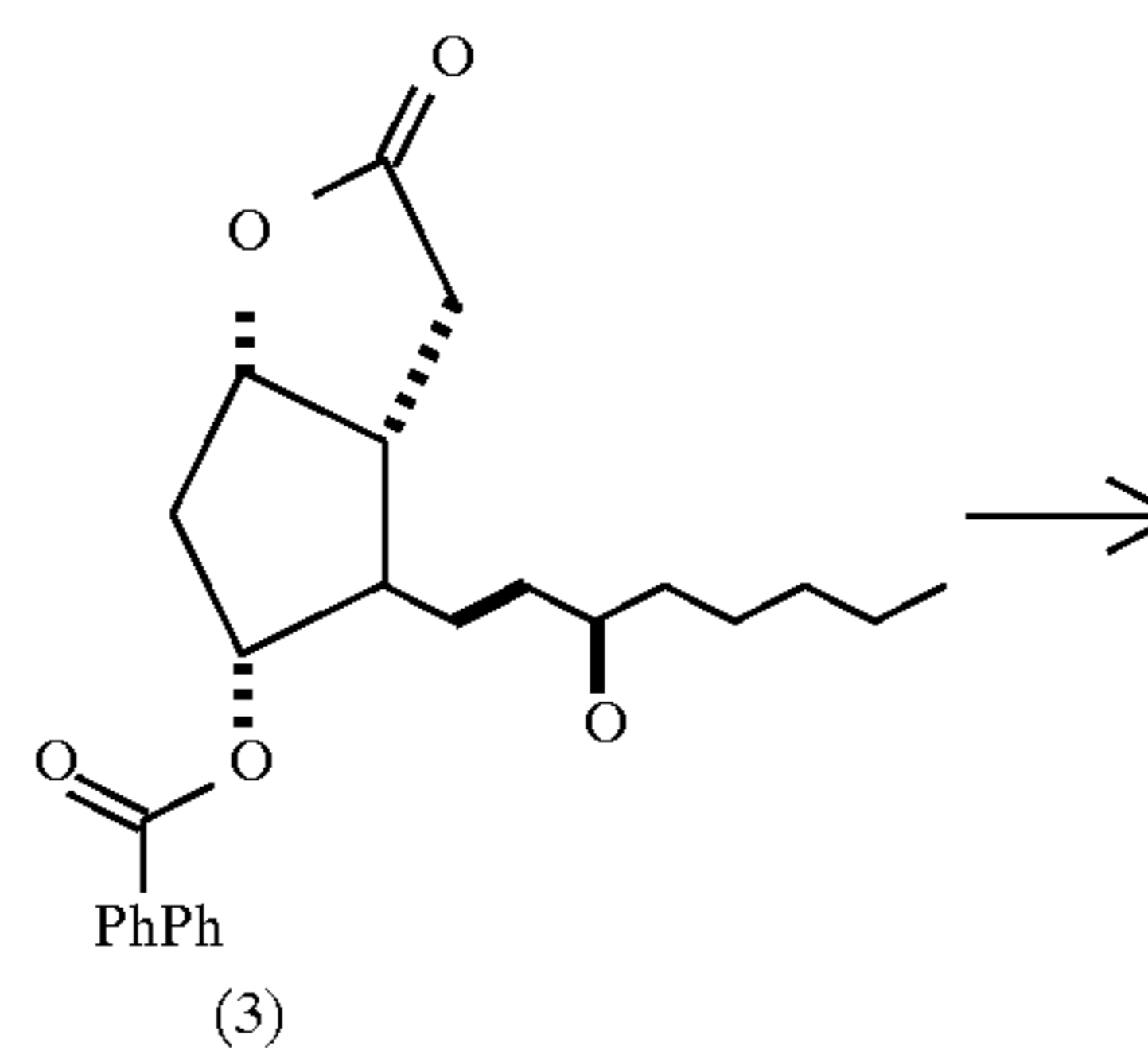
Synthetic scheme I
