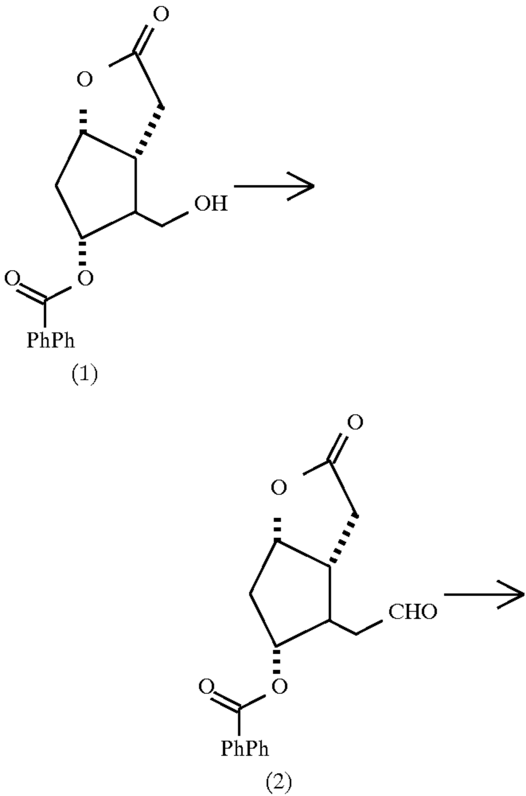
Synthetic scheme I
