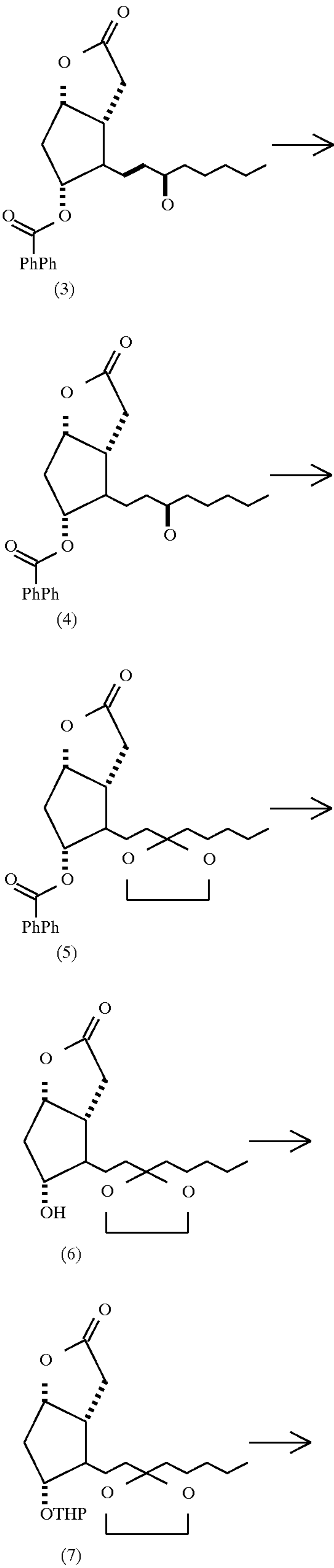
Synthetic scheme I
