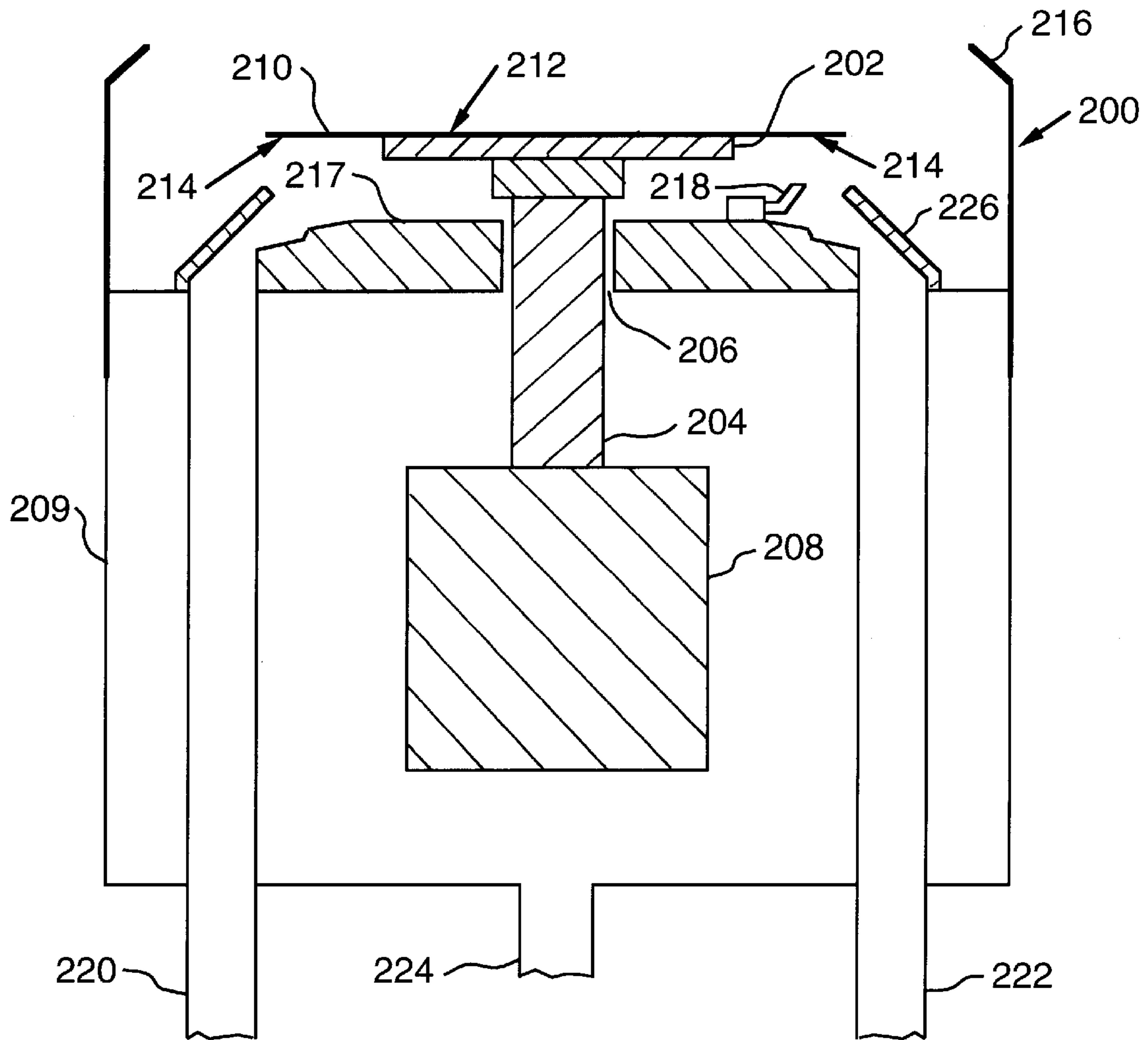
FIG. 1 Prior Art
