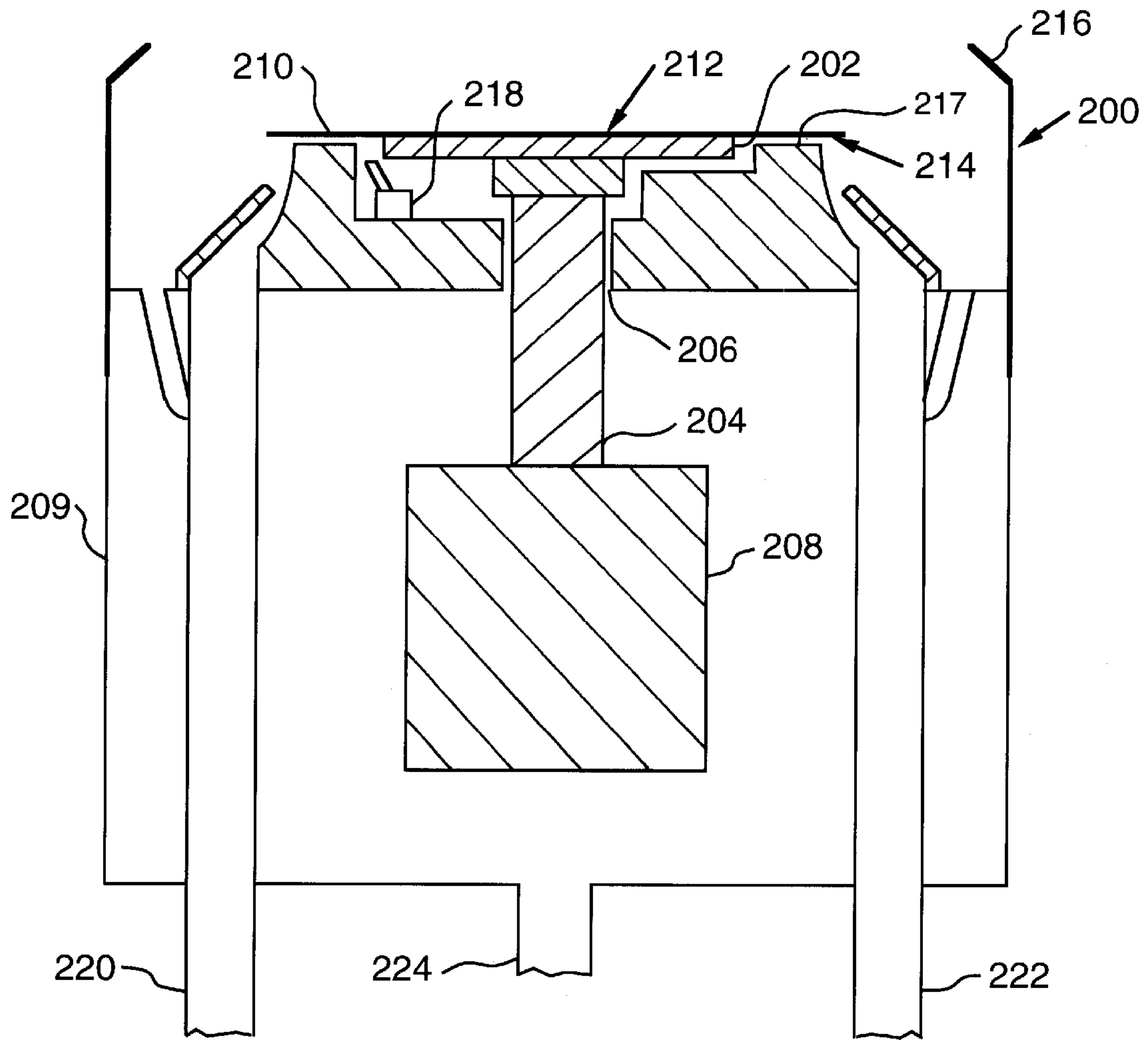
FIG. 2 Prior Art
