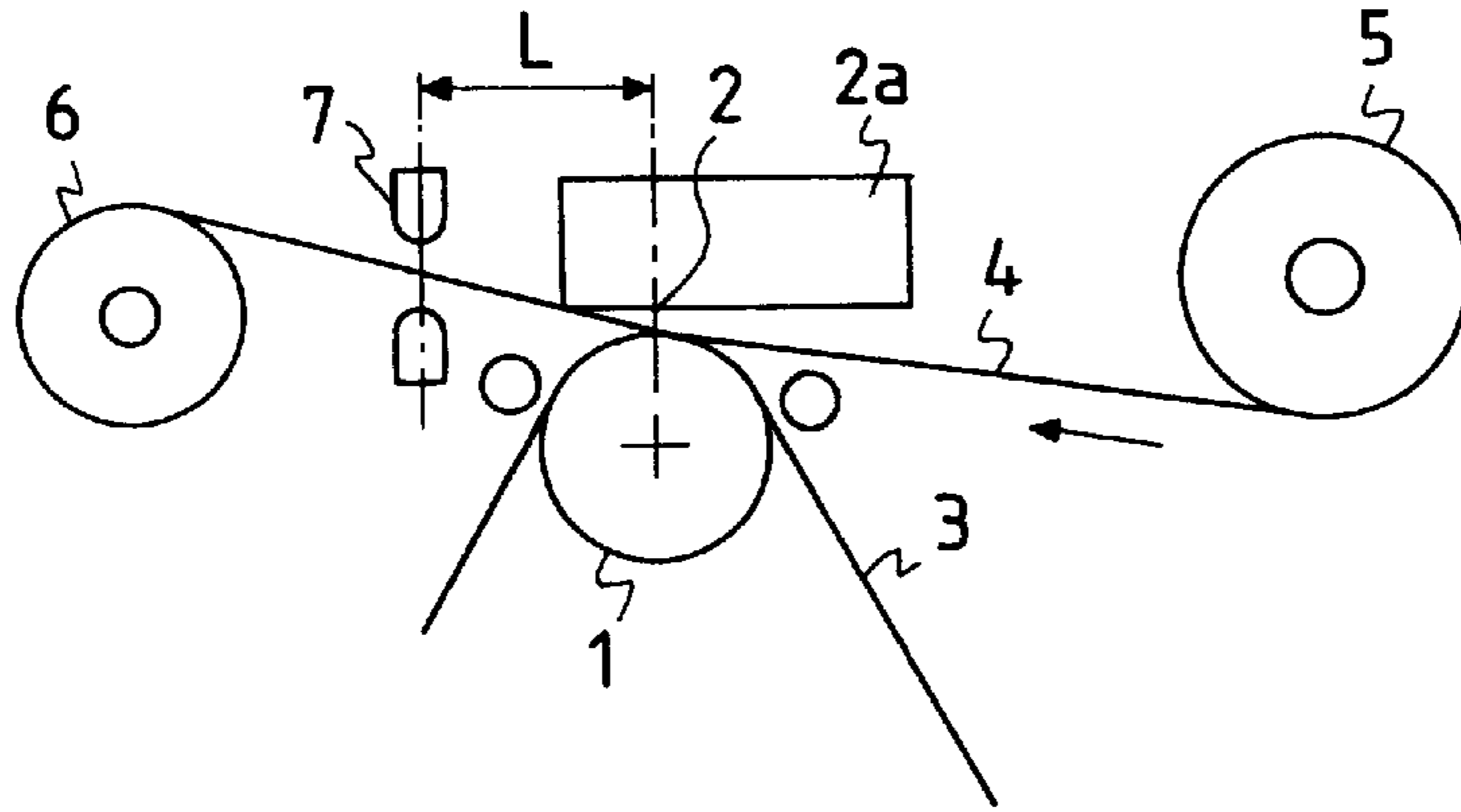
FIG. 13 PRIOR ART
