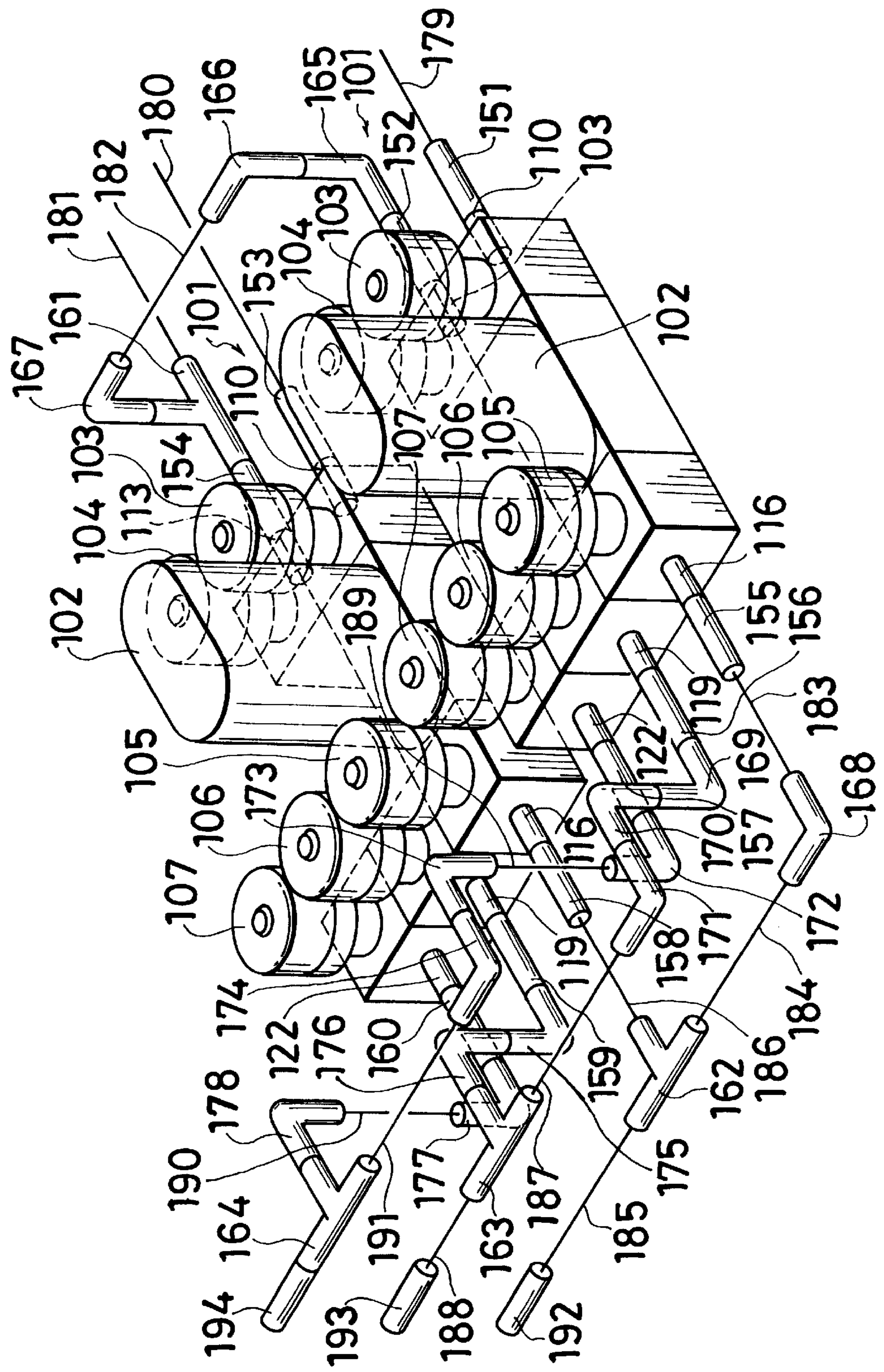
FIG. 7 PRIOR ART
