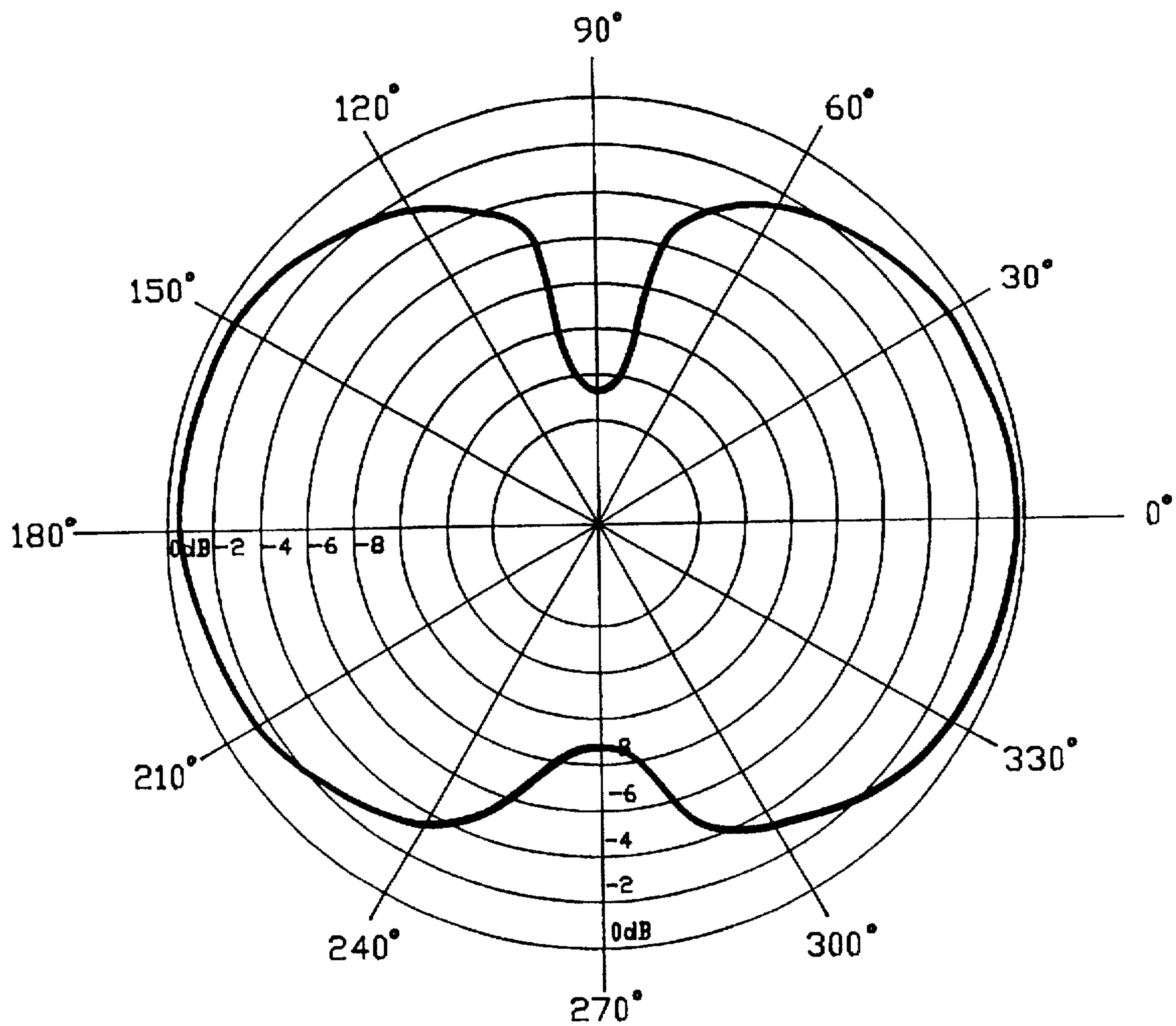
PATTERN NORMALIZED RELATIVE TO THE MAXIMUM GAIN (-3.5dBd) OF 433 MHz ANTENNA
