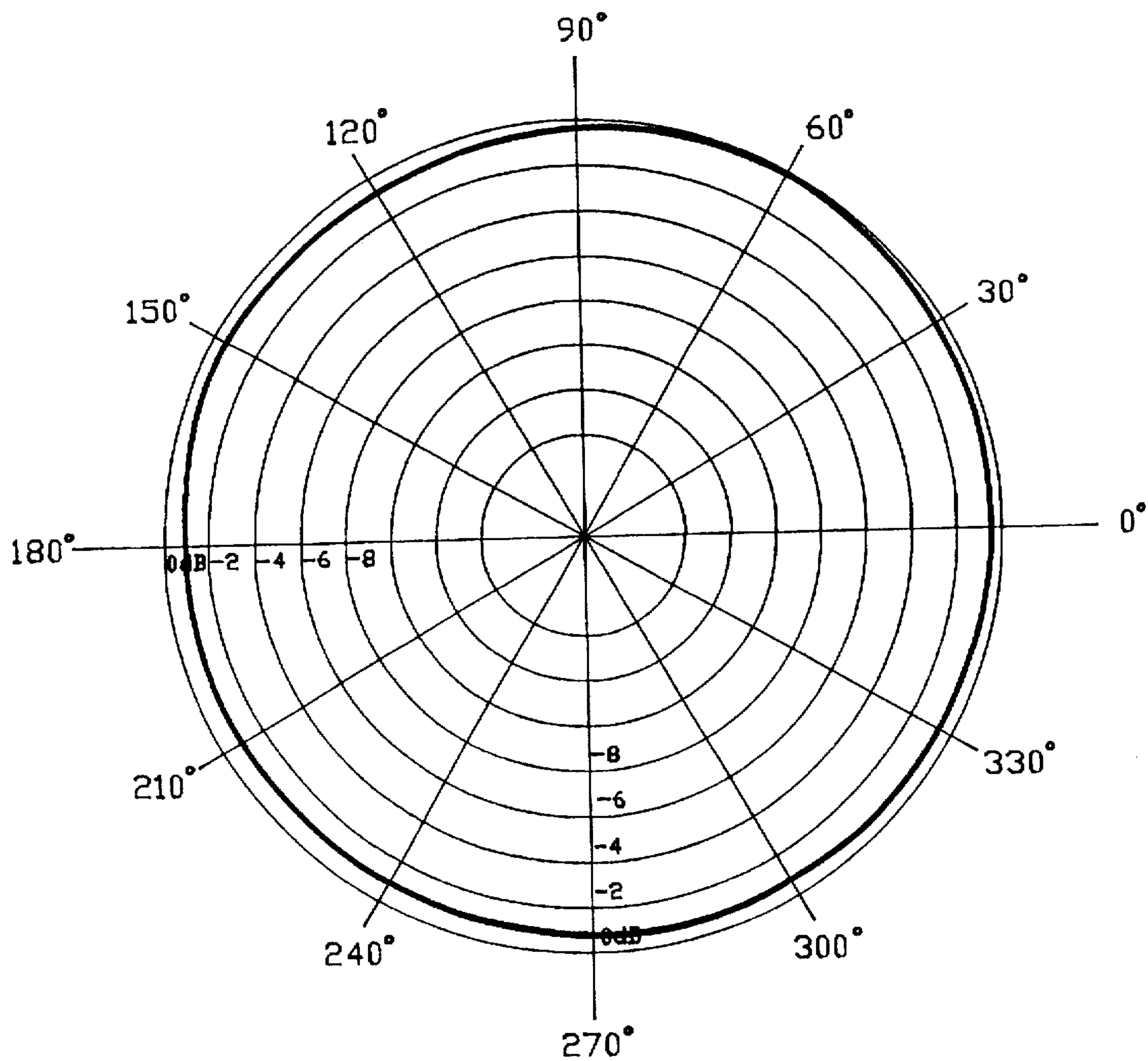
PATTERN NORMALIZED RELATIVE TO THE MAXIMUM GAIN OF 315 MHz ANTENNA
