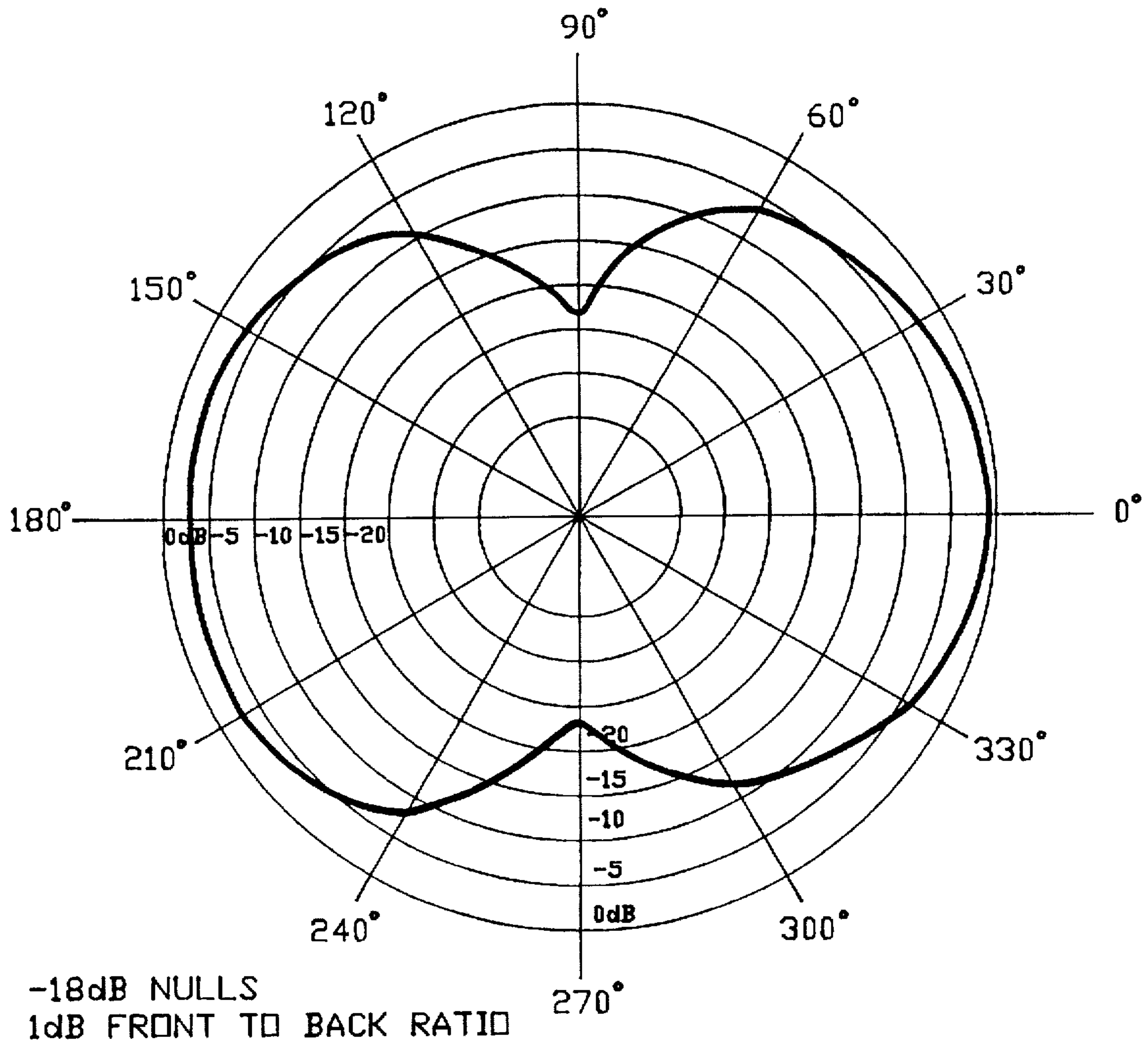
PATTERN NORMALIZED RELATIVE TO THE MAXIMUM GAIN (-6.5dBd) OF 315 MHz ANTENNA
