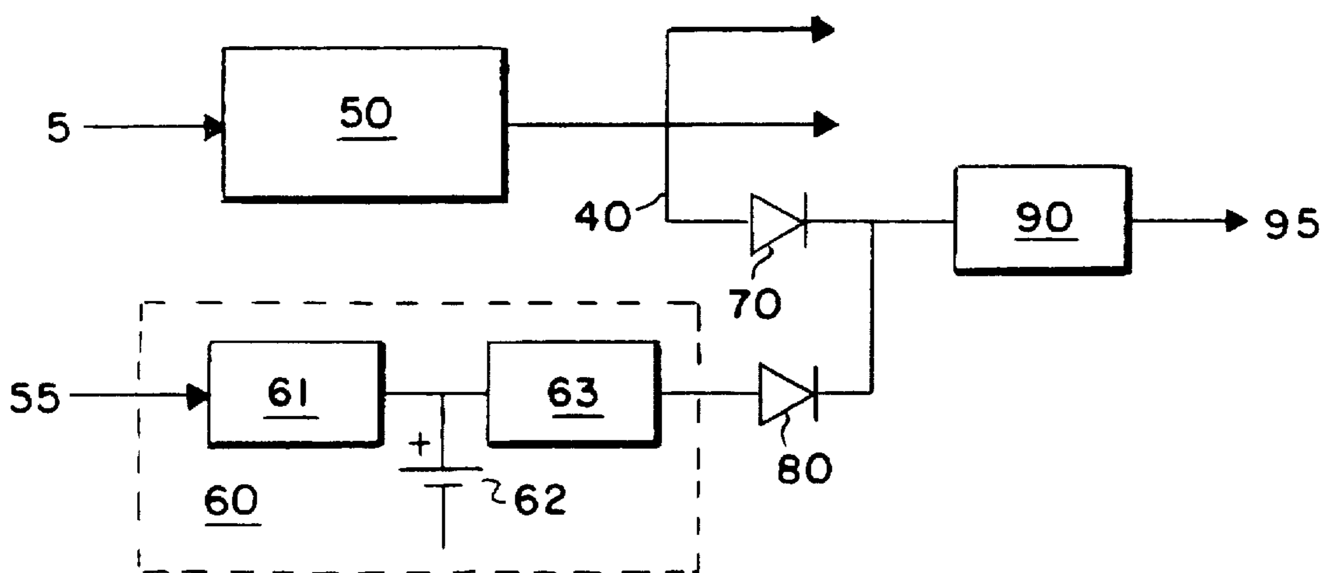
FIG. 2 PRIOR ART
