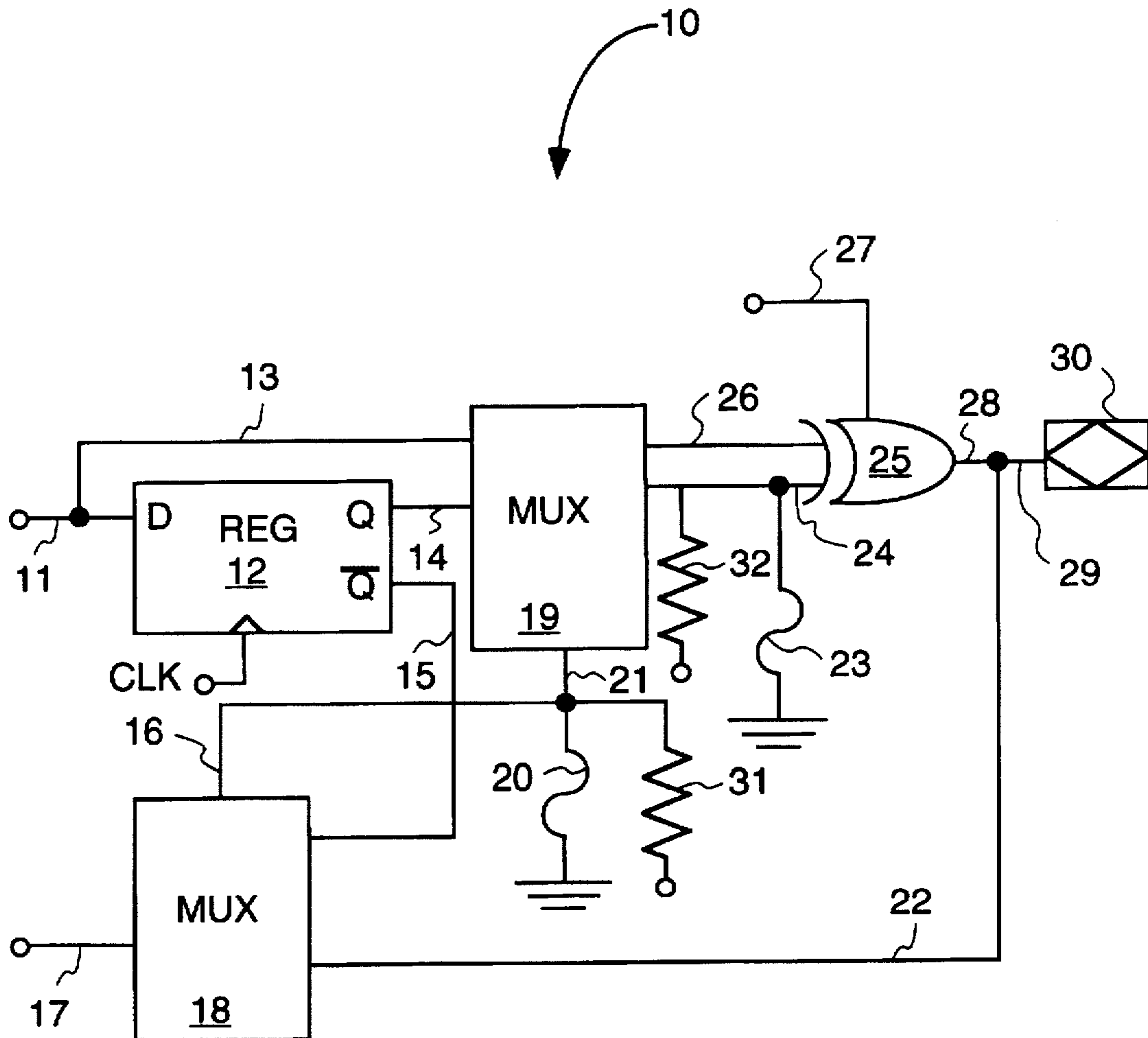
FIG. 1 PRIOR ART
