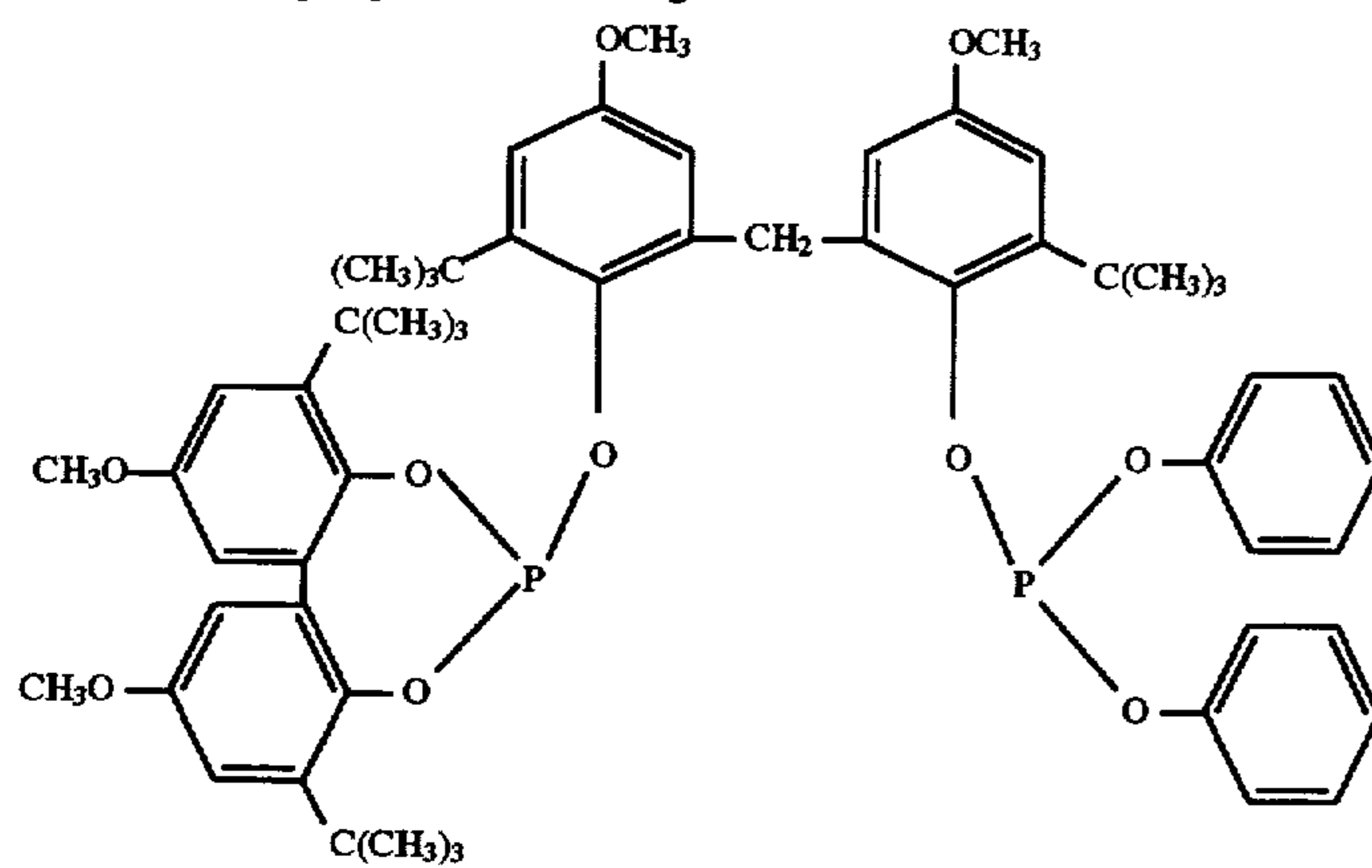
Ligand R
