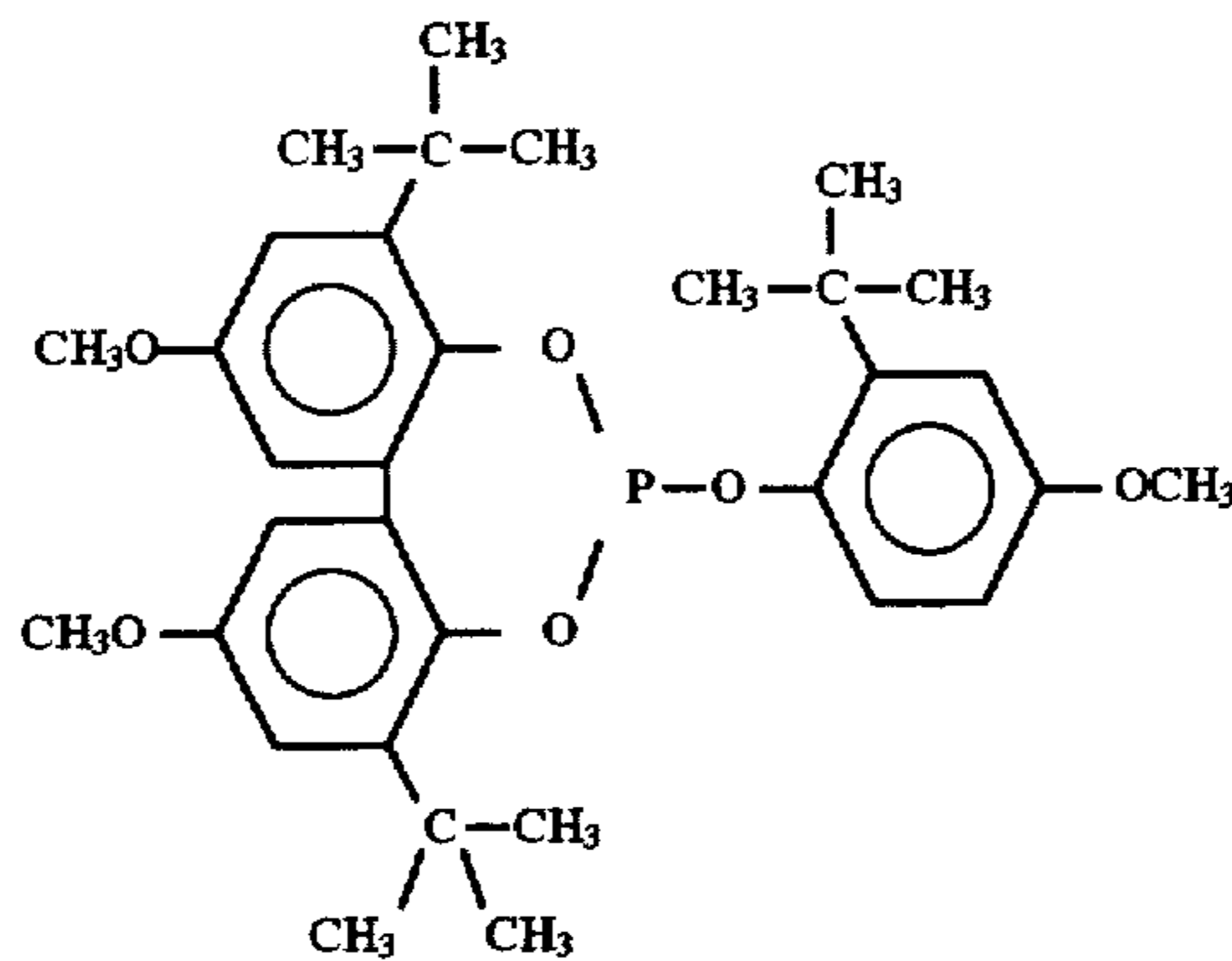
Ligand A
