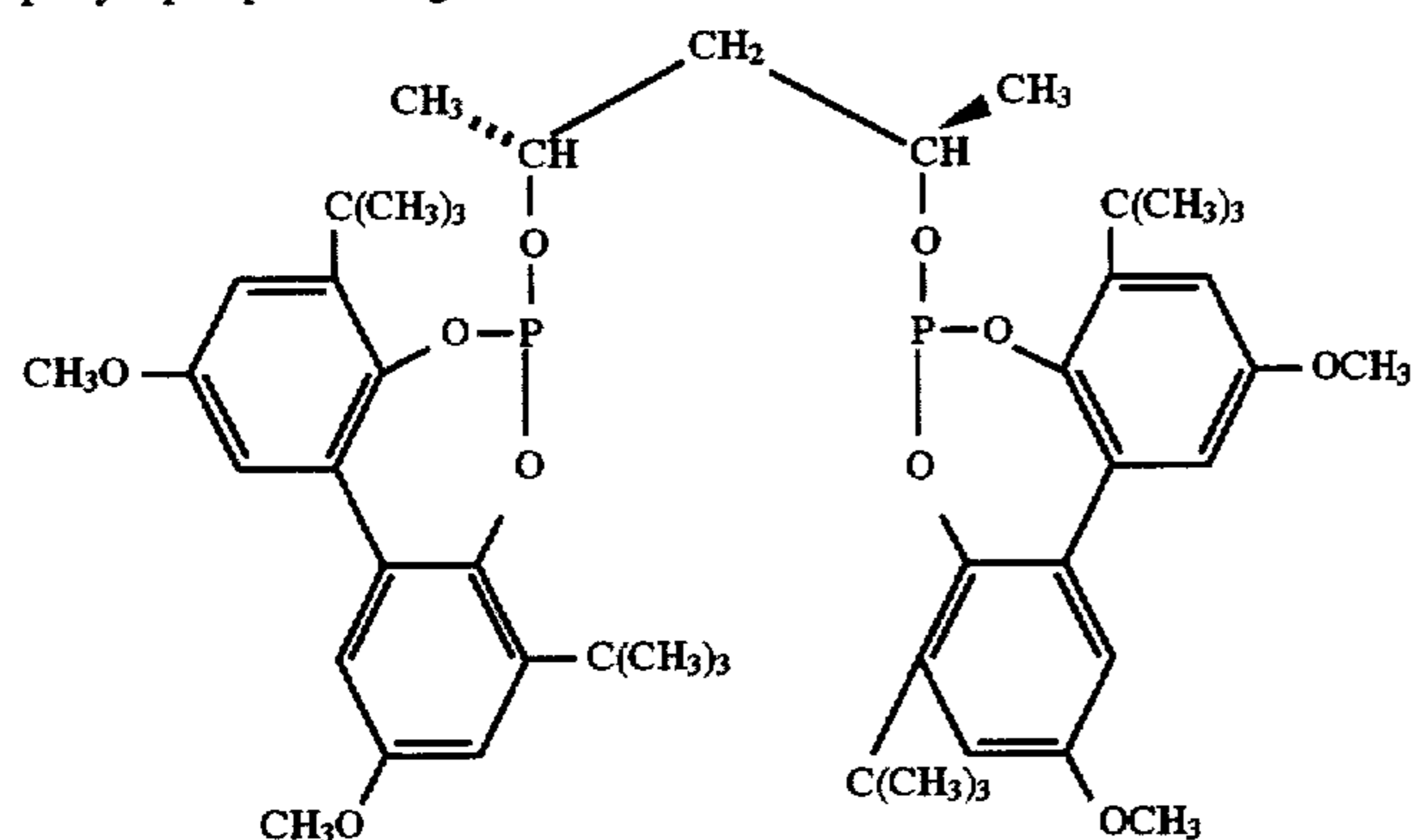
Ligand M
