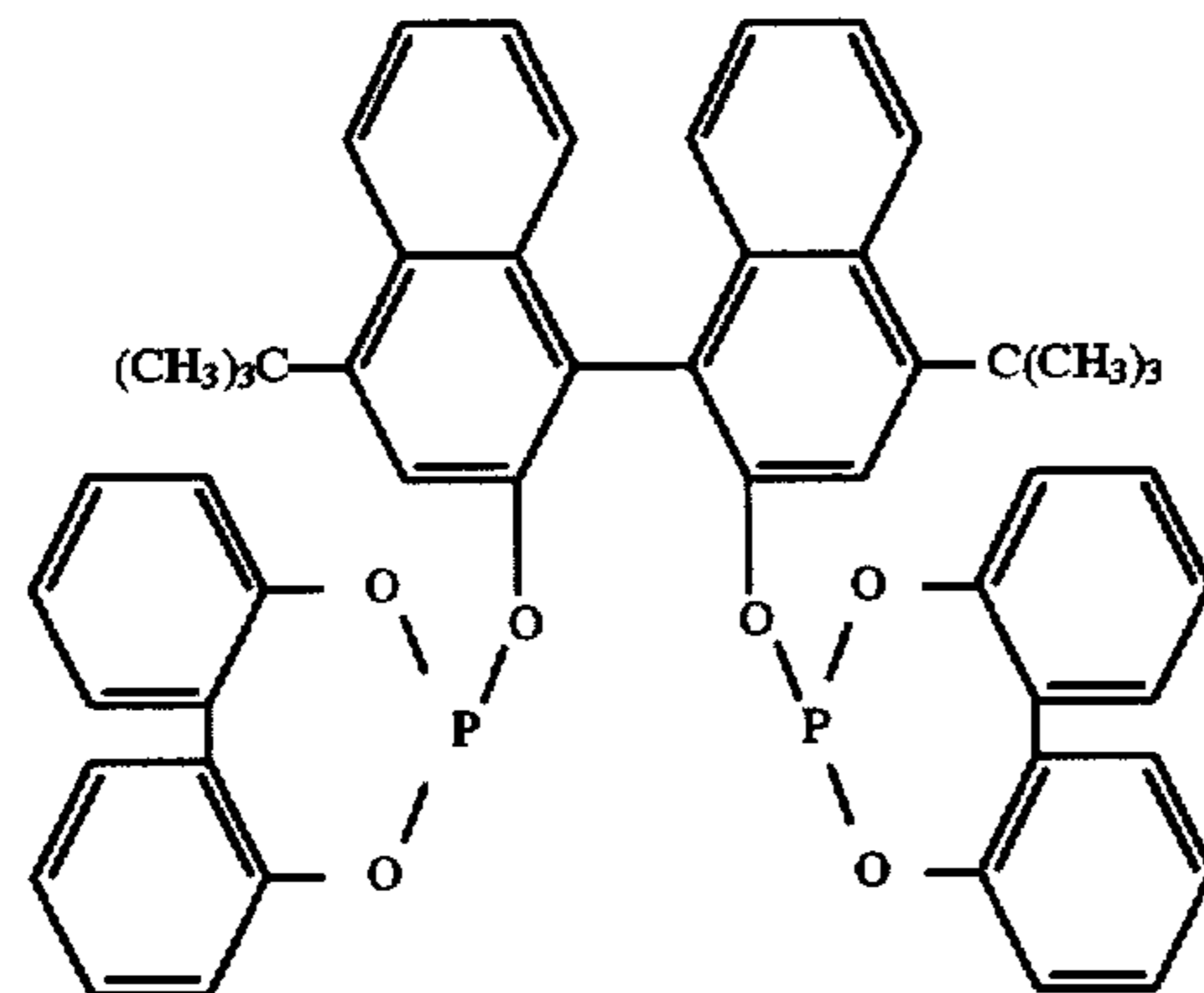
Ligand C
