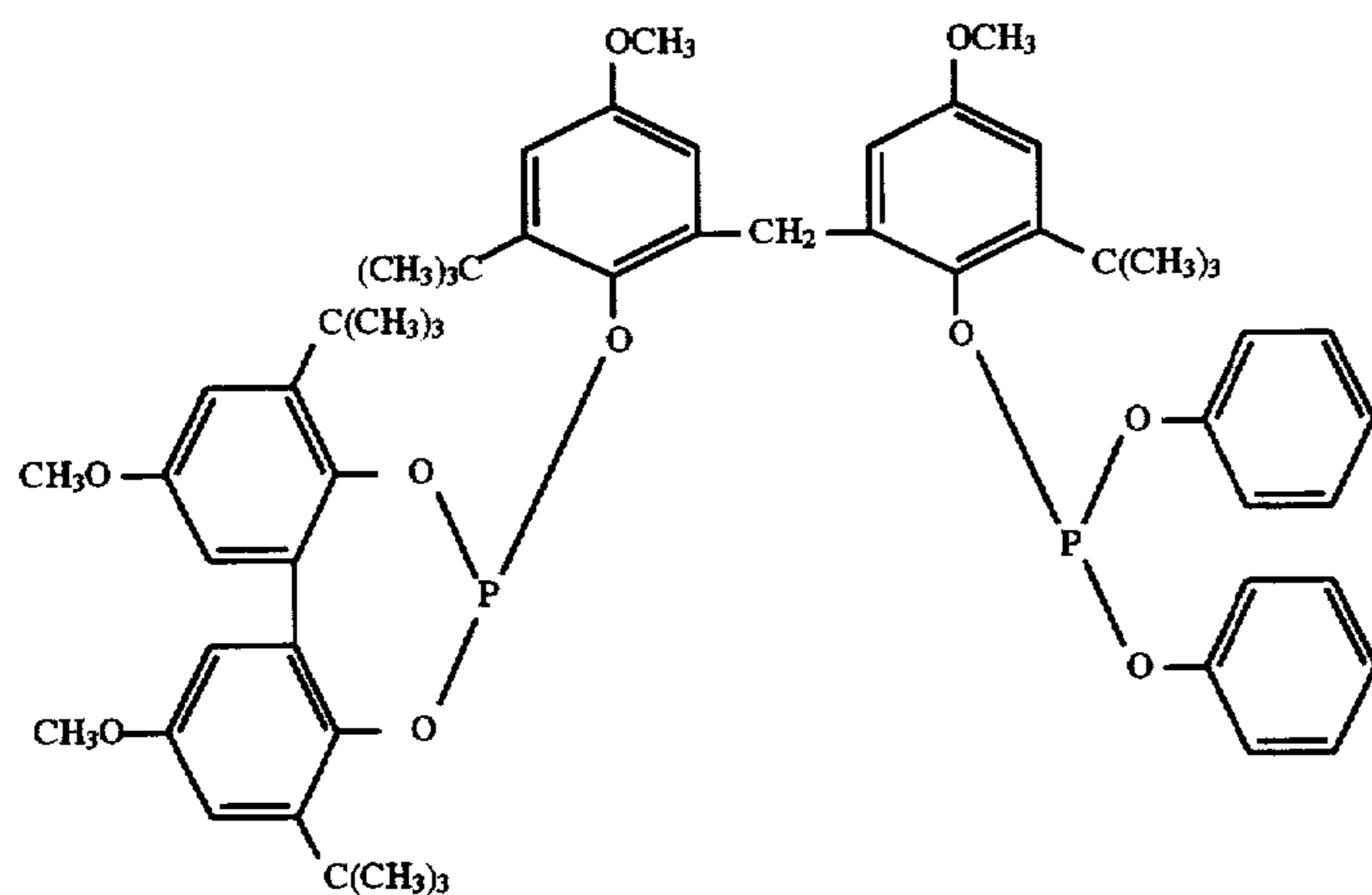
Ligand R
