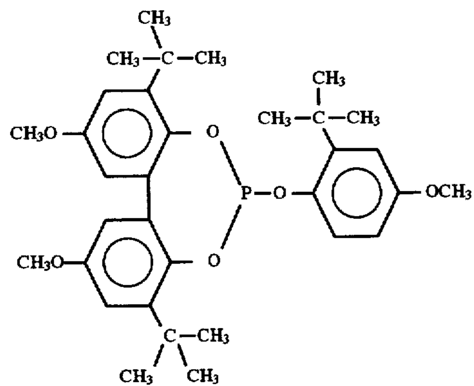
Ligand A
