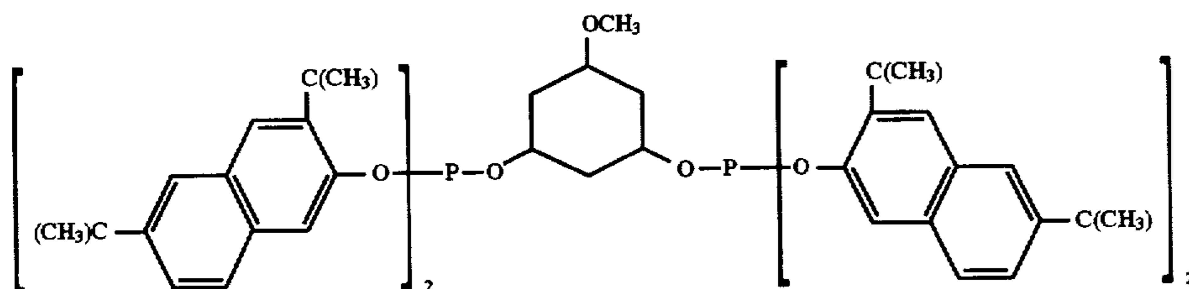
Ligand S
