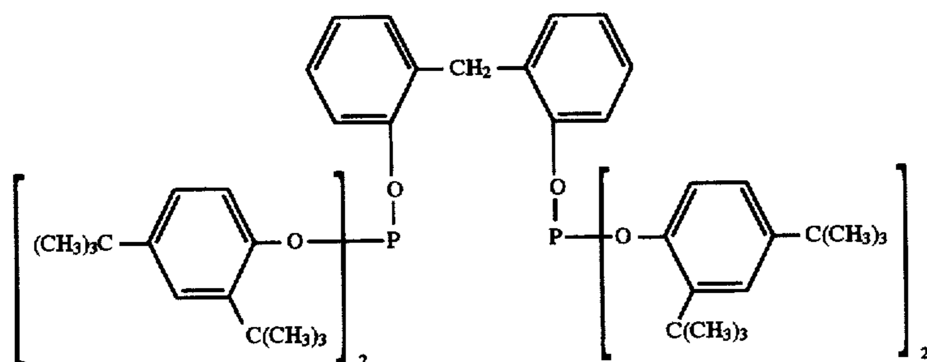
Ligand U
