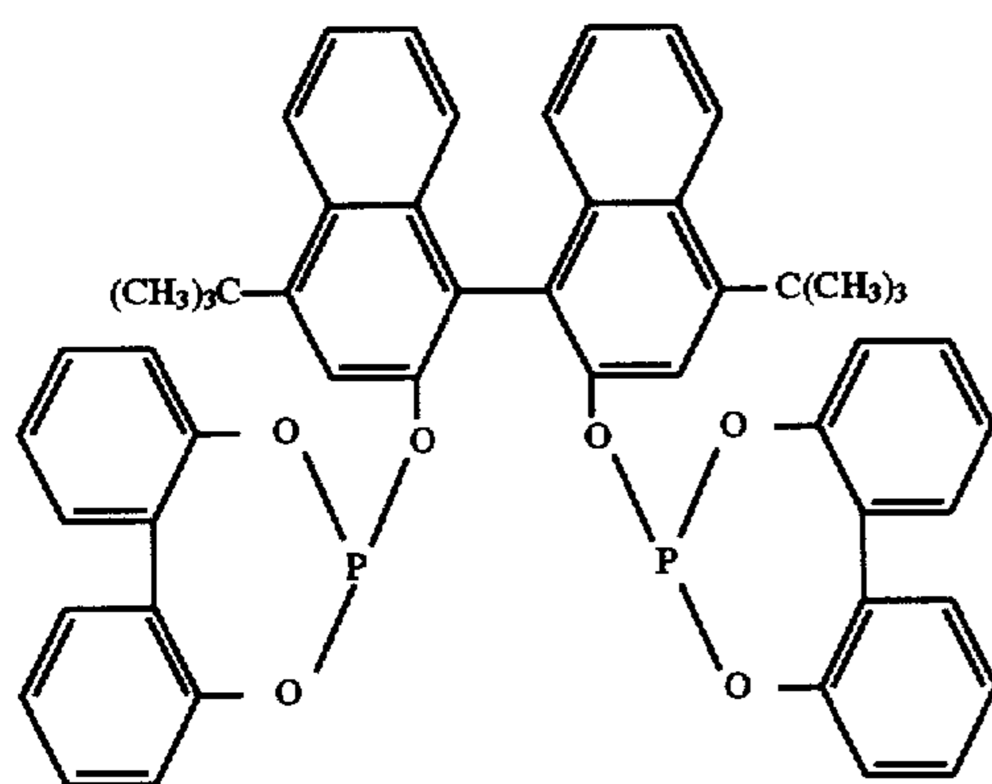
Ligand C
