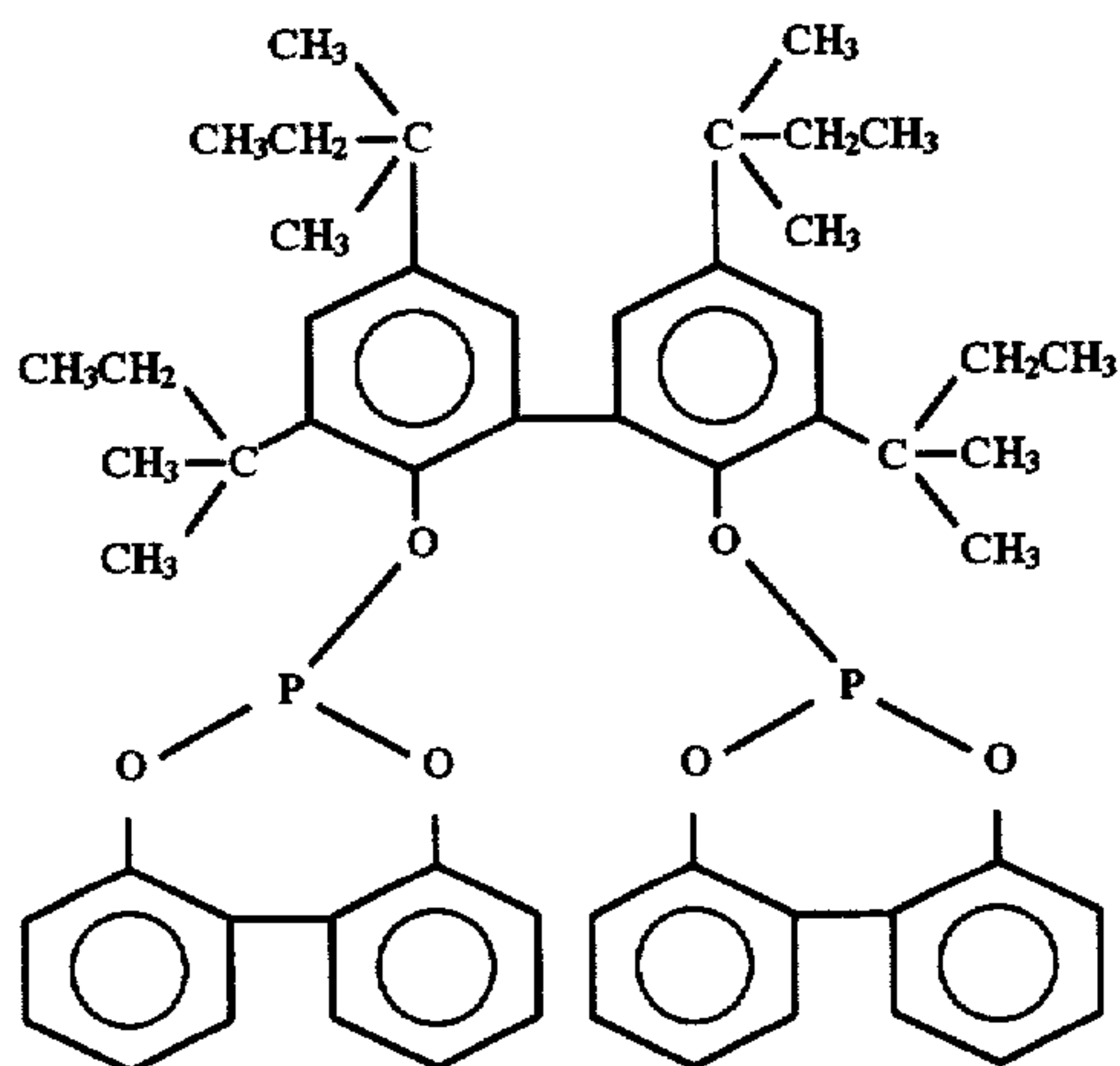
Ligand C
