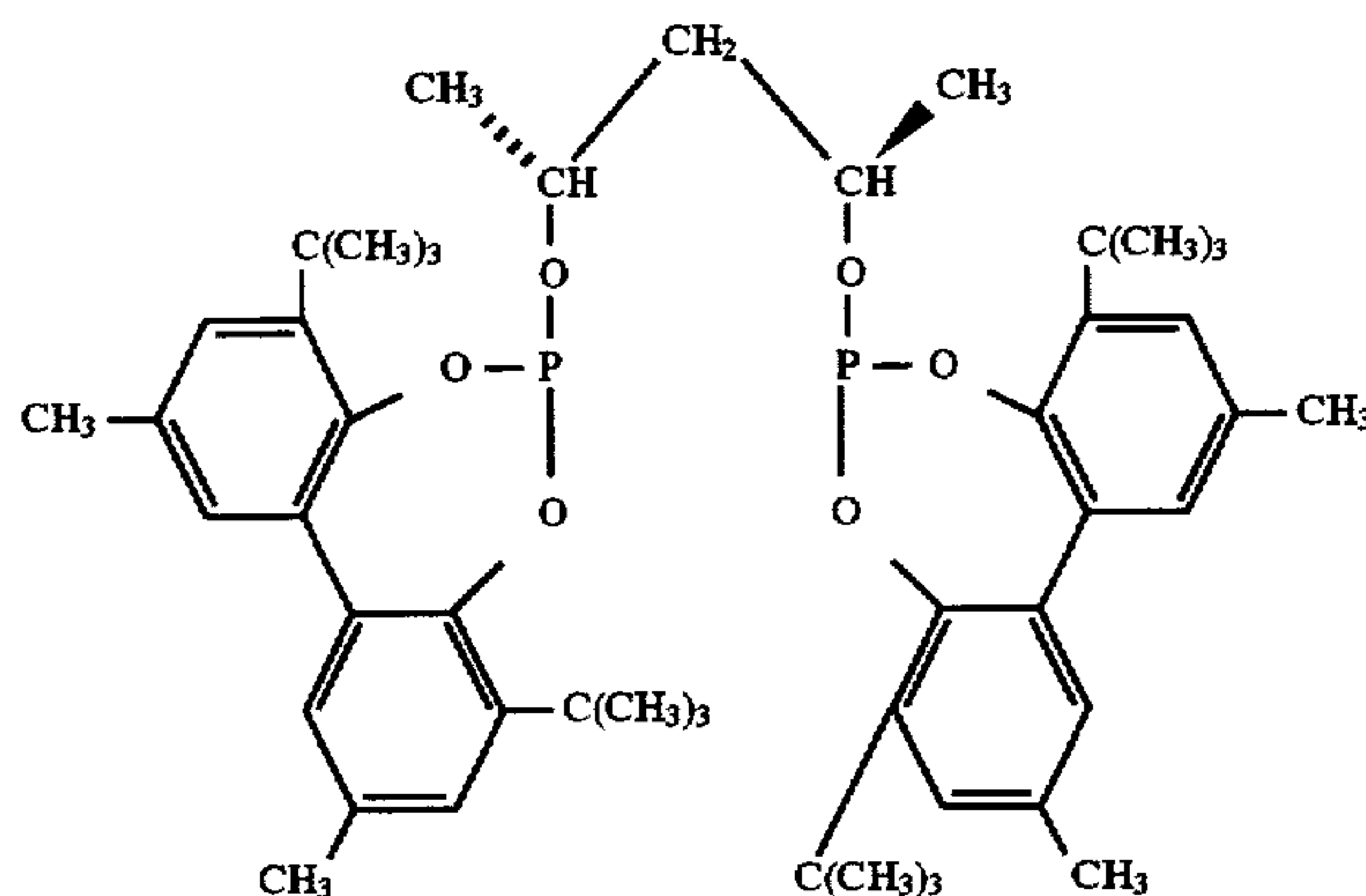
Ligand H
