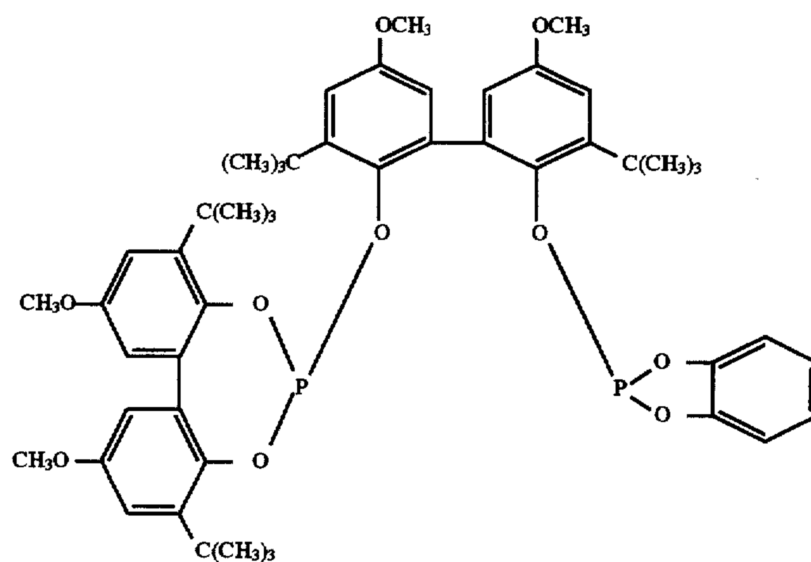
Ligand M
