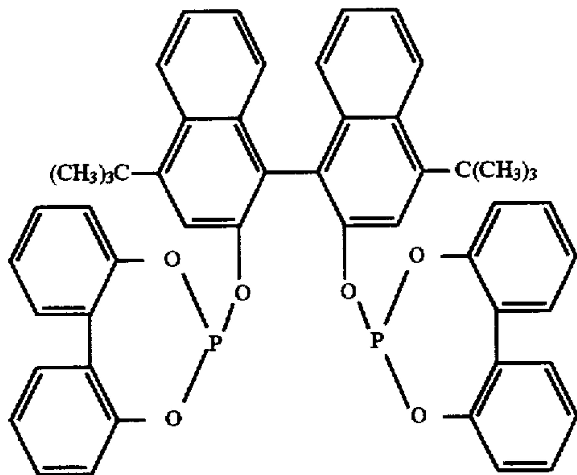
Ligand A
