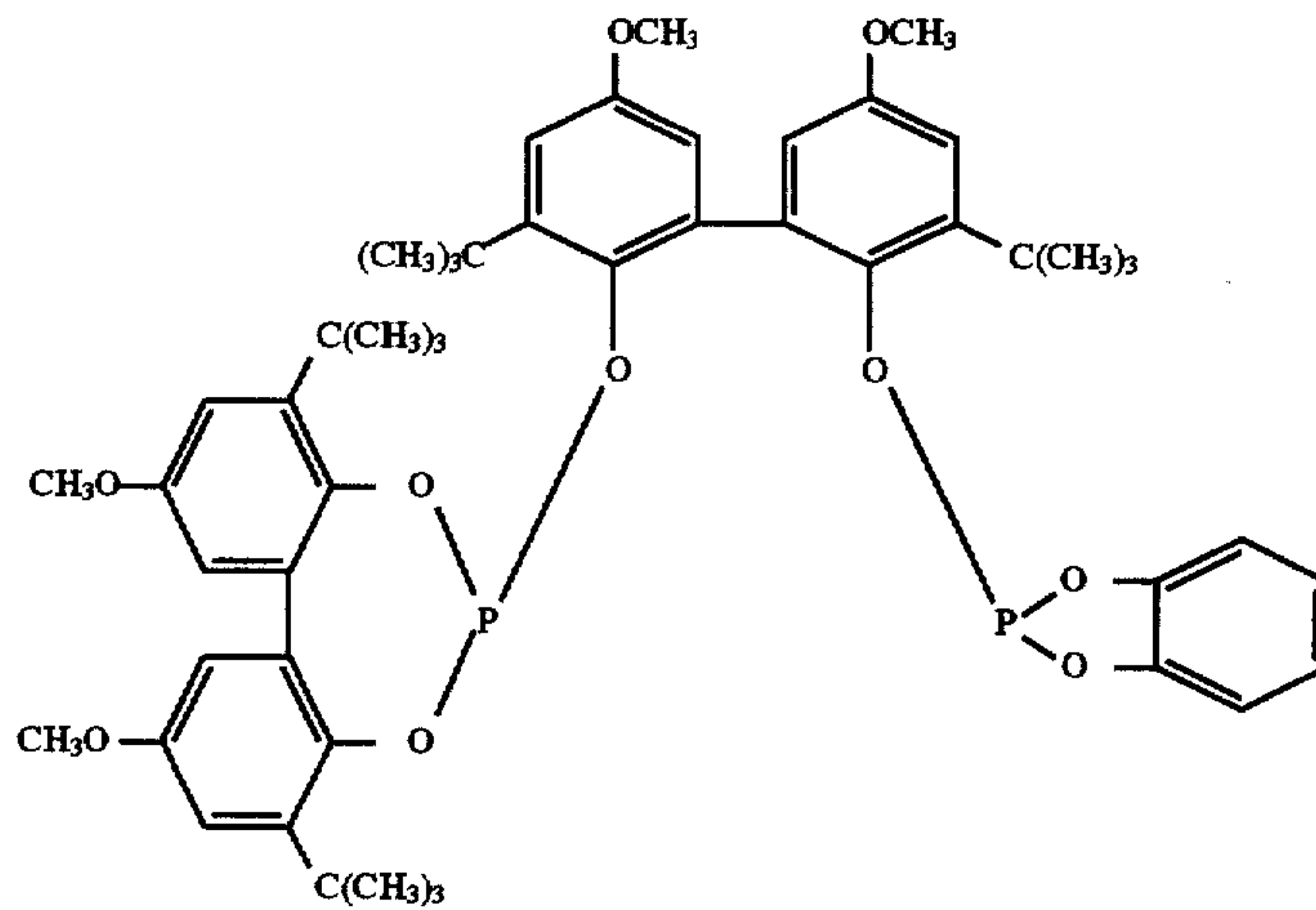
Ligand M
