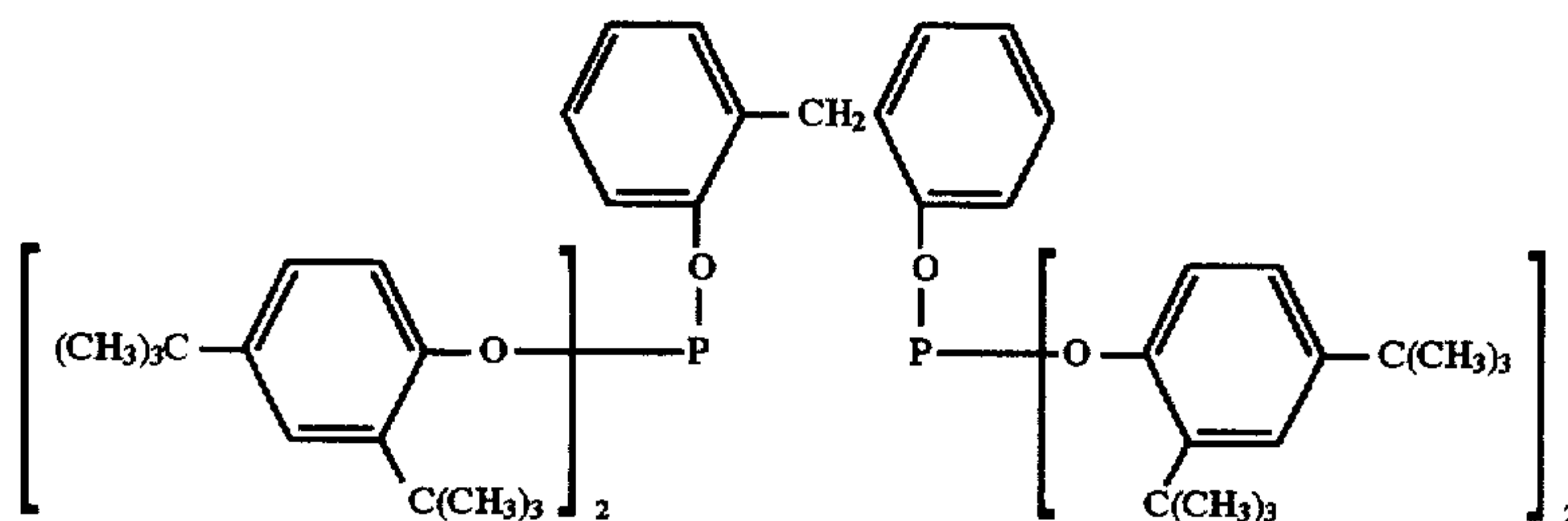
Ligand S
