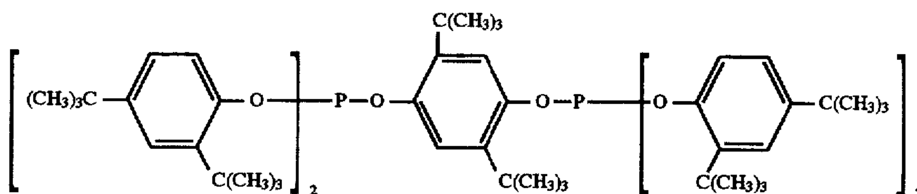
Ligand R
