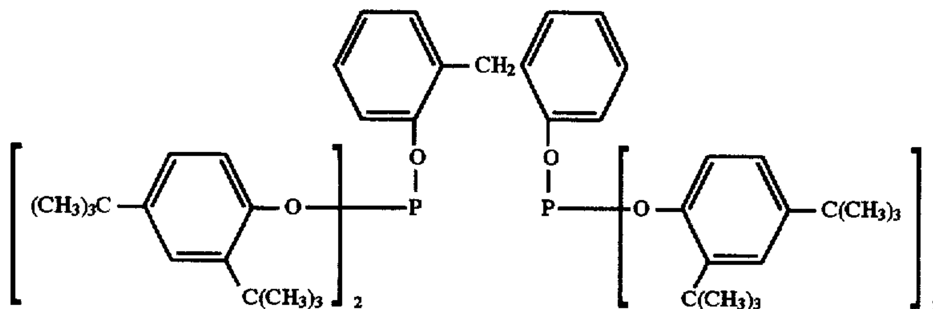
Ligand S
