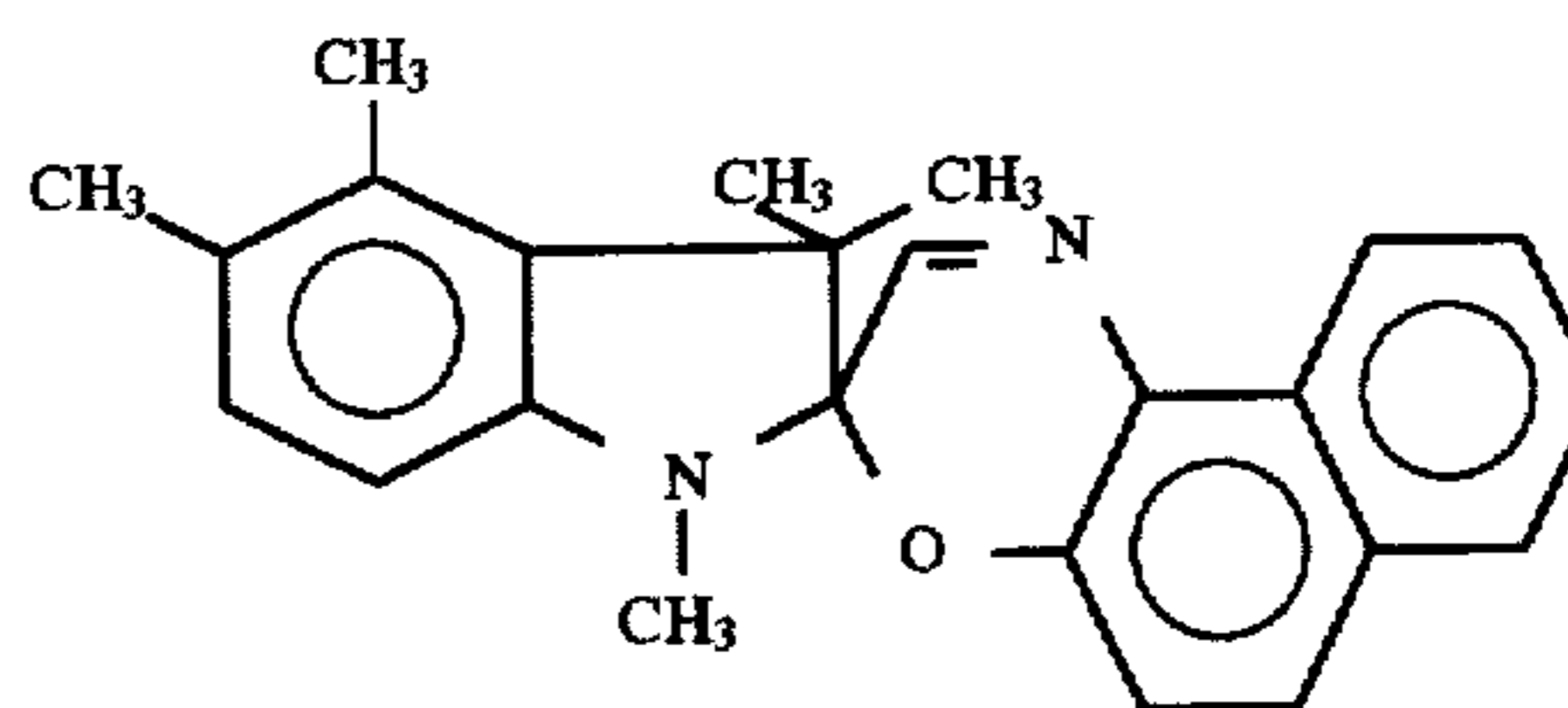
1,3,3,5,6-pentamethylspiro(indolino-2,3'-[3H]naphtho(2,1b)-(1,4)oxazine)
