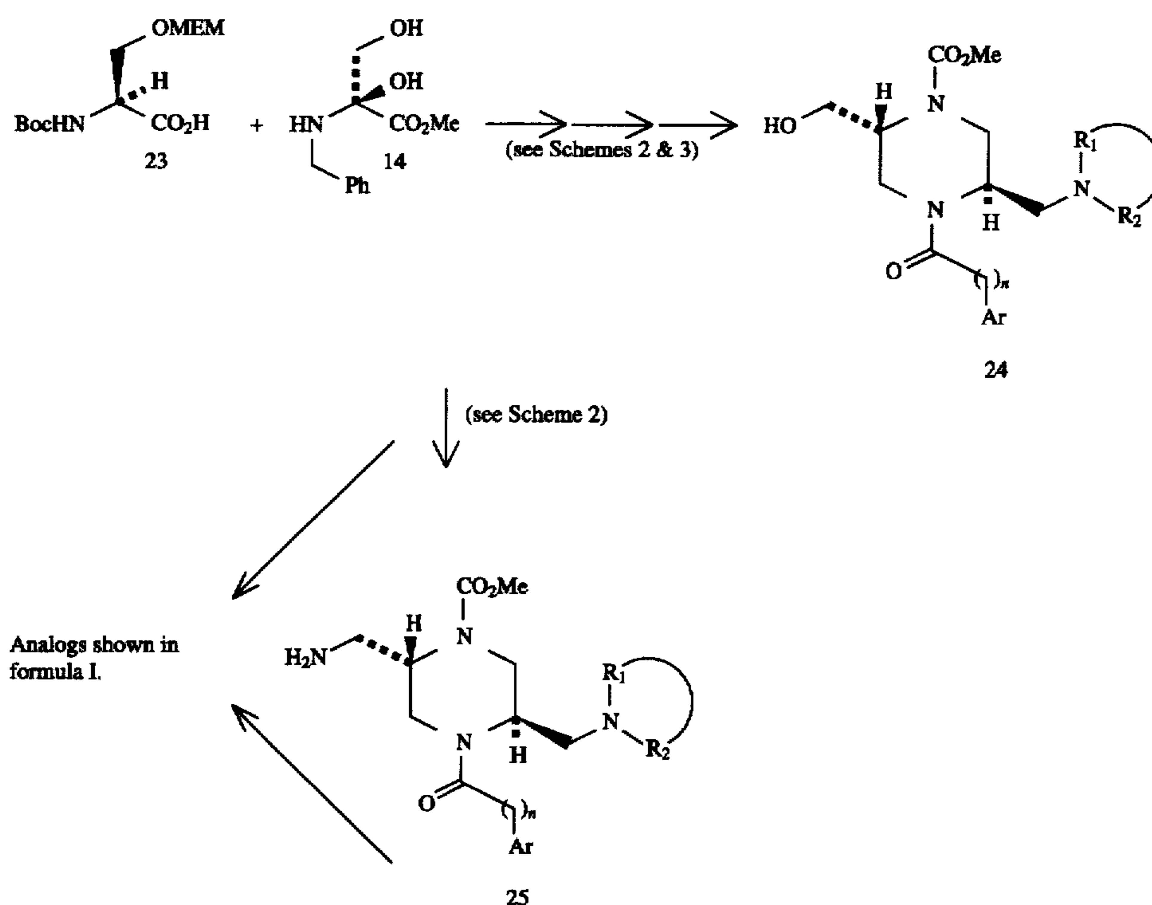
Scheme 4.
