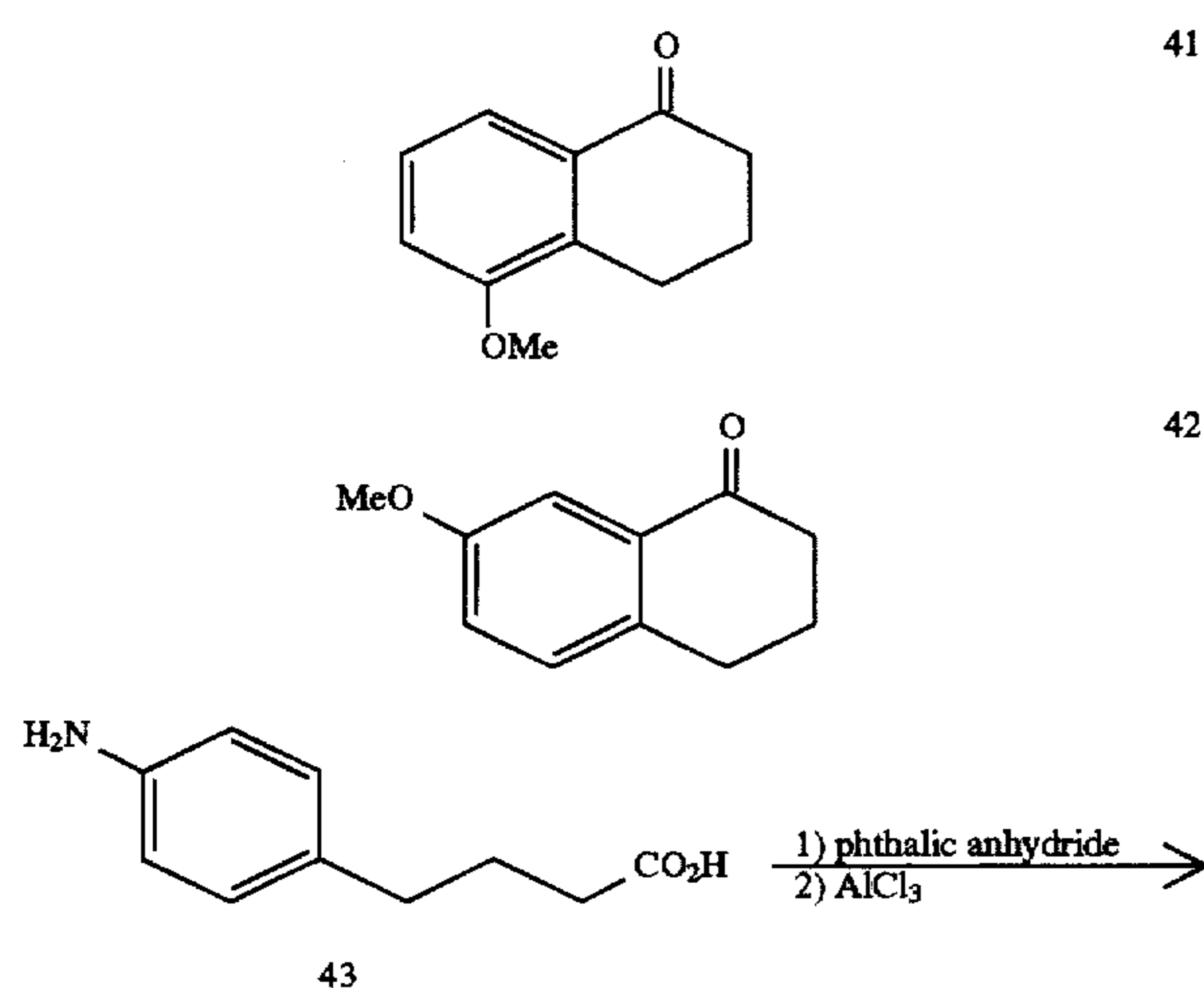
Scheme 5.
