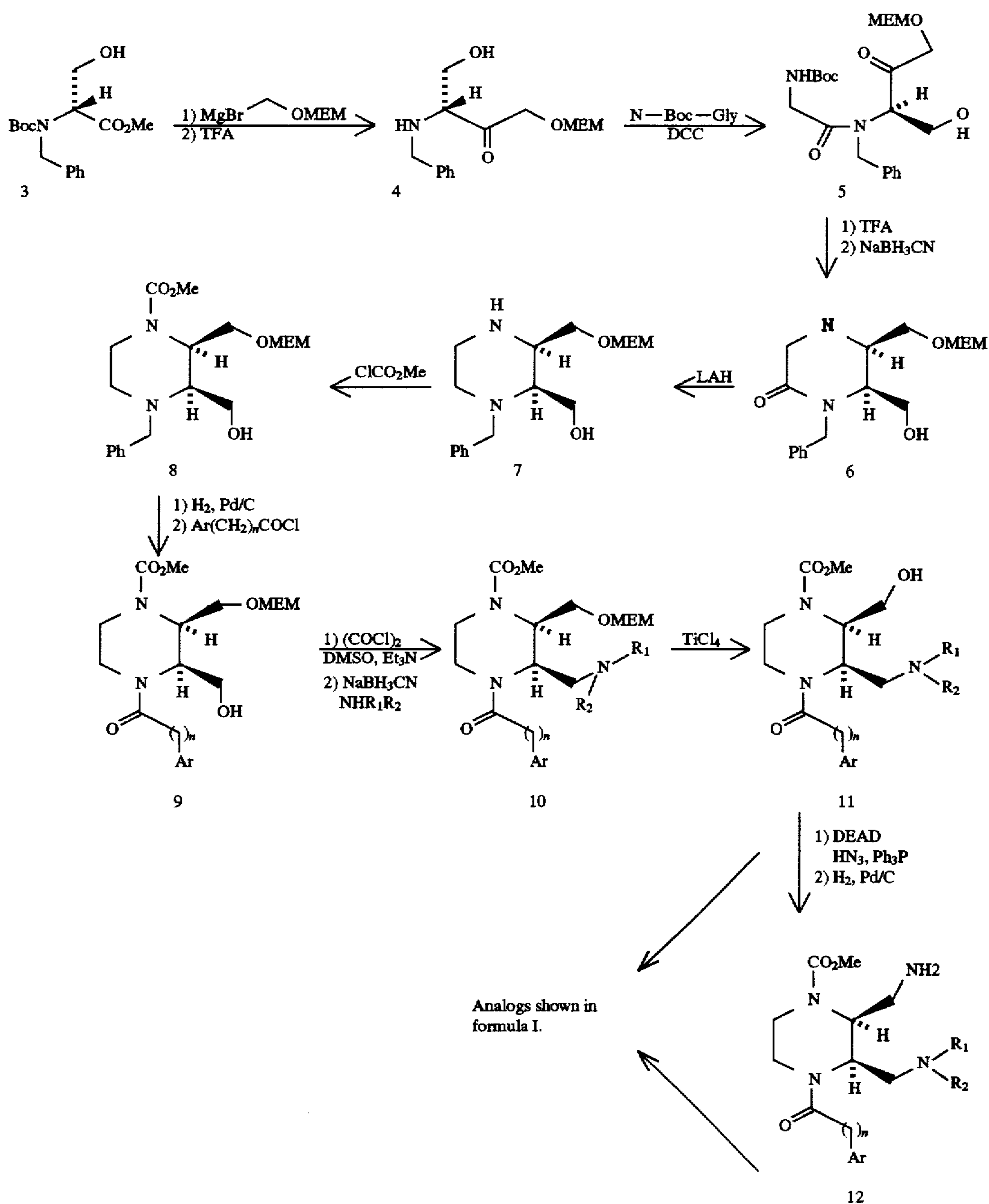
Scheme 2.
