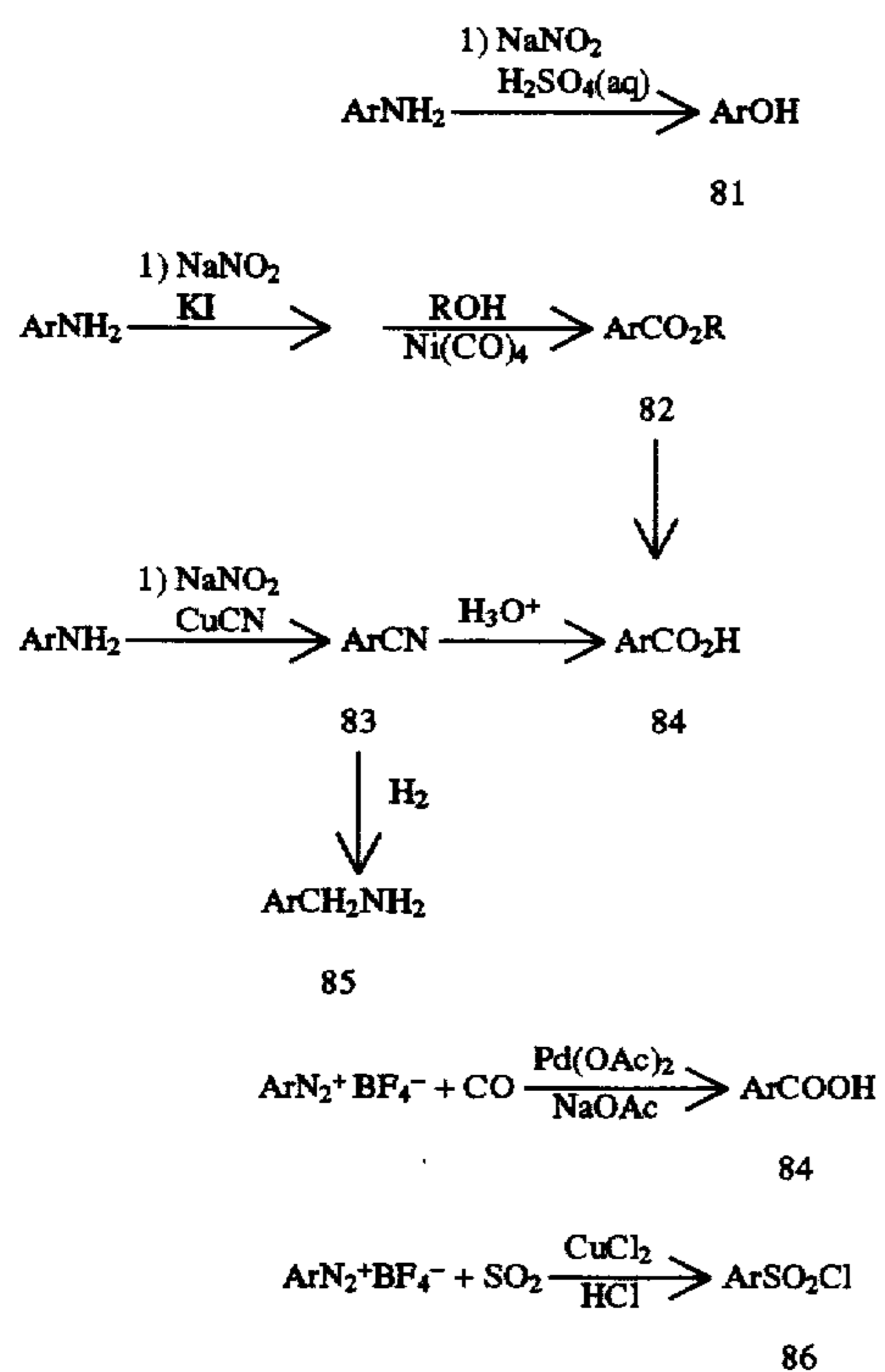
Scheme 7.
