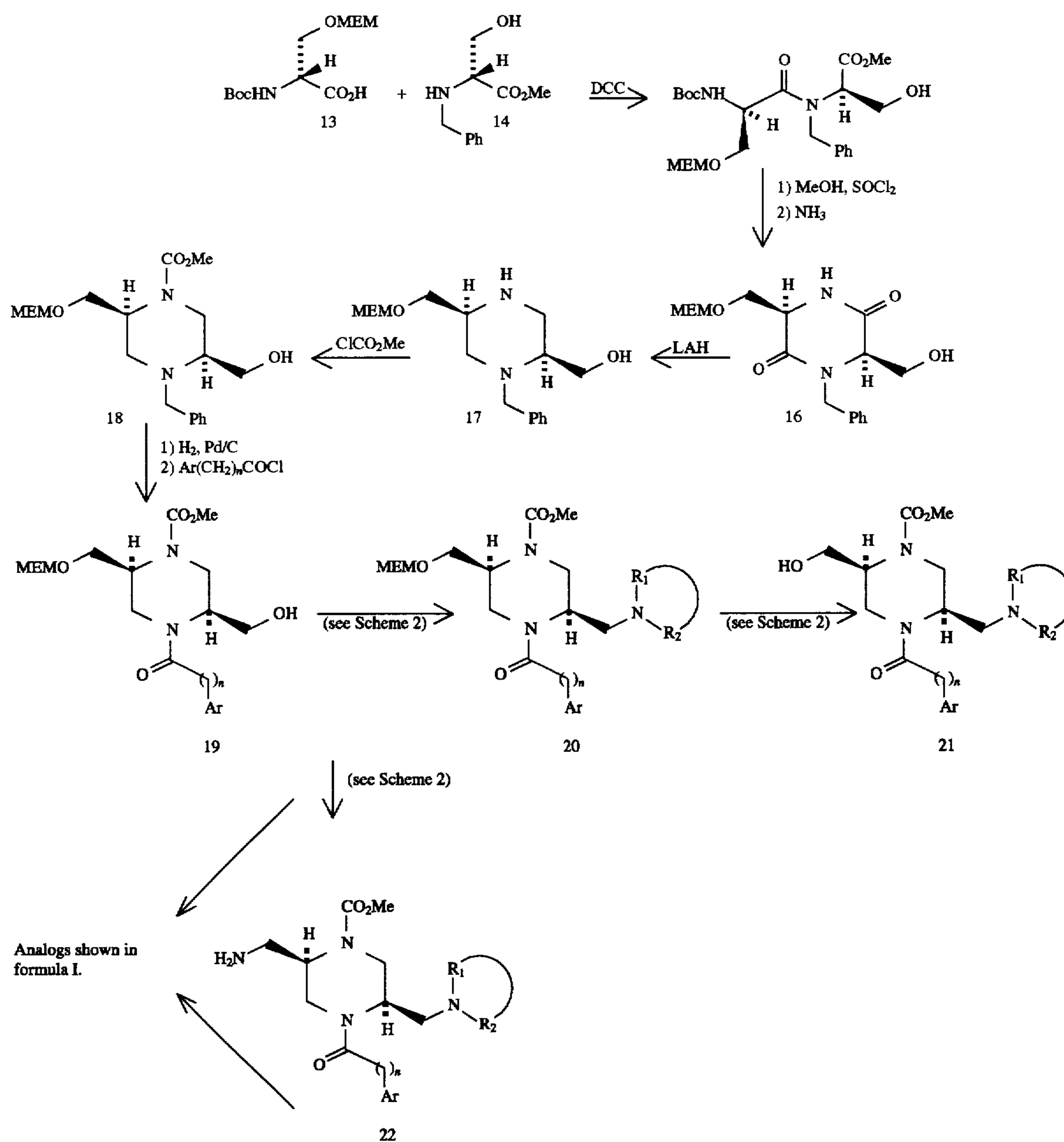
SCHEME 3.
