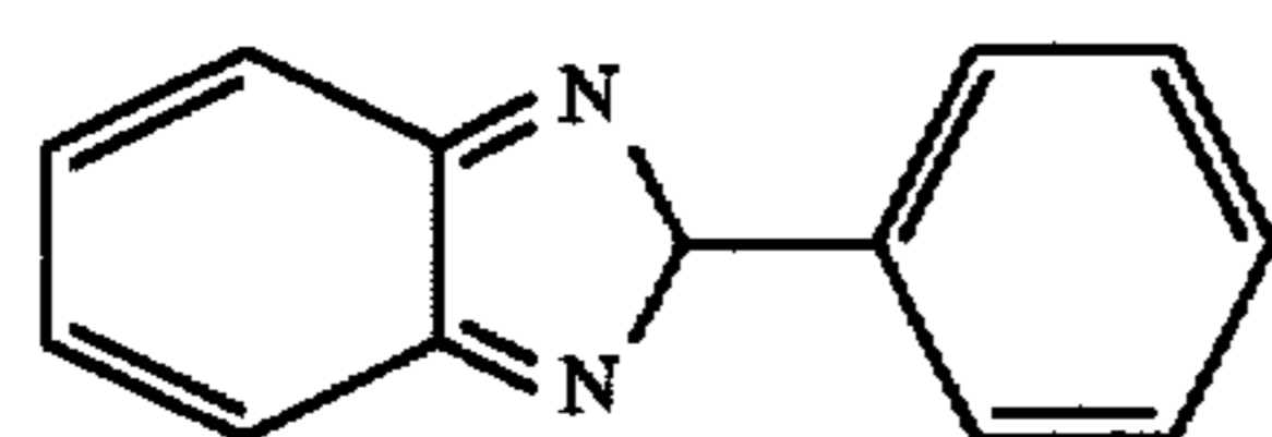
Phenylbenzimidazole
