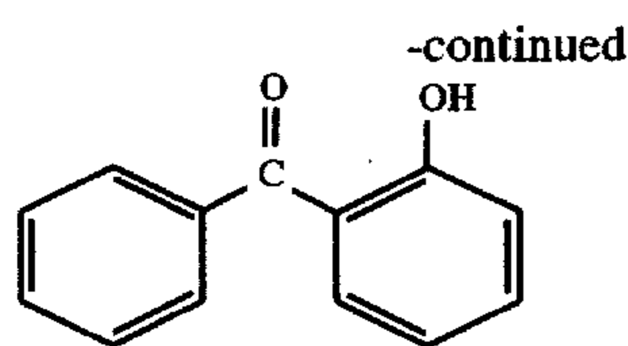
2-Hydroxybenzophenone
