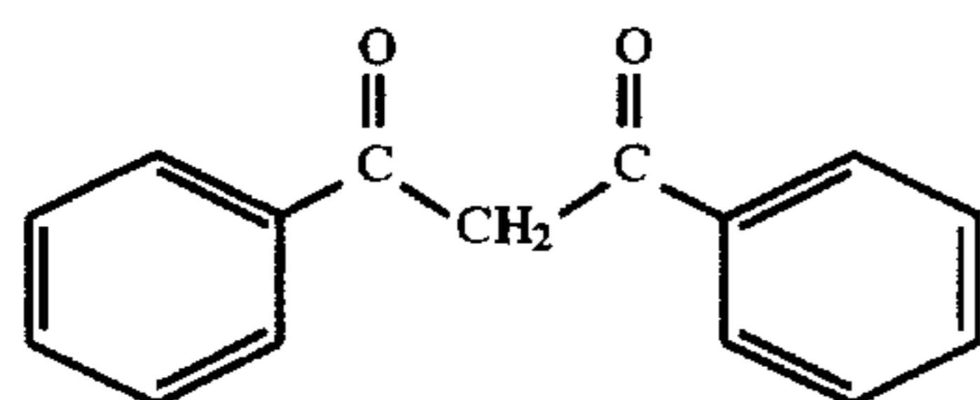
Dibenzoylmethane
