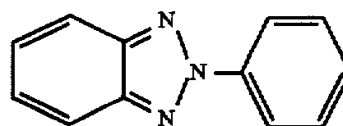
Phenylbenzotriazole
