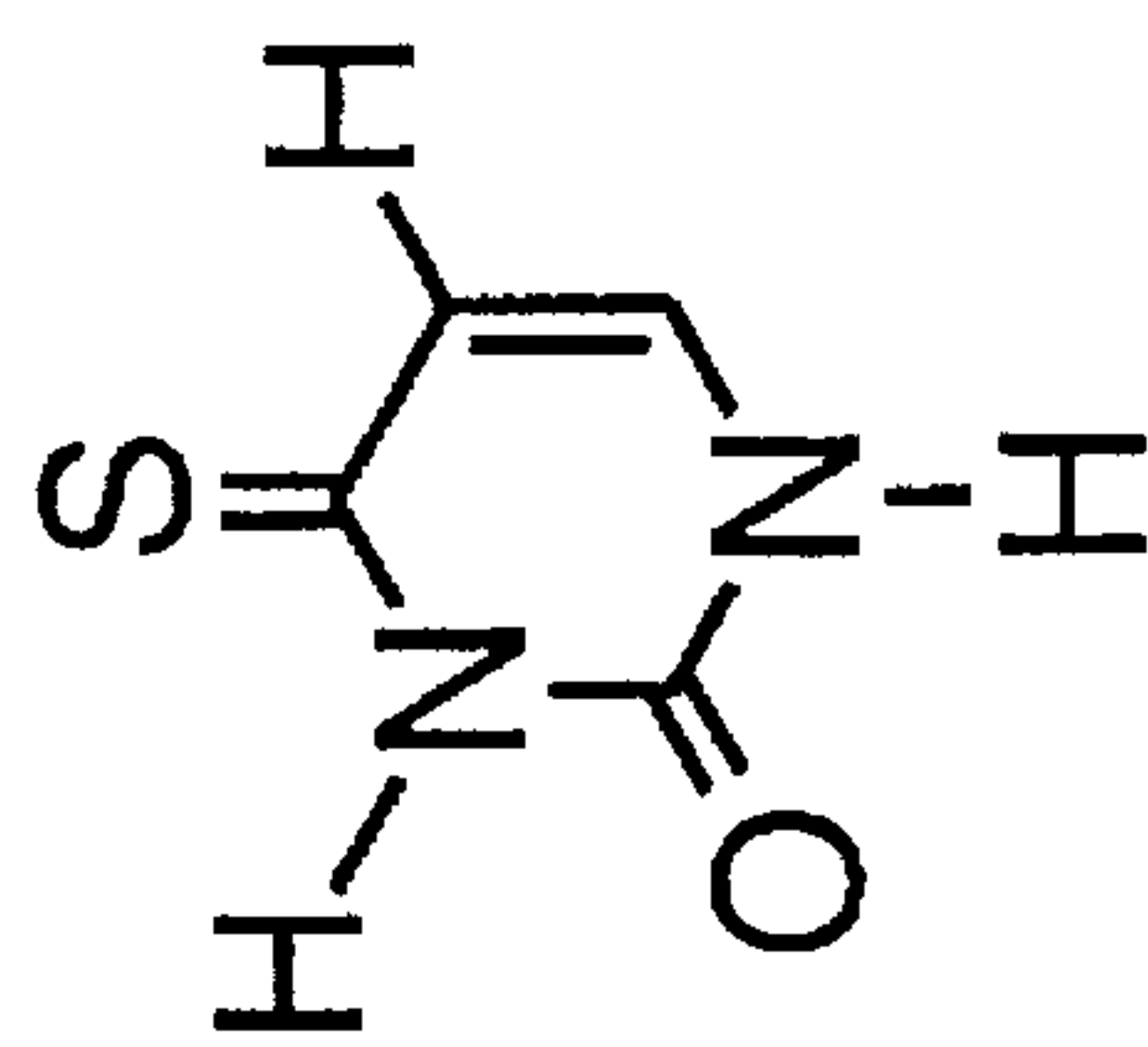
4-thiouracil
