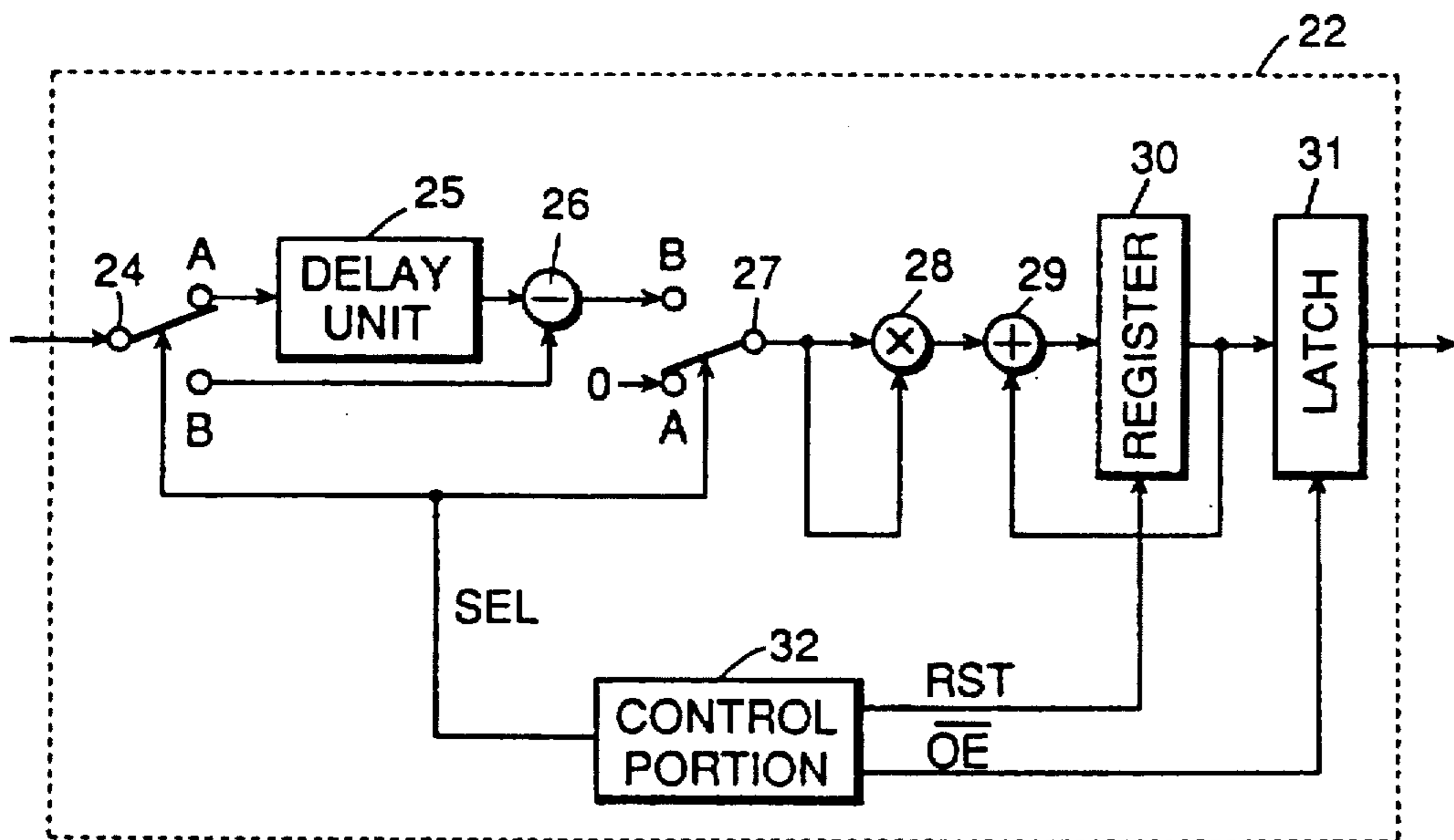
FIG.5 ( PRIOR ART )
