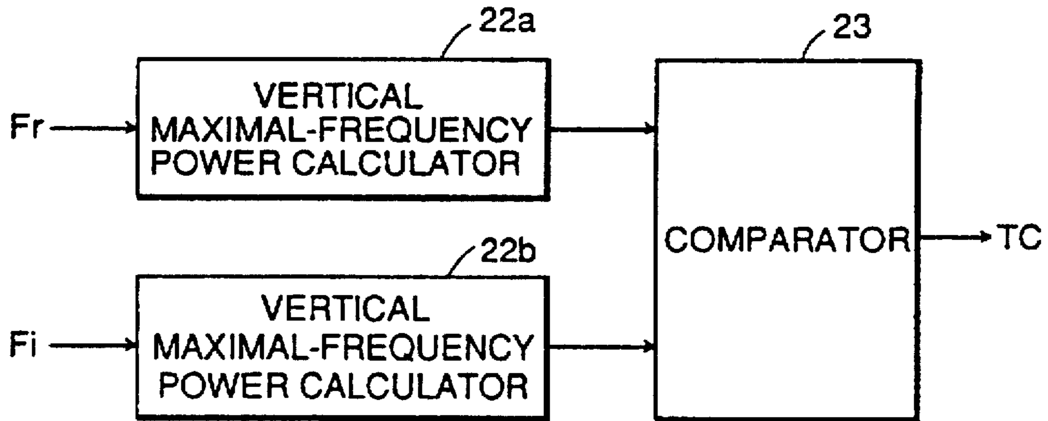
FIG.4 ( PRIOR ART )
