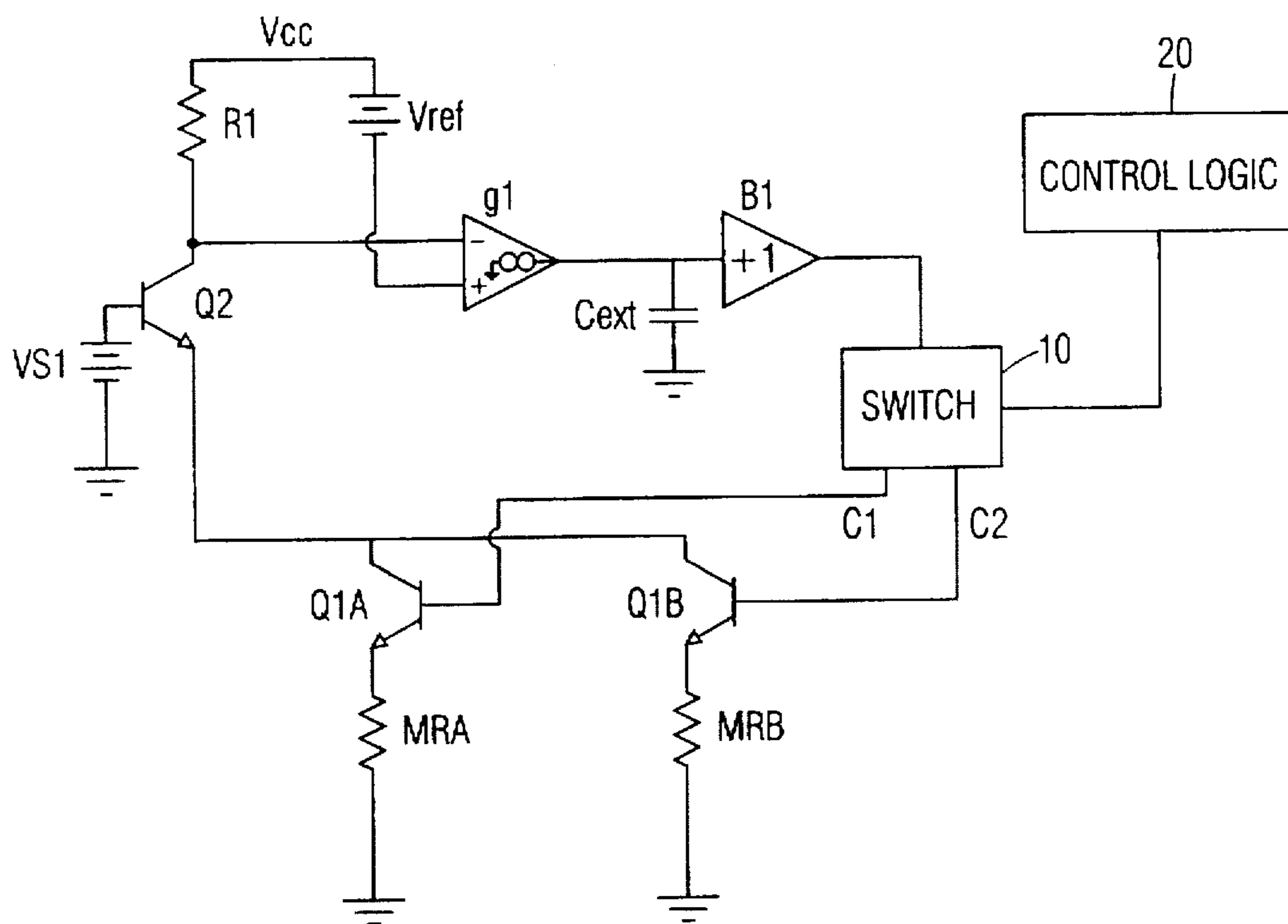
FIG. 1 (PRIOR ART)
