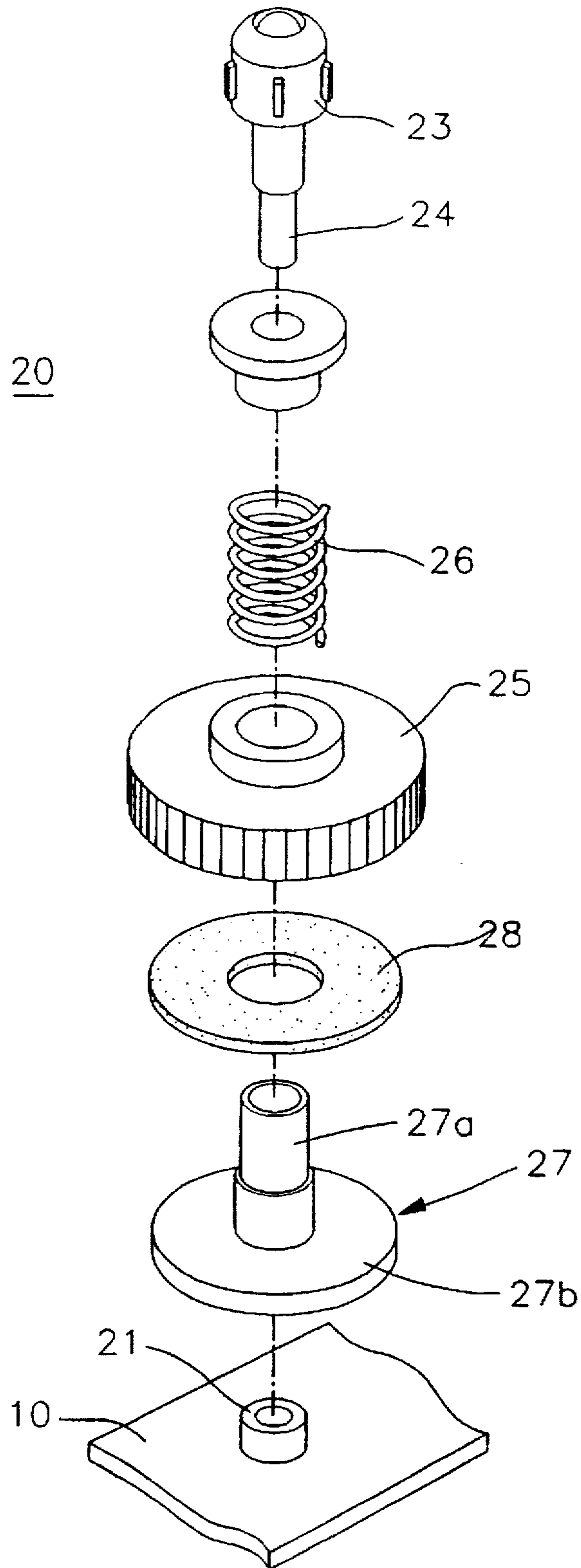
FIG. 1 PRIOR ART
