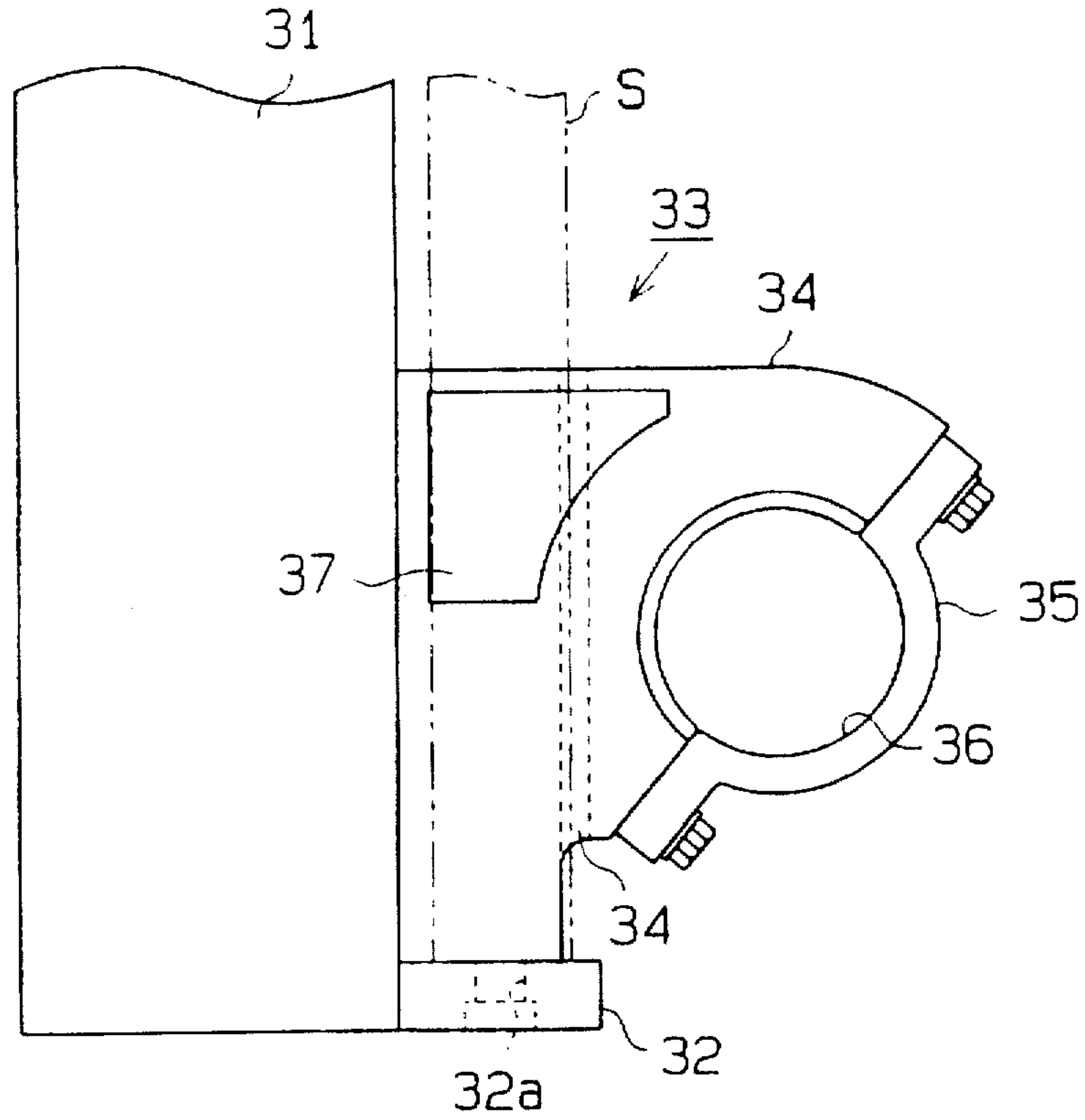
Fig.6 (Prior Art)
