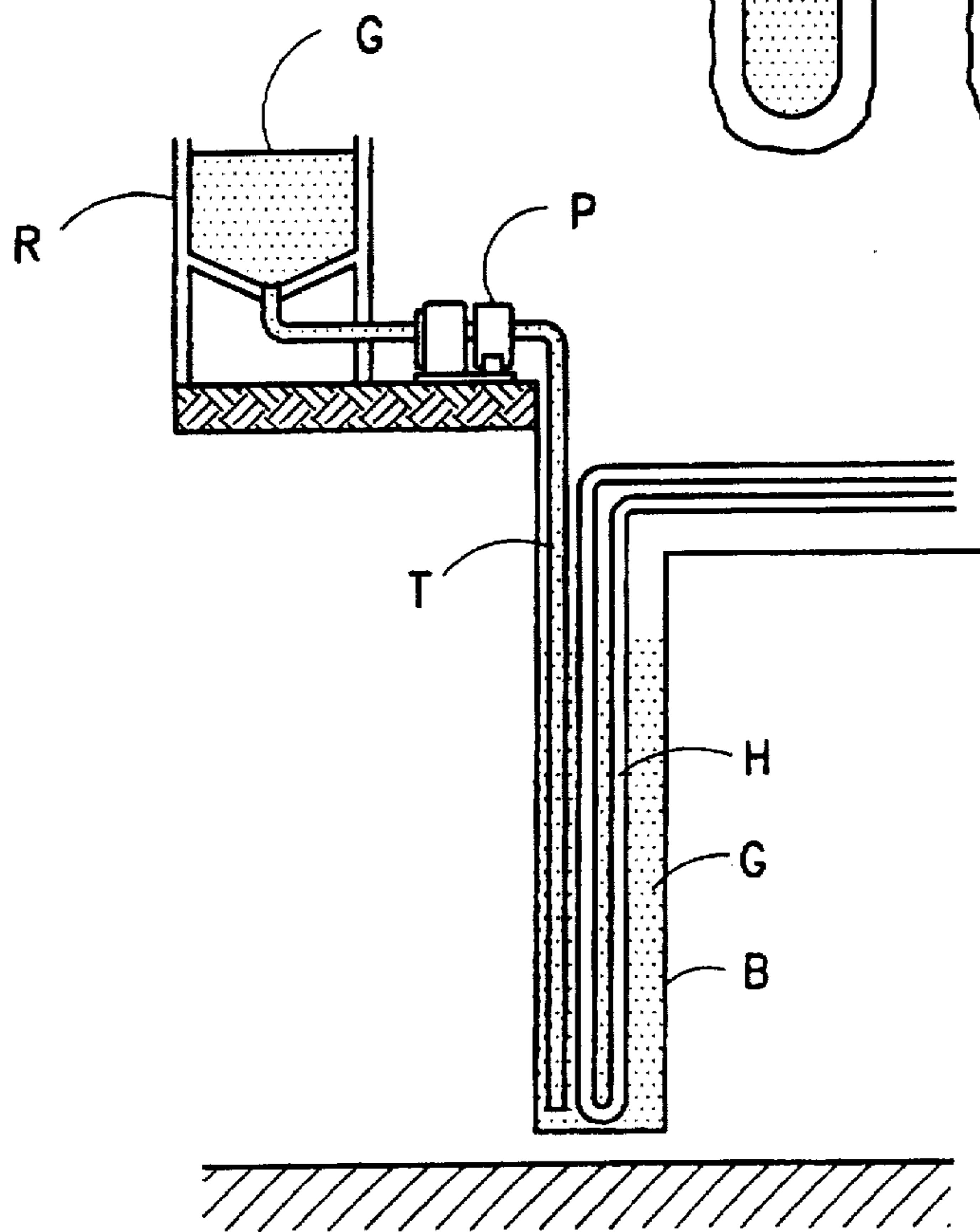
FIG. 2 (PRIOR ART)
