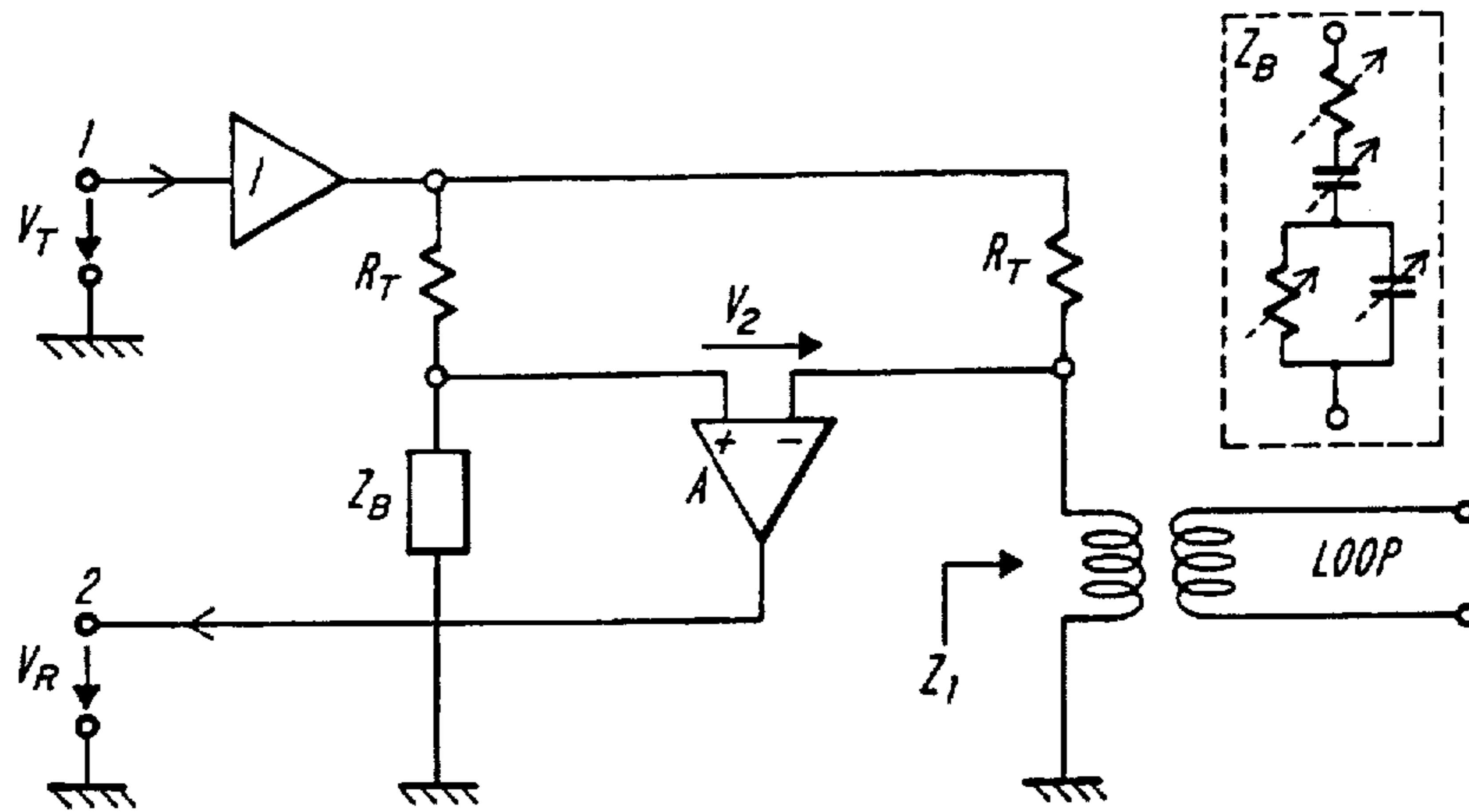
FIG. 3 PRIOR ART
