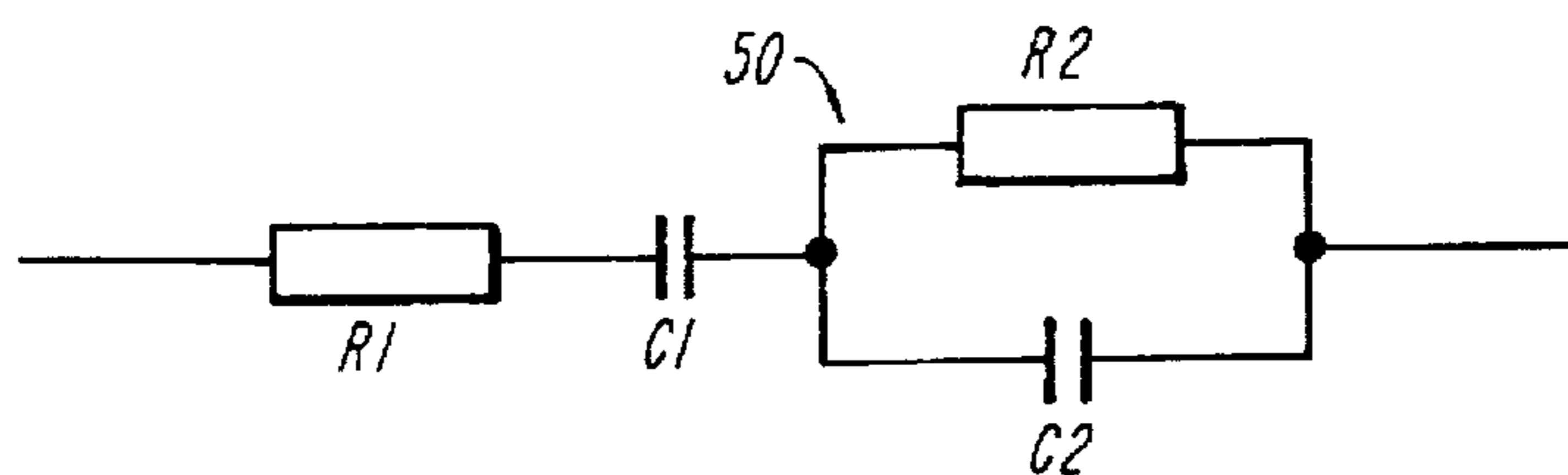
FIG. 5 PRIOR ART
