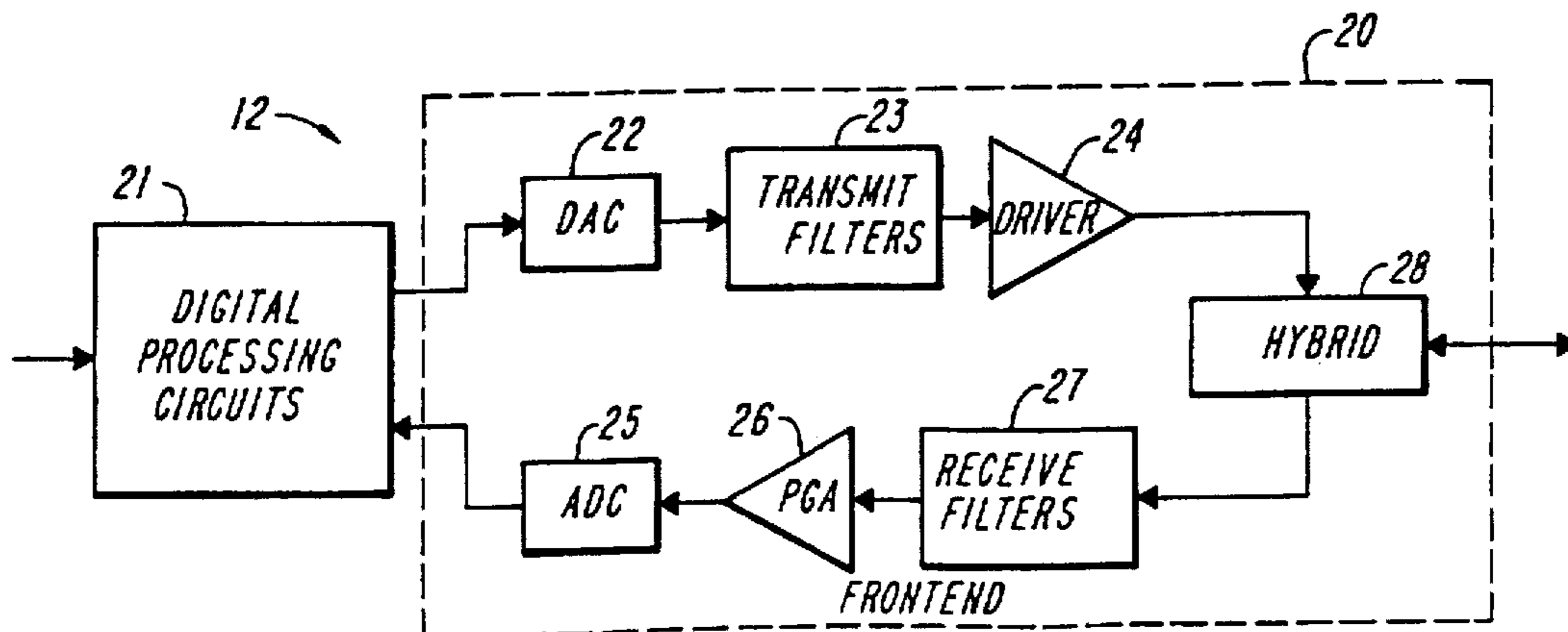
FIG. 2 PRIOR ART
