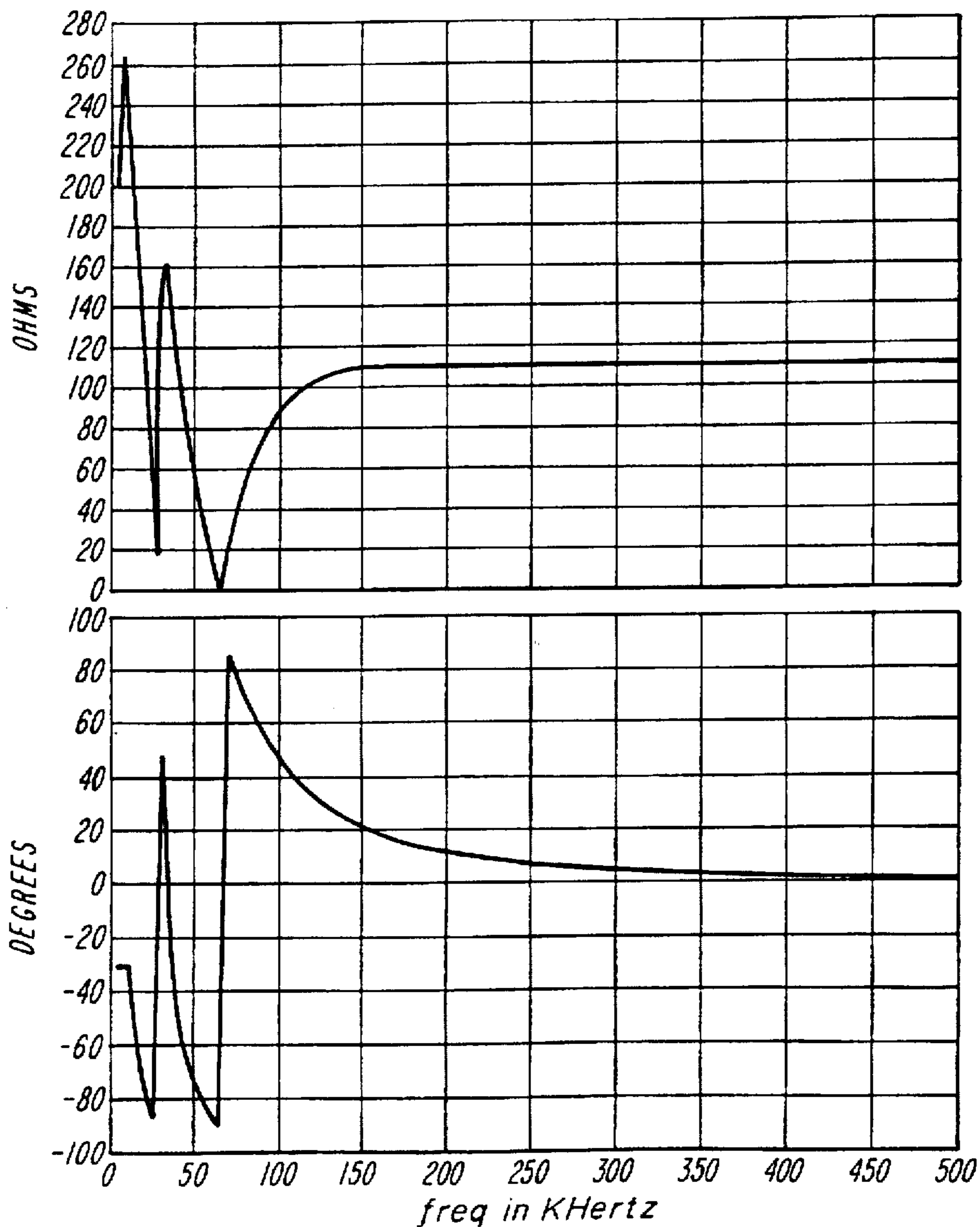
FIG. 6 PRIOR ART
