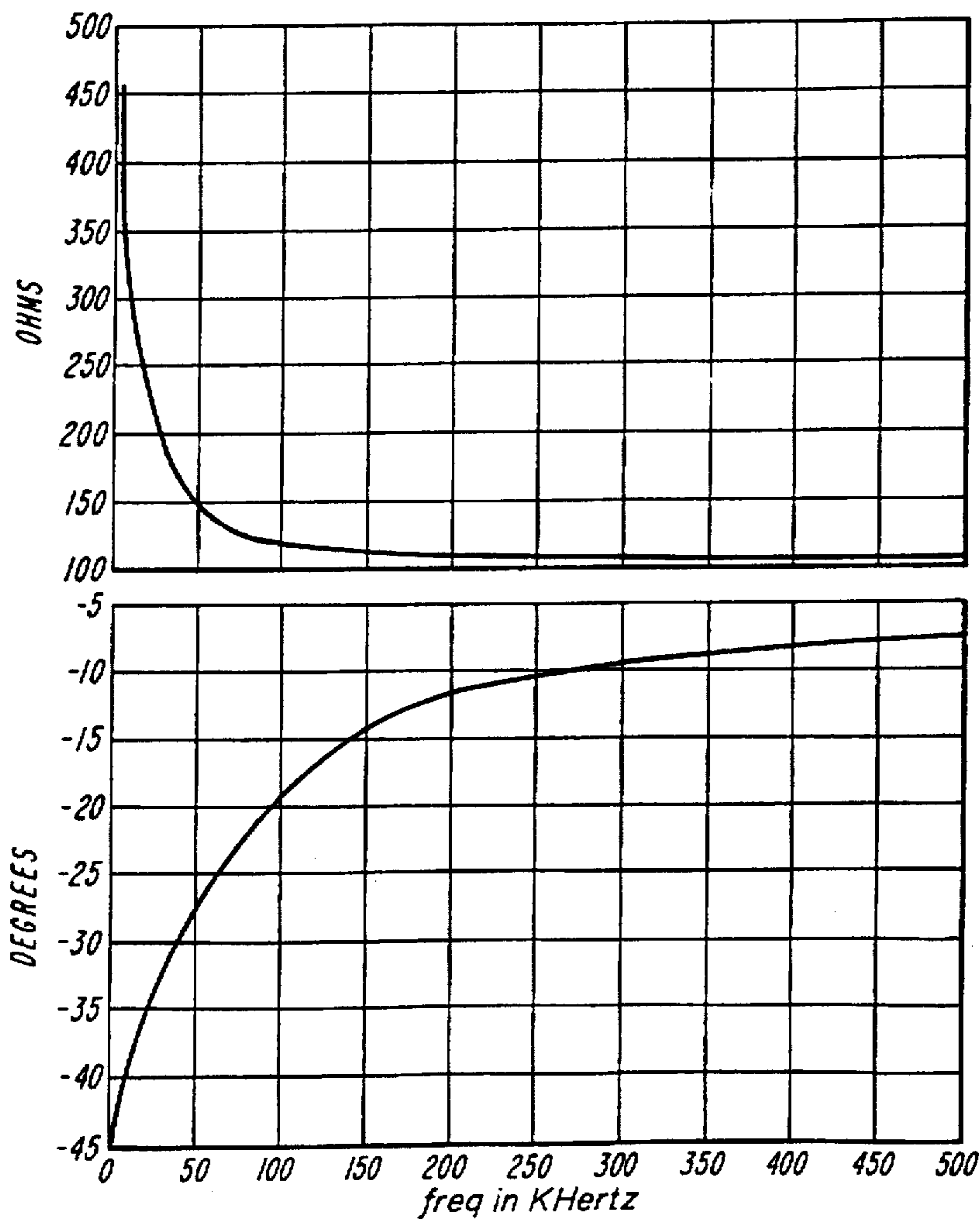
FIG. 4 PRIOR ART
