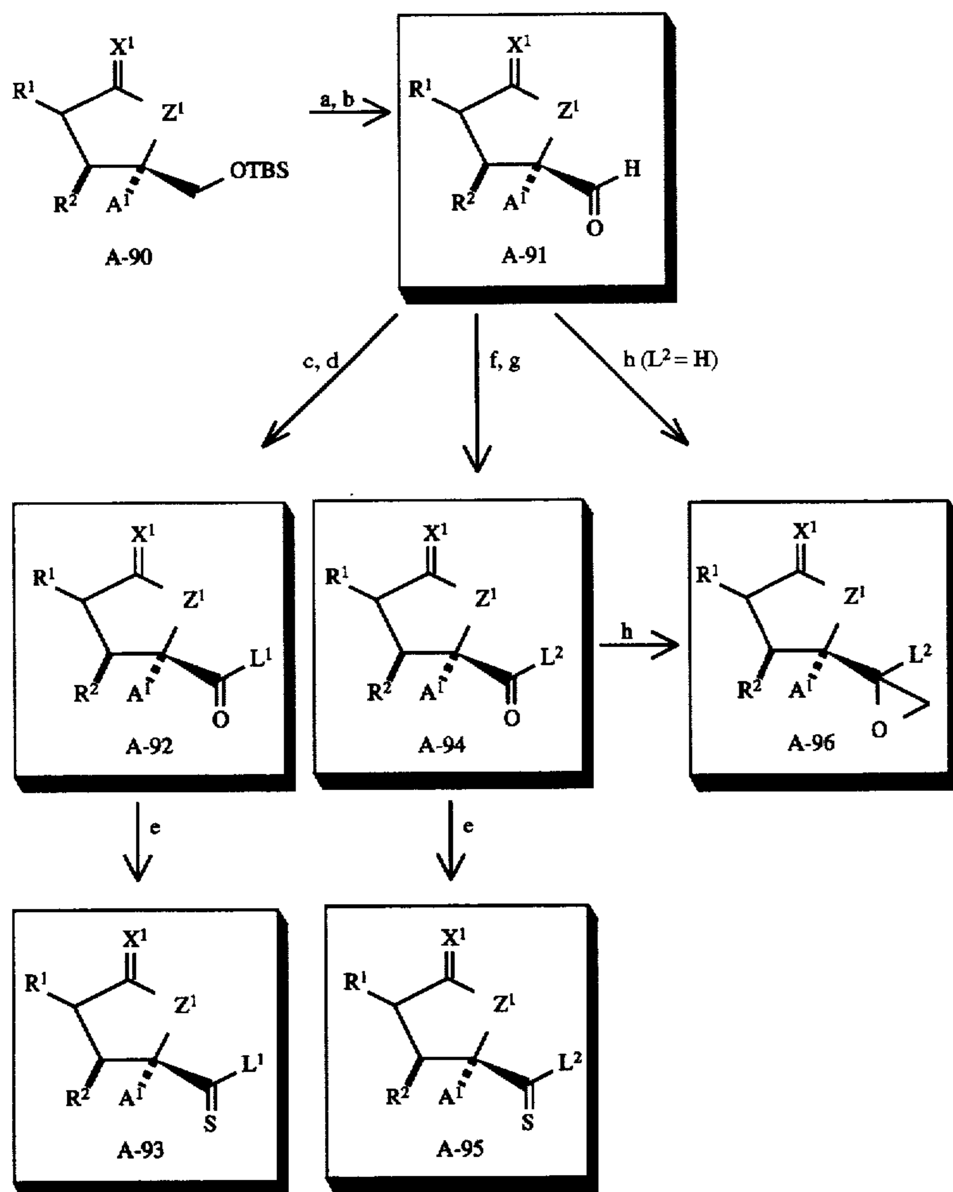
Scheme 13b
