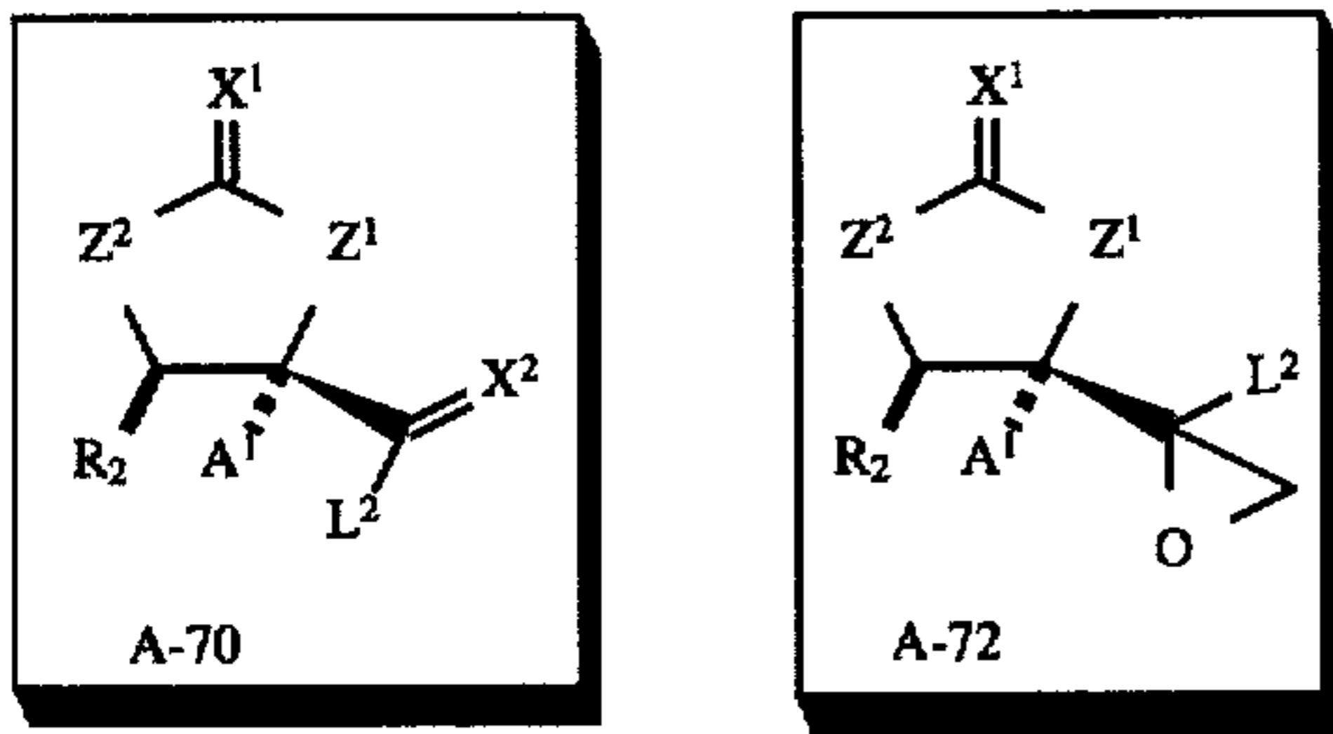
-continued Scheme 11
