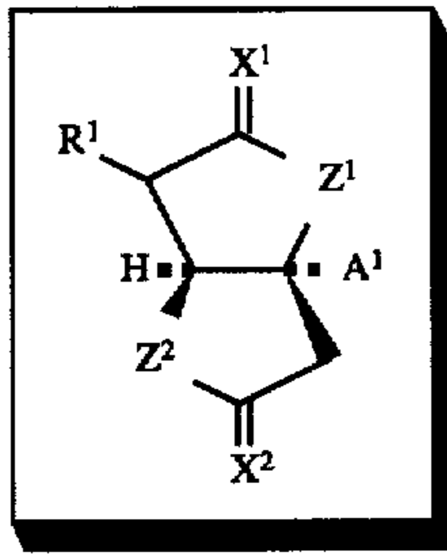
Scheme 22
