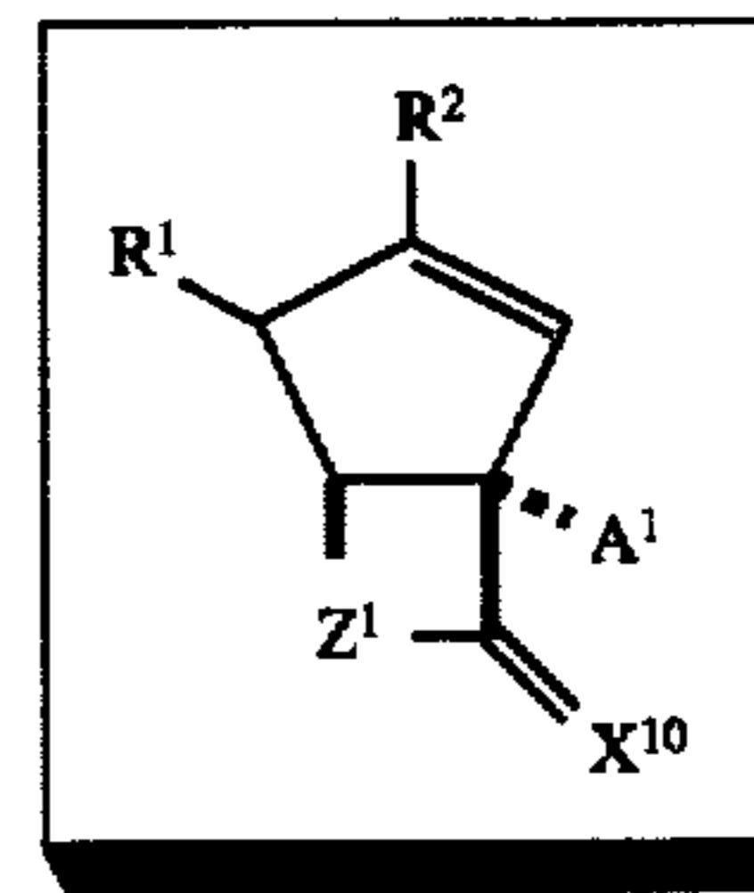
Scheme 23
