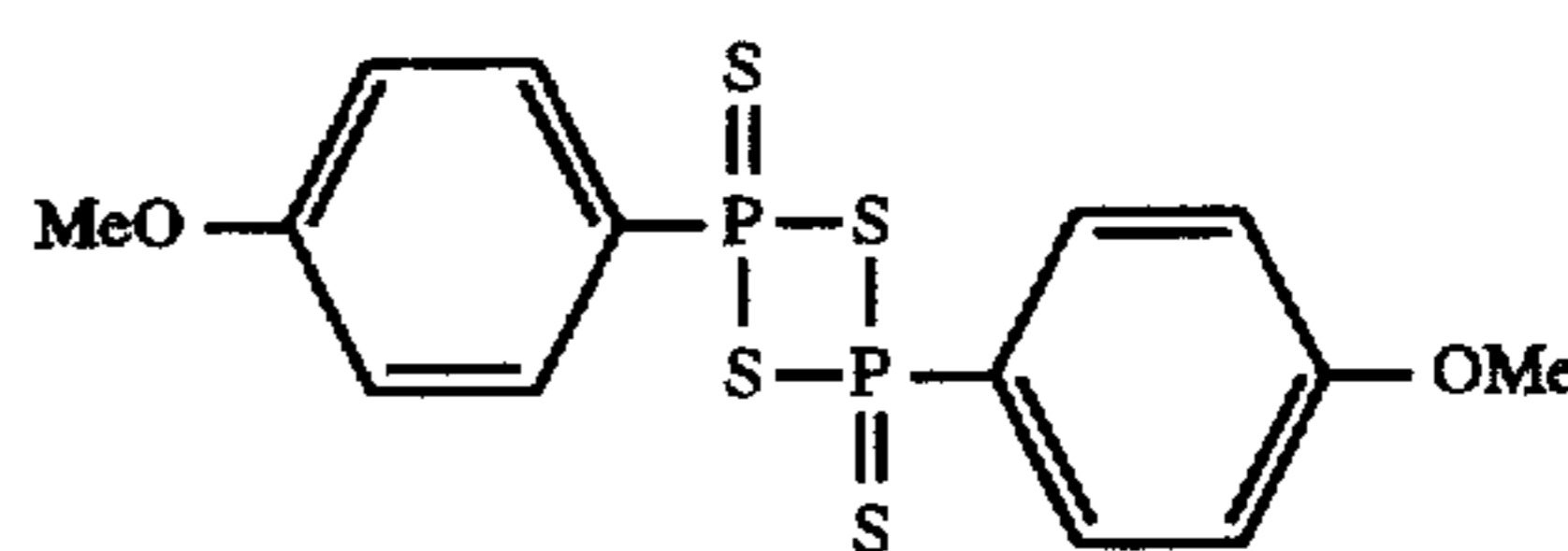
Lawesson's reagent
