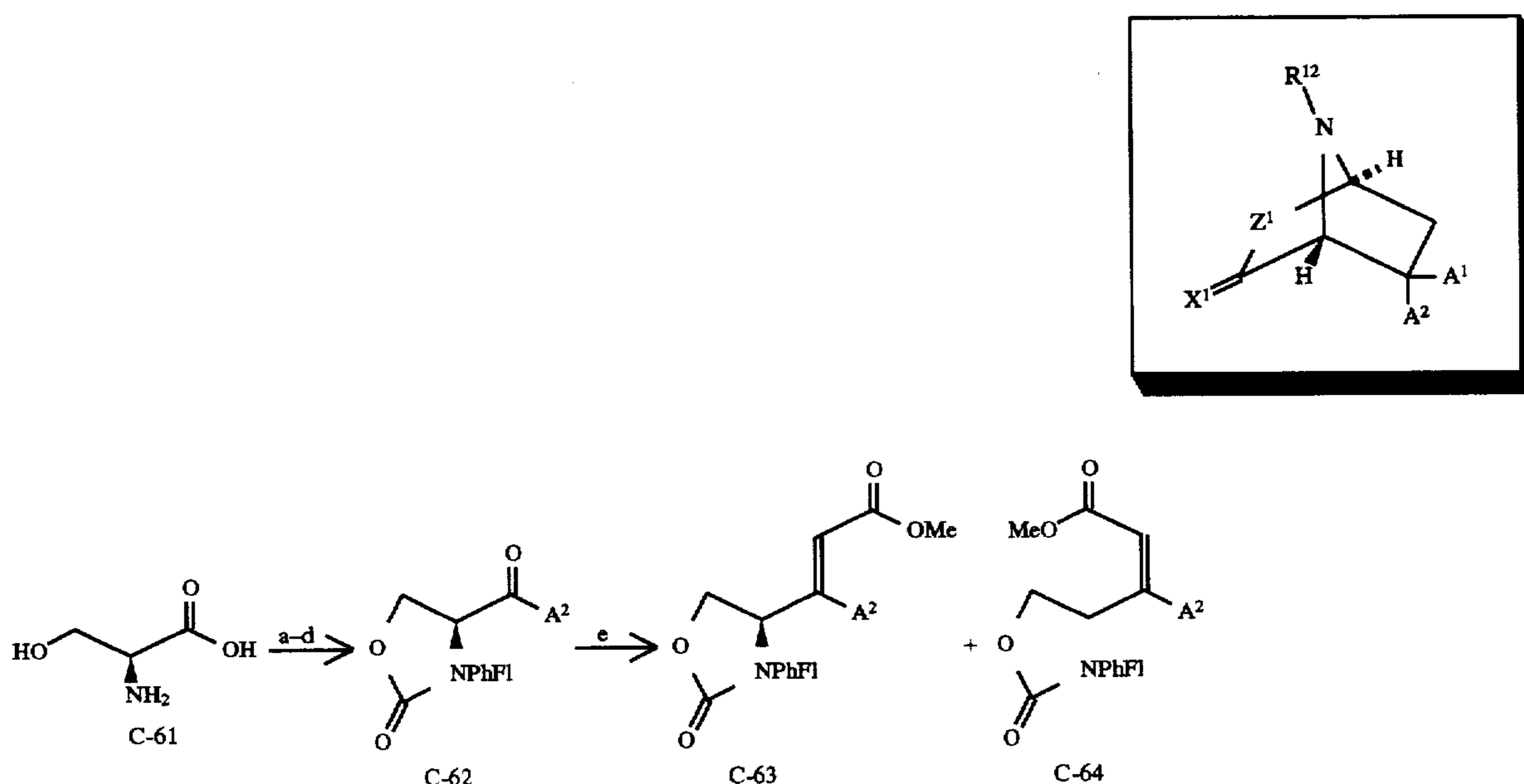
Scheme 27
