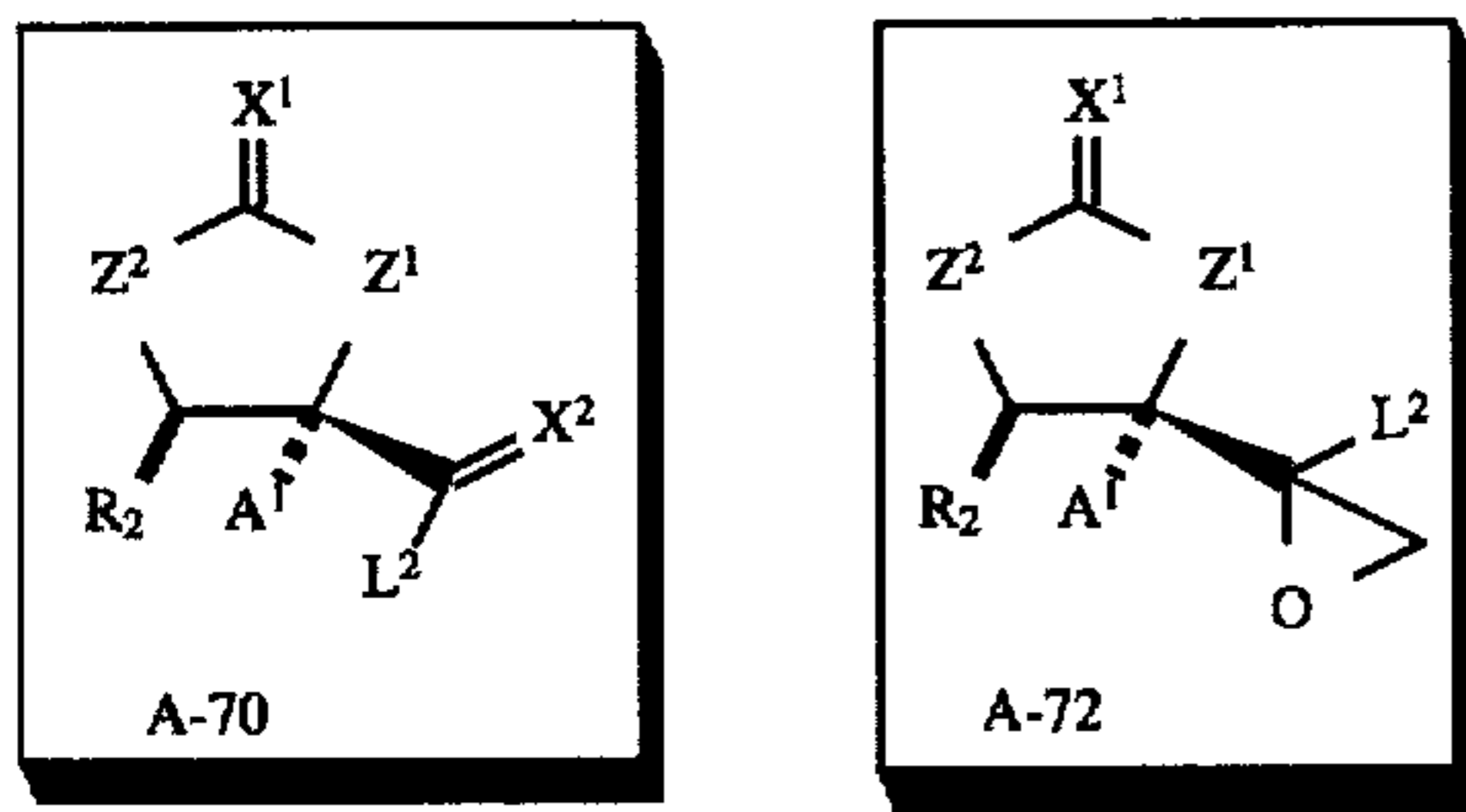
-continued Scheme 11
