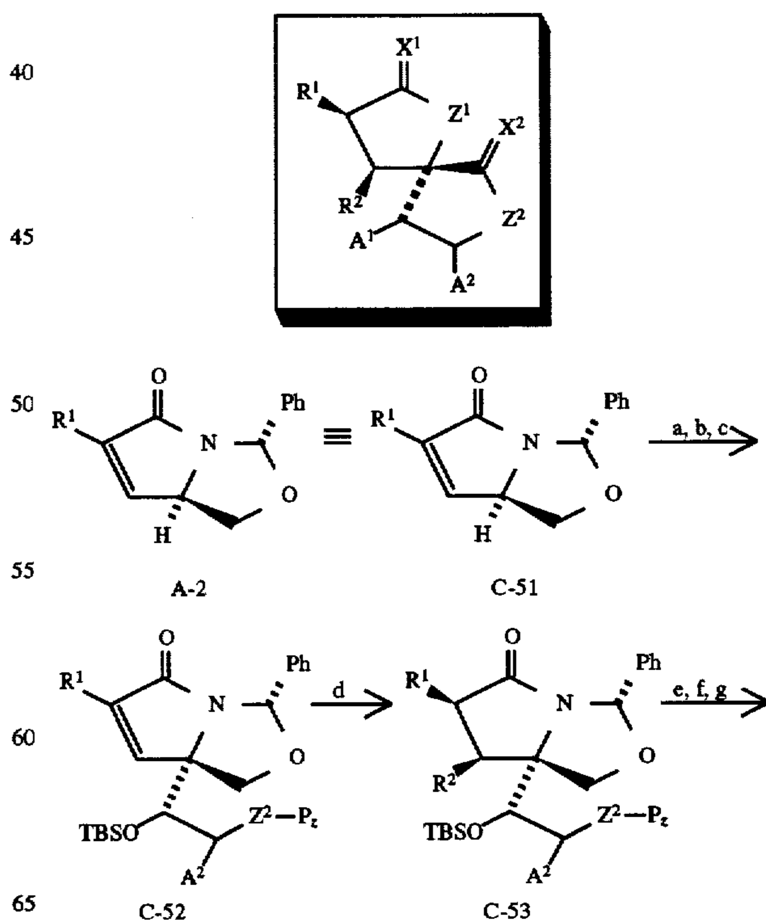
Scheme 26
