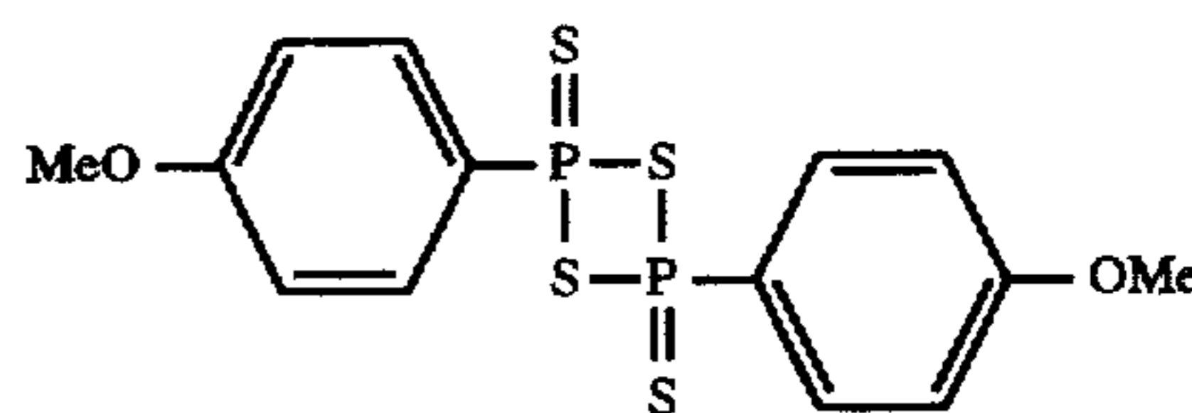
Lawesson's reagent
