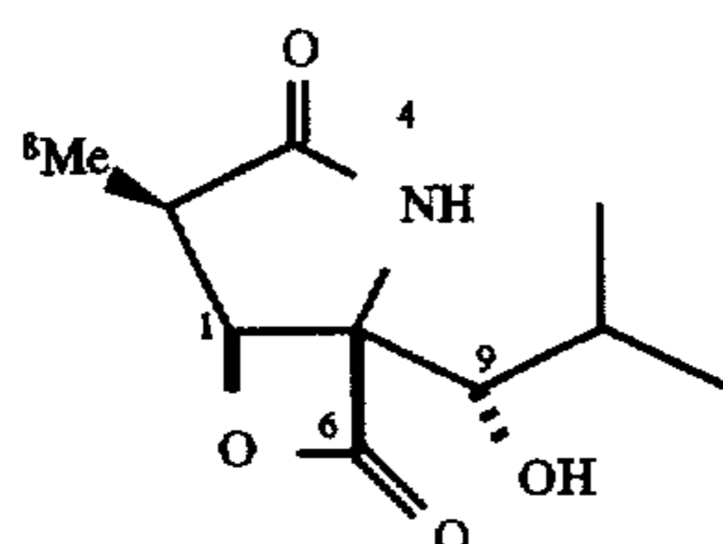
Lactacystin \beta -lactone
