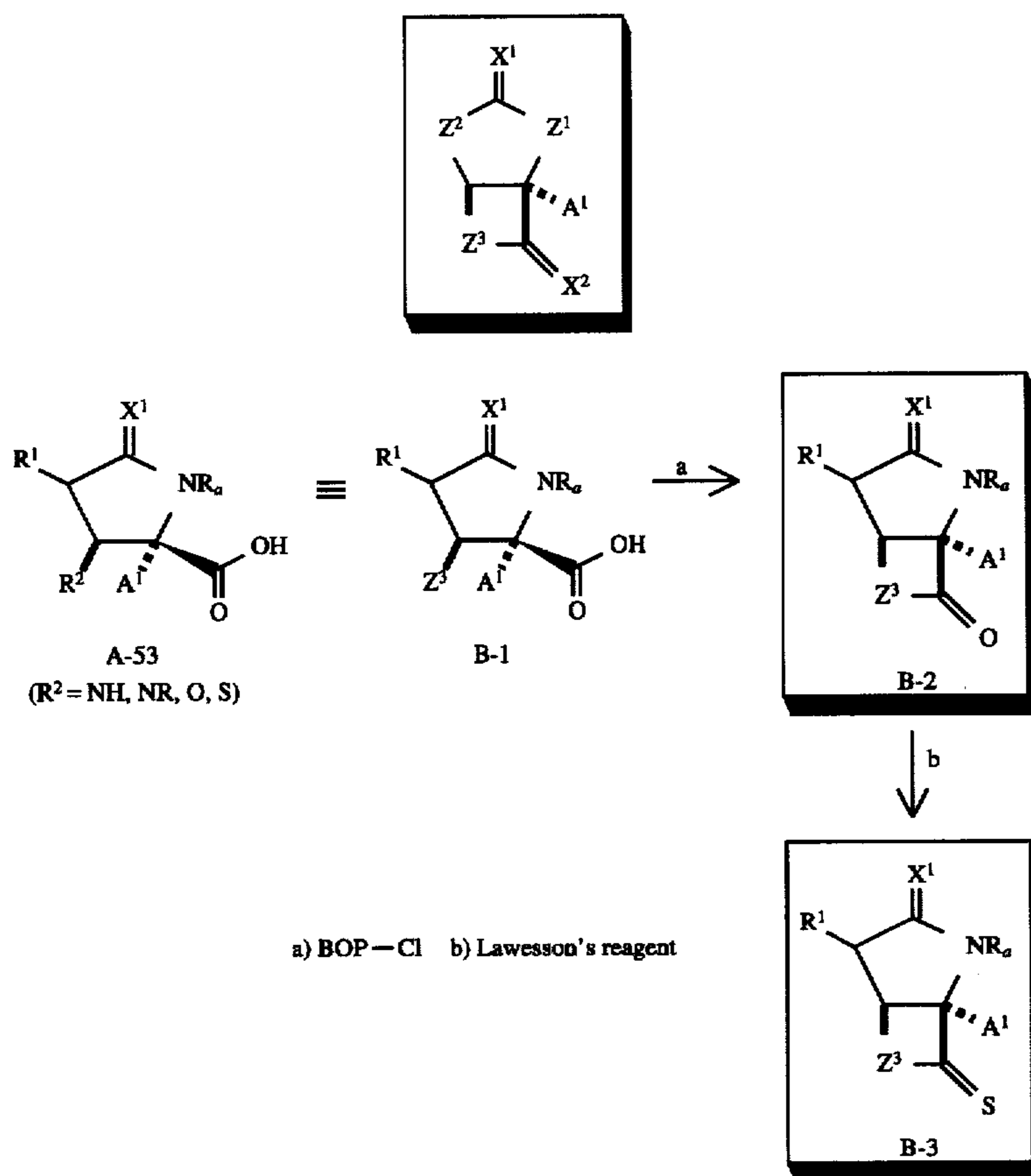
Scheme 14
