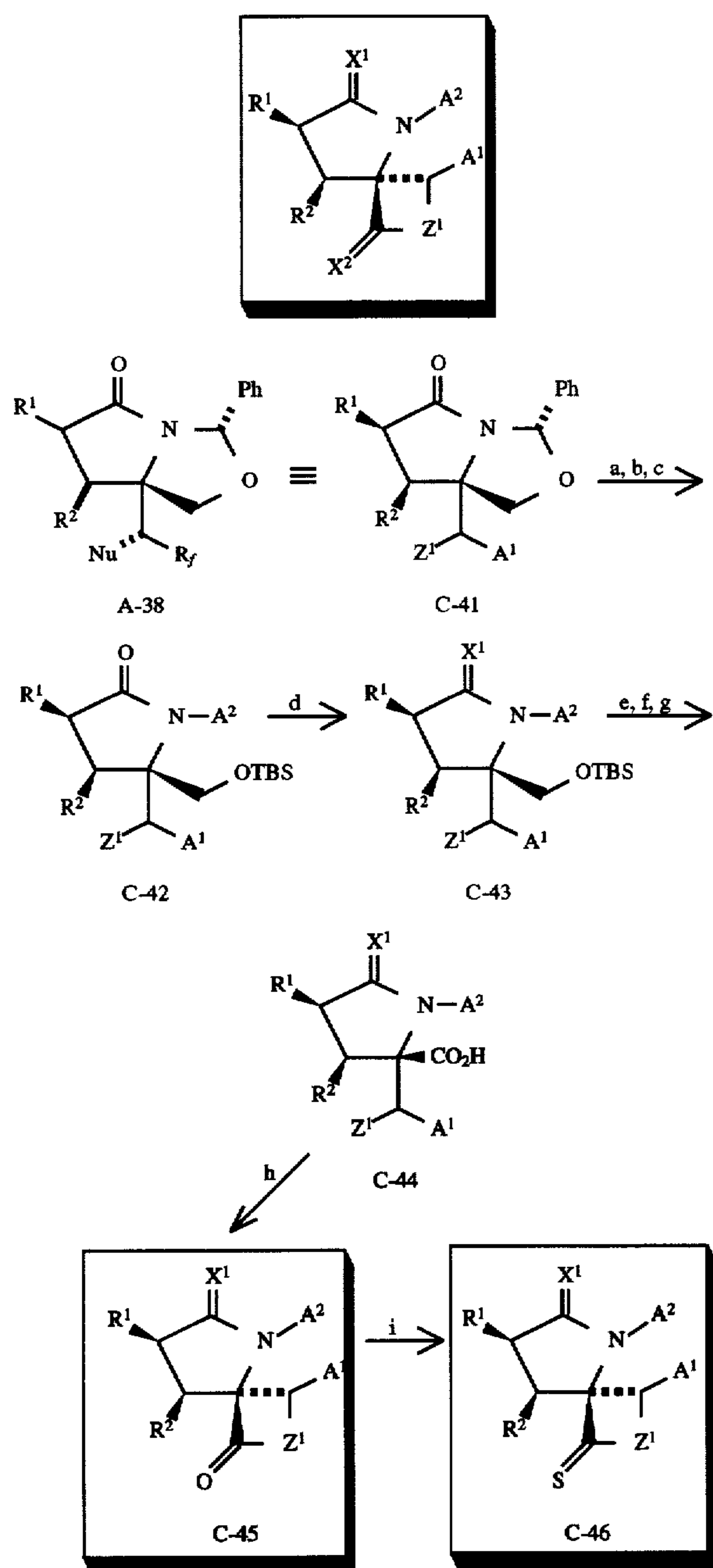
Scheme 25
