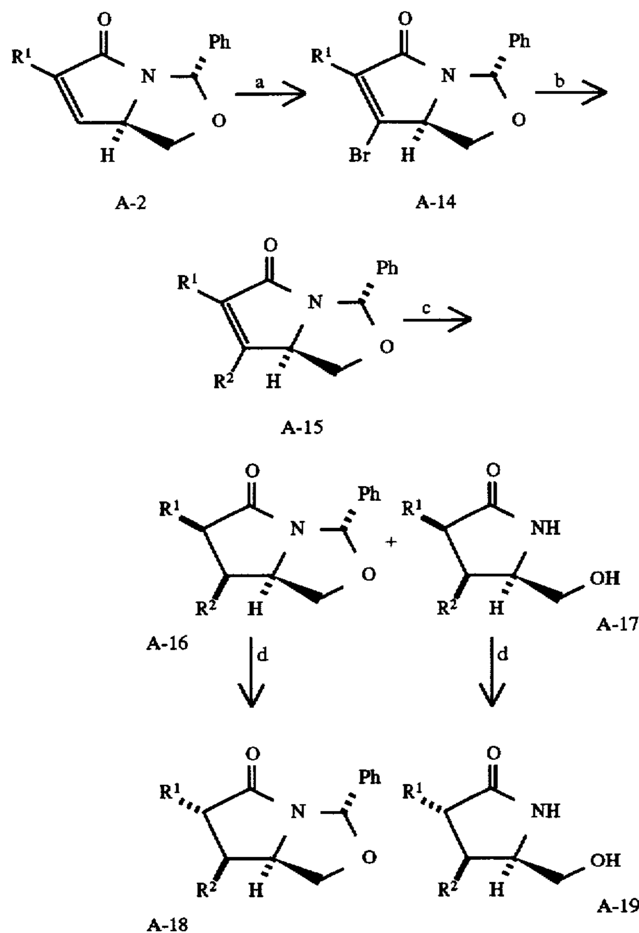
Scheme 2
