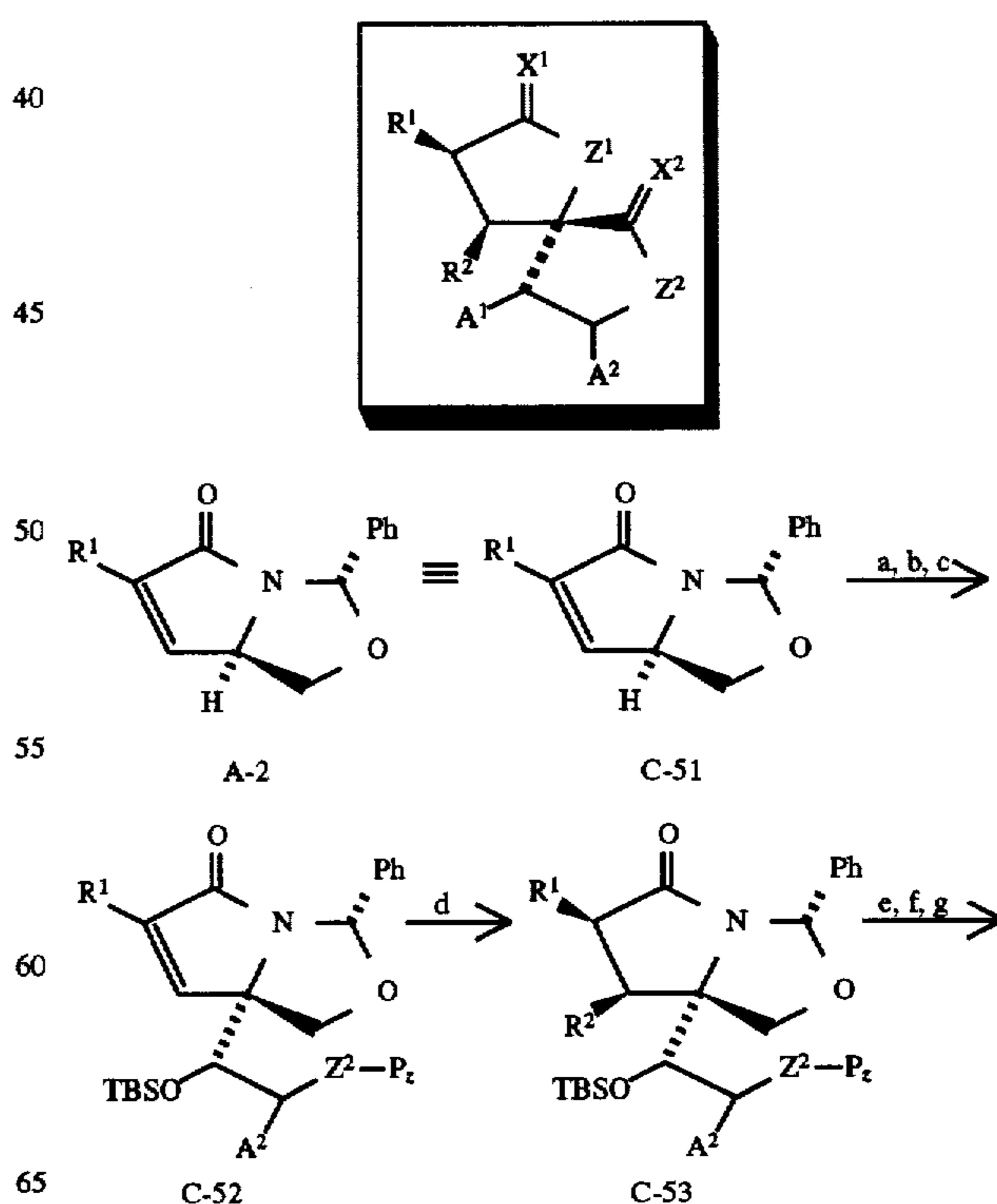
Scheme 26
