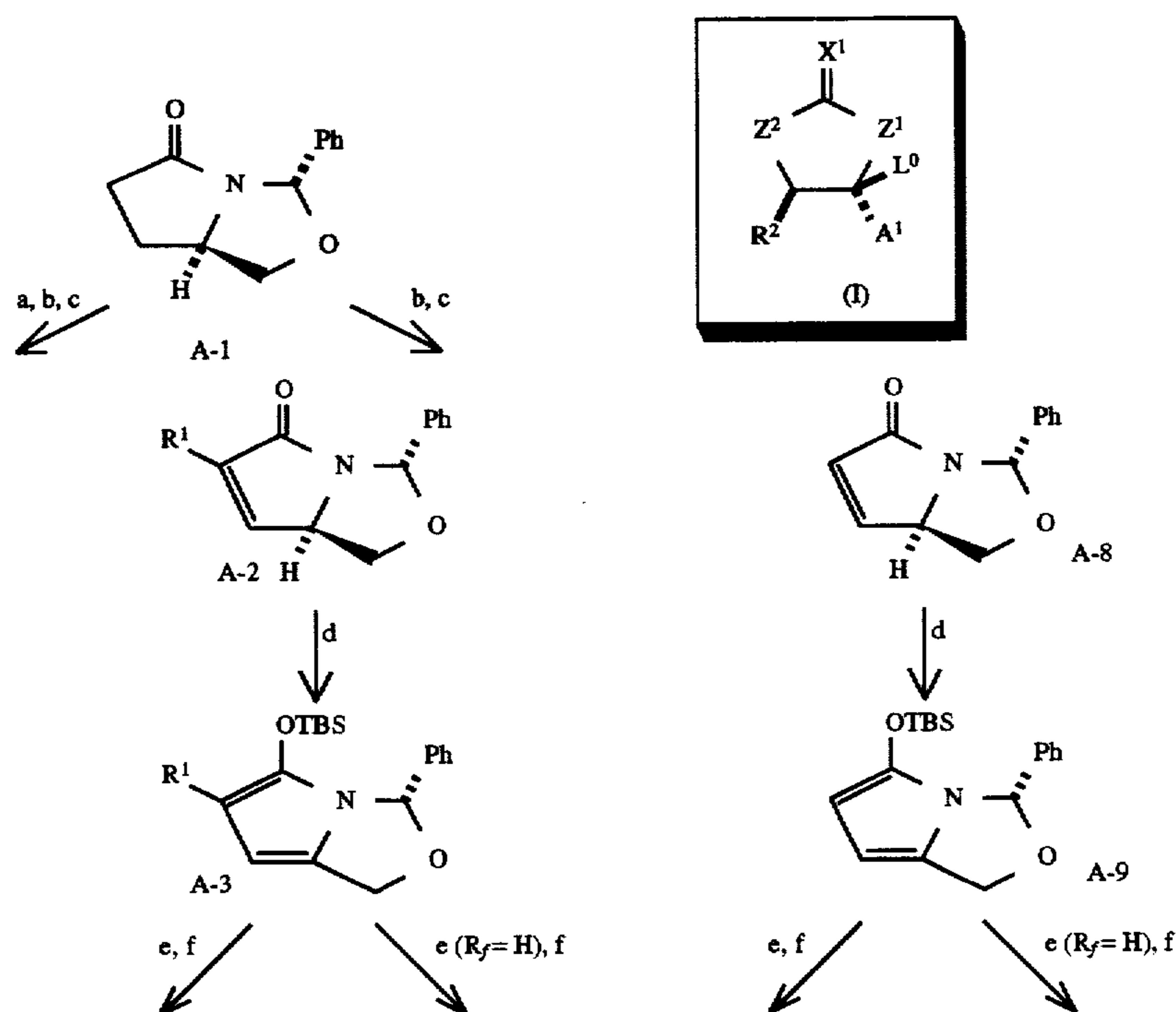
Scheme 1
