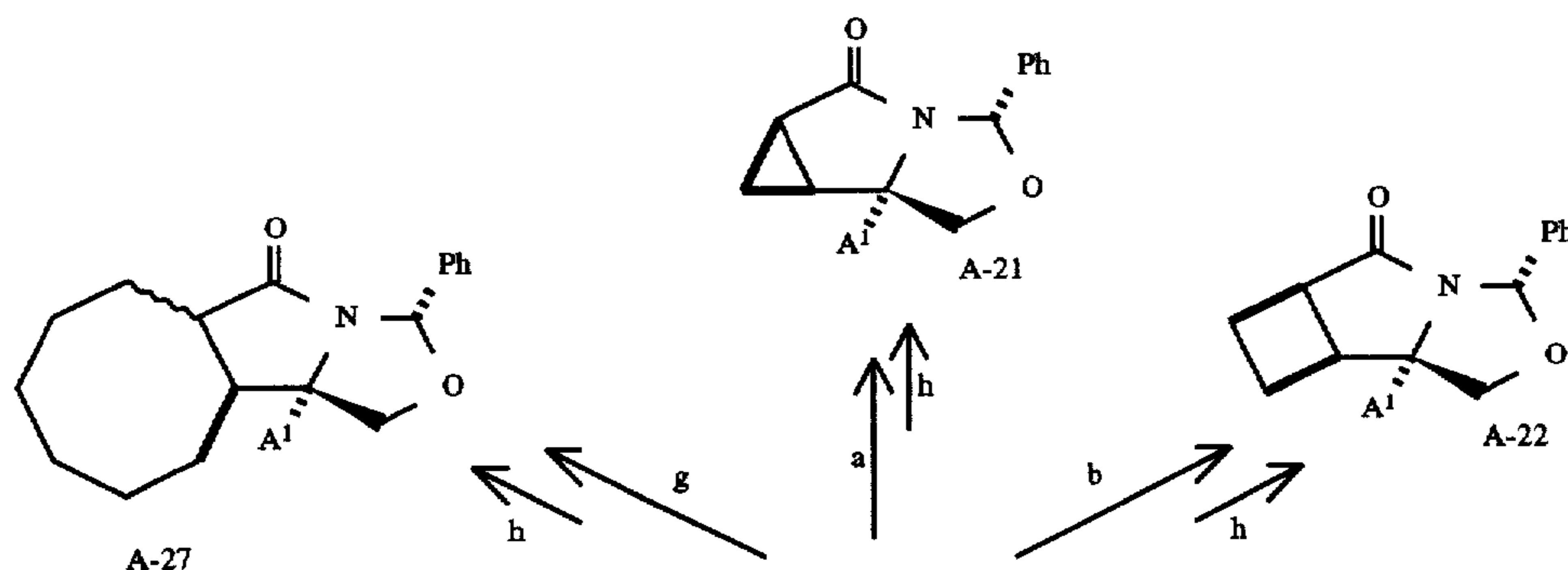
Scheme 3
