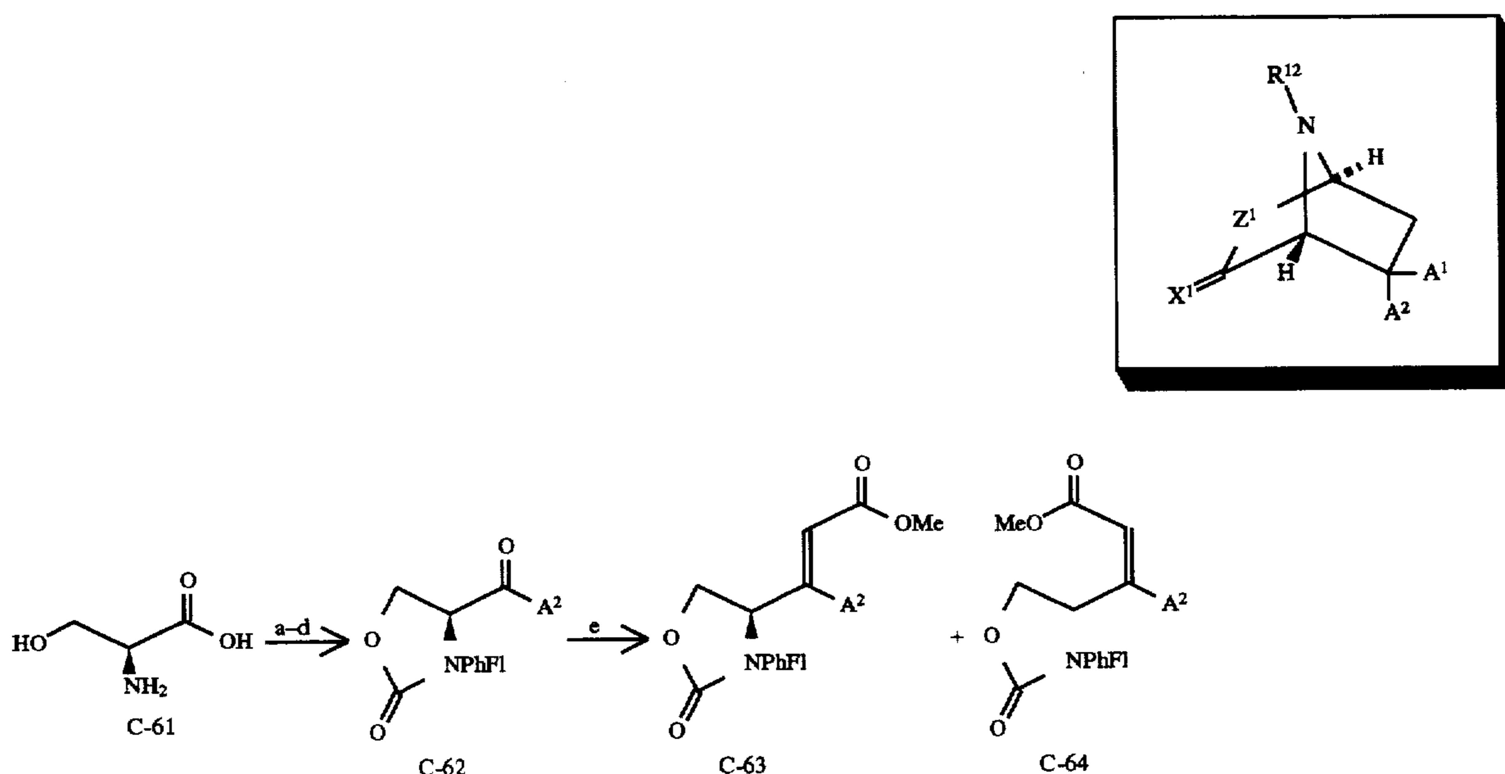
Scheme 27
