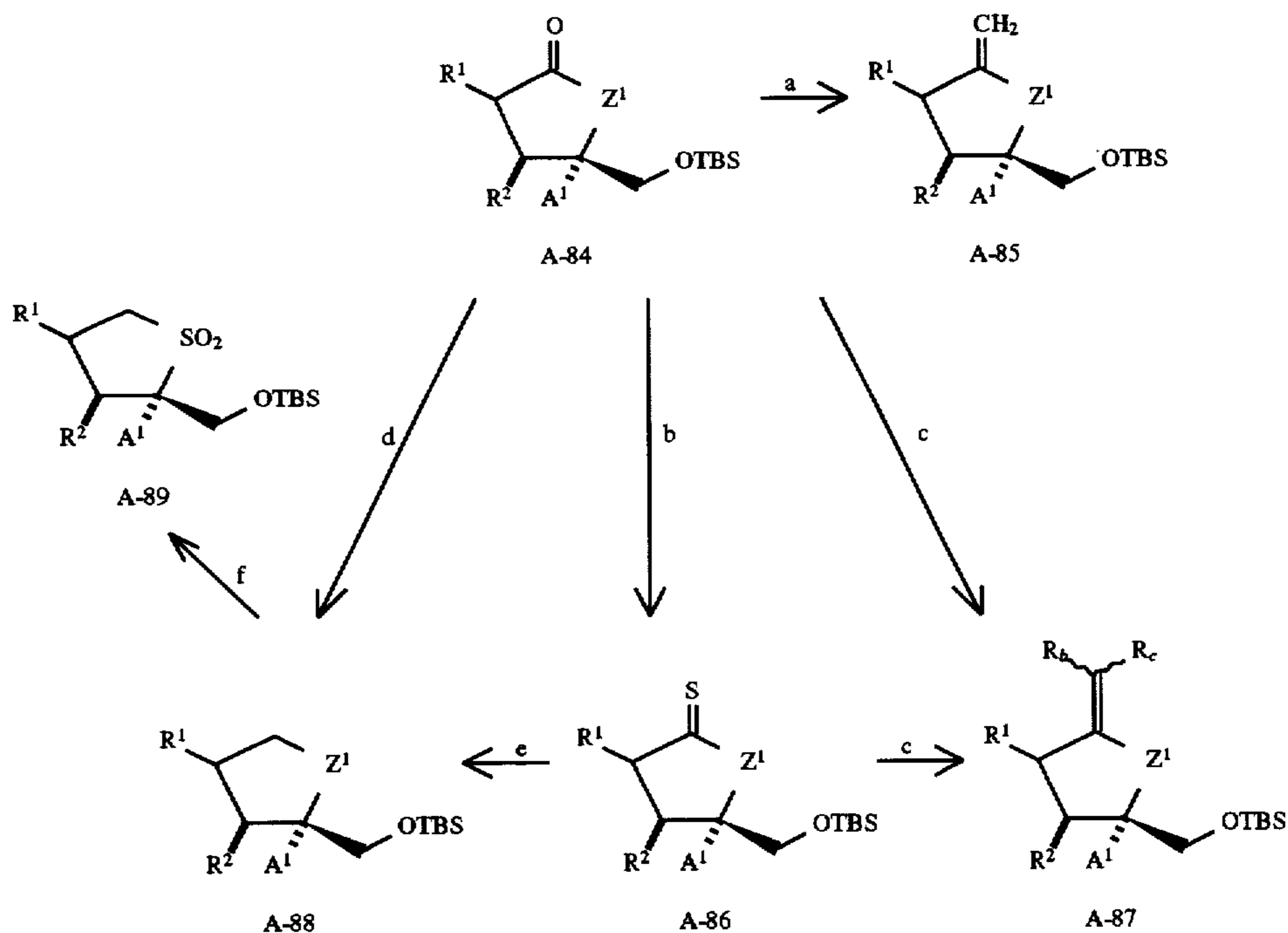
Scheme 13a
