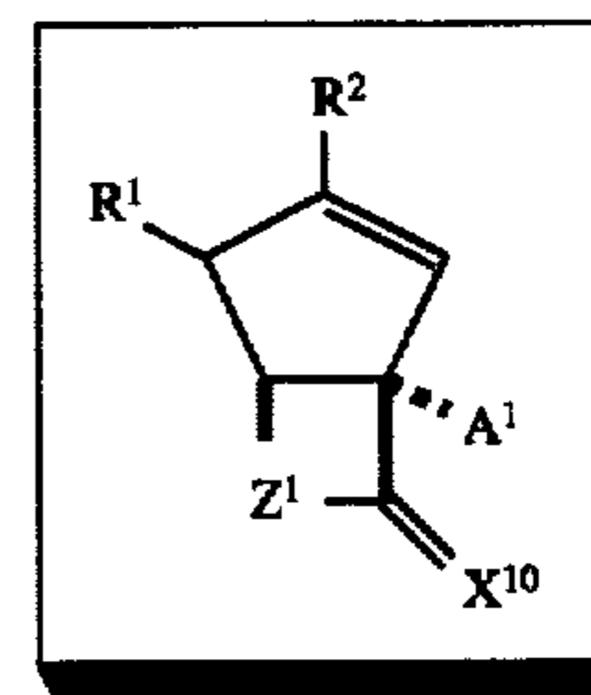
Scheme 23
