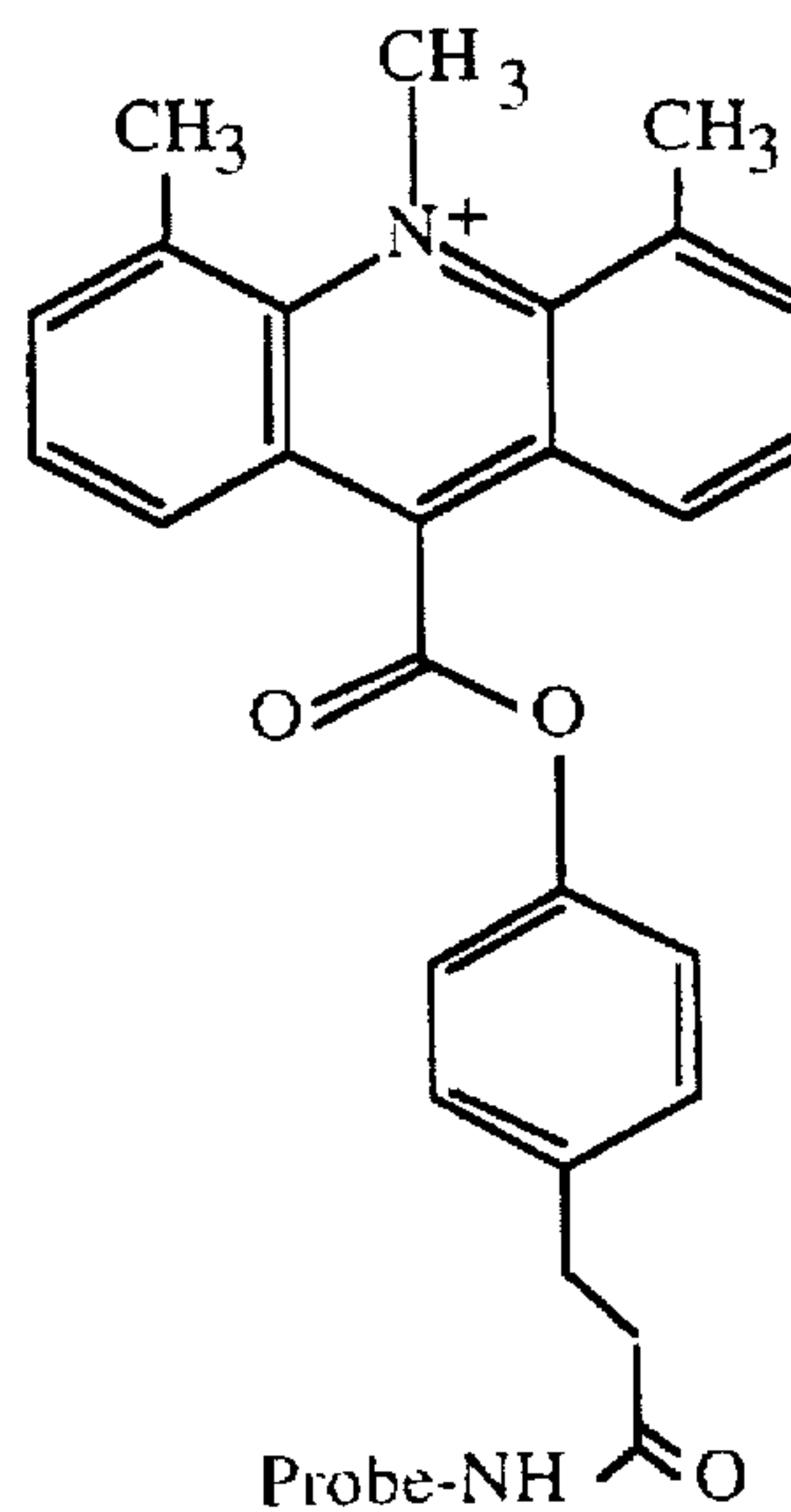
4,5-diMe-AE
