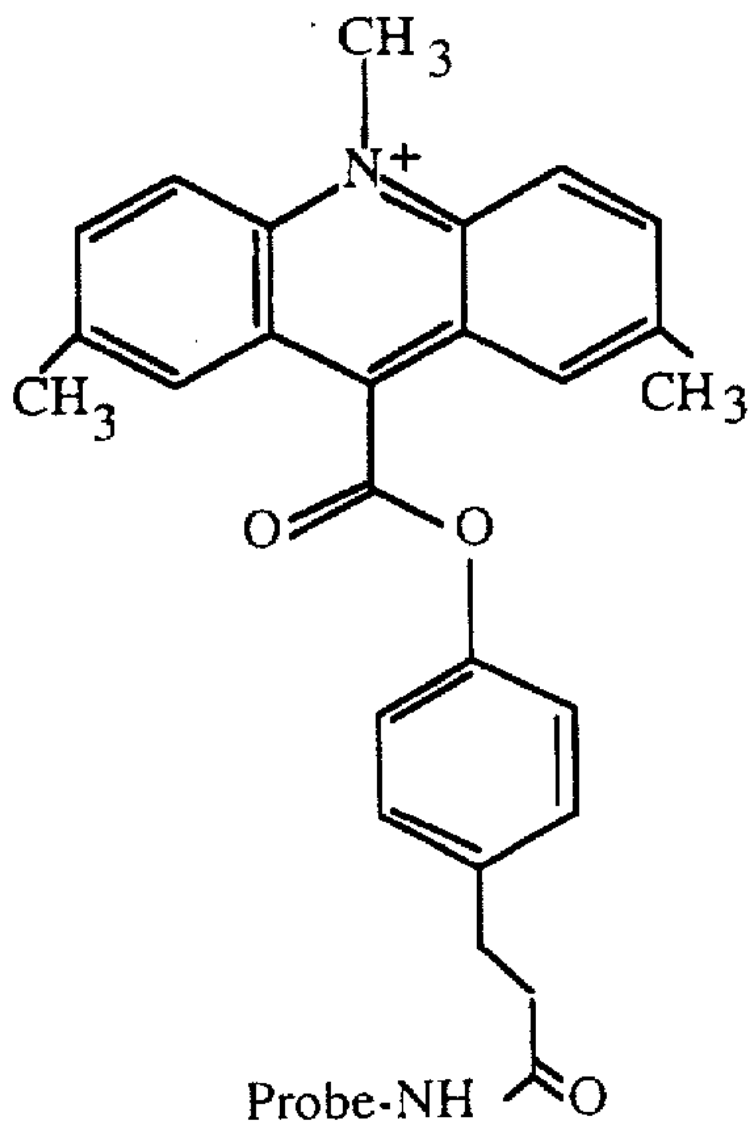
2,7-diMe-AE
