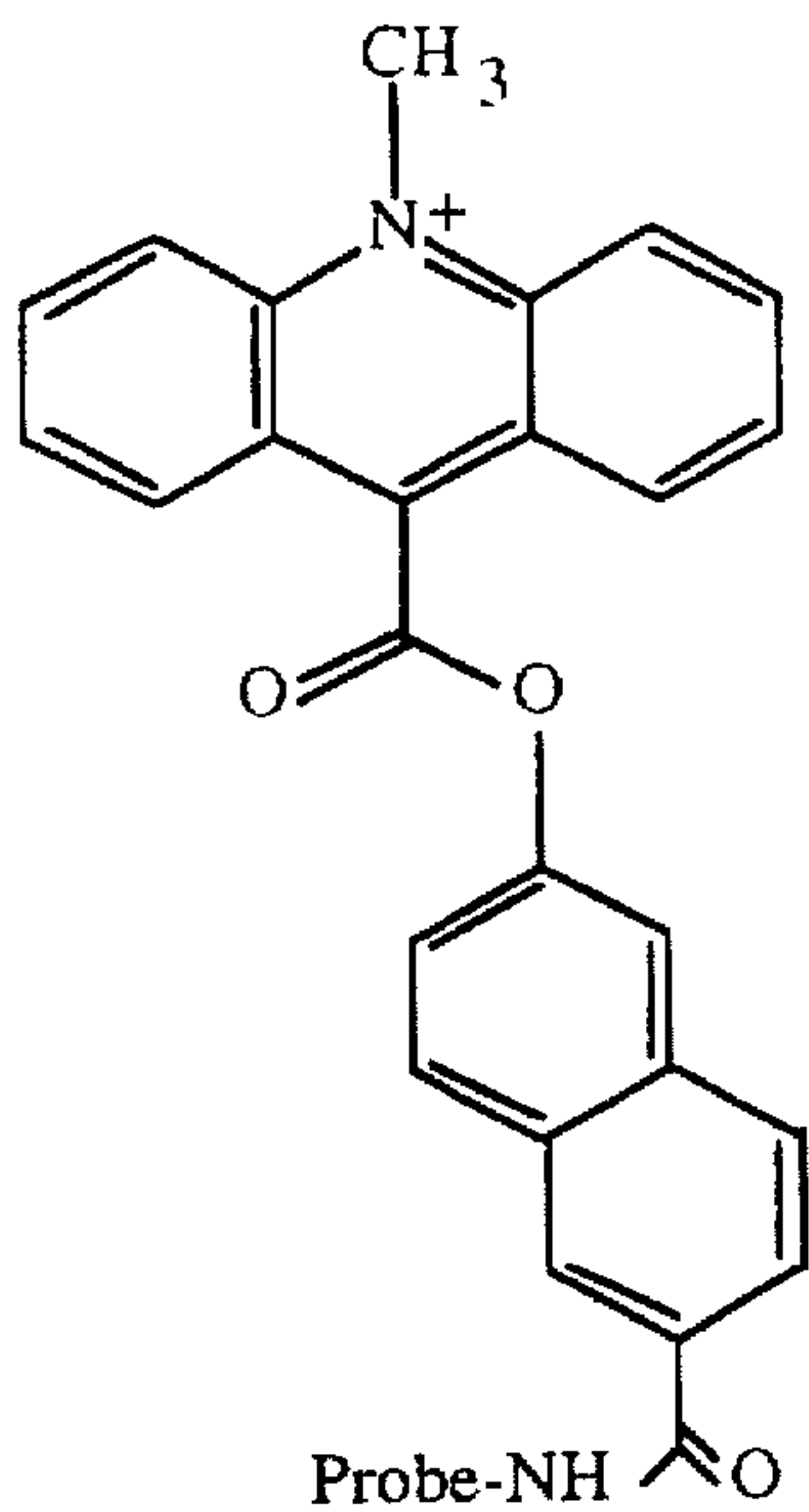
naphthyl-AE
