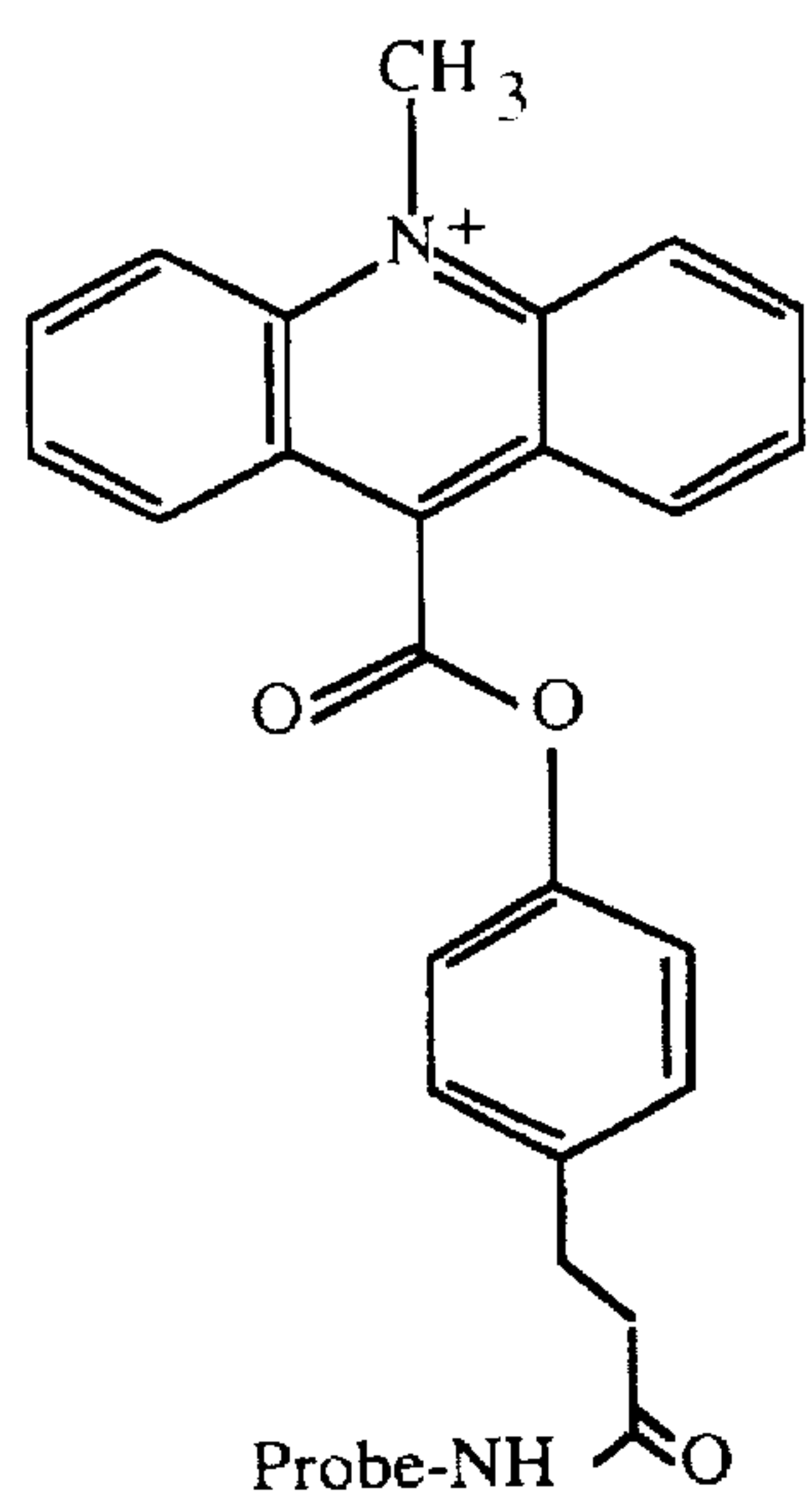
Standard-AE
