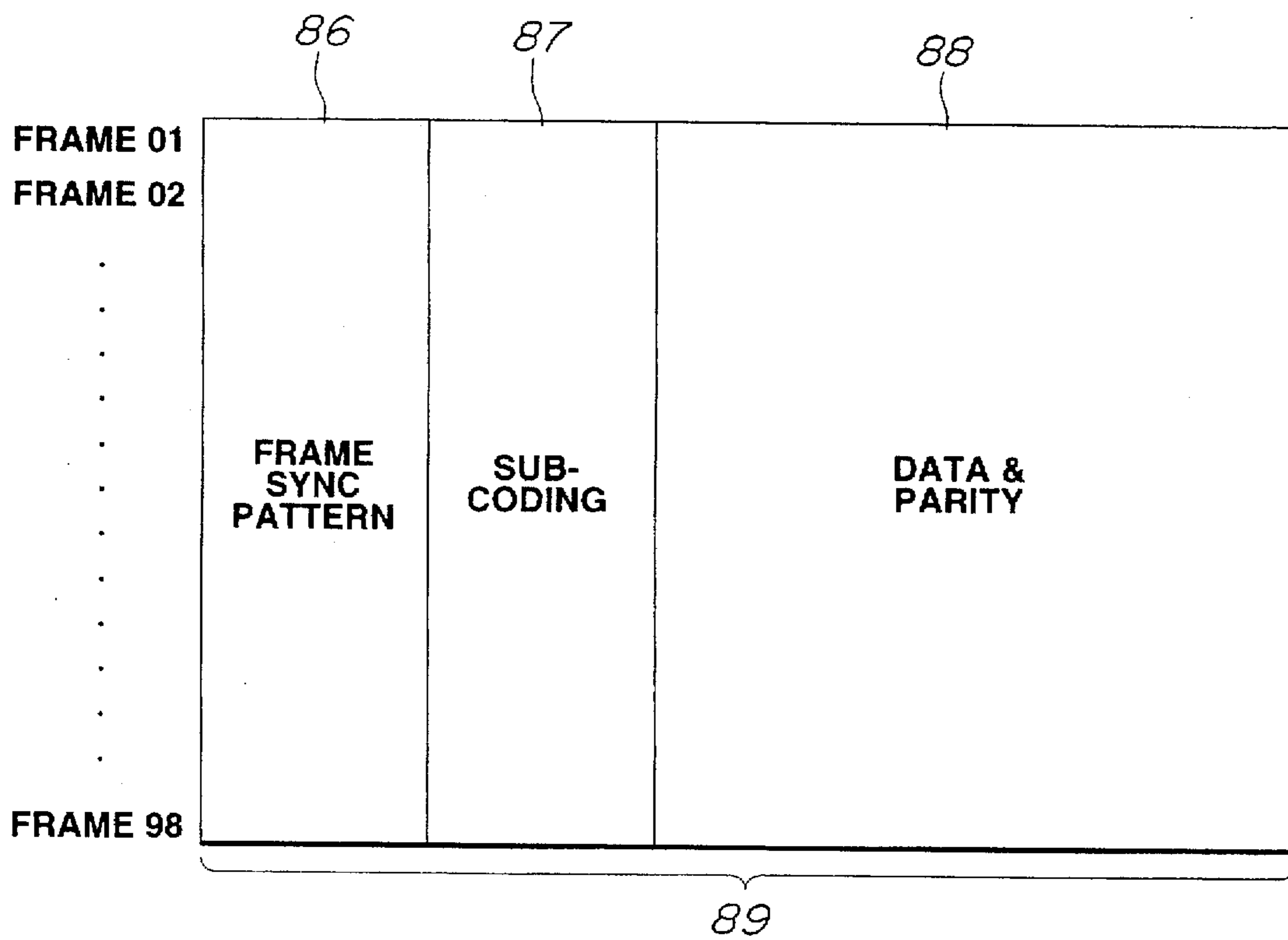
FIG.4 (PRIOR ART)
