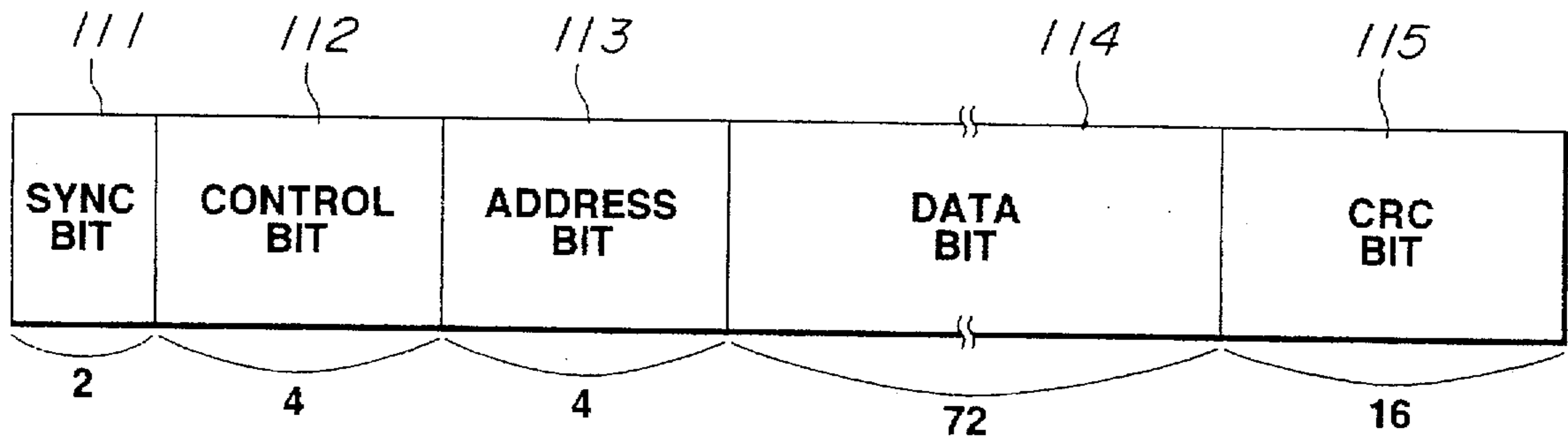
FIG.6 (PRIOR ART)
