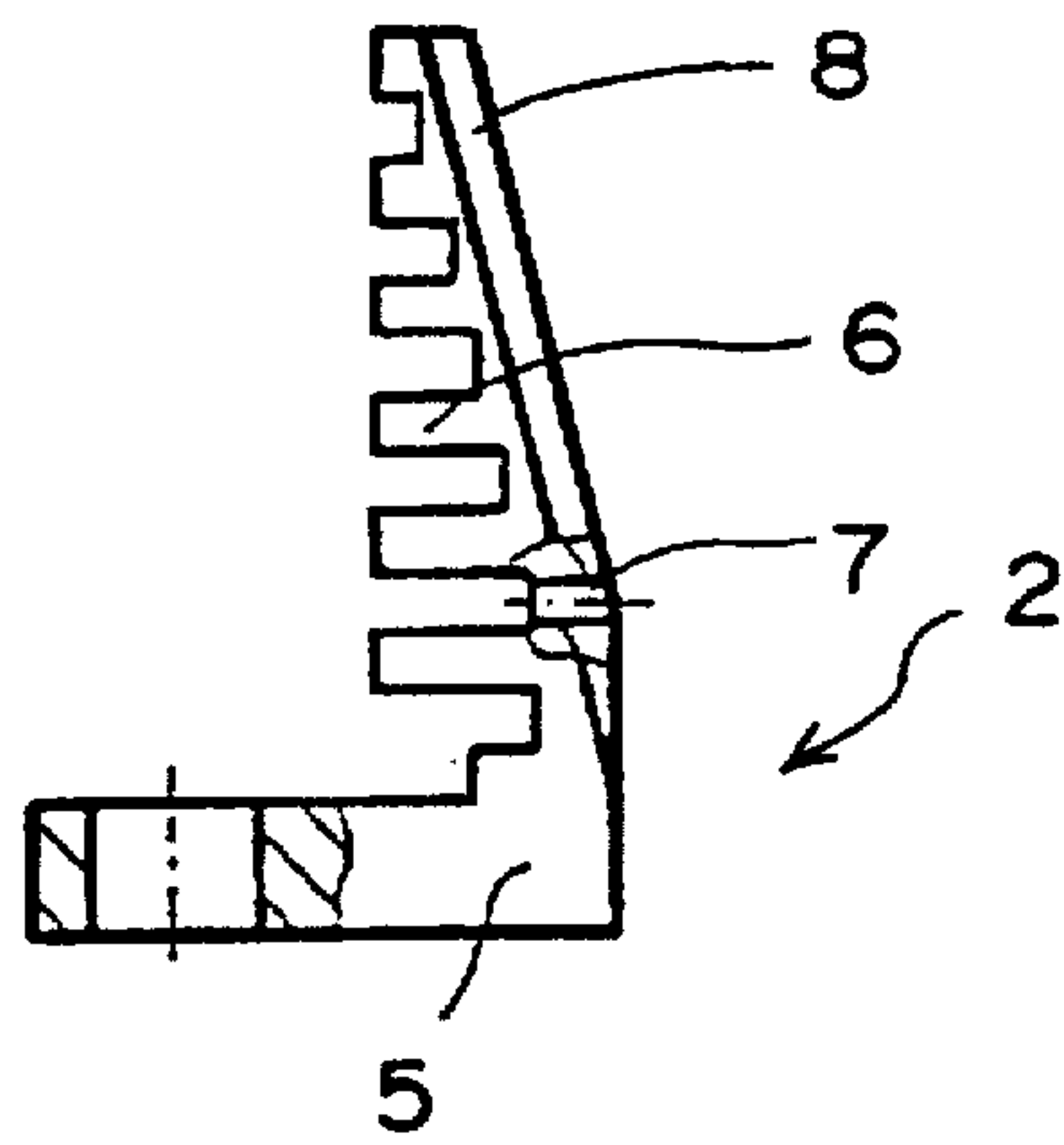
FIG. 1 (PRIOR ART)
