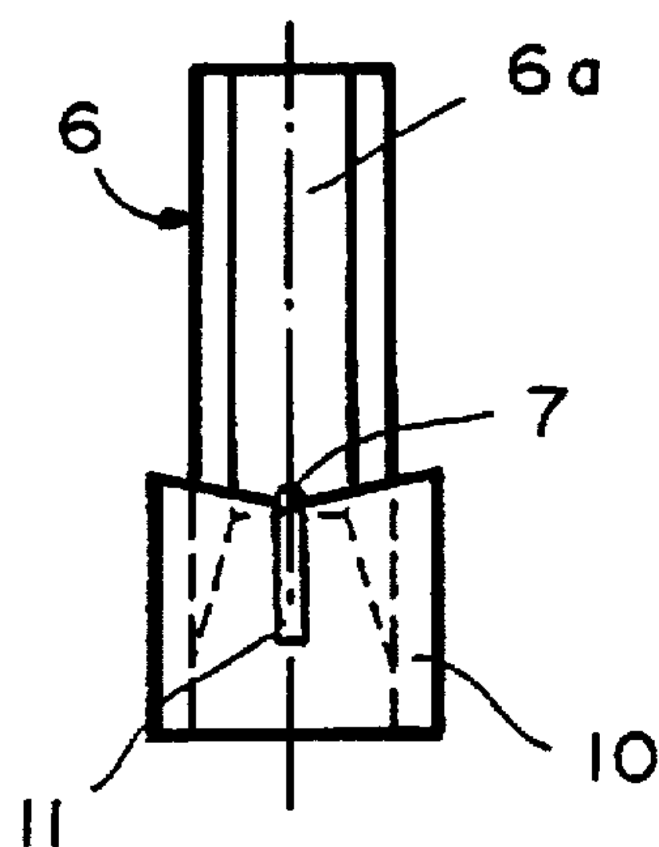
FIG. 4 (PRIOR ART)
