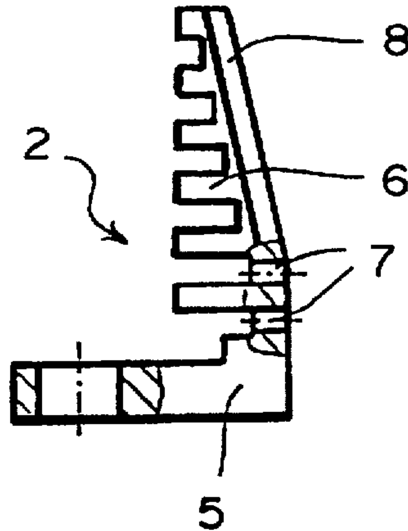
FIG. 2 (PRIOR ART)
