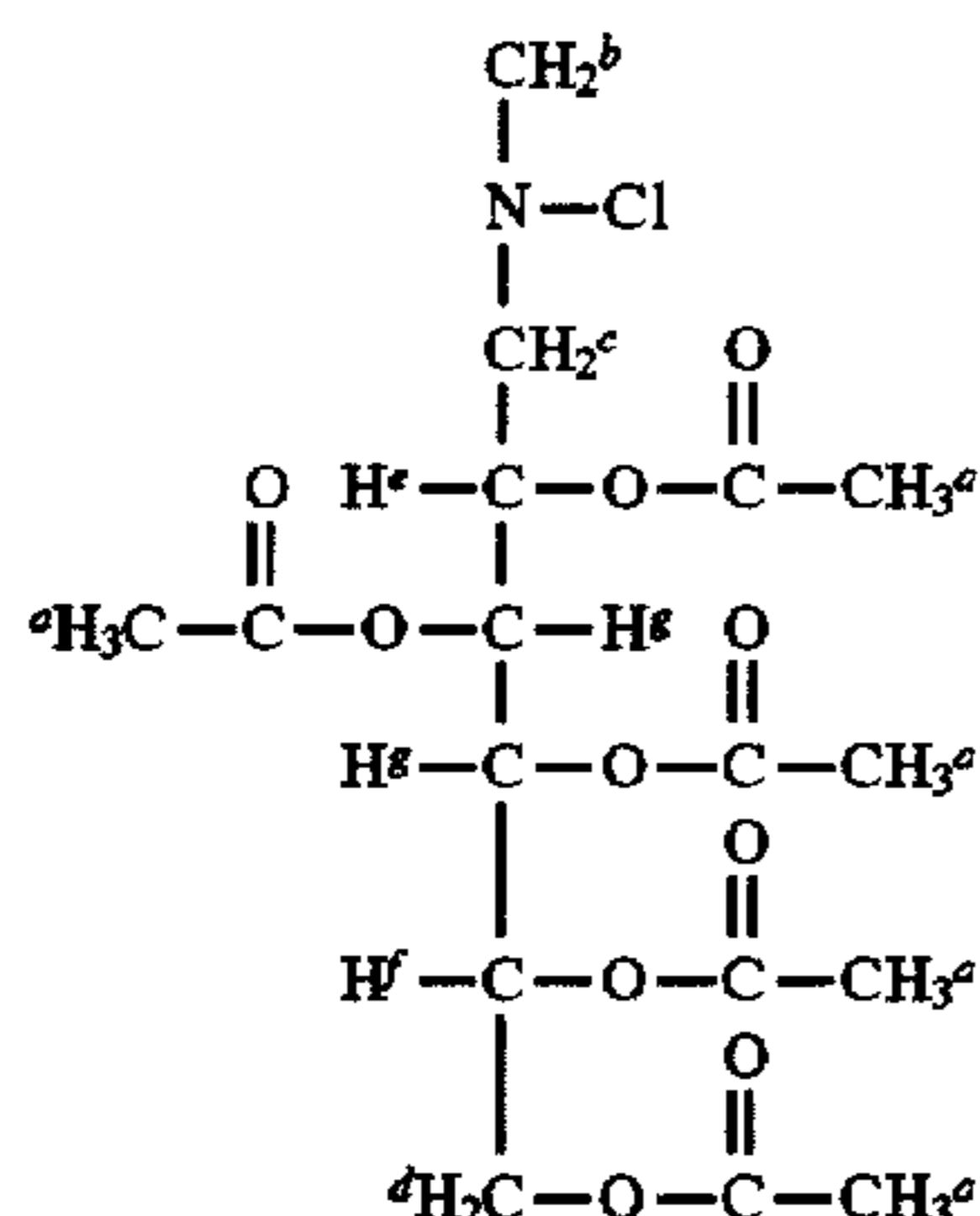
Penta-O-Acetyl-N-Chloro-N-Methylglucamine
