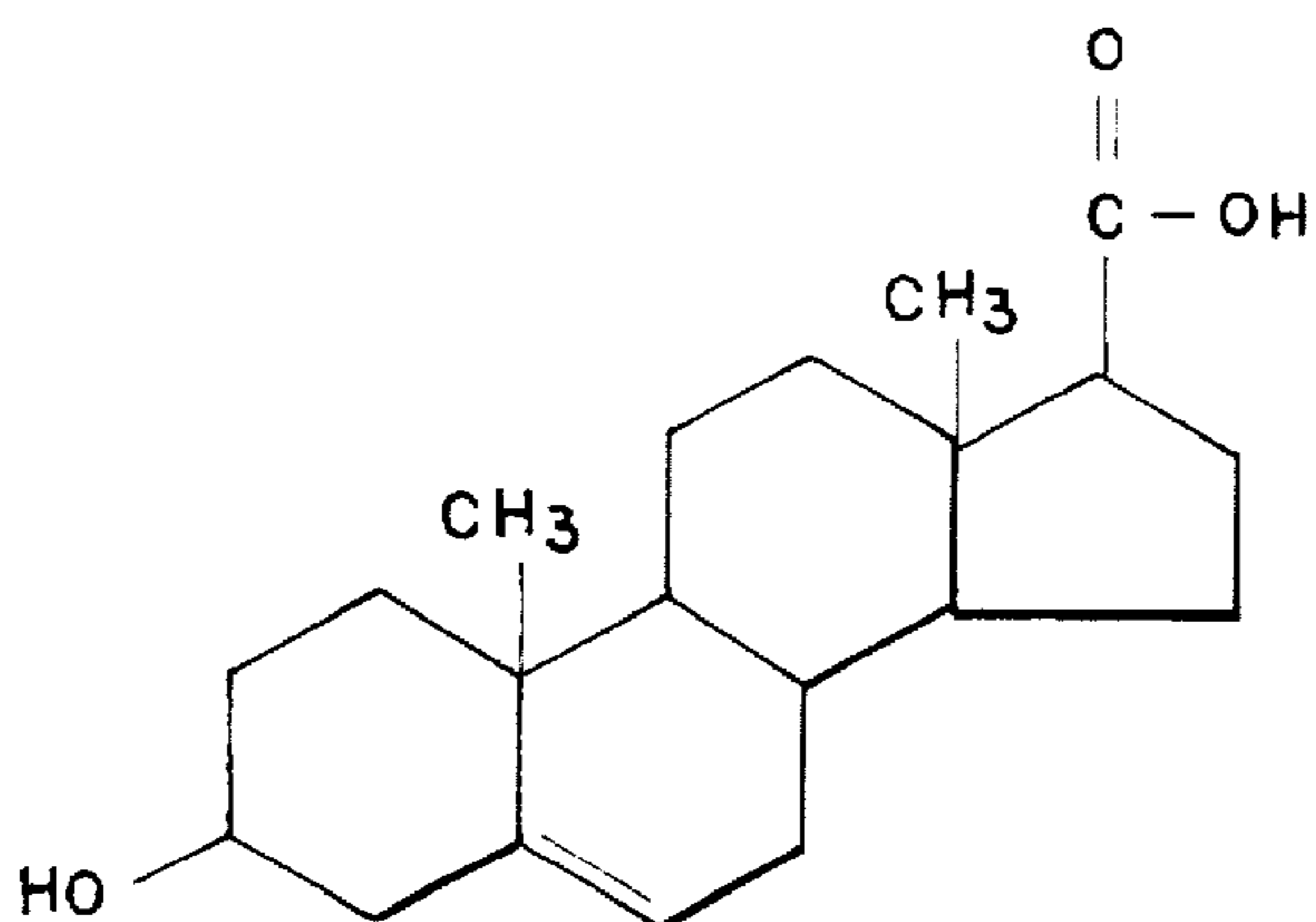
5-ANDROSTEN-3B-OL-17B-CARBOXYLIC ACID
