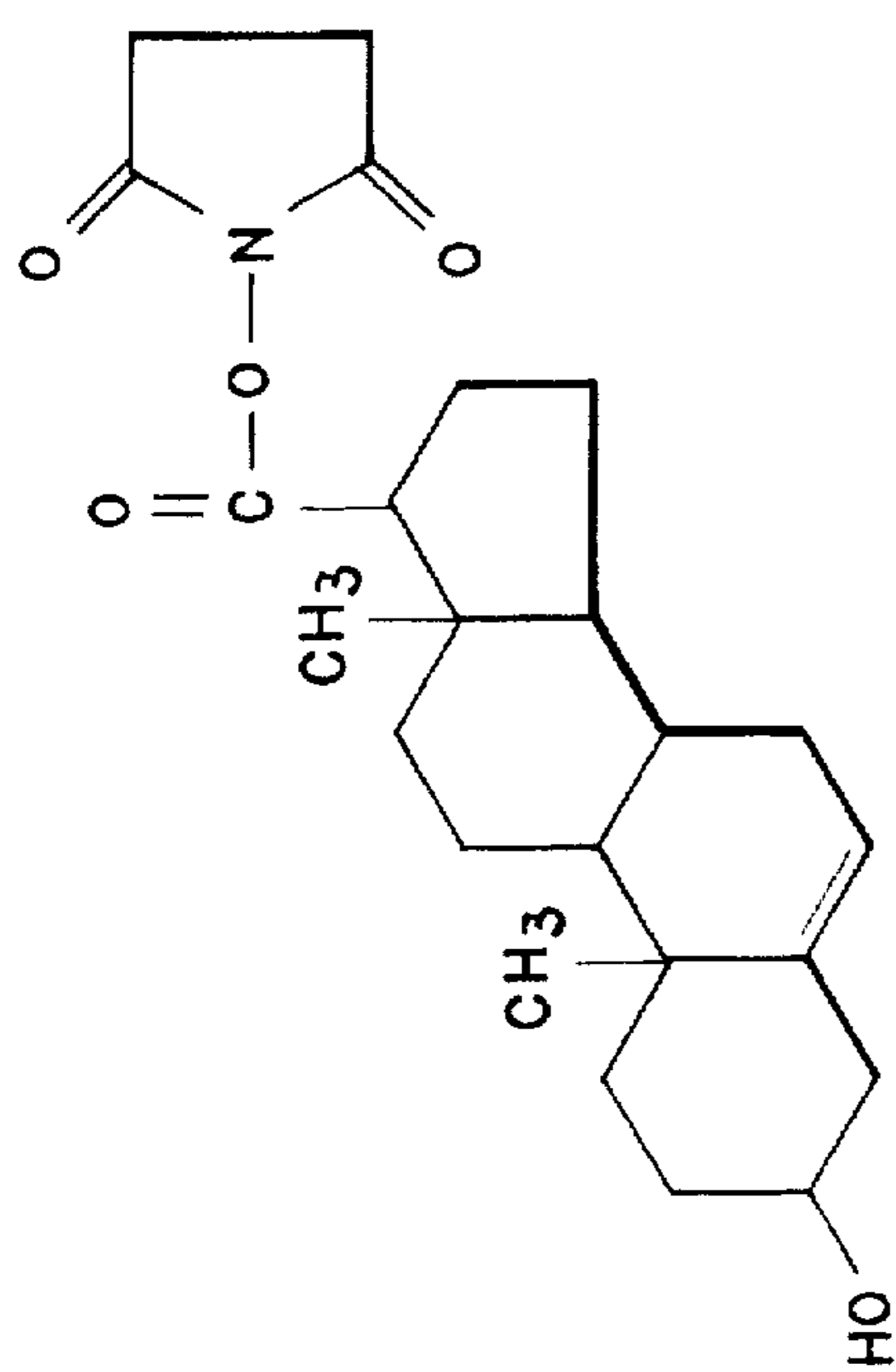
CHOLESTEROL ESTER
