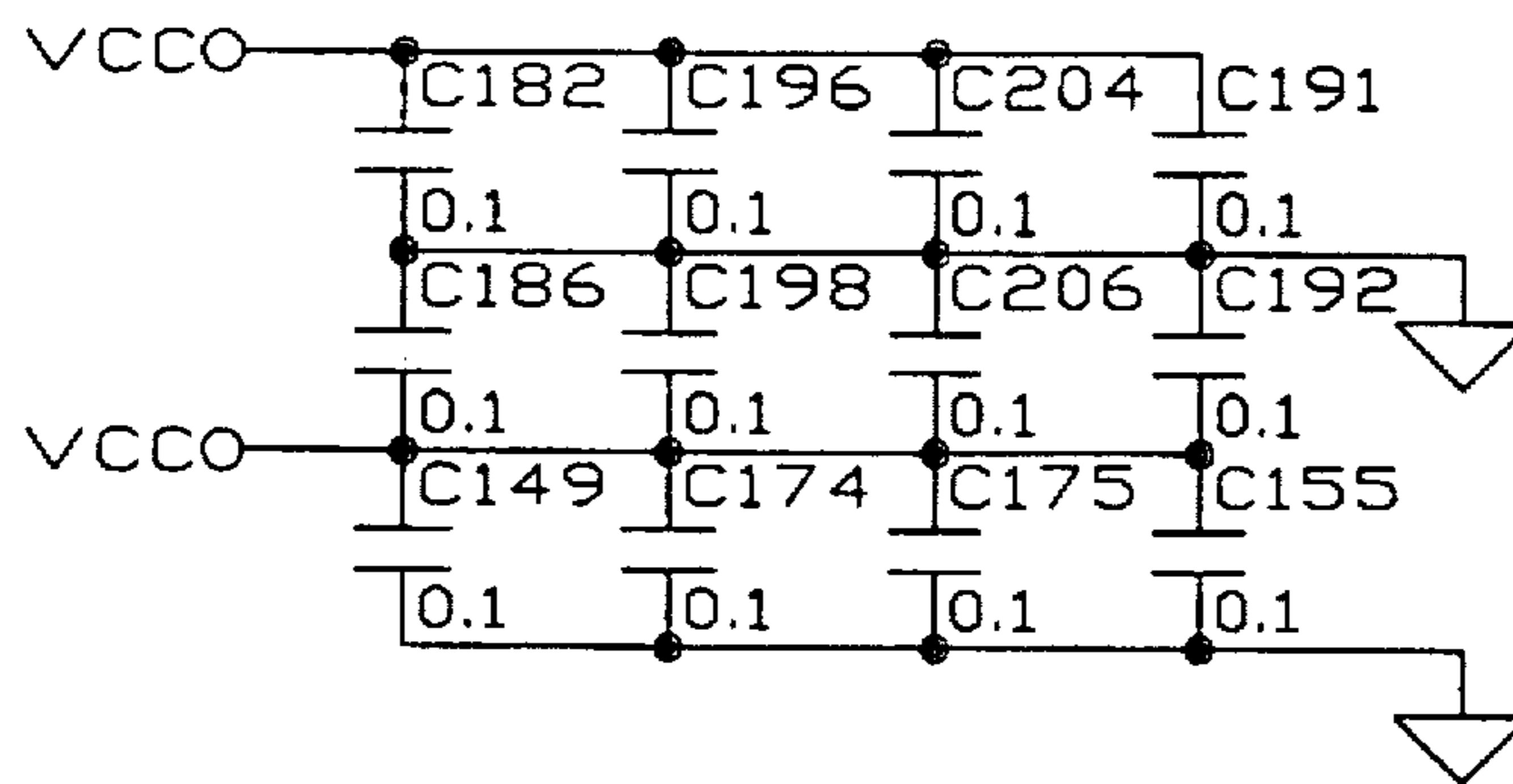
DECOUPLING FOR MACH435'S FOR PINS 2,21,42,63
