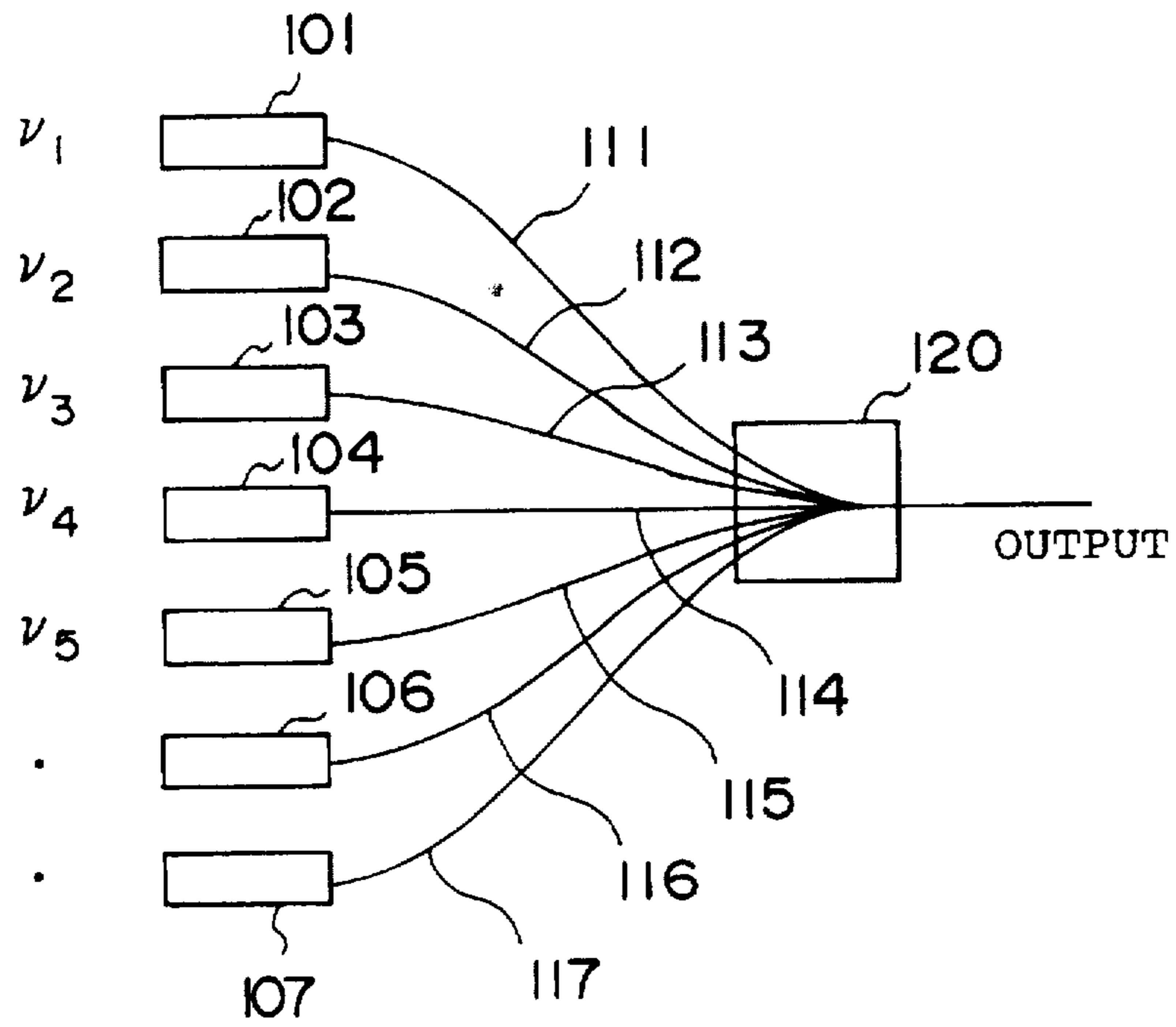
FIG.1 (Prior Art)
