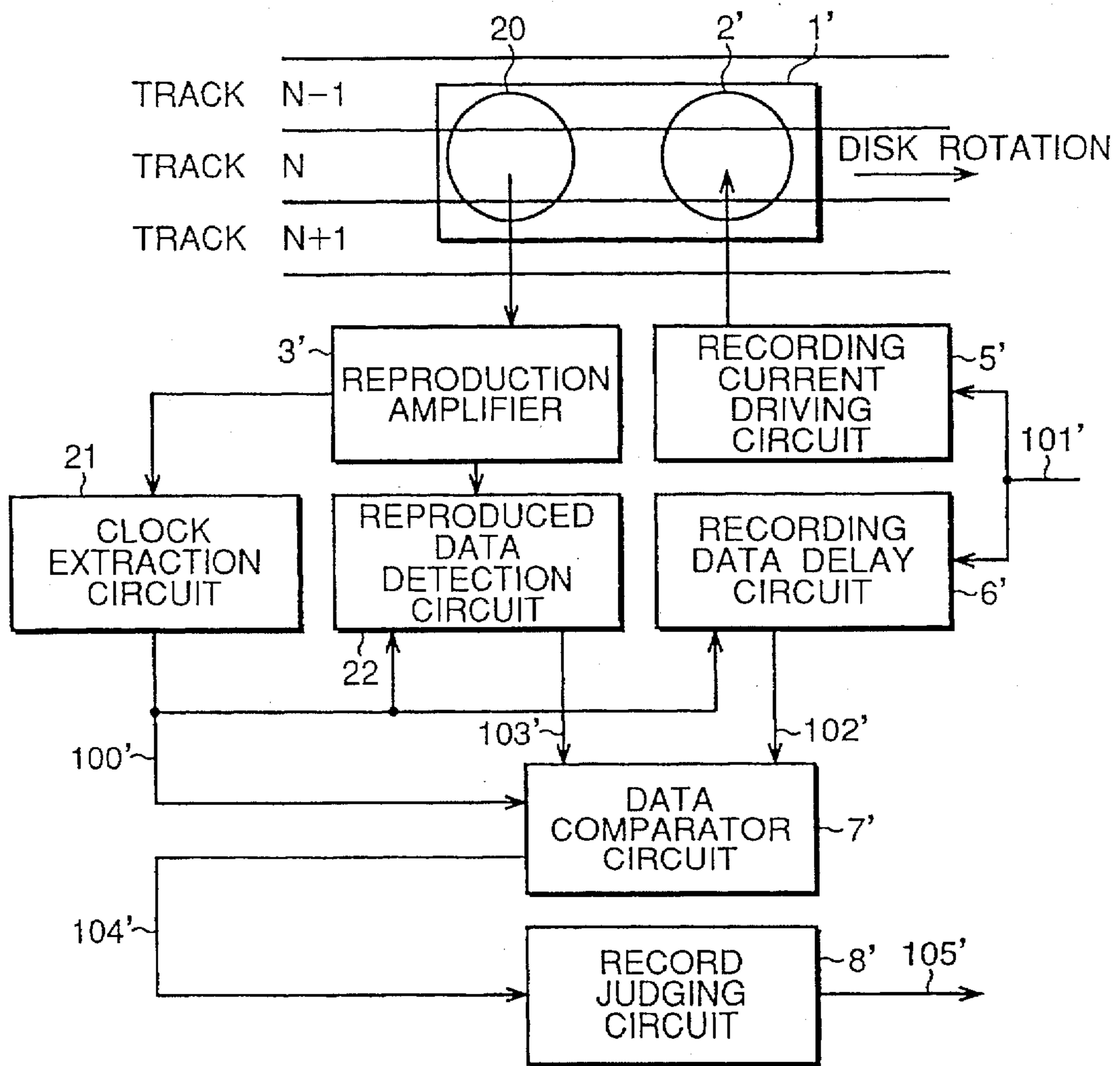
FIG. 1 PRIOR ART
