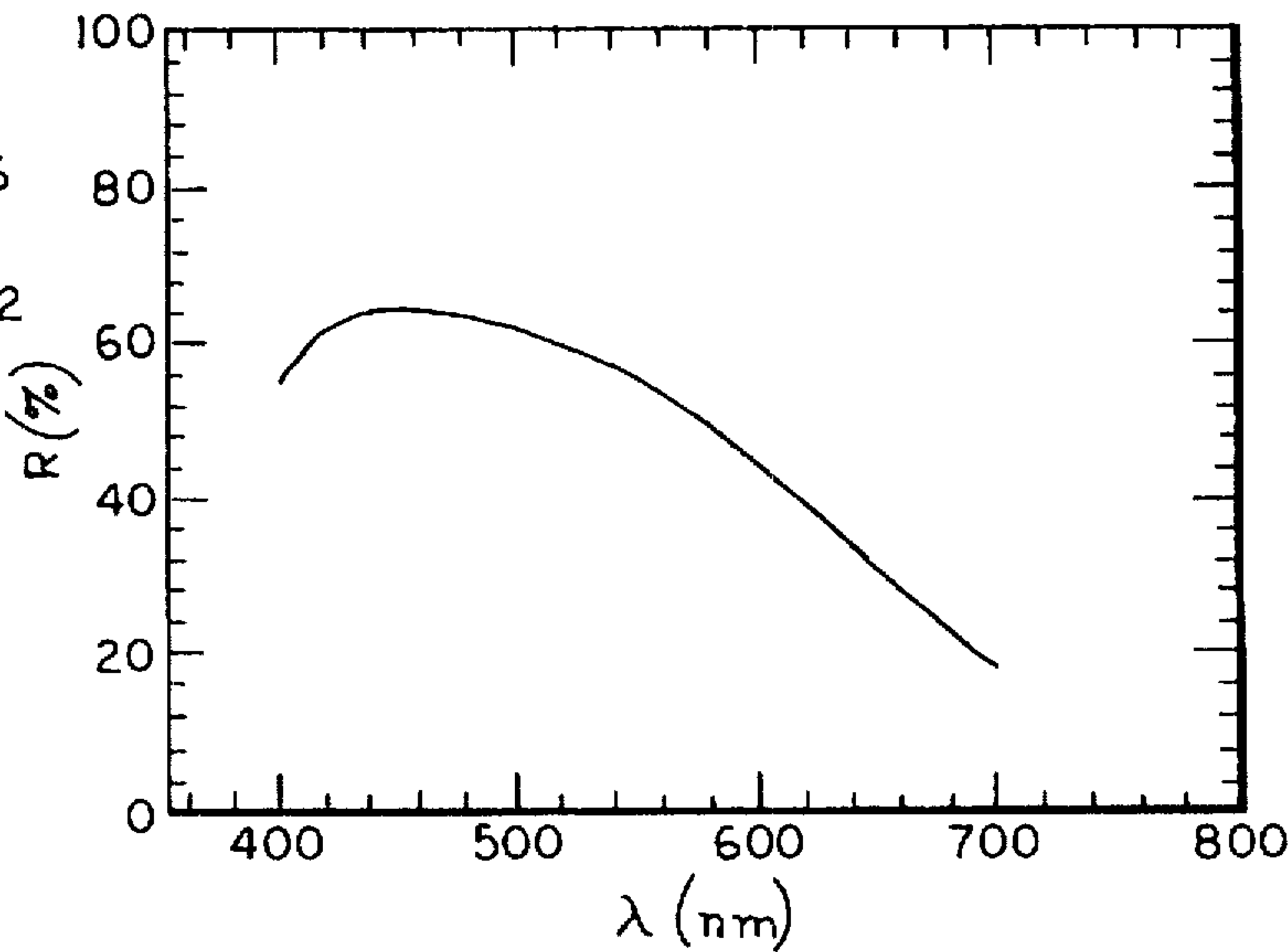
FIG.13 (PRIOR ART)
