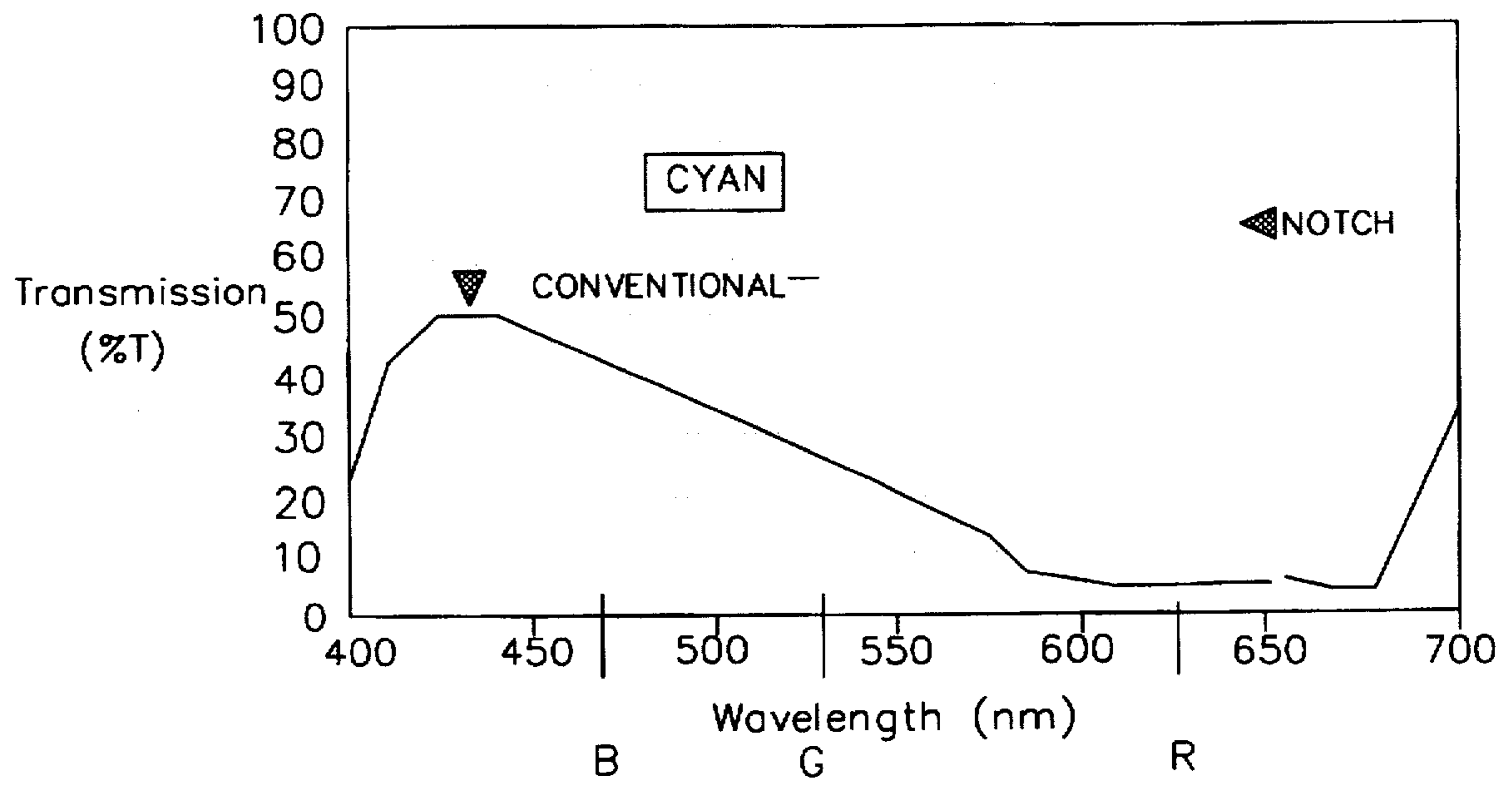
Conventional vs. notch polarizer
