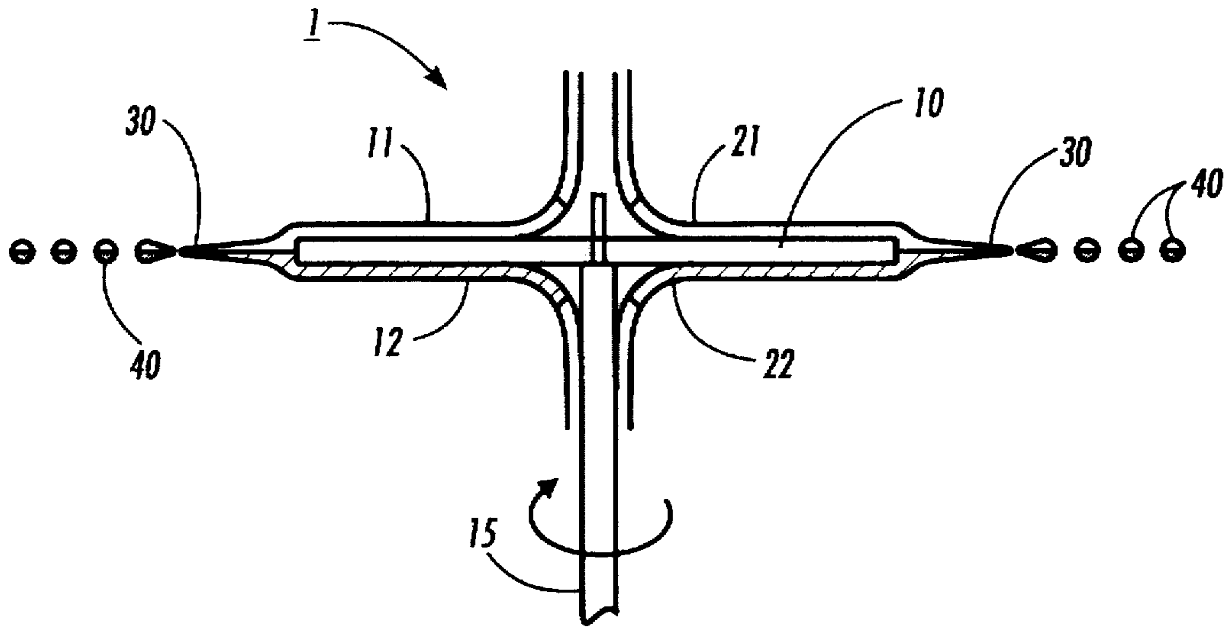
FIG. 1 (Prior Art)
