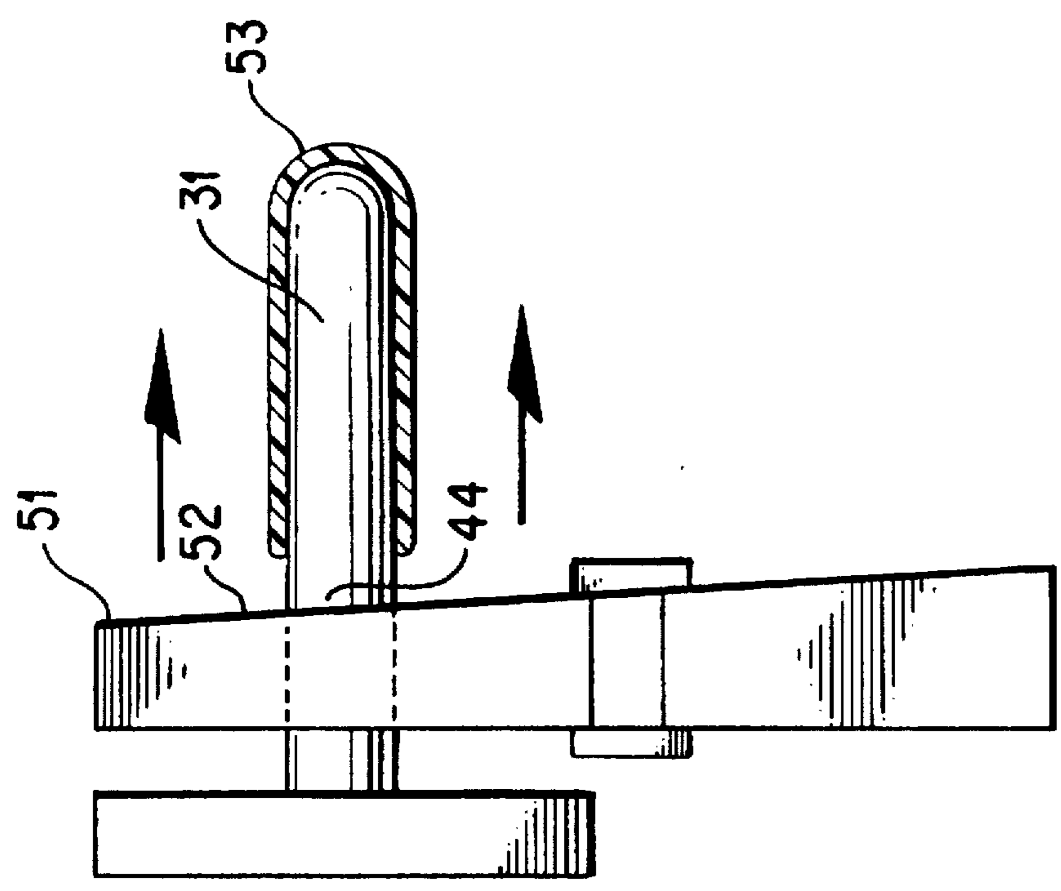
FIG. 5 (PRIOR ART)
