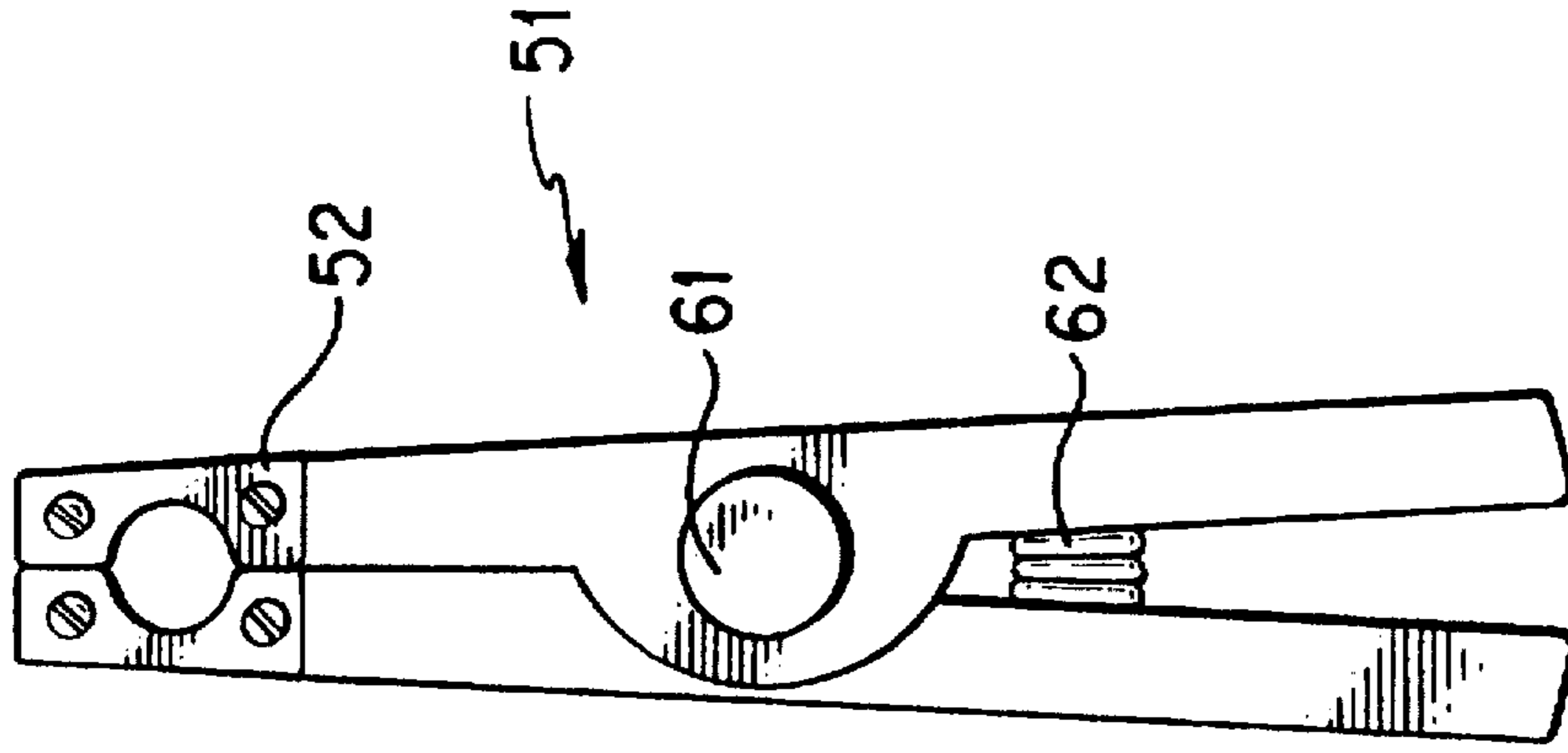
FIG. 6 (PRIOR ART)
