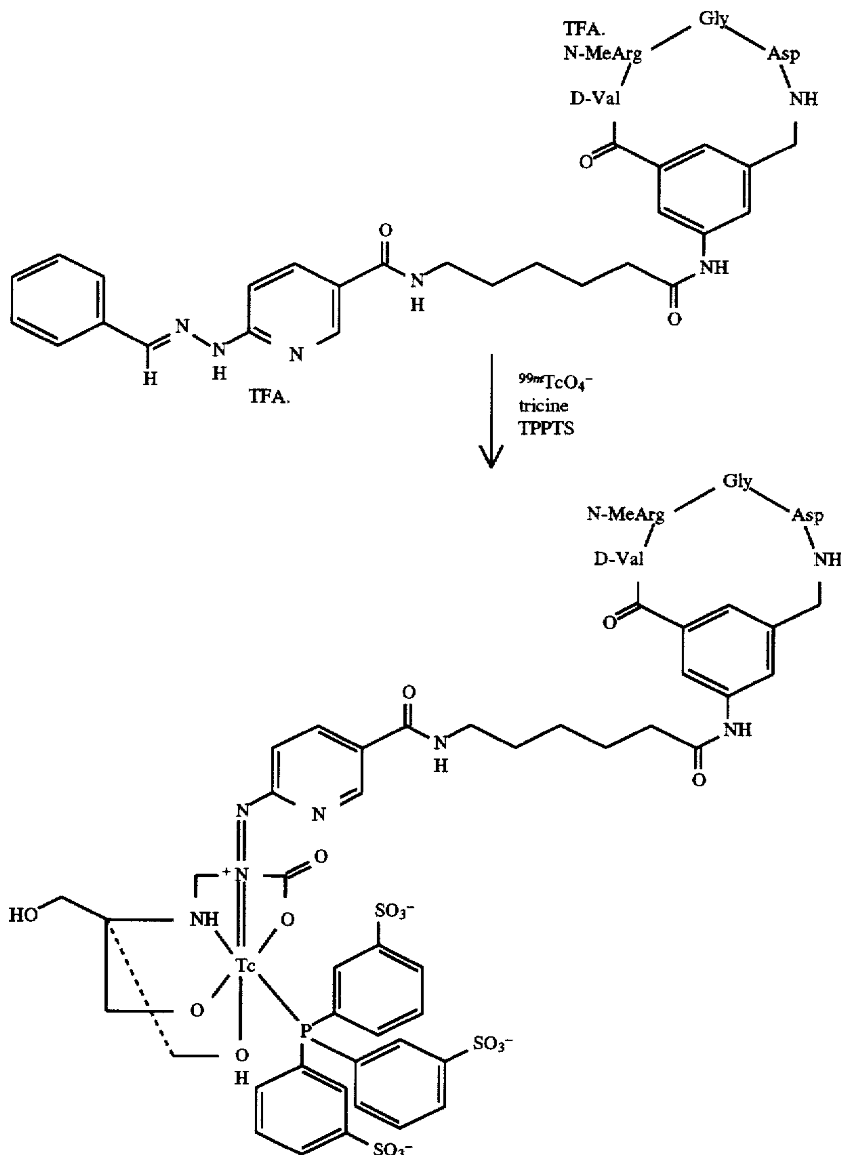
Scheme 6
