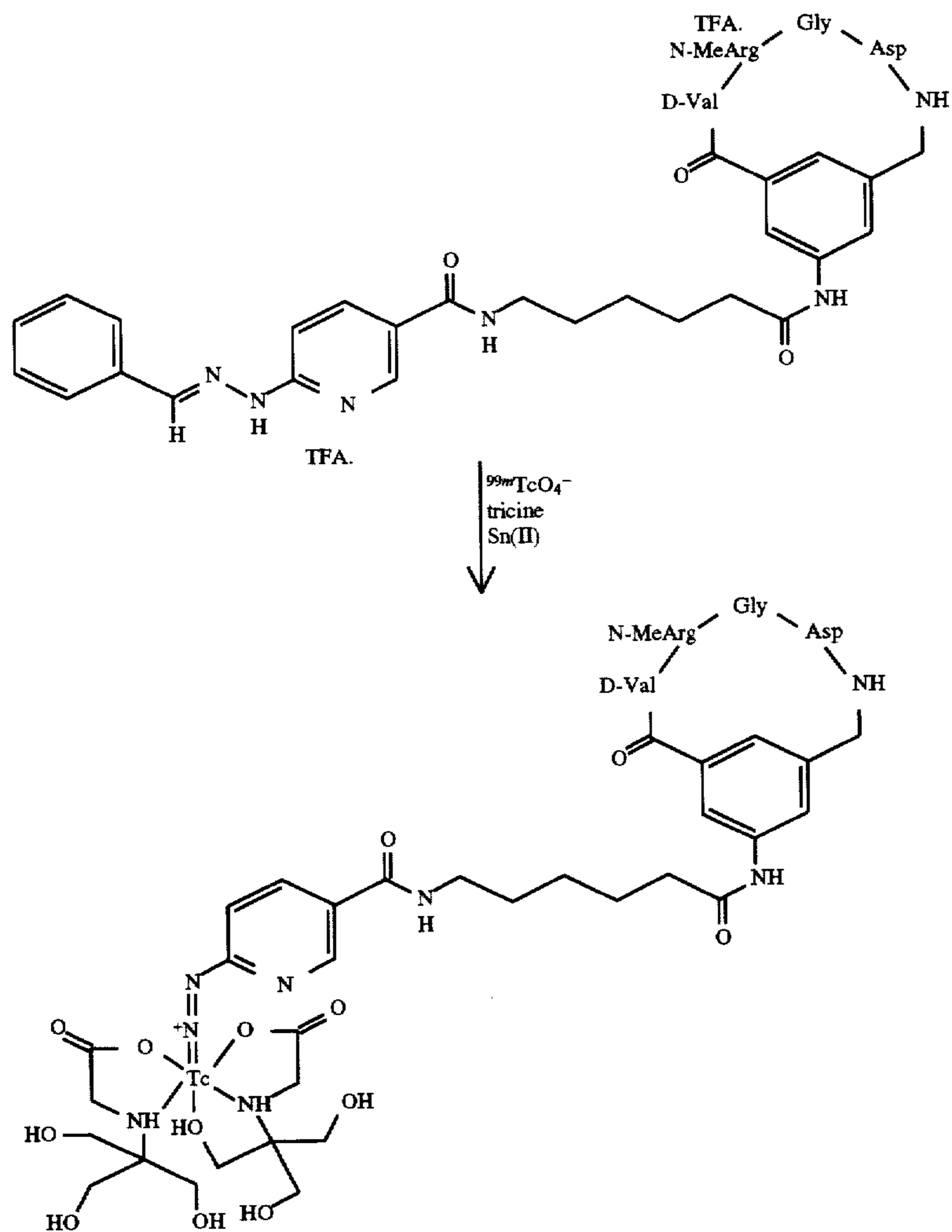
Scheme 5.
