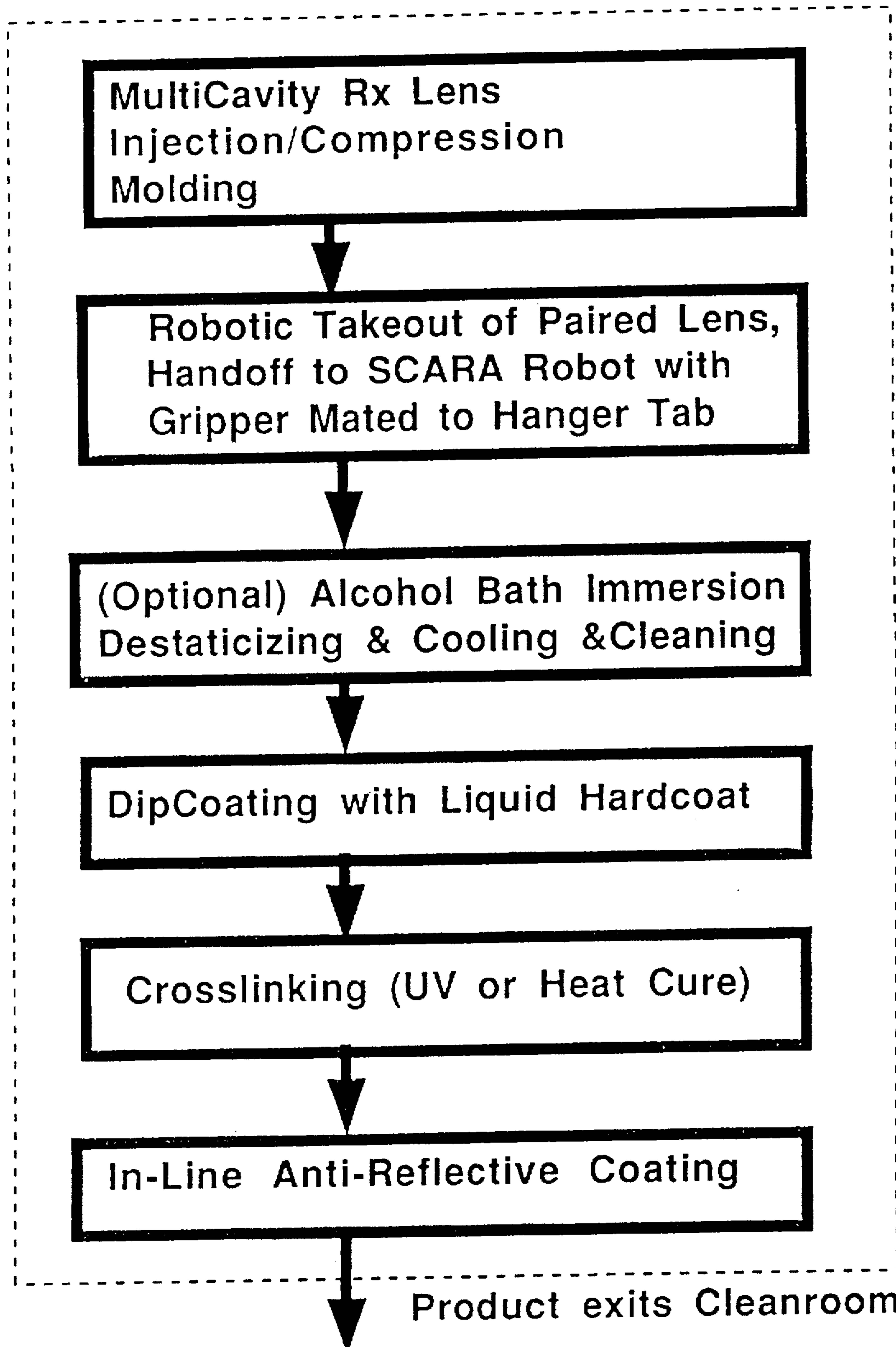
Figure 4D: In-Line Automated AR Vacuum Coat of "Mold and Dipcoat" ("Continuous Process")
