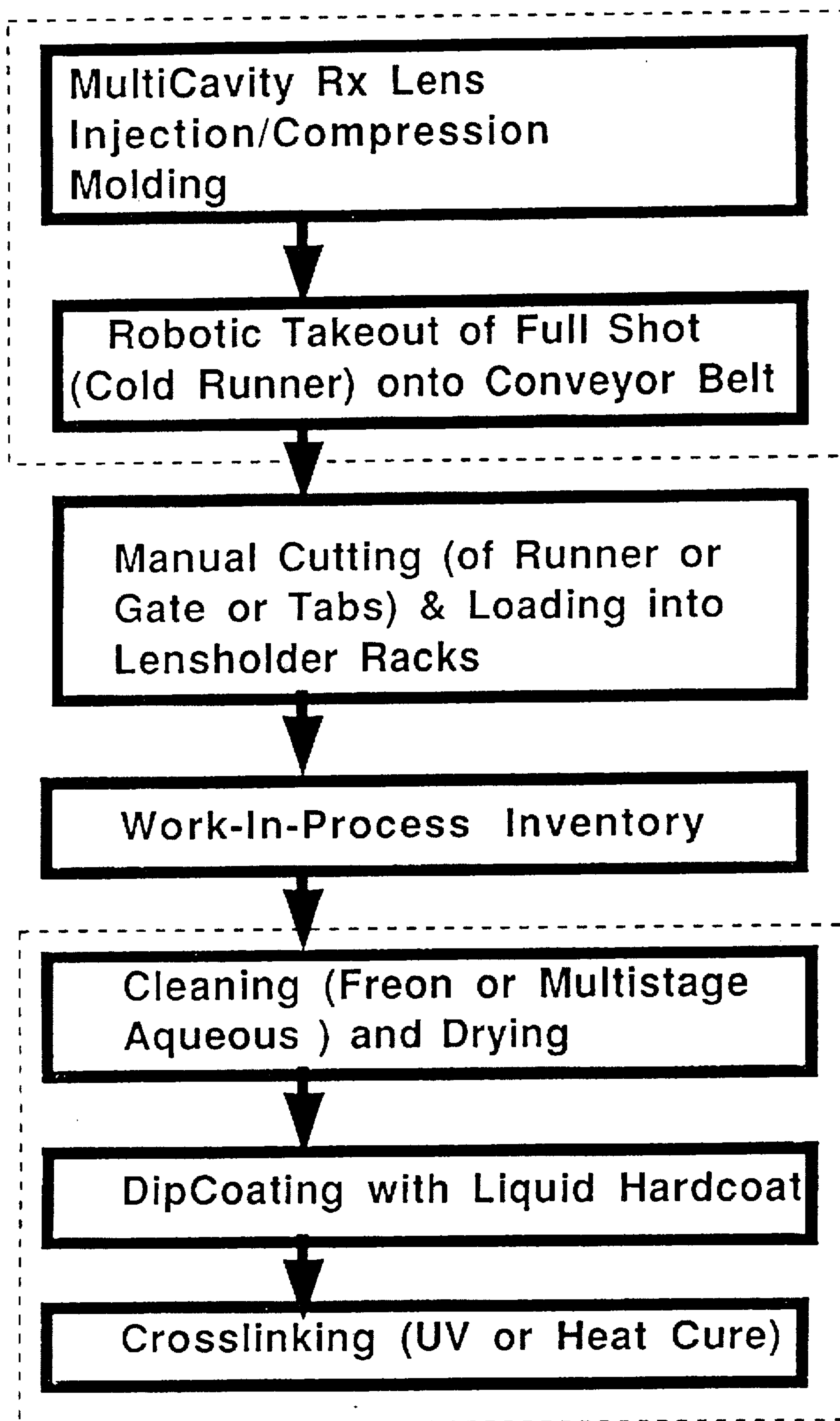
Figure 4A: Comparative Example ("Batch Process")
