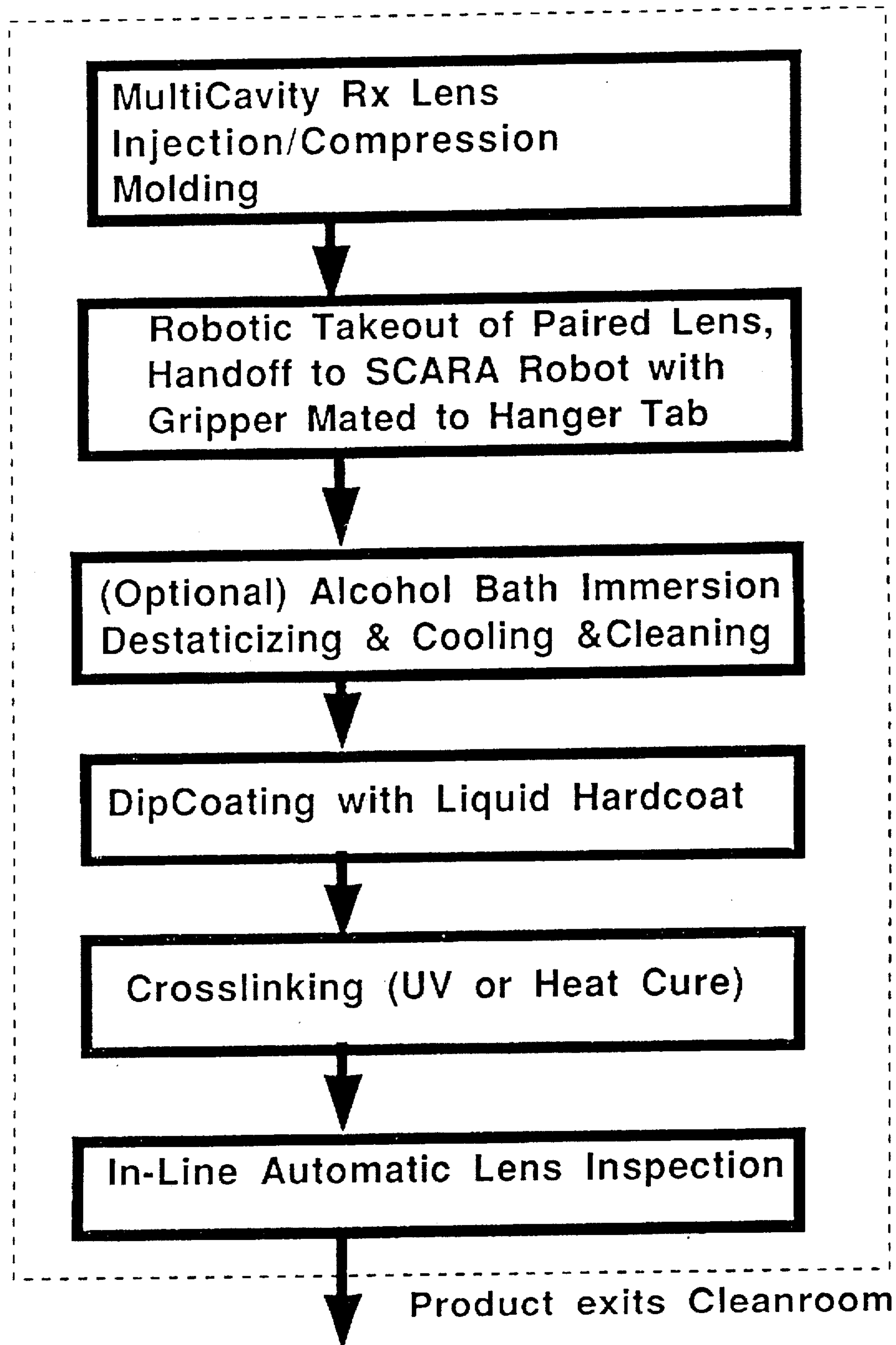
Figure 4C: In-Line Automated Inspection of "Mold and Dipcoat" ("Continuous Process")
