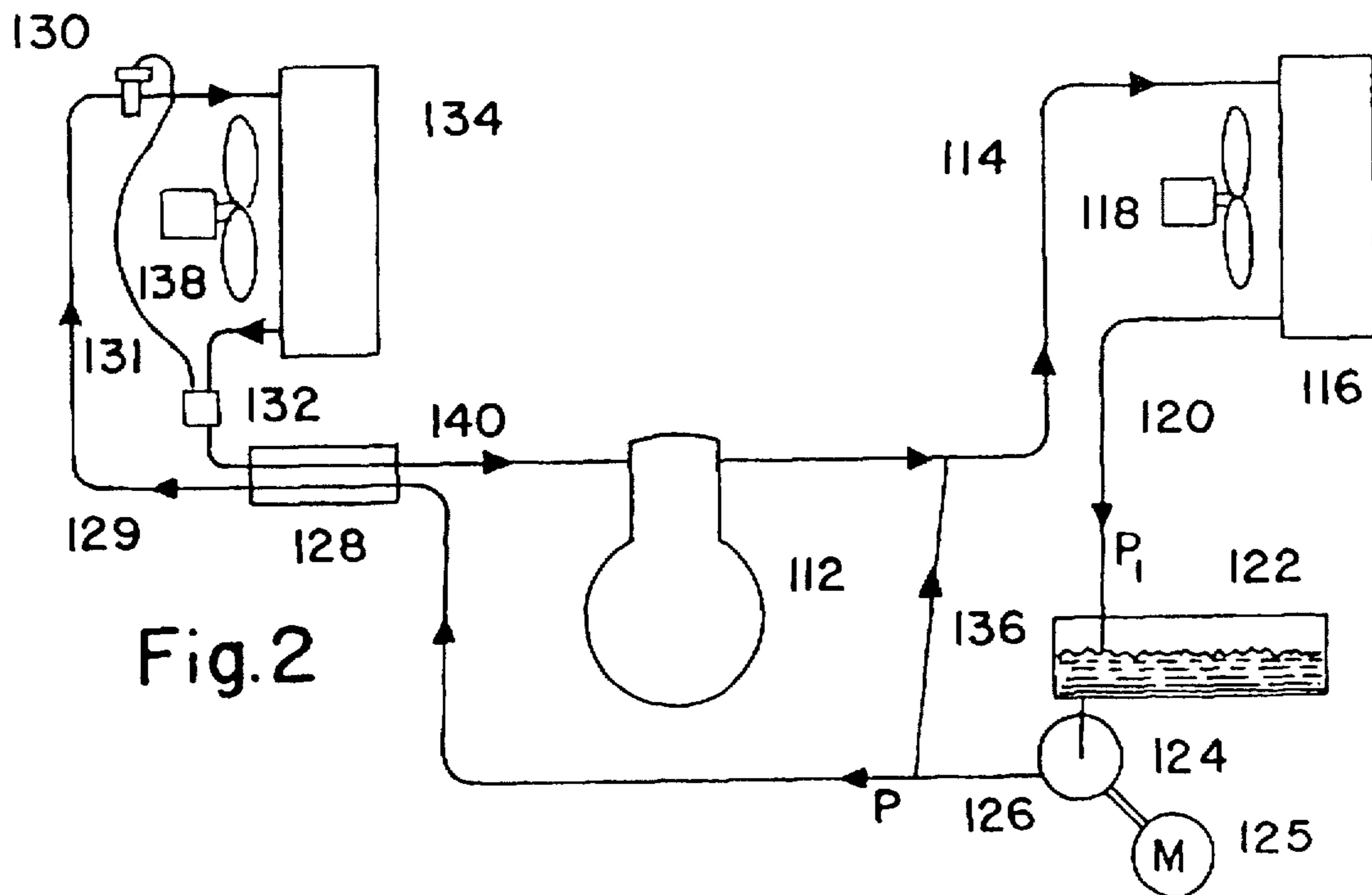
FIG. 2 (PRIOR ART)
