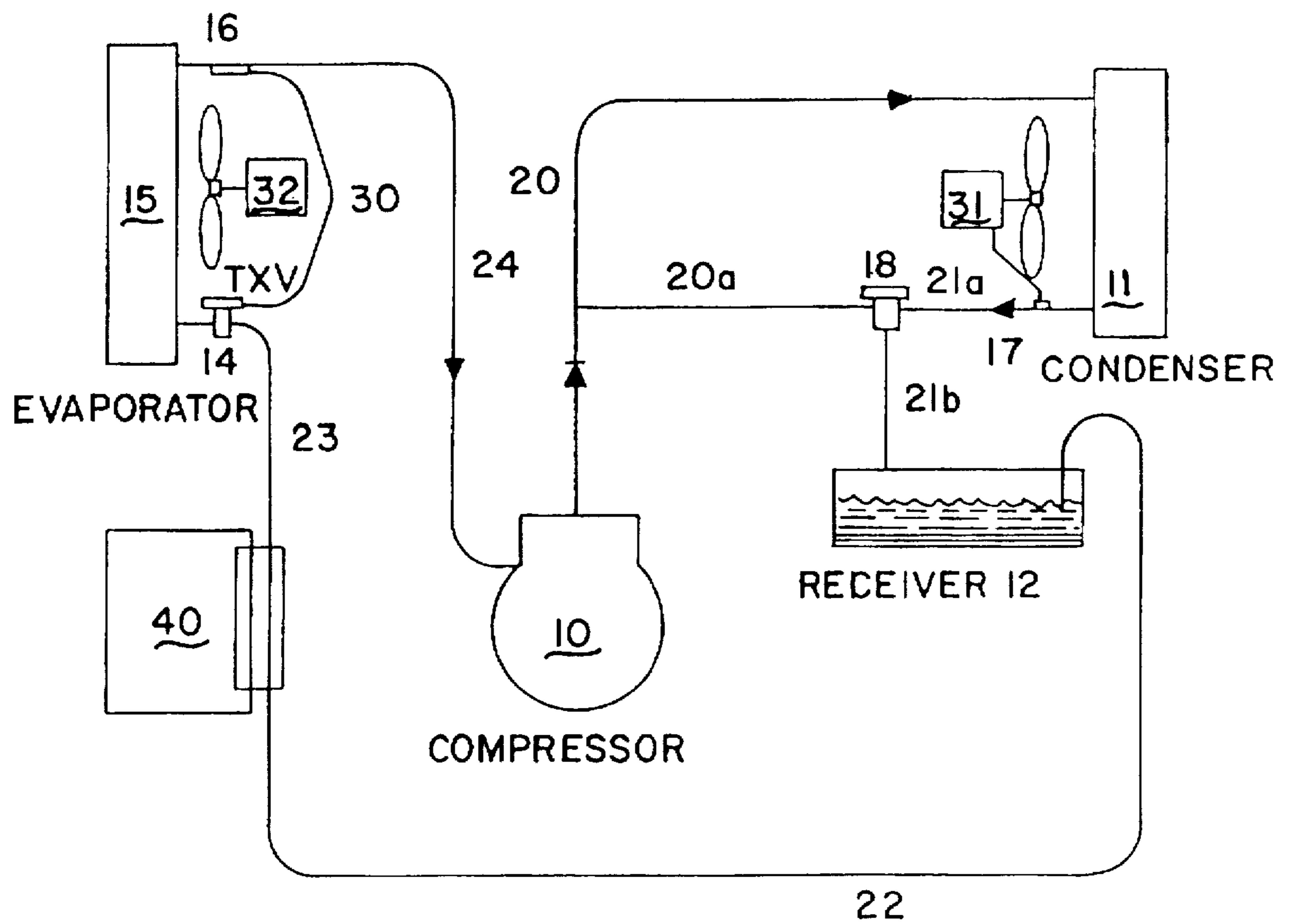
FIG. 1 (PRIOR ART)
