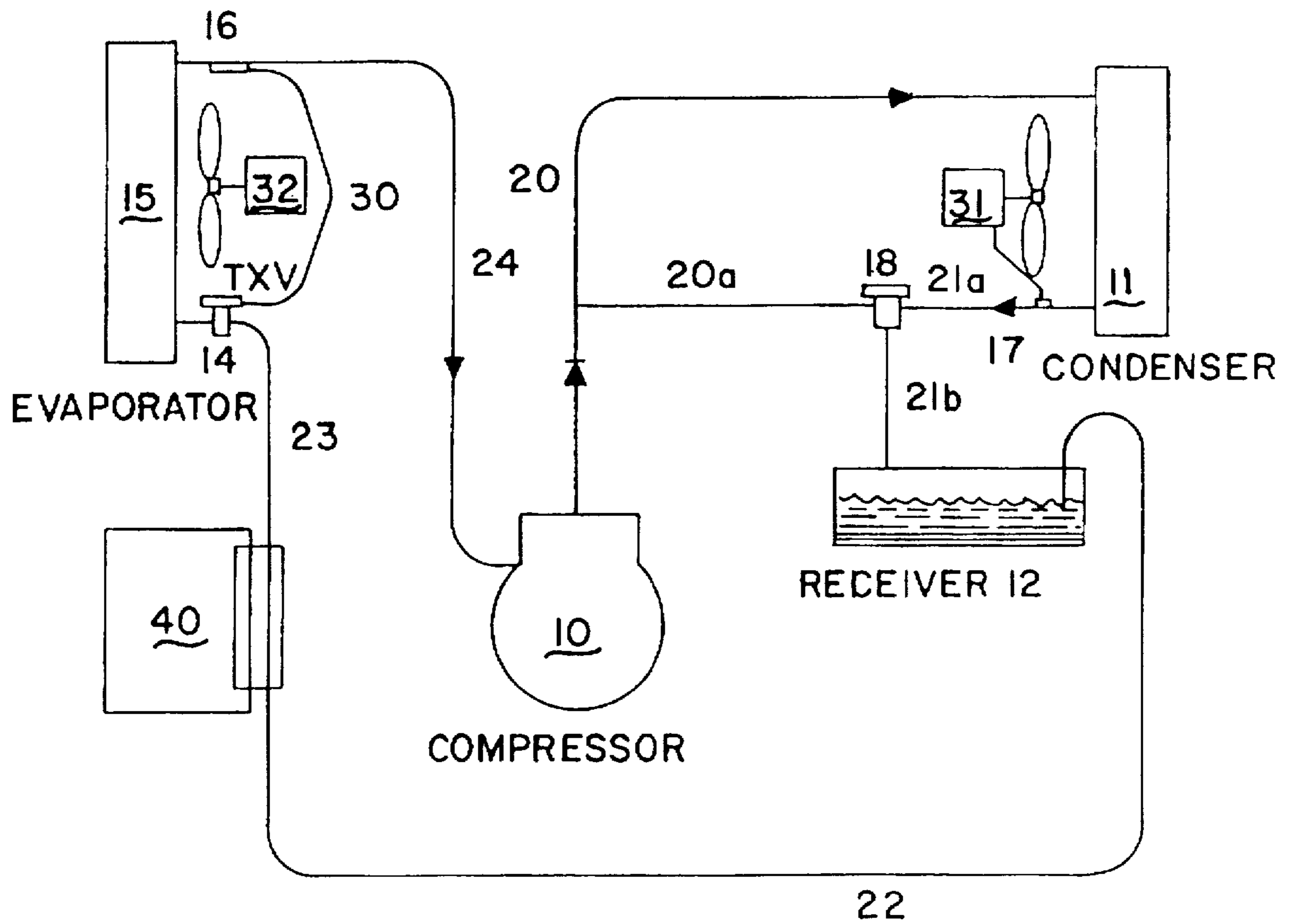
FIG. 1 (PRIOR ART)
