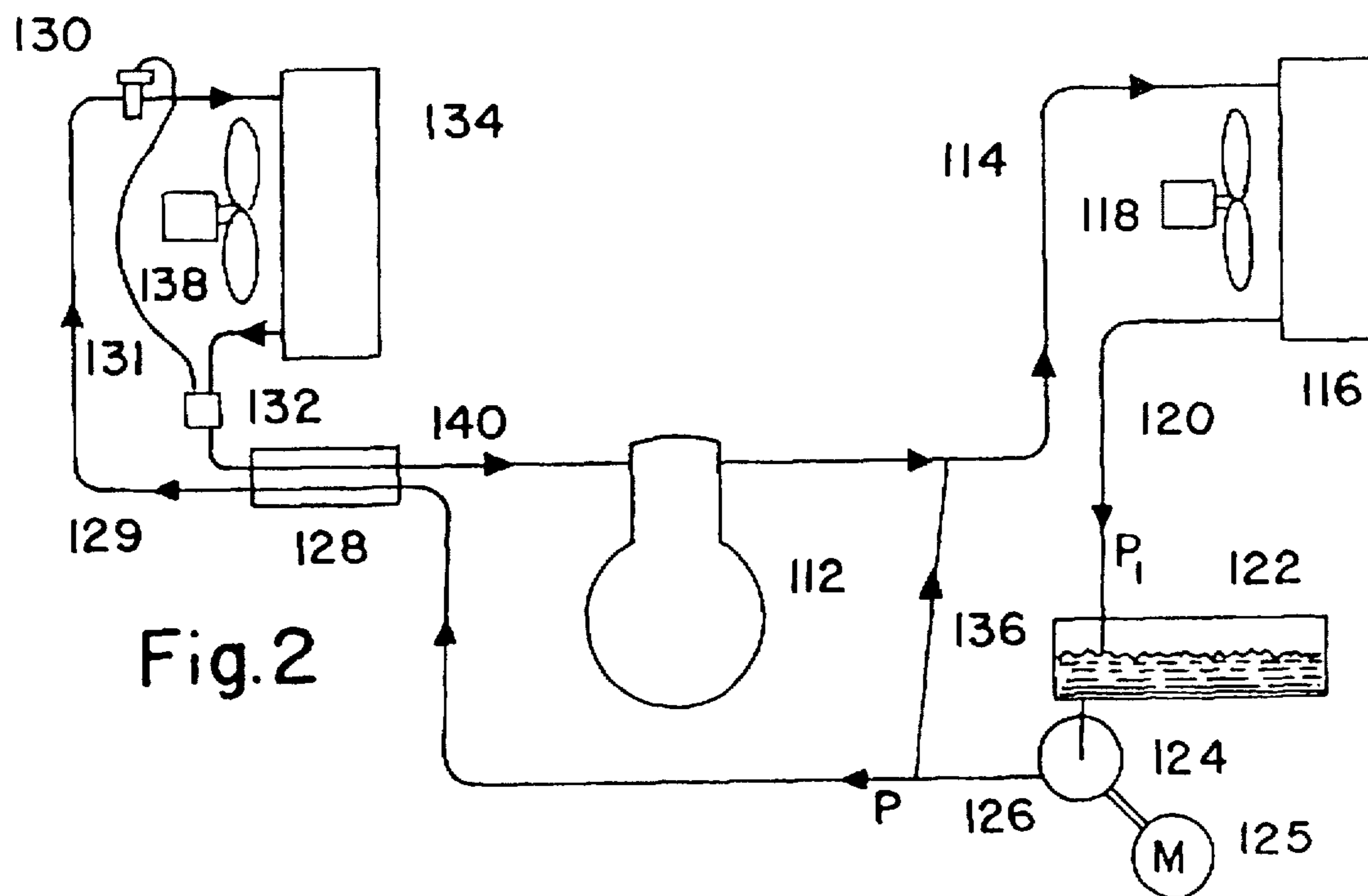
FIG. 2 (PRIOR ART)
